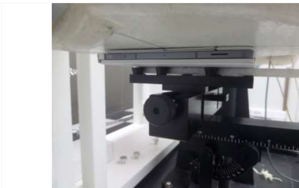
Distance of 0 mm from the EUT with Cover Variant 2
