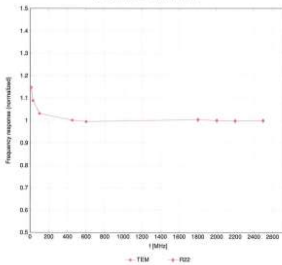
Frequency Response of E-Field (TEM-Cell:R110 EXX, Waveguide:R22)
