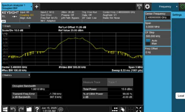
6 dB Bandwidth plot (High-CH 39)
