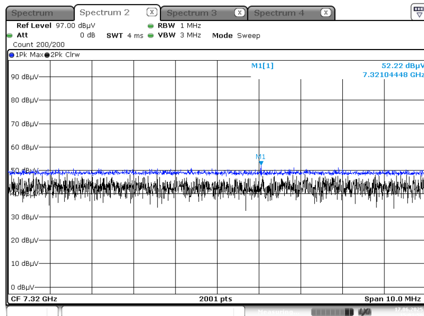
Radiated Spurious Emissions plot – Peak Result (Ch.17 3rd Harmonic)
