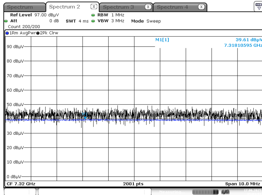
Radiated Spurious Emissions plot – Average Result (Ch.17 3rd Harmonic)
