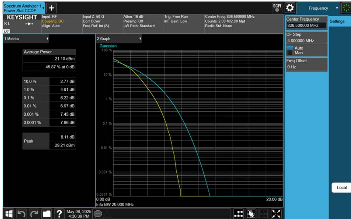
NR26(Part22)_20 M_PAR_Mid_16QAM_FullRB
