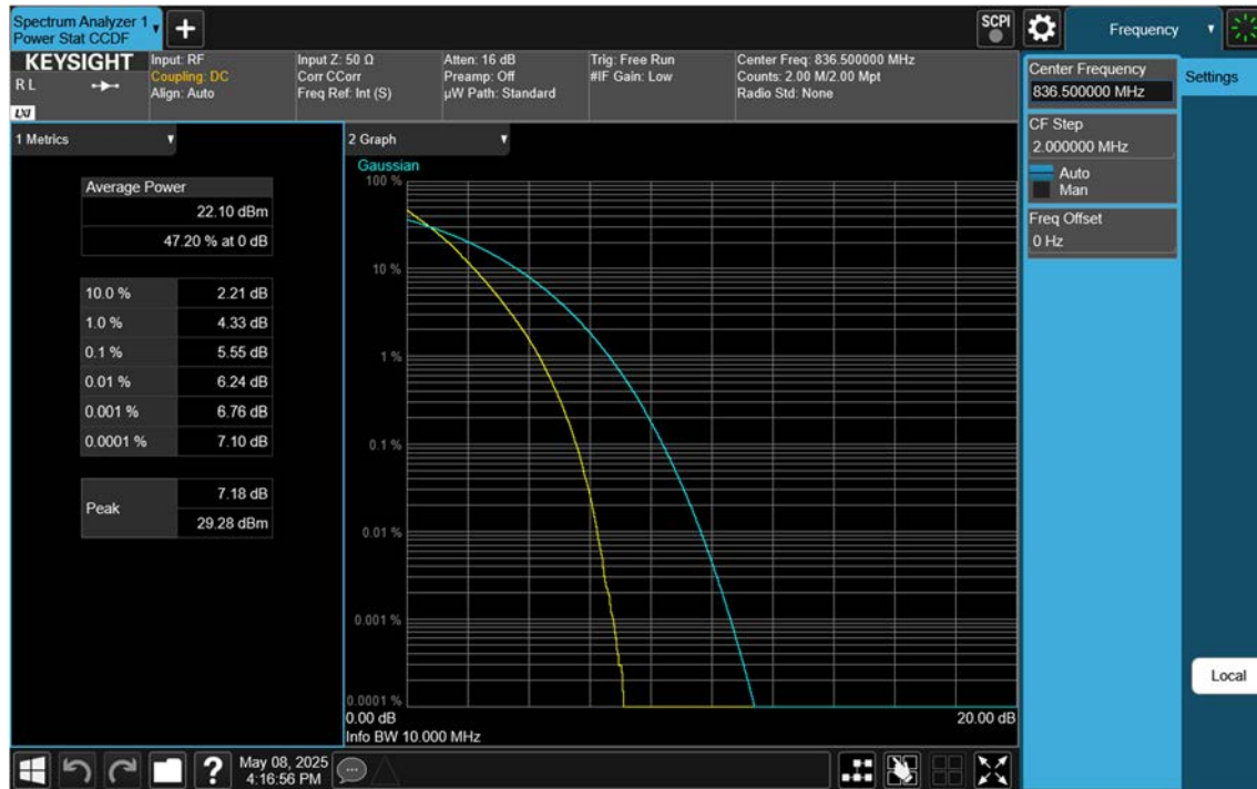
NR26(Part22)_10 M_PAR_Mid_QPSK_FullRB
