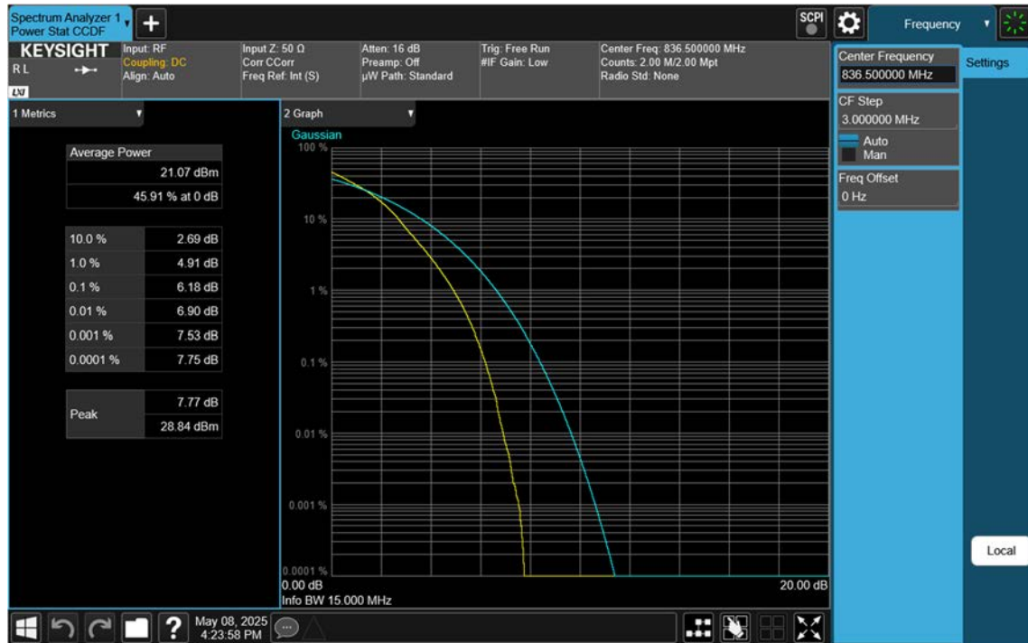
NR26(Part22)_15 M_PAR_Mid_16QAM_FullRB
