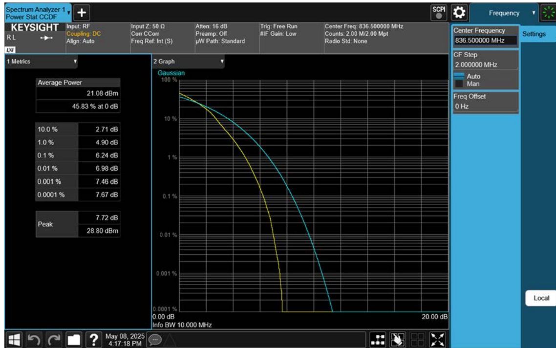
NR26(Part22)_10 M_PAR_Mid_16QAM_FullRB
