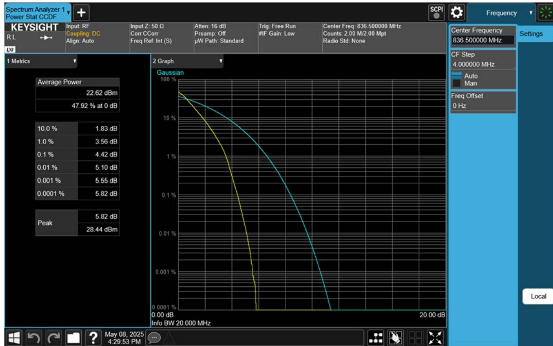
NR26(Part22)_20 M_PAR_Mid_BPSK_FullRB
