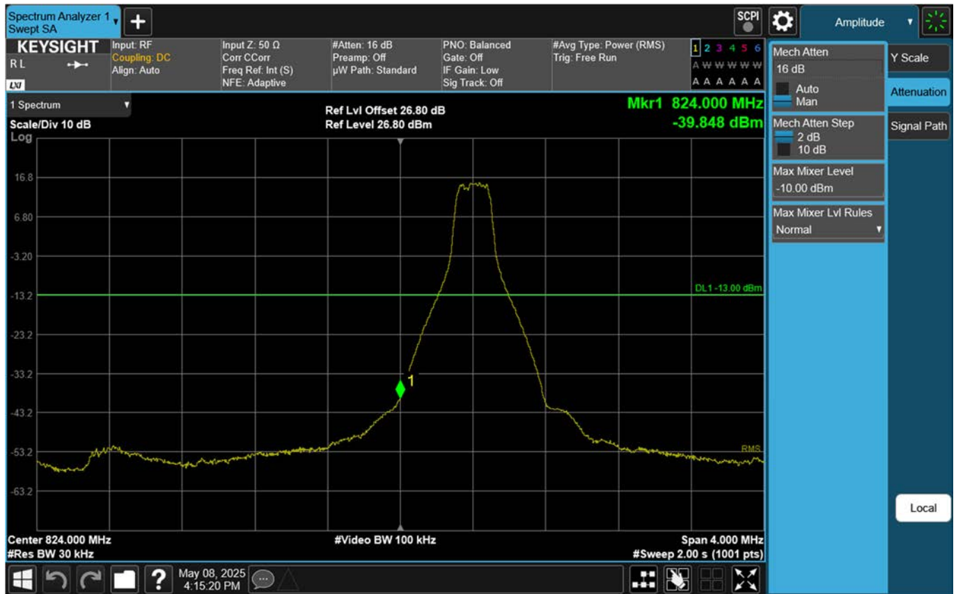
Lower Band Edge Plot (10 M BW Ch.165800 BPSK_RB 1_Offset 0)
