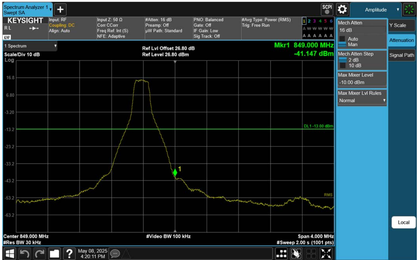
Upper Band Edge Plot (10 M BW Ch.168800 BPSK_RB 1_Offset 49)
