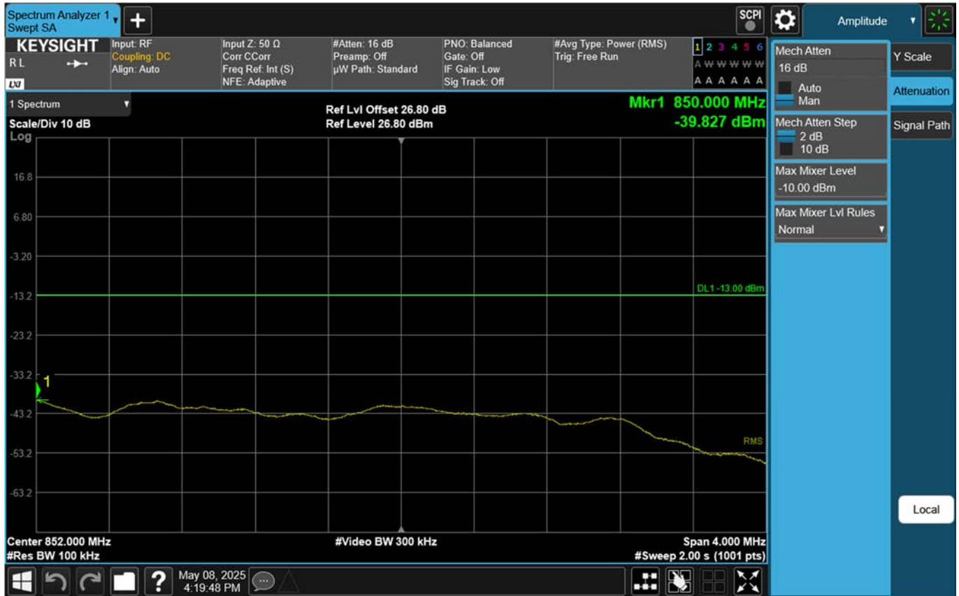
Upper Extended Band Edge Plot (10 M BW Ch.168800 BPSK_RB 50_0)
