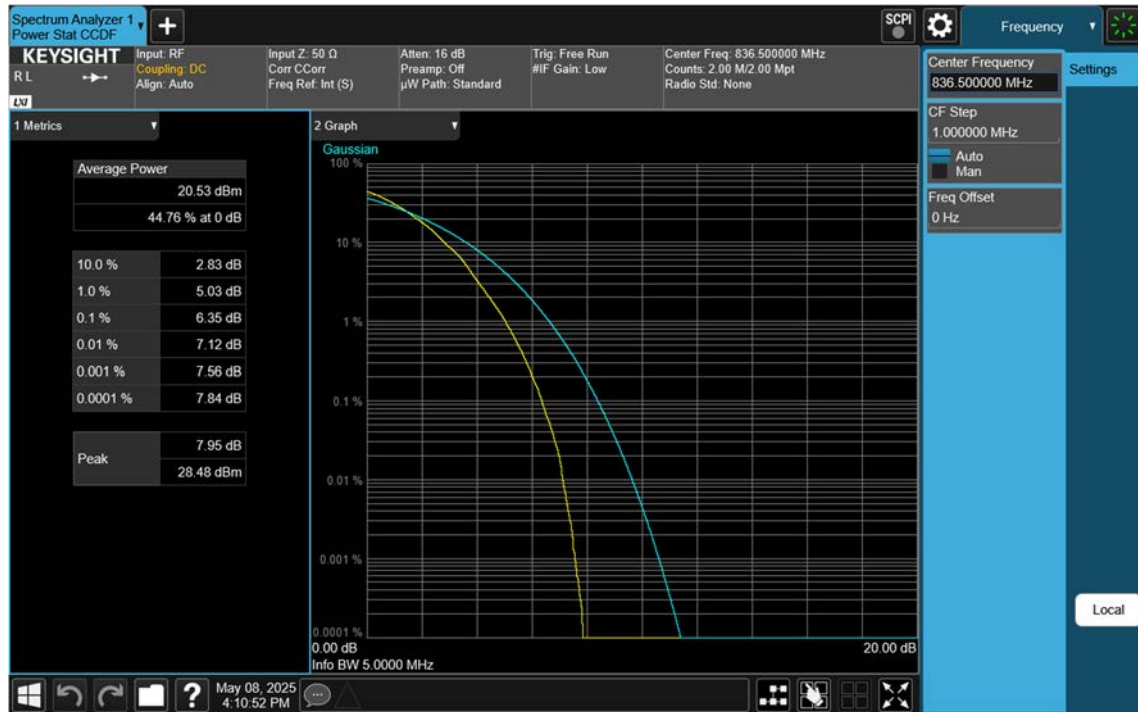
NR26(Part22)_5 M_PAR_Mid_64QAM_FullRB
