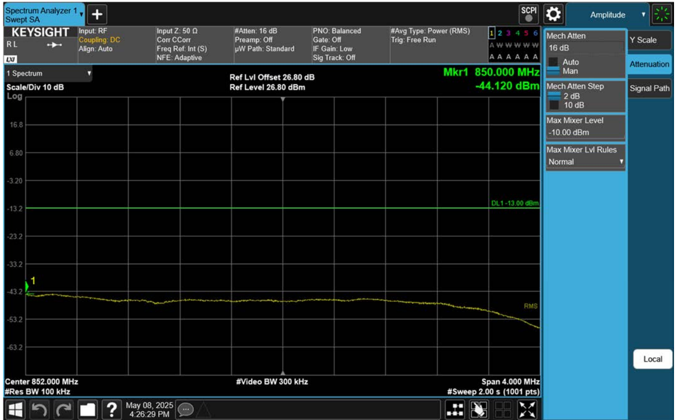
Upper Extended Band Edge Plot (15 M BW Ch.168300 BPSK_RB 75_0)
