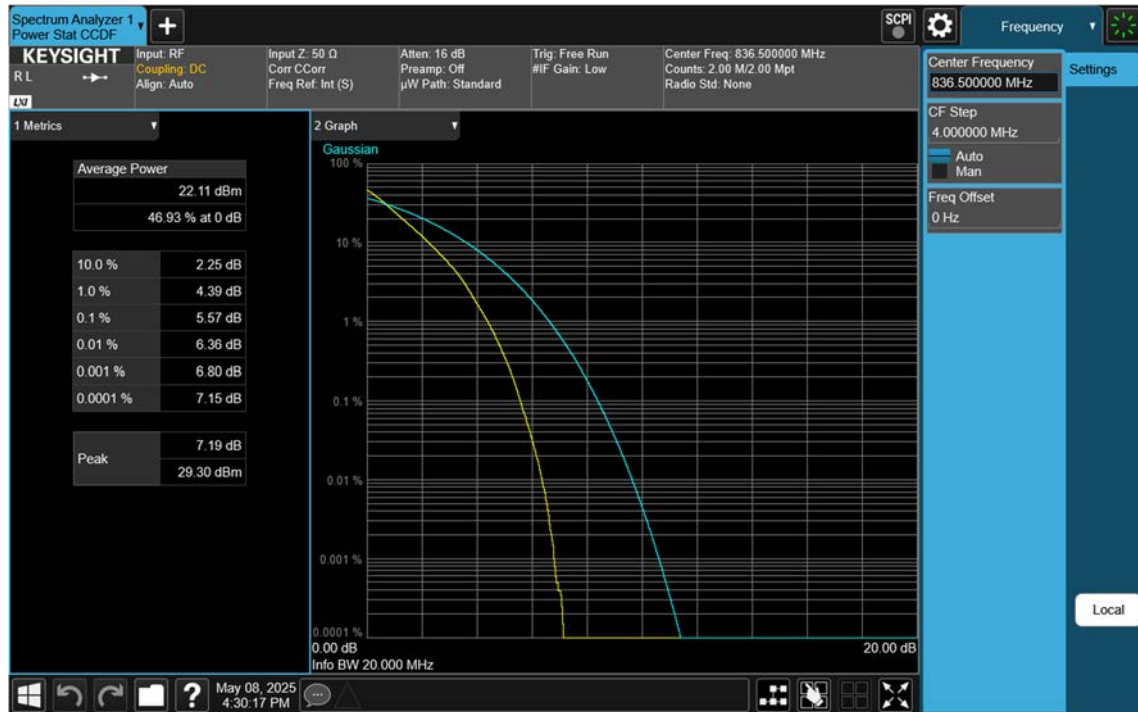
NR26(Part22)_20 M_PAR_Mid_QPSK_FullRB
