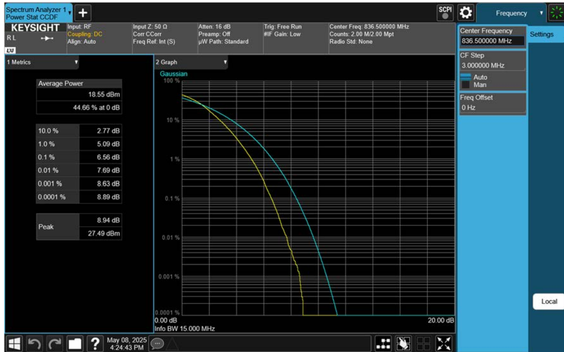
NR26(Part22)_15 M_PAR_Mid_256QAM_FullRB
