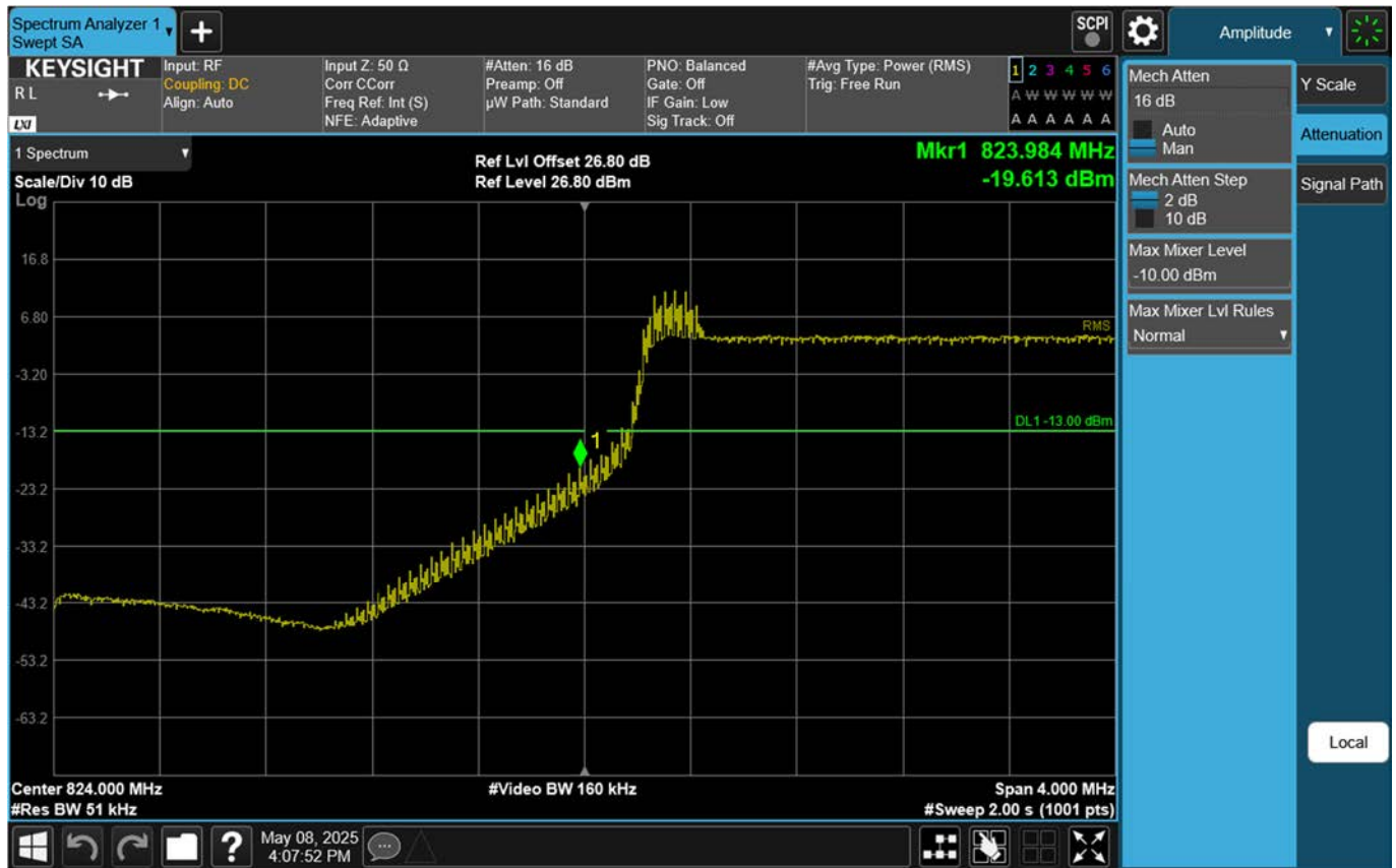
Lower Band Edge Plot (5 M BW Ch.165300 BPSK_RB 25_Offset 0)
