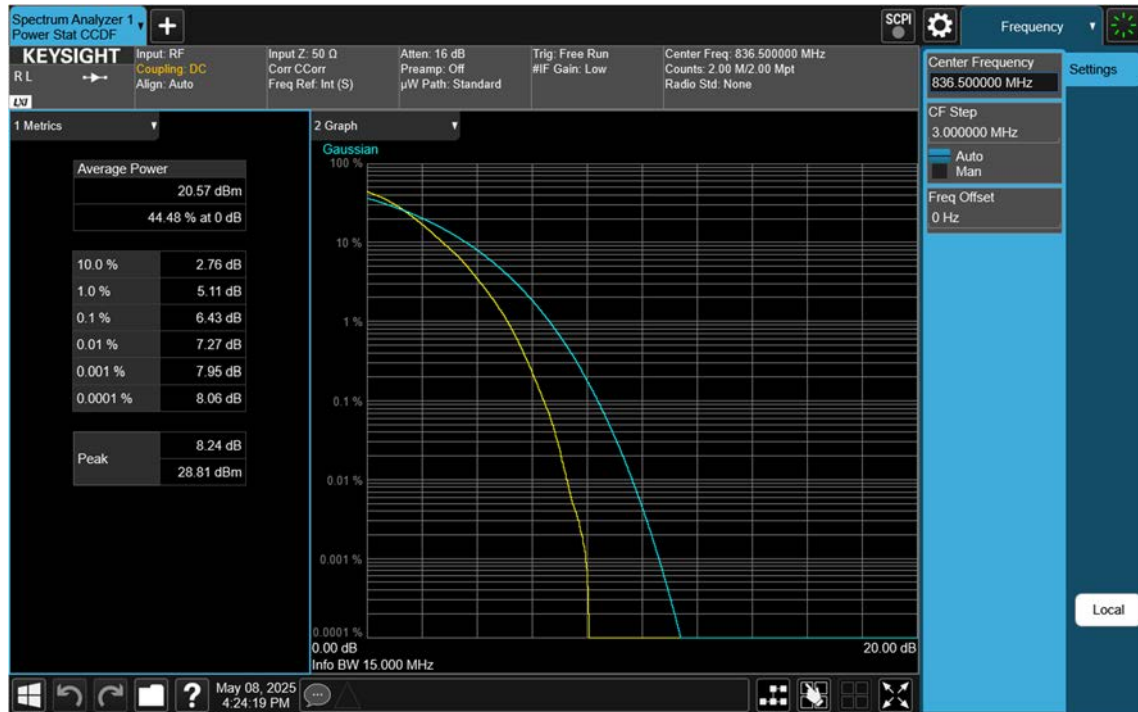
NR26(Part22)_15 M_PAR_Mid_64QAM_FullRB
