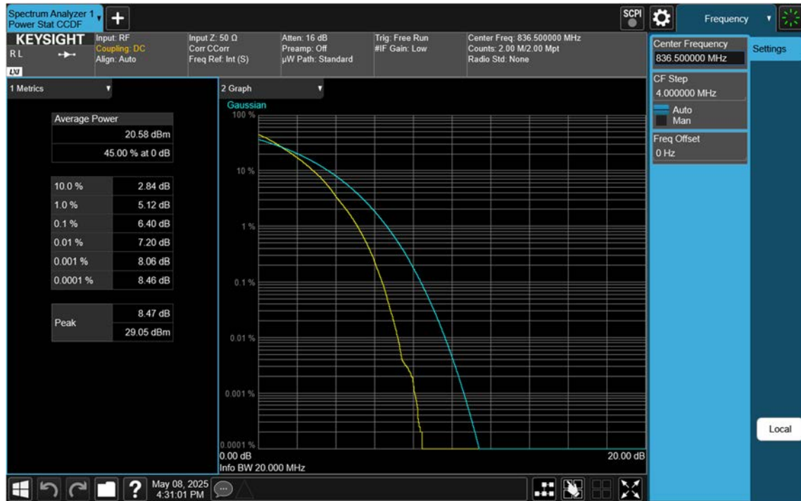
NR26(Part22)_20 M_PAR_Mid_64QAM_FullRB
