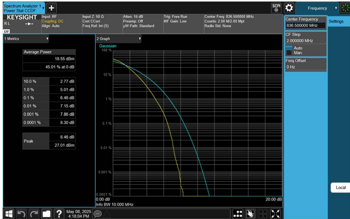
NR26(Part22)_10 M_PAR_Mid_256QAM_FullRB
