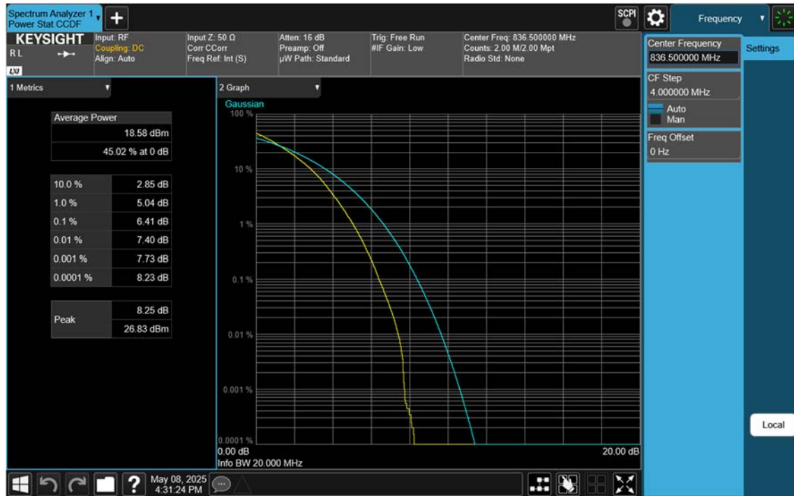
NR26(Part22)_20 M_PAR_Mid_256QAM_FullRB
