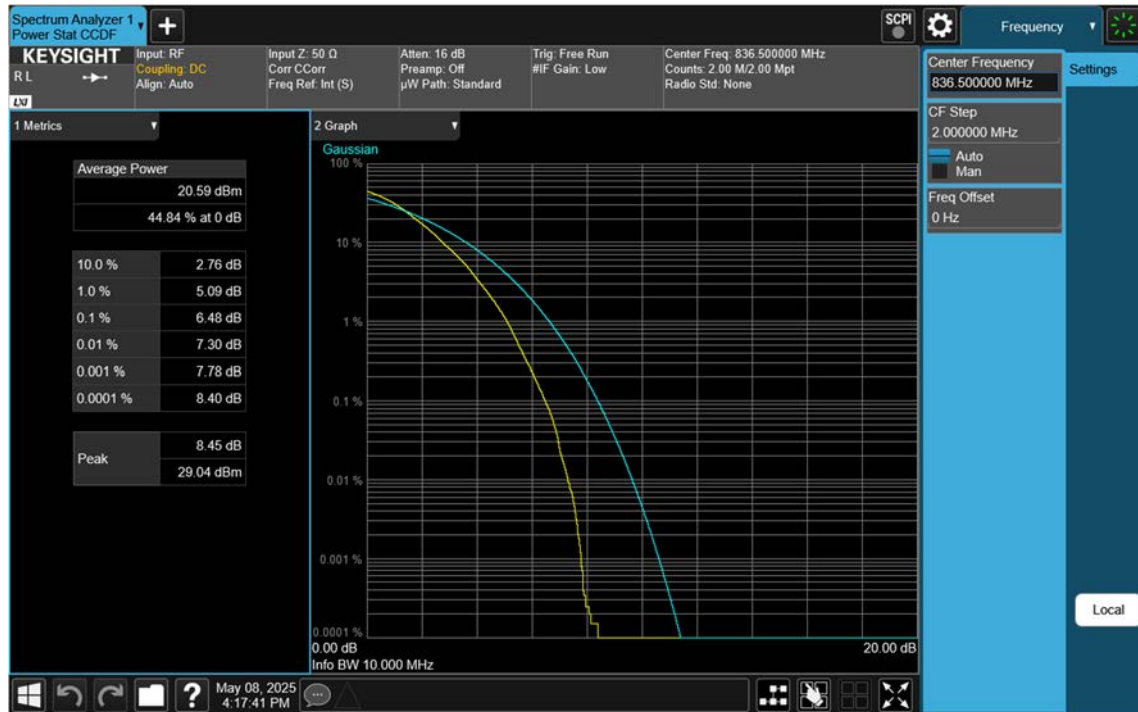
NR26(Part22)_10 M_PAR_Mid_64QAM_FullRB
