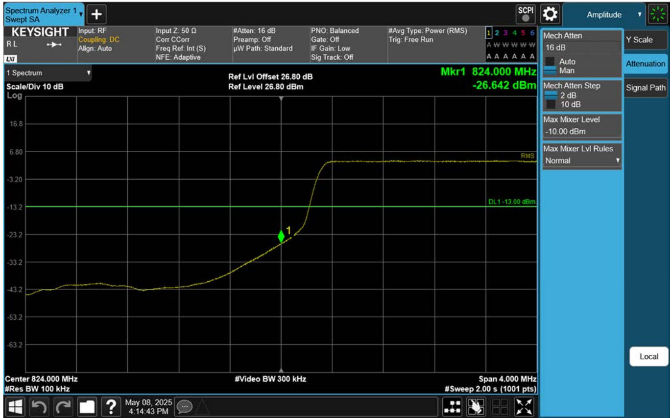
Lower Band Edge Plot (10 M BW Ch.165800 BPSK_RB 50_Offset 0)
