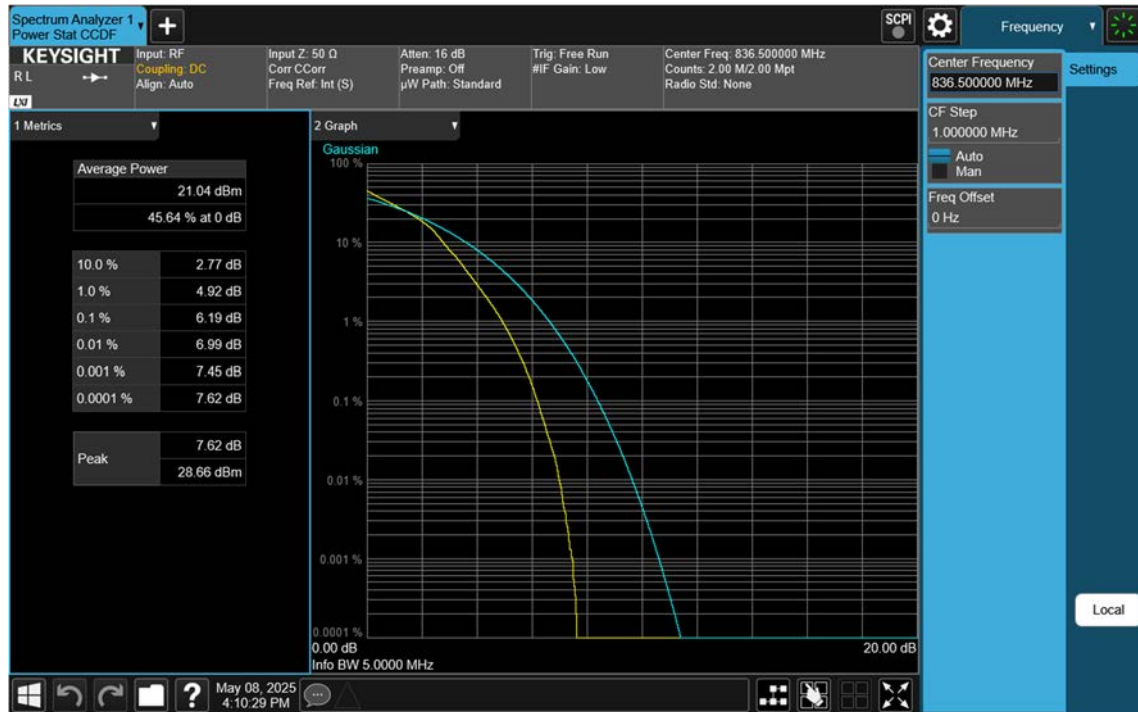
NR26(Part22)_5 M_PAR_Mid_16QAM_FullRB
