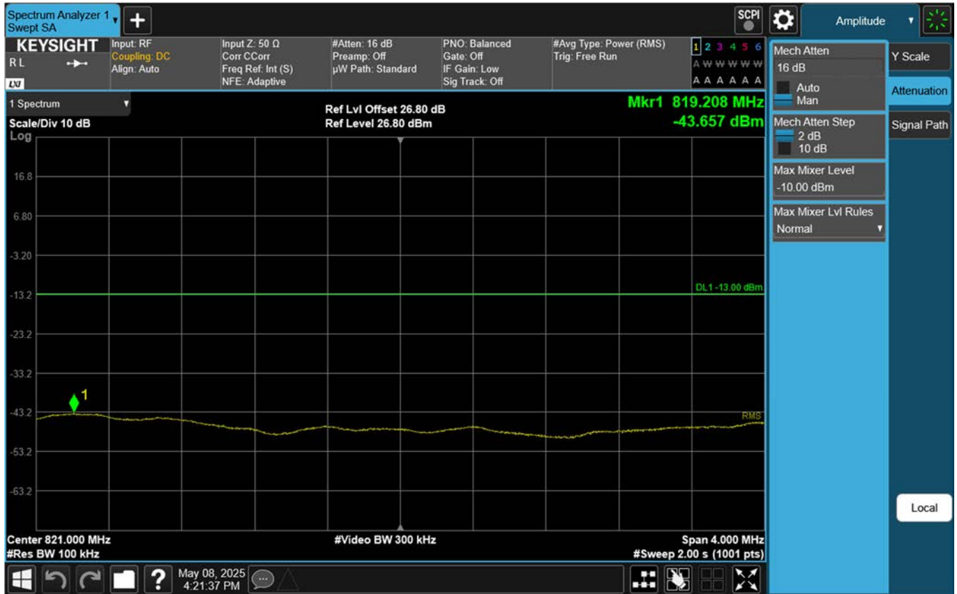
Lower Extended Band Edge Plot (15 M BW Ch.166300 BPSK_RB 75_0)
