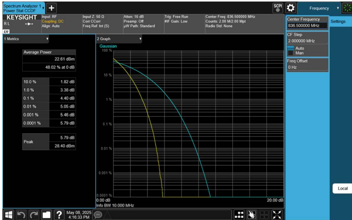
NR26(Part22)_10 M_PAR_Mid_BPSK_FullRB
