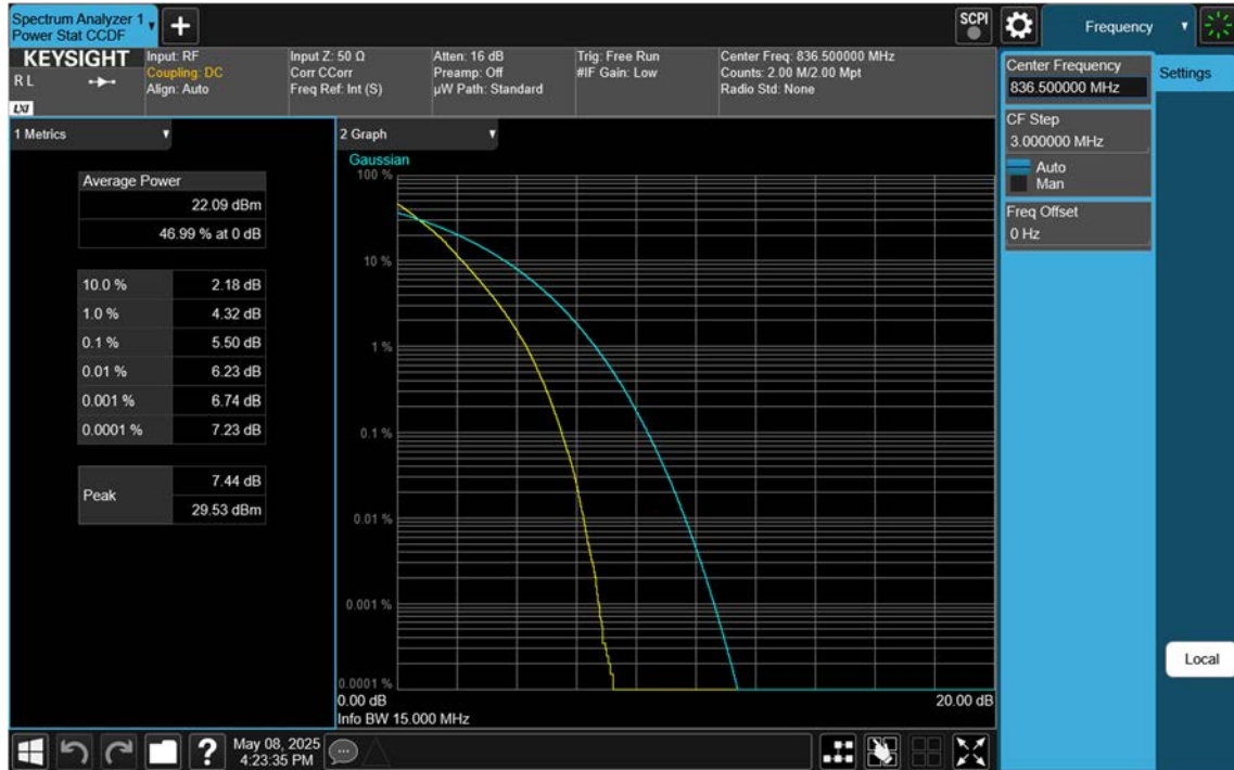
NR26(Part22)_15 M_PAR_Mid_QPSK_FullRB
