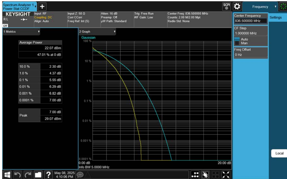
NR26(Part22)_5 M_PAR_Mid_QPSK_FullRB
