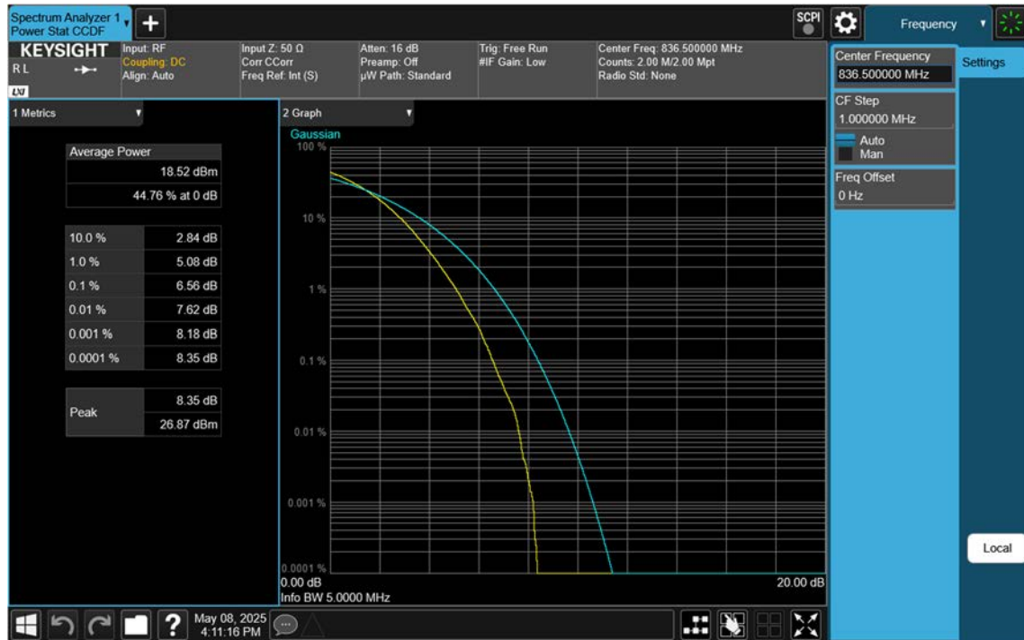
NR26(Part22)_5 M_PAR_Mid_256QAM_FullRB
