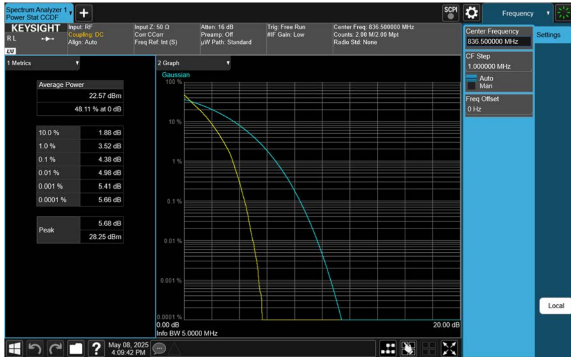
NR26(Part22)_5 M_PAR_Mid_BPSK_FullRB
