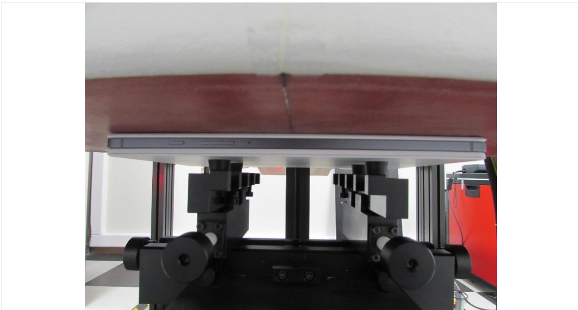
Distance of 0 mm from the EUT with Cover Variant 2
