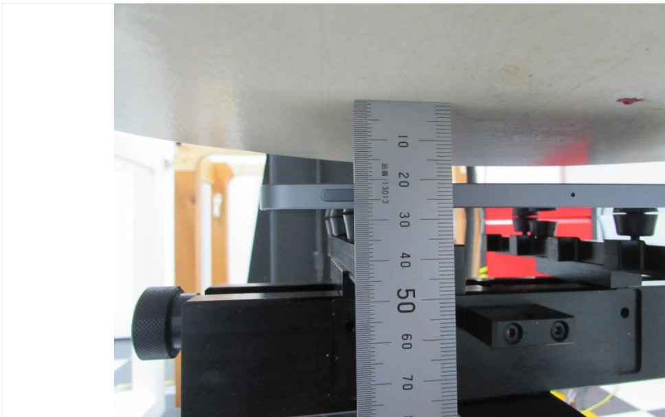
Distance of 21 mm from the EUT
