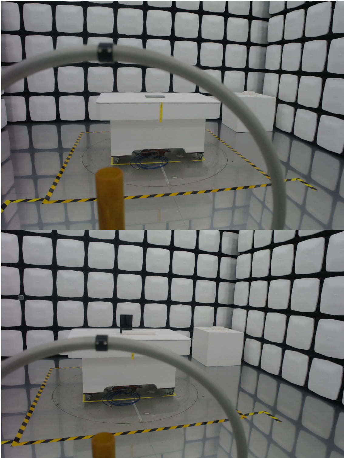
Digitizer Radiated Test Setup Photo for below 30 MHz:
