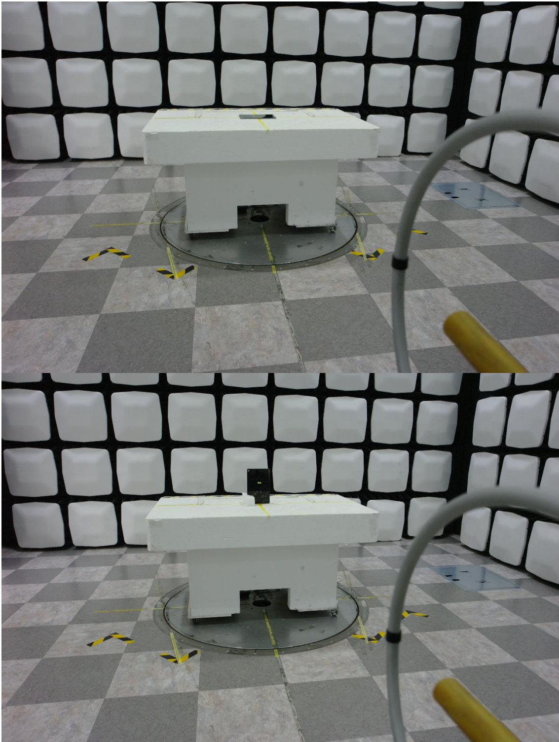
Digitizer(S-pen) Radiated Test Setup Photo for below 30 MHz:
