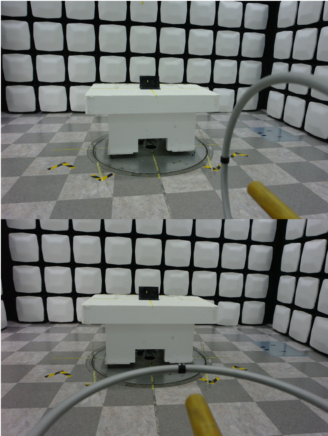
Digitizer(Keyboard cover detection) Radiated Test Setup Photo for below 30 MHz:
