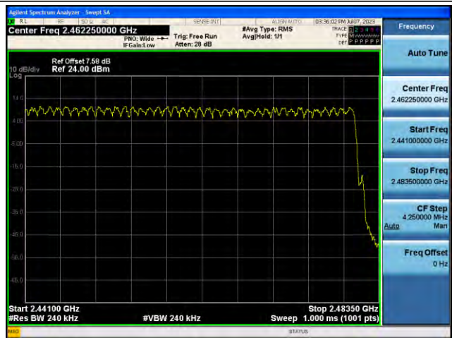
\pi/4 DQPSK Number of Channels (2.441 GHz - 2.483.5 GHz)
