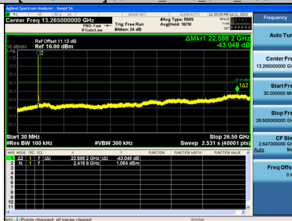
[MIMO ANT. 2] 802.11n HT20 Ch.1 MCS12
