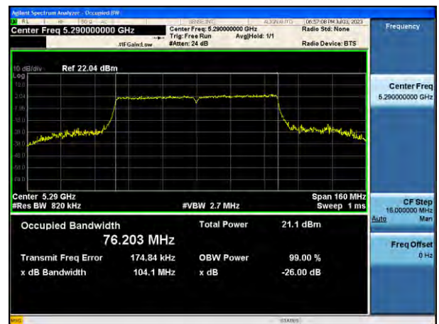
802.11ac(VHT80) 26 dB Bandwidth (CH 58)
