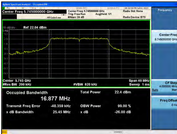
802.11ac(VHT20) 26 dB Bandwidth (CH 149)
