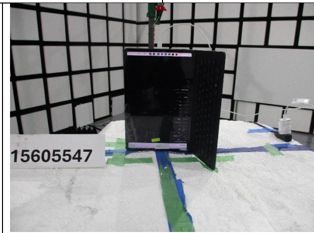
Z-ORIENTATION
