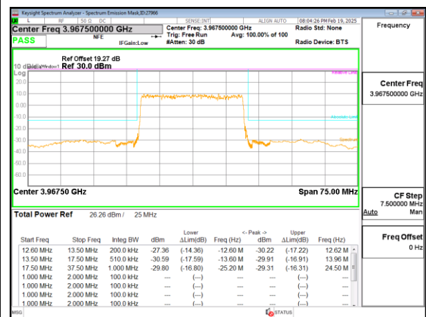
5G NR n77 25MHz BPSK High Channel RB64-0
