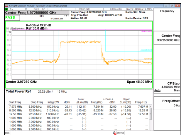
5G NR n77 15MHz BPSK High Channel RB36-0
