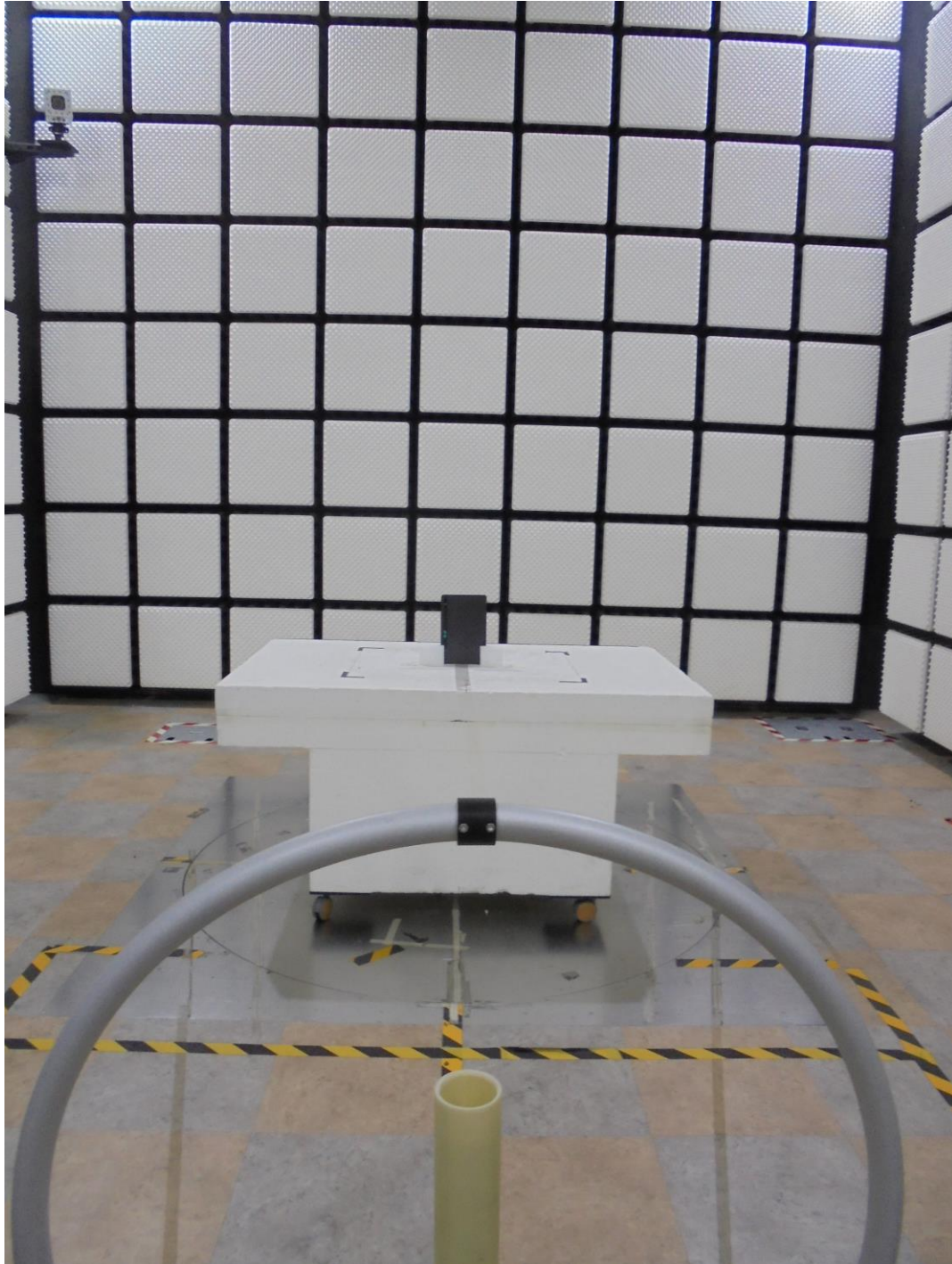
WPS Radiated Test Setup Photo for below 30 MHz:
