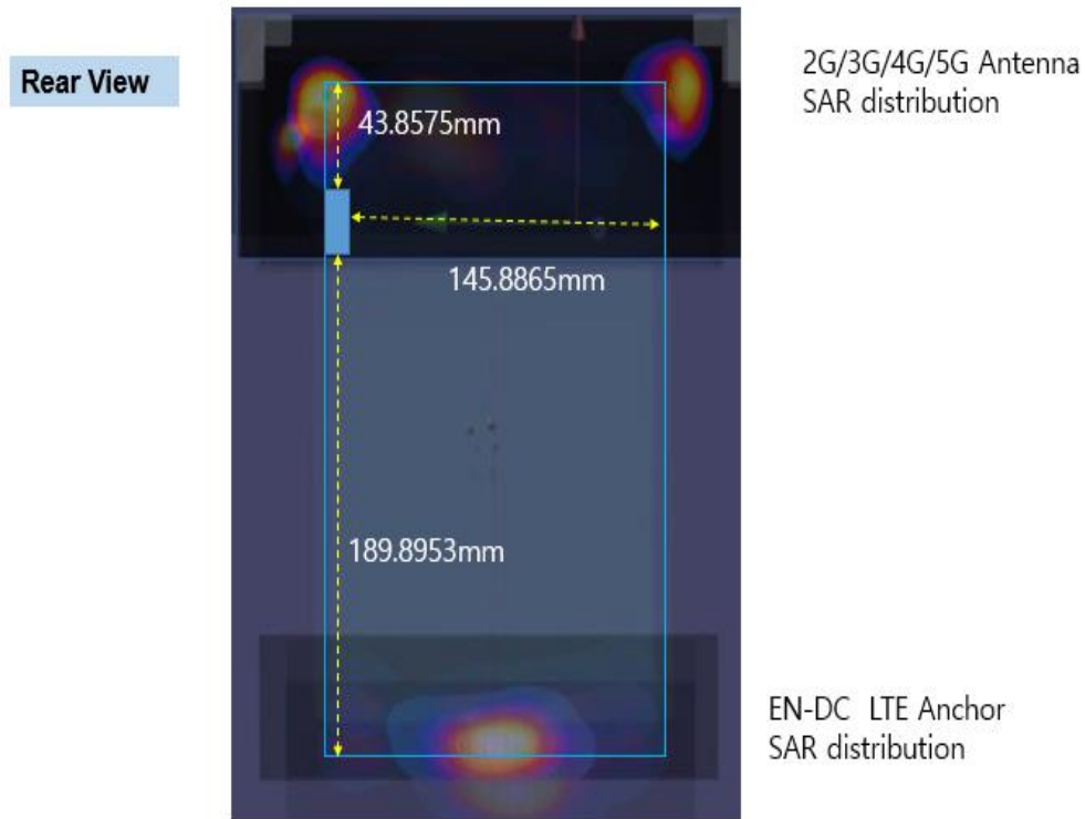
Rear side overlay showing SAR and PD peak distribution
