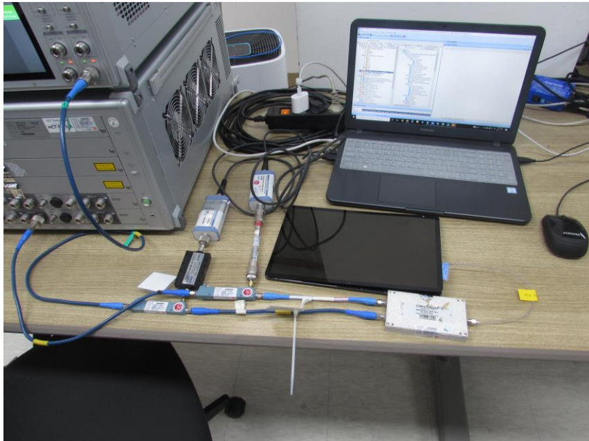
Test setup photo- 4 (8-1 SAR Setup)
