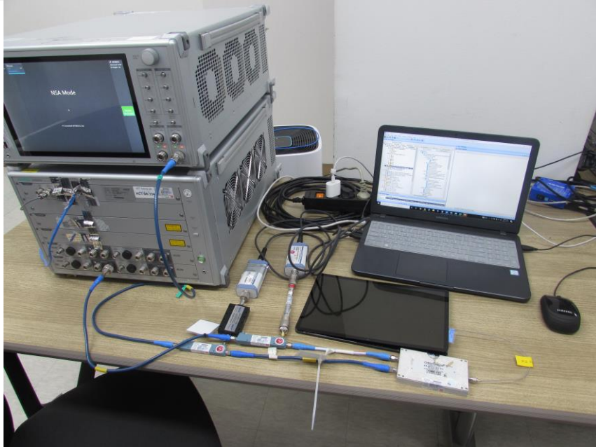
Test setup photo- 3 (7-1(c)NR FR1power measurement)
