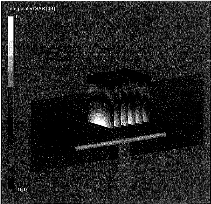
0 dB = 16.1 W/Kg
