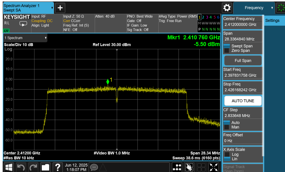
Plot 7-46. Power Spectral Density Plot MIMO ANT2 (802.11ax) (2.4GHz) – Ch. 1)
