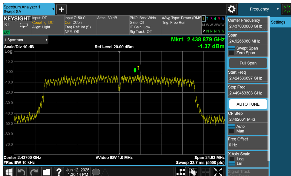
Plot 7-44. Power Spectral Density Plot MIMO ANT1 (802.11n (2.4GHz) – Ch. 6)
