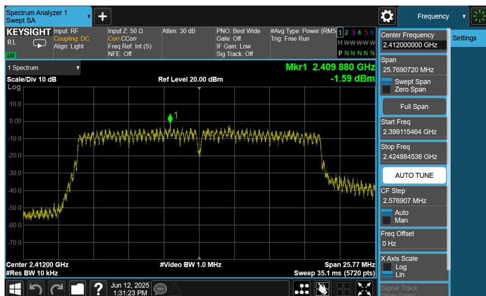
Plot 7-43. Power Spectral Density Plot MIMO ANT2 (802.11n (2.4GHz) – Ch. 1)
