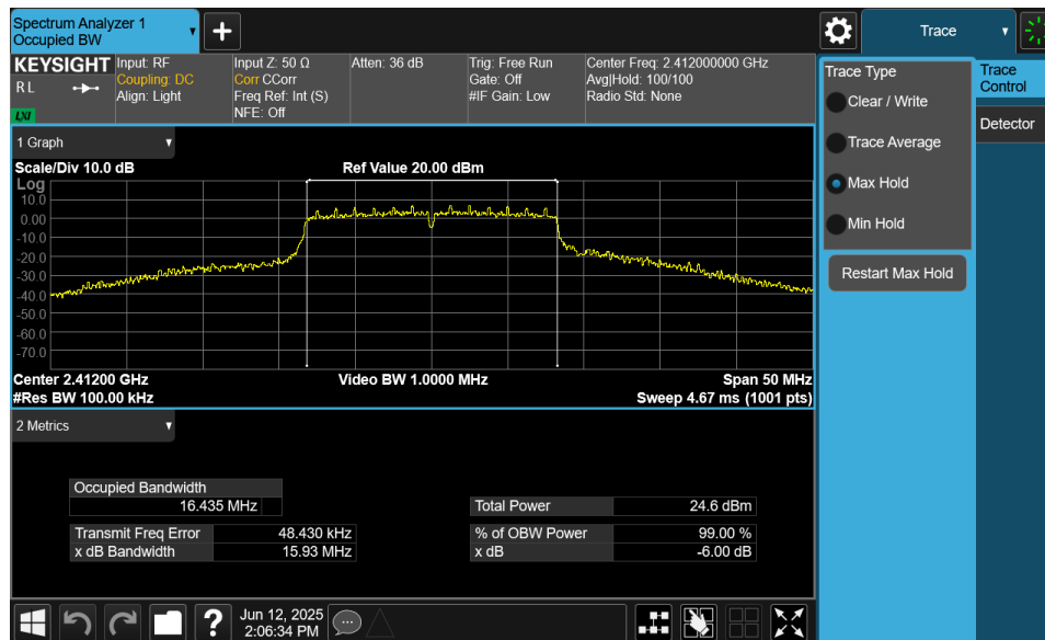
Plot 7-4. 6dB Bandwidth Plot MIMO ANT1 (802.11g – Ch. 1)
