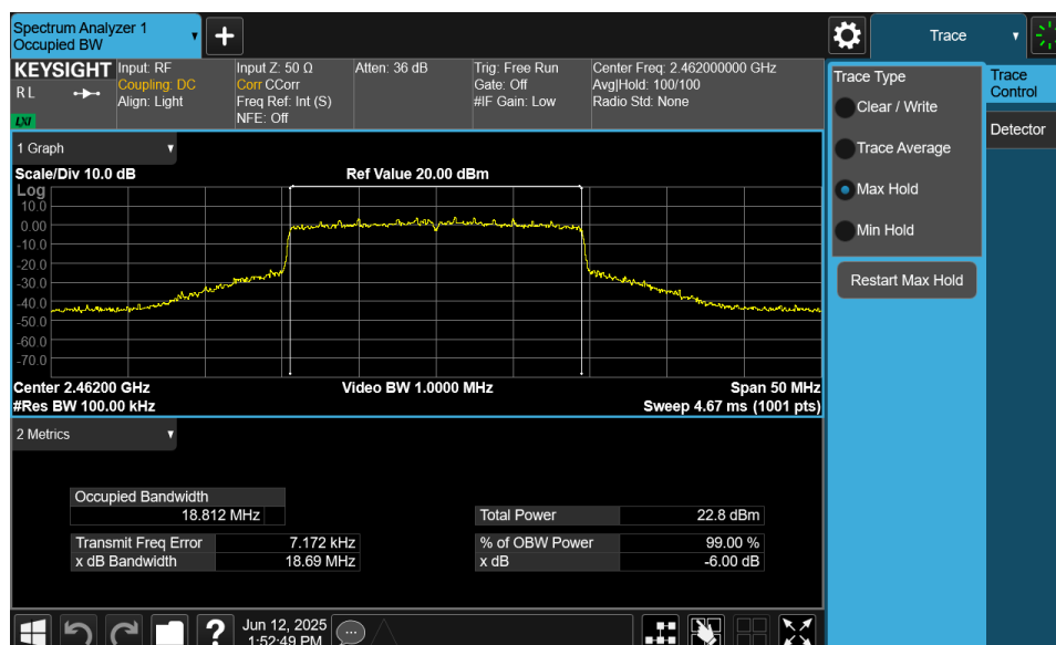
Plot 7-12. 6dB Bandwidth Plot MIMO ANT1 (802.11ax (2.4GHz) – Ch. 11)
