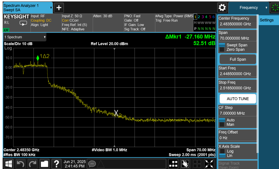
Plot 7-55. Band Edge Plot MIMO ANT1 (802.11g – Ch. 9)
