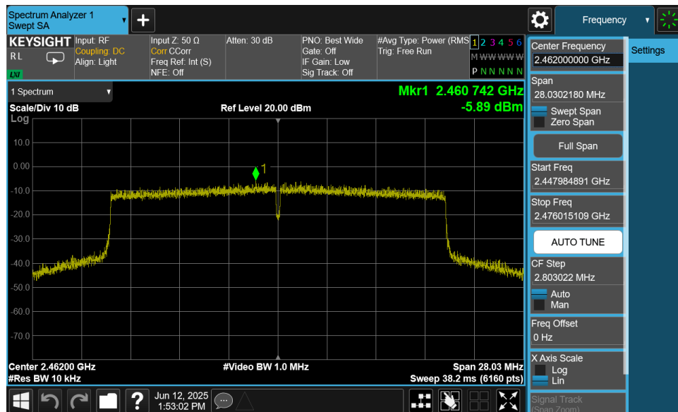
Plot 7-36. Power Spectral Density Plot MIMO ANT1 (802.11ax (2.4GHz) – Ch. 11)
