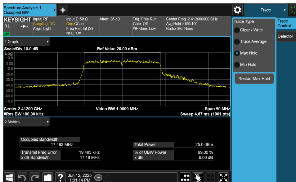
Plot 7-19. 6dB Bandwidth Plot MIMO ANT2 (802.11n (2.4GHz) – Ch. 1)
