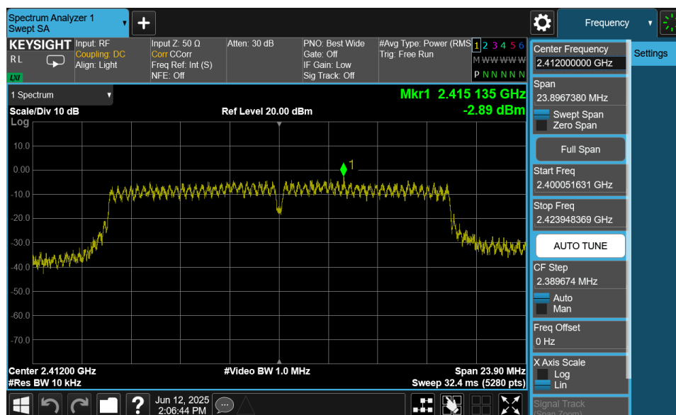
Plot 7-28. Power Spectral Density Plot MIMO ANT1 (802.11g – Ch. 1)
