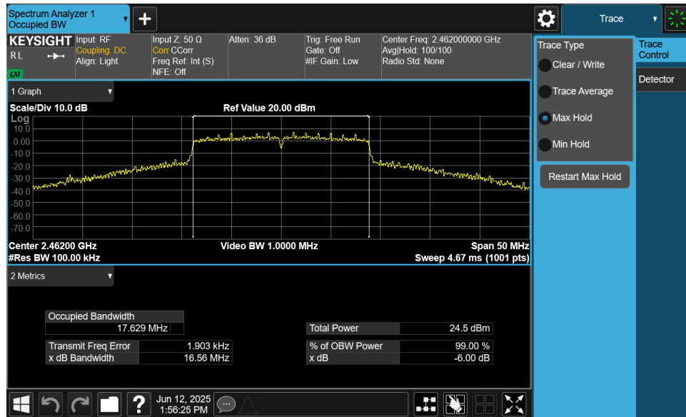
Plot 7-9. 6dB Bandwidth Plot MIMO ANT1 (802.11n (2.4GHz) – Ch. 11)
