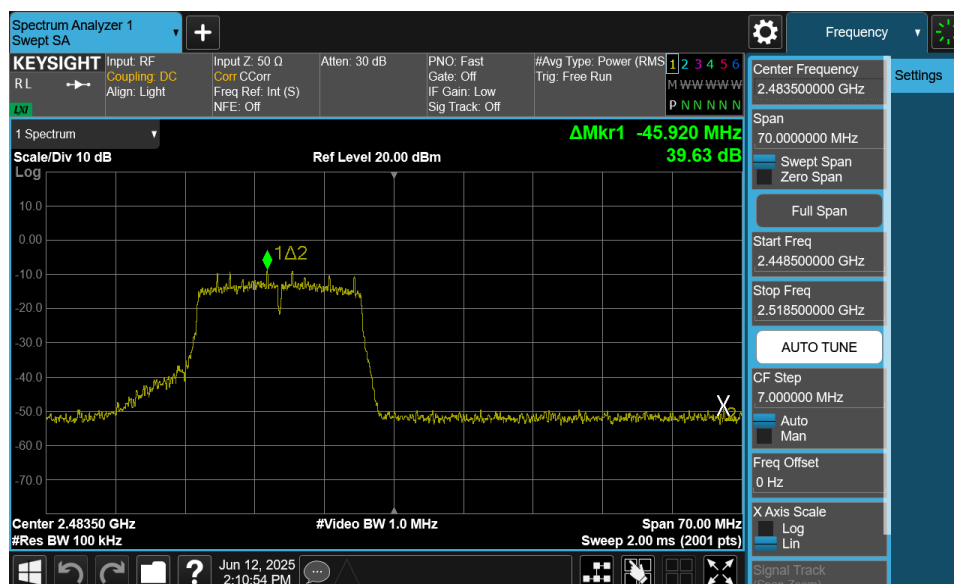
Plot 7-59. Band Edge Plot MIMO ANT1 (802.11g – Ch. 13)
