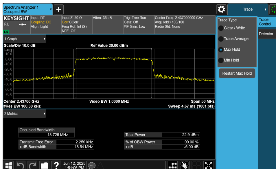
Plot 7-11. 6dB Bandwidth Plot MIMO ANT1 (802.11ax (2.4GHz) – Ch. 6)
