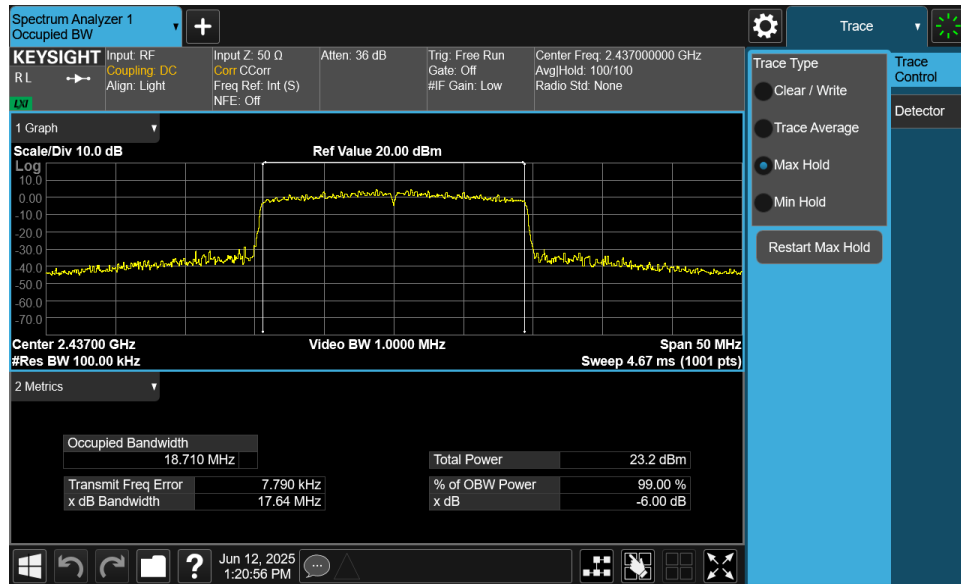
Plot 7-23. 6dB Bandwidth Plot MIMO ANT2 (802.11ax (2.4GHz) – Ch. 6)
