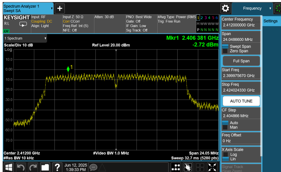
Plot 7-40. Power Spectral Density Plot MIMO ANT2 (802.11g – Ch. 1)
