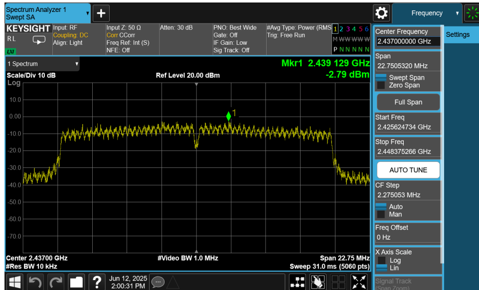
Plot 7-32. Power Spectral Density Plot MIMO ANT1 (802.11n (2.4GHz) – Ch. 6)
