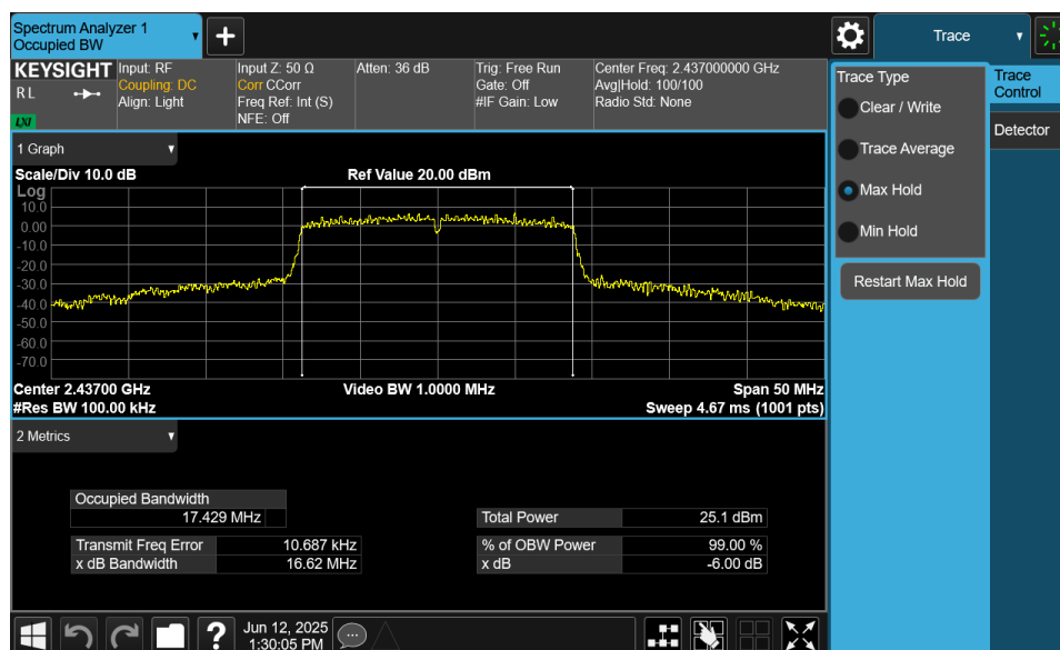
Plot 7-20. 6dB Bandwidth Plot MIMO ANT2 (802.11n (2.4GHz) – Ch. 6)
