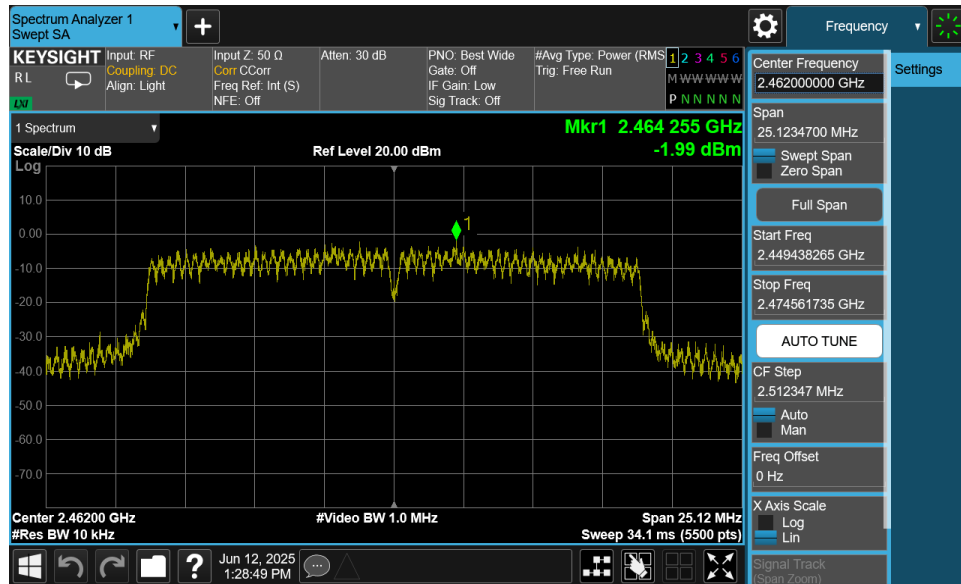
Plot 7-45. Power Spectral Density Plot MIMO ANT2 (802.11n) (2.4GHz) – Ch. 11)
