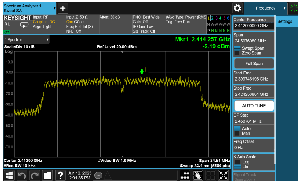
Plot 7-31. Power Spectral Density Plot MIMO ANT1 (802.11n (2.4GHz) – Ch. 1)
