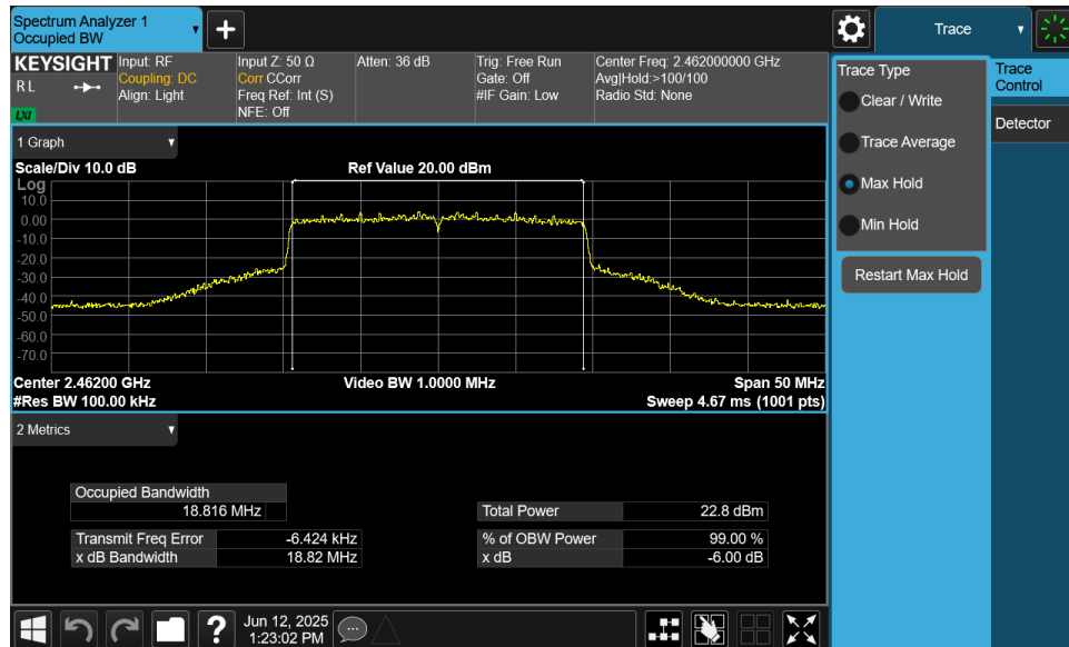
Plot 7-24. 6dB Bandwidth Plot MIMO ANT2 (802.11ax (2.4GHz) – Ch. 11)
