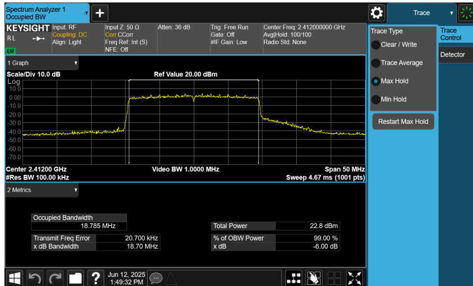
Plot 7-10. 6dB Bandwidth Plot MIMO ANT1 (802.11ax (2.4GHz) – Ch. 1)
