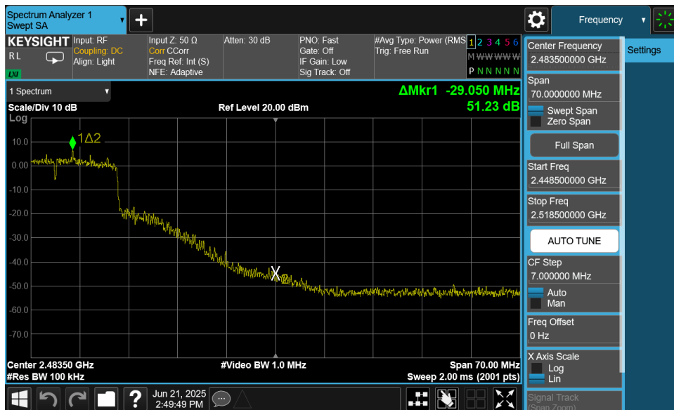
Plot 7-62. Band Edge Plot MIMO ANT1 (802.11n (2.4GHz) – Ch. 9)
