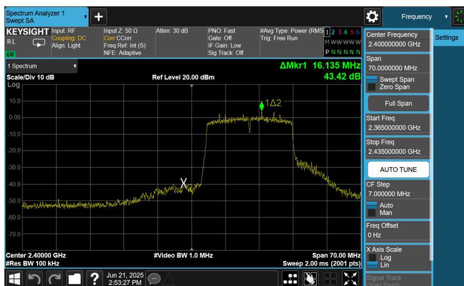
Plot 7-60. Band Edge Plot MIMO ANT1 (802.11n (2.4GHz) – Ch. 1)
