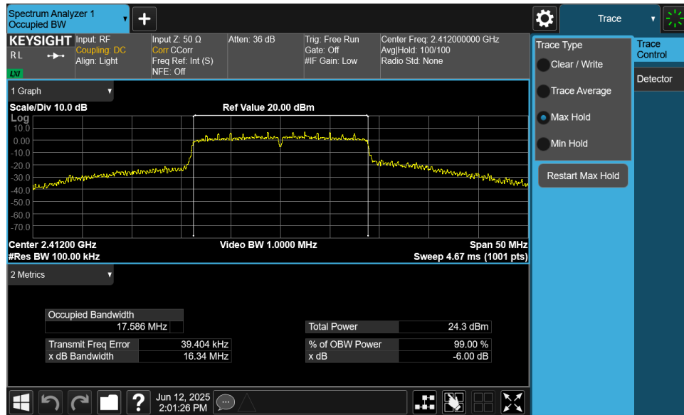
Plot 7-7. 6dB Bandwidth Plot MIMO ANT1 (802.11n (2.4GHz) – Ch. 1)
