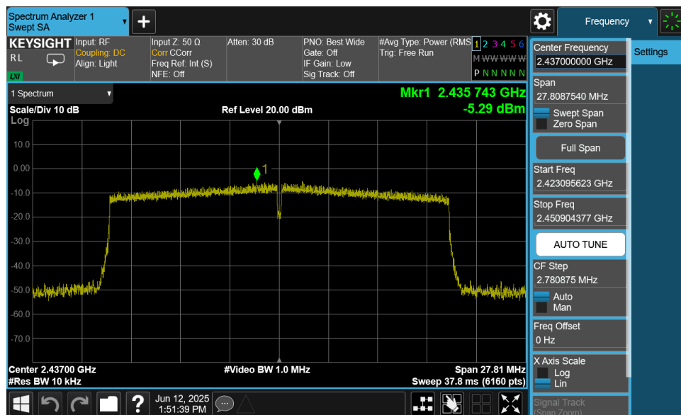
Plot 7-35. Power Spectral Density Plot MIMO ANT1 (802.11ax (2.4GHz) – Ch. 6)
