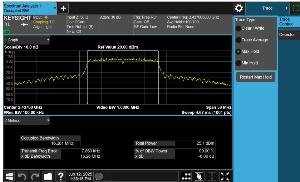
Plot 7-17. 6dB Bandwidth Plot MIMO ANT2 (802.11g – Ch. 6)
