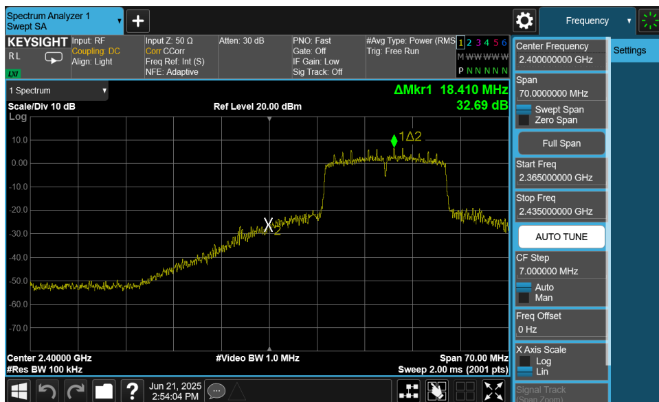
Plot 7-61. Band Edge Plot MIMO ANT1 (802.11n (2.4GHz) – Ch. 2)
