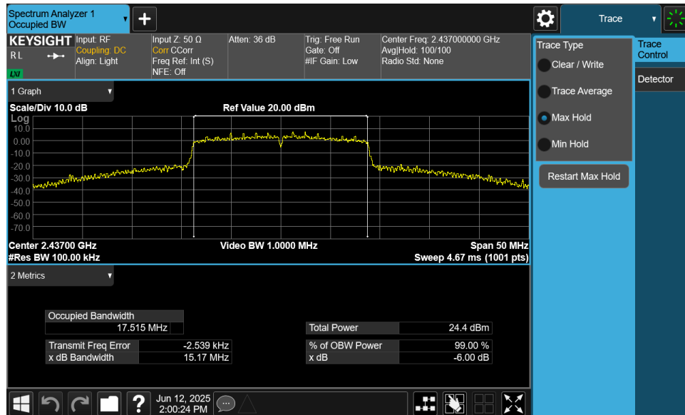
Plot 7-8. 6dB Bandwidth Plot MIMO ANT1 (802.11n (2.4GHz) – Ch. 6)
