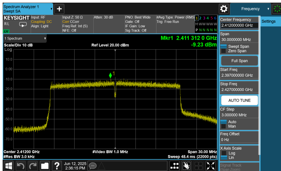
Plot 7-16. Power Spectral Density Plot MIMO ANT1 (802.11ax OFDMA – 242 Tones – Ch. 1)
