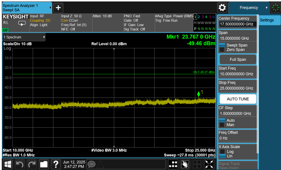
Plot 7-60. Conducted Spurious Plot MIMO ANT2 (802.11ax OFDMA – 242 Tones – Ch. 1)
