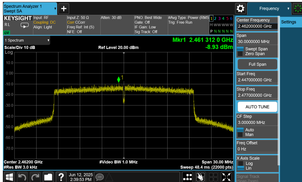
Plot 7-18. Power Spectral Density Plot MIMO ANT1 (802.11ax OFDMA – 242 Tones – Ch. 11)
