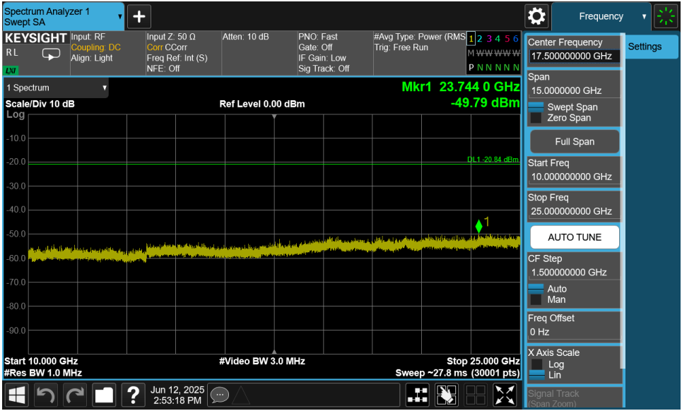
Plot 7-56. Conducted Spurious Plot MIMO ANT2 (802.11ax OFDMA – 26 Tones – Ch. 6)
