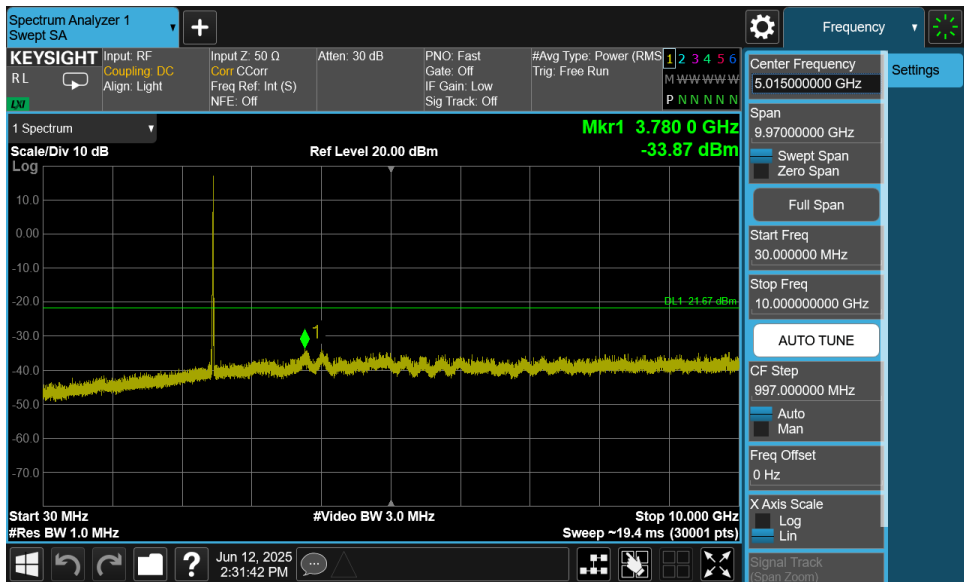
Plot 7-45. Conducted Spurious Plot MIMO ANT1 (802.11ax OFDMA – 26 Tones – Ch. 11)
