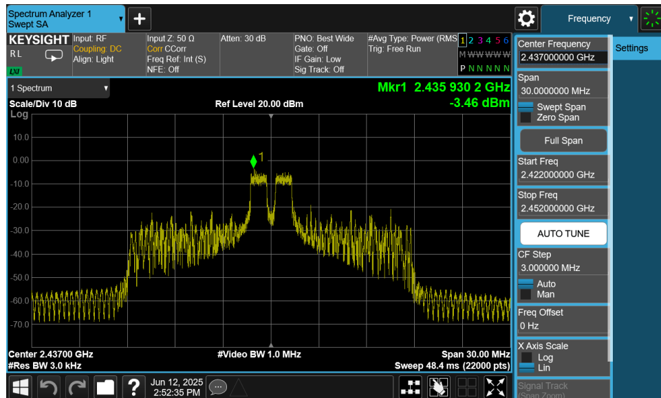
Plot 7-20. Power Spectral Density Plot MIMO ANT2 (802.11ax OFDMA – 26 Tones – Ch. 6)
