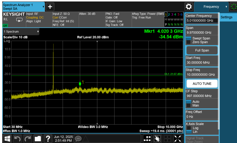
Plot 7-57. Conducted Spurious Plot MIMO ANT2 (802.11ax OFDMA – 26 Tones – Ch. 11)
