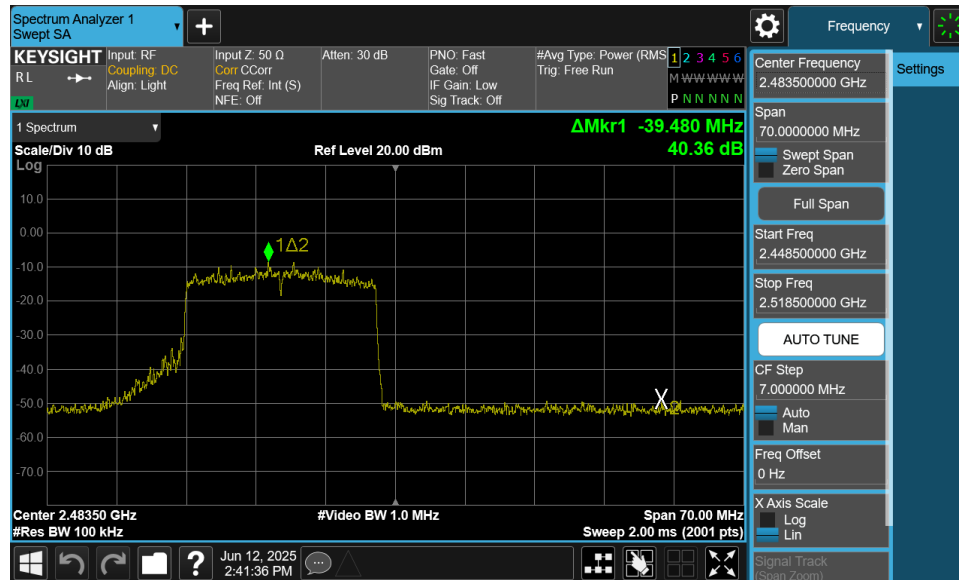
Plot 7-32. Band Edge Plot MIMO ANT1 (802.11ax OFDMA – 242 Tones – Ch. 13)
