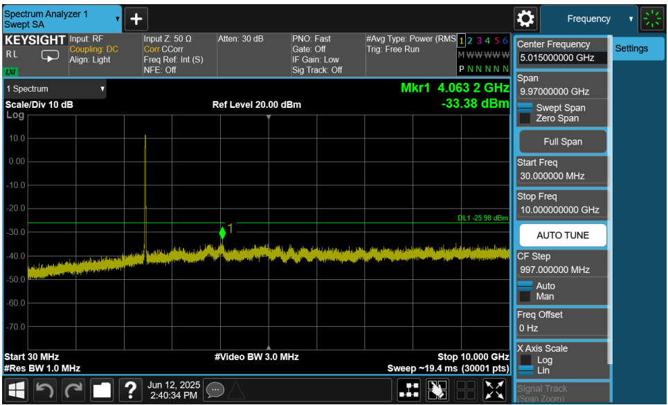
Plot 7-51. Conducted Spurious Plot MIMO ANT1 (802.11ax OFDMA – 242 Tones – Ch. 11)
