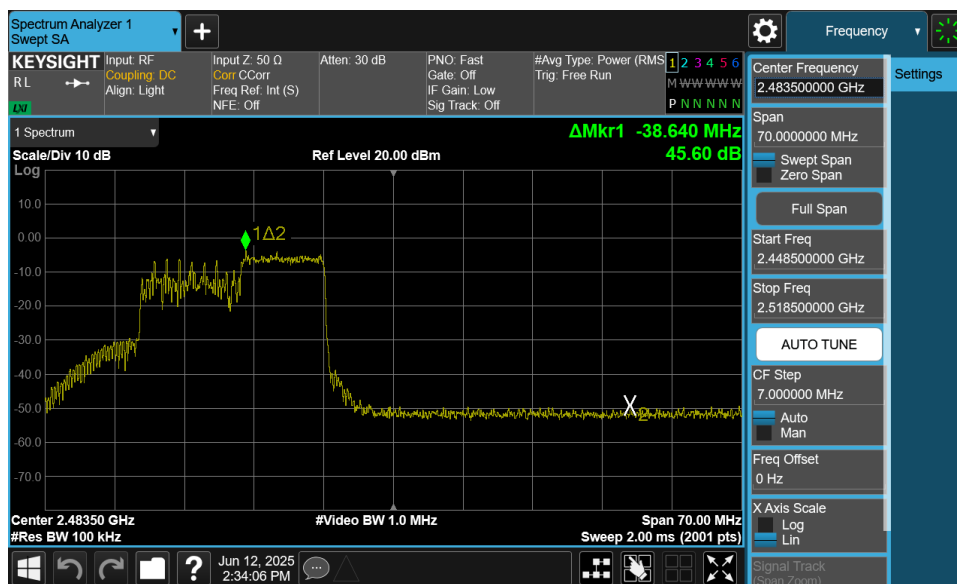
Plot 7-27. Band Edge Plot MIMO ANT1 (802.11ax OFDMA – 106 Tones – Ch. 12)
