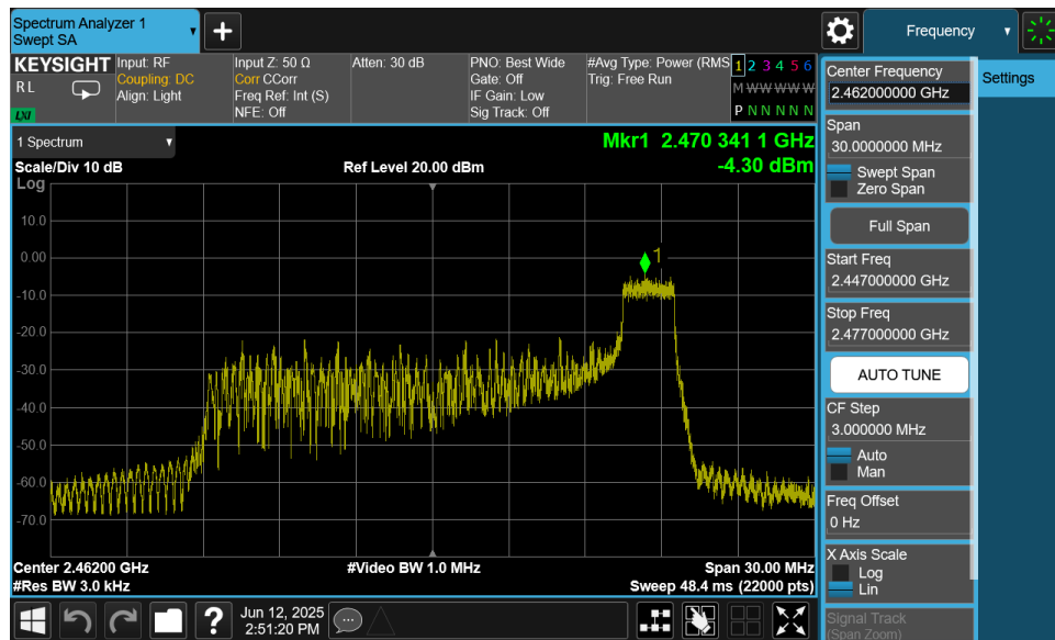
Plot 7-21. Power Spectral Density Plot MIMO ANT2 (802.11ax OFDMA – 26 Tones – Ch. 11)
