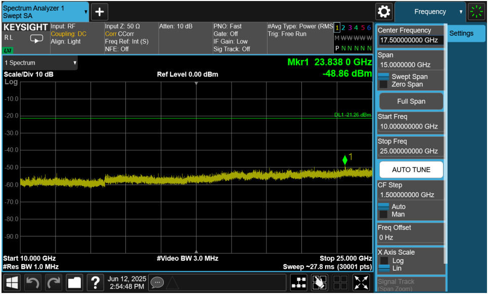
Plot 7-54. Conducted Spurious Plot MIMO ANT2 (802.11ax OFDMA – 26 Tones – Ch. 1)
