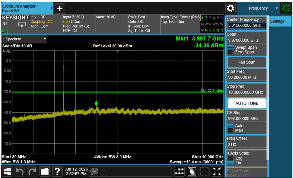
Plot 7-55. Conducted Spurious Plot MIMO ANT2 (802.11ax OFDMA – 26 Tones – Ch. 6)
