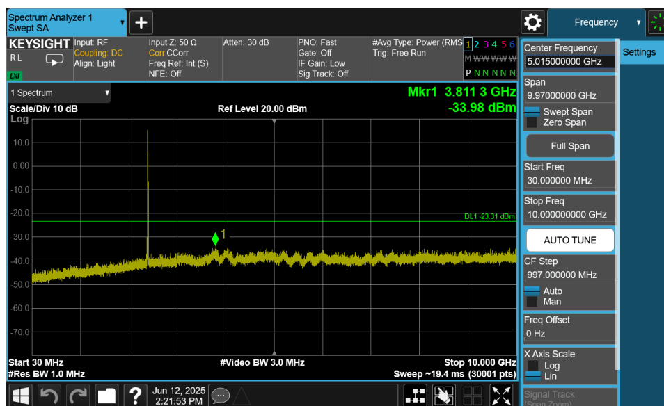
Plot 7-41. Conducted Spurious Plot MIMO ANT1 (802.11ax OFDMA – 26 Tones – Ch. 1)
