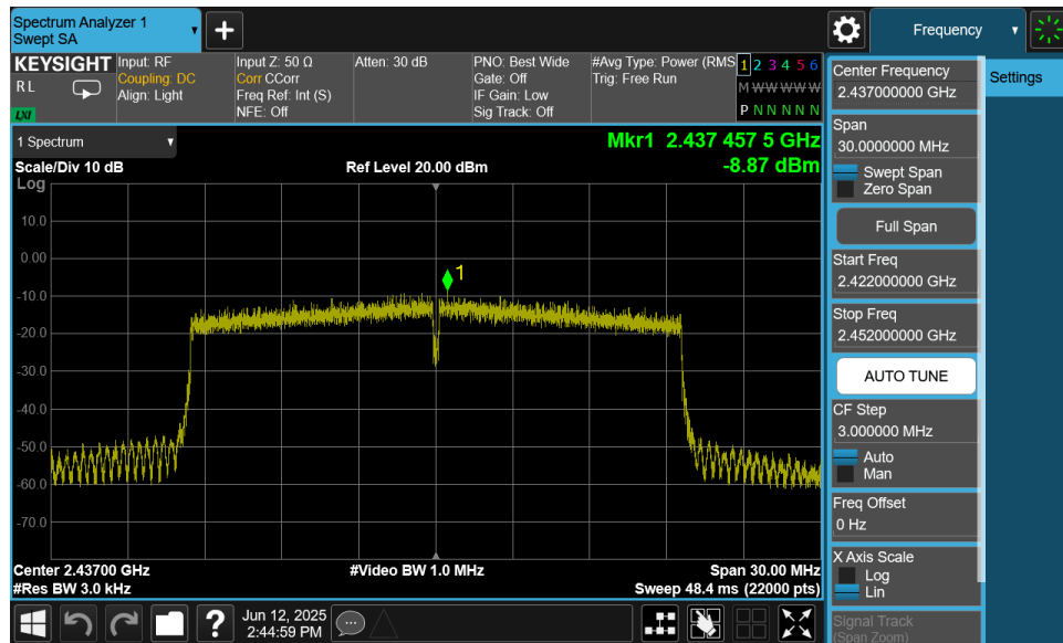
Plot 7-23. Power Spectral Density Plot MIMO ANT2 (802.11ax OFDMA – 242 Tones – Ch. 6)
