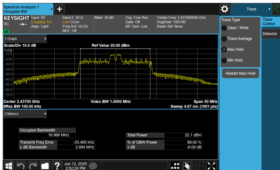
Plot 7-8. 6dB Bandwidth Plot MIMO ANT2 (802.11ax OFDMA – 26 Tones – Ch. 6)
