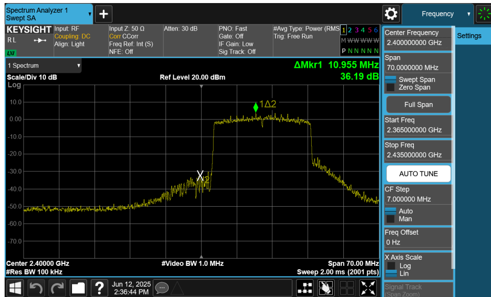
Plot 7-29. Band Edge Plot MIMO ANT1 (802.11ax OFDMA – 242 Tones – Ch. 1)
