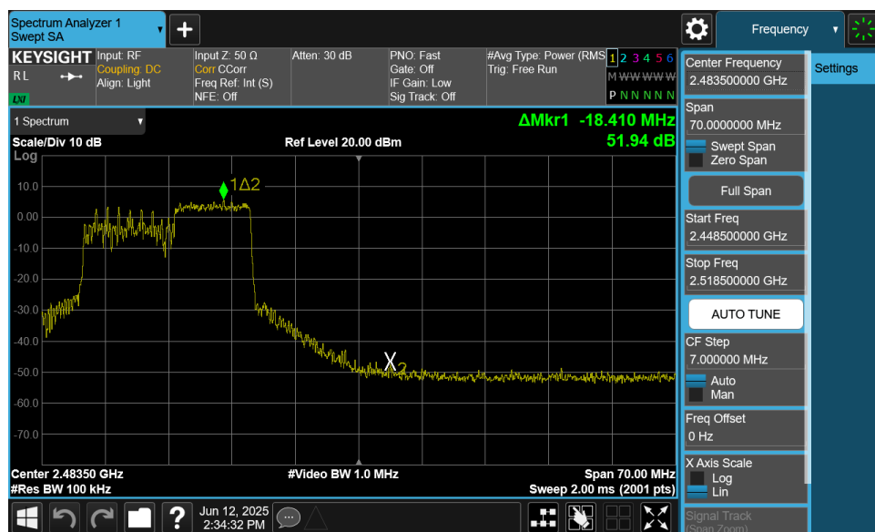
Plot 7-26. Band Edge Plot MIMO ANT1 (802.11ax OFDMA – 106 Tones – Ch. 11)
