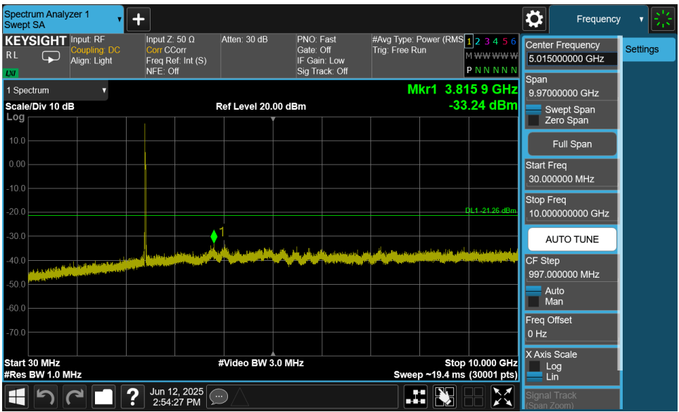
Plot 7-53. Conducted Spurious Plot MIMO ANT2 (802.11ax OFDMA – 26 Tones – Ch. 1)
