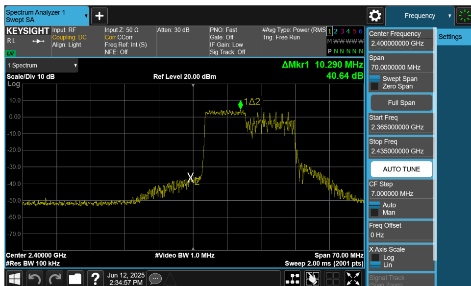
Plot 7-25. Band Edge Plot MIMO ANT1 (802.11ax OFDMA – 106 Tones – Ch. 1)
