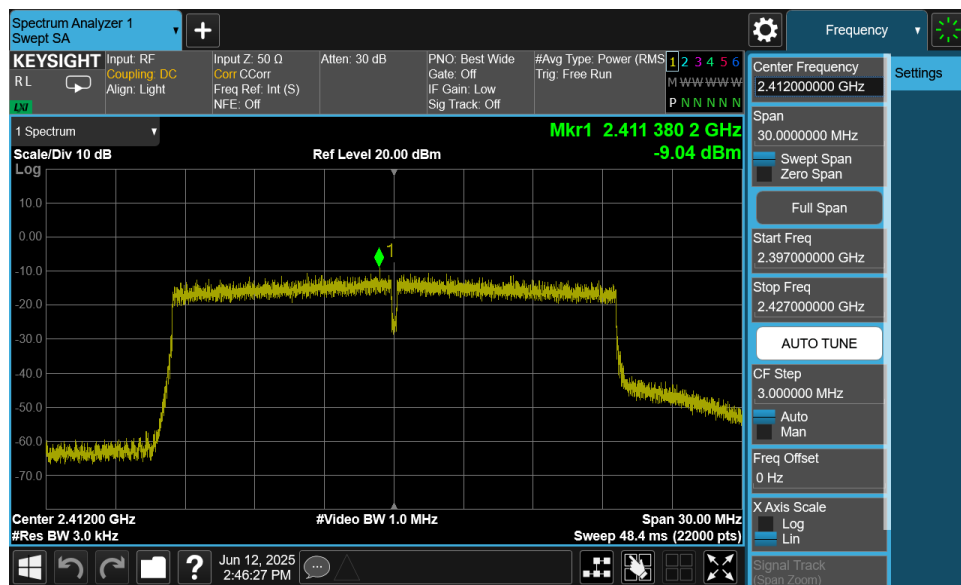
Plot 7-22. Power Spectral Density Plot MIMO ANT2 (802.11ax OFDMA – 242 Tones – Ch. 1)
