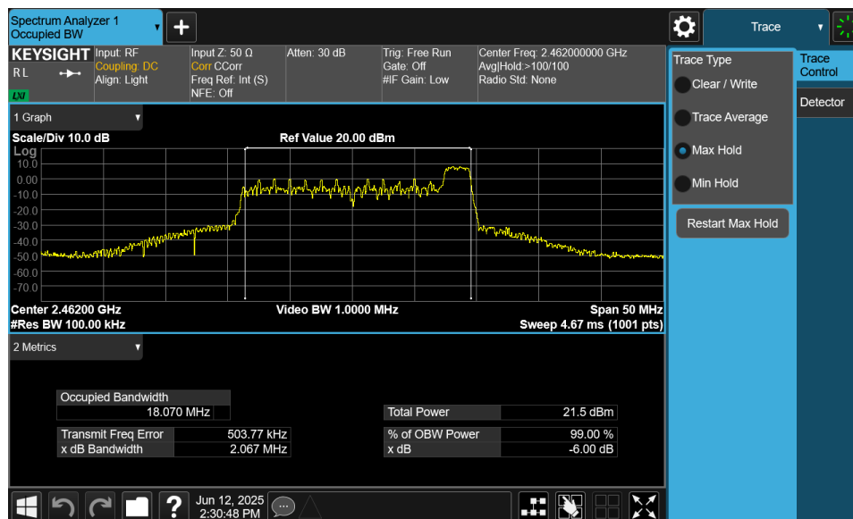
Plot 7-3. 6dB Bandwidth Plot MIMO ANT1 (802.11ax OFDMA – 26 Tones – Ch. 11)
