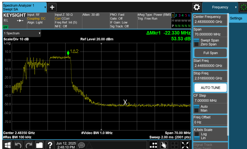
Plot 7-34. Band Edge Plot MIMO ANT2 (802.11ax OFDMA – 106 Tones – Ch. 11)
