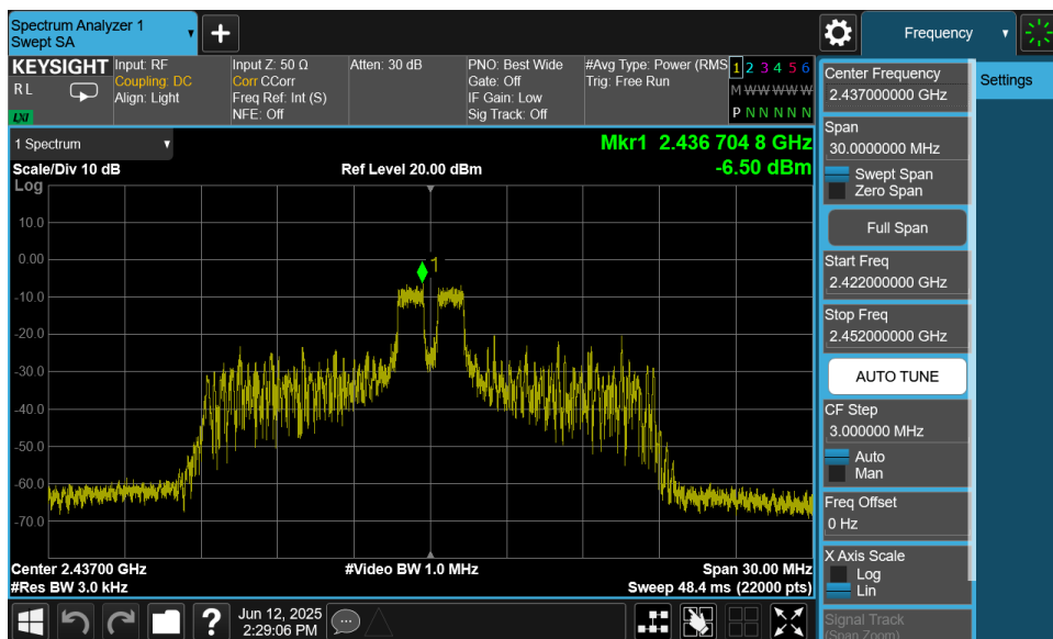
Plot 7-14. Power Spectral Density Plot MIMO ANT1 (802.11ax OFDMA – 26 Tones – Ch. 6)
