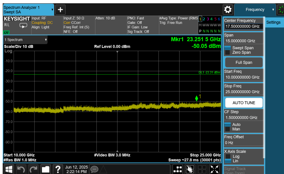
Plot 7-42. Conducted Spurious Plot MIMO ANT1 (802.11ax OFDMA – 26 Tones – Ch. 1)
