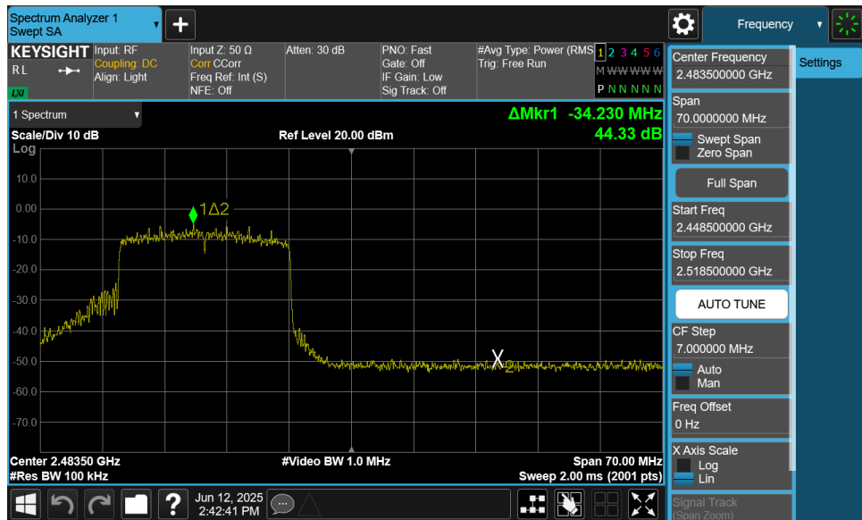
Plot 7-39. Band Edge Plot MIMO ANT2 (802.11ax OFDMA – 242 Tones – Ch. 12)
