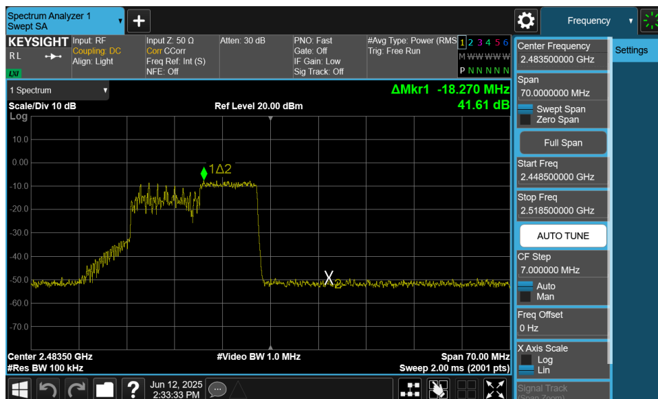
Plot 7-28. Band Edge Plot MIMO ANT1 (802.11ax OFDMA – 106 Tones – Ch. 13)
