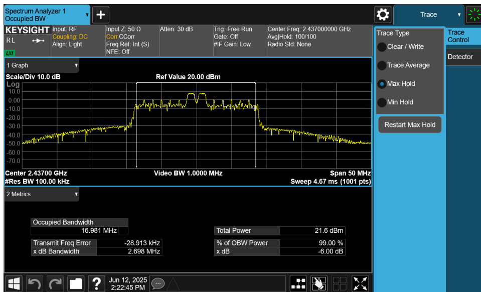
Plot 7-2. 6dB Bandwidth Plot MIMO ANT1 (802.11ax OFDMA – 26 Tones – Ch. 6)
