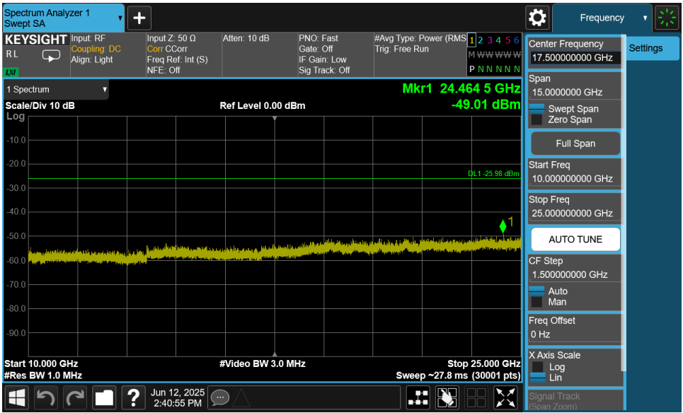
Plot 7-52. Conducted Spurious Plot MIMO ANT1 (802.11ax OFDMA – 242 Tones – Ch. 11)
