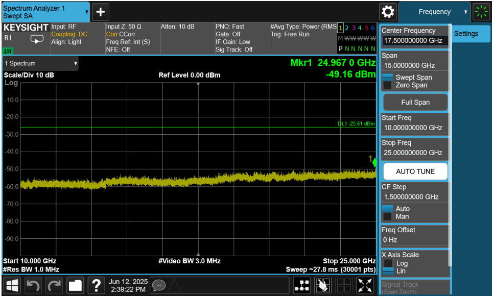
Plot 7-50. Conducted Spurious Plot MIMO ANT1 (802.11ax OFDMA – 242 Tones – Ch. 6)
