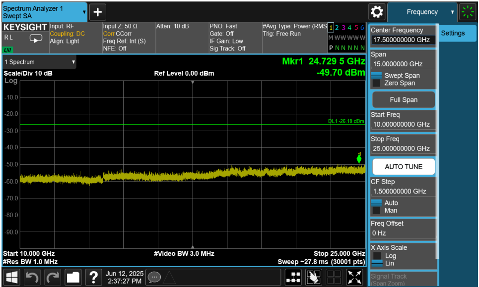
Plot 7-48. Conducted Spurious Plot MIMO ANT1 (802.11ax OFDMA – 242 Tones – Ch. 1)
