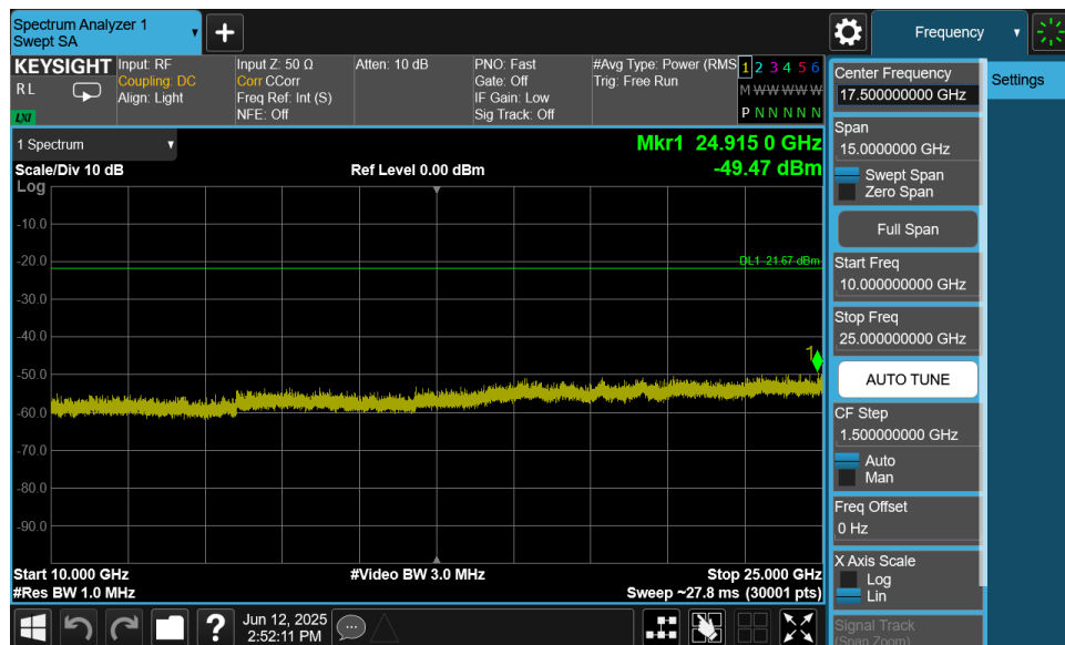
Plot 7-58. Conducted Spurious Plot MIMO ANT2 (802.11ax OFDMA – 26 Tones – Ch. 11)
