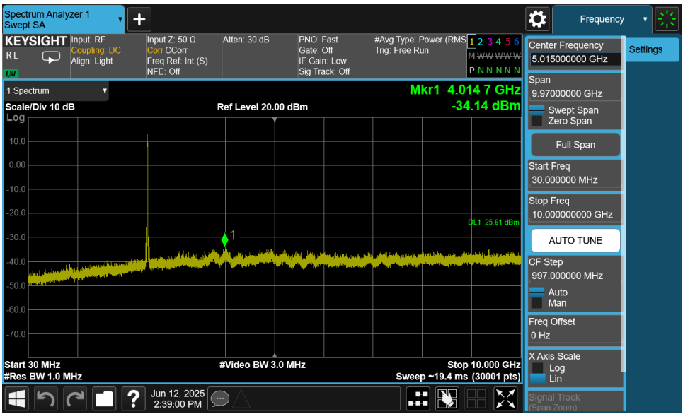
Plot 7-49. Conducted Spurious Plot MIMO ANT1 (802.11ax OFDMA – 242 Tones – Ch. 6)
