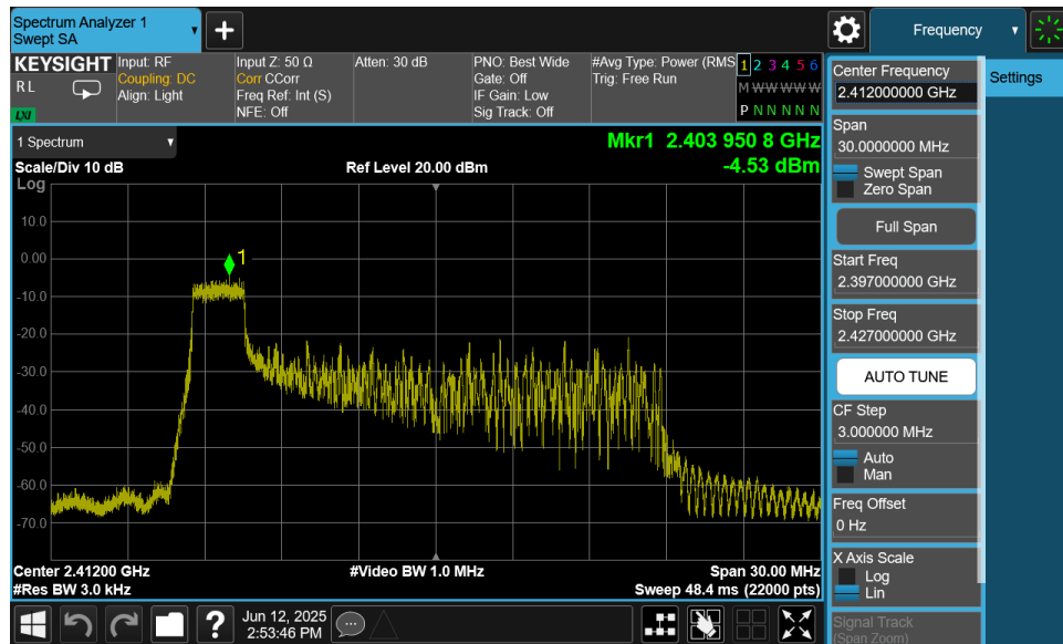
Plot 7-19. Power Spectral Density Plot MIMO ANT2 (802.11ax OFDMA – 26 Tones – Ch. 1)
