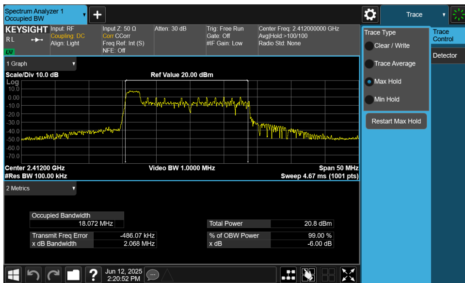
Plot 7-1. 6dB Bandwidth Plot MIMO ANT1 (802.11ax OFDMA – 26 Tones – Ch. 1)
