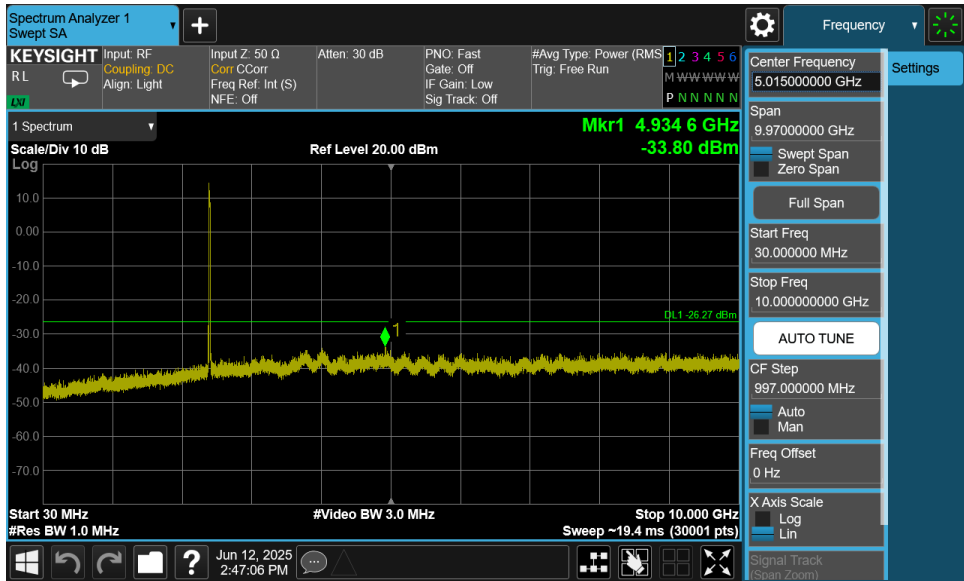
Plot 7-59. Conducted Spurious Plot MIMO ANT2 (802.11ax OFDMA – 242 Tones – Ch. 1)
