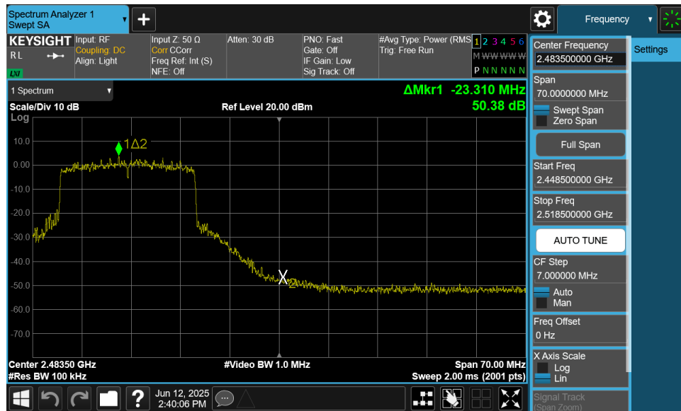
Plot 7-30. Band Edge Plot MIMO ANT1 (802.11ax OFDMA – 242 Tones – Ch. 11)
