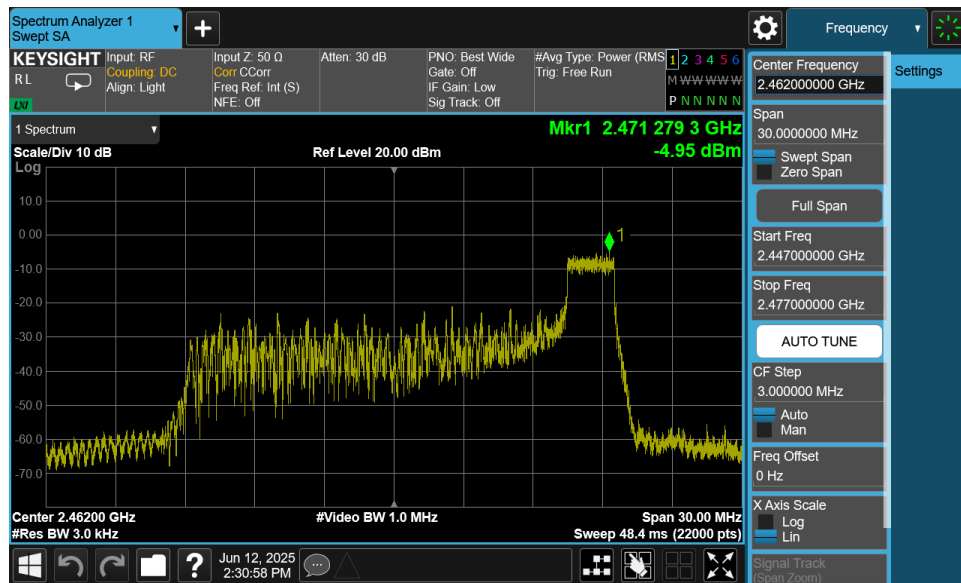
Plot 7-15. Power Spectral Density Plot MIMO ANT1 (802.11ax OFDMA – 26 Tones – Ch. 11)
