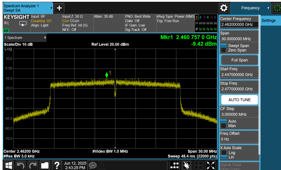
Plot 7-24. Power Spectral Density Plot MIMO ANT2 (802.11ax OFDMA – 242 Tones – Ch. 11)
