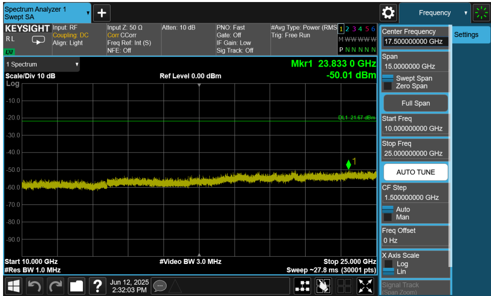
Plot 7-46. Conducted Spurious Plot MIMO ANT1 (802.11ax OFDMA – 26 Tones – Ch. 11)
