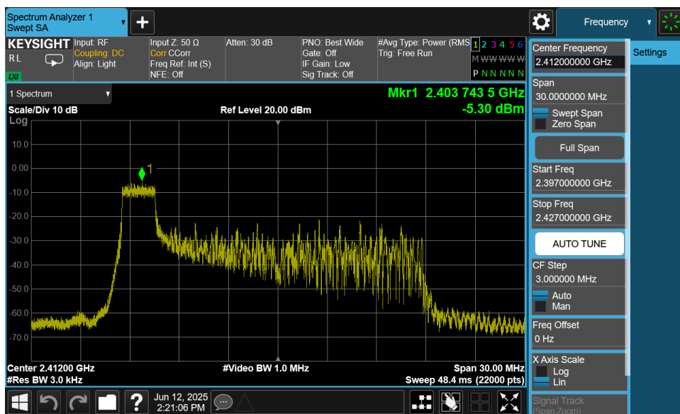
Plot 7-13. Power Spectral Density Plot MIMO ANT1 (802.11ax OFDMA – 26 Tones – Ch. 1)
