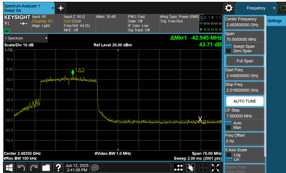
Plot 7-31. Band Edge Plot MIMO ANT1 (802.11ax OFDMA – 242 Tones – Ch. 12)
