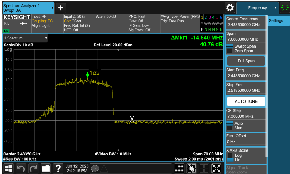
Plot 7-40. Band Edge Plot MIMO ANT2 (802.11ax OFDMA – 242 Tones – Ch. 13)
