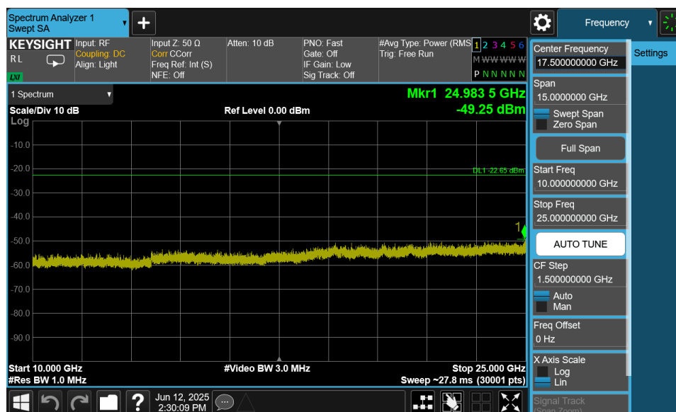
Plot 7-44. Conducted Spurious Plot MIMO ANT1 (802.11ax OFDMA – 26 Tones – Ch. 6)
