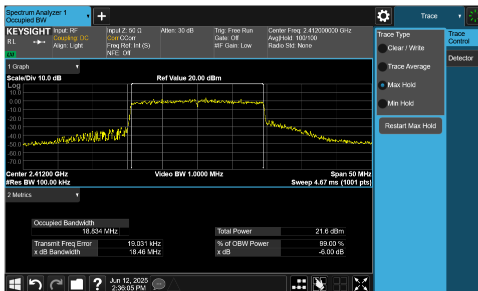
Plot 7-4. 6dB Bandwidth Plot MIMO ANT1 (802.11ax OFDMA – 242 Tones – Ch. 1)
