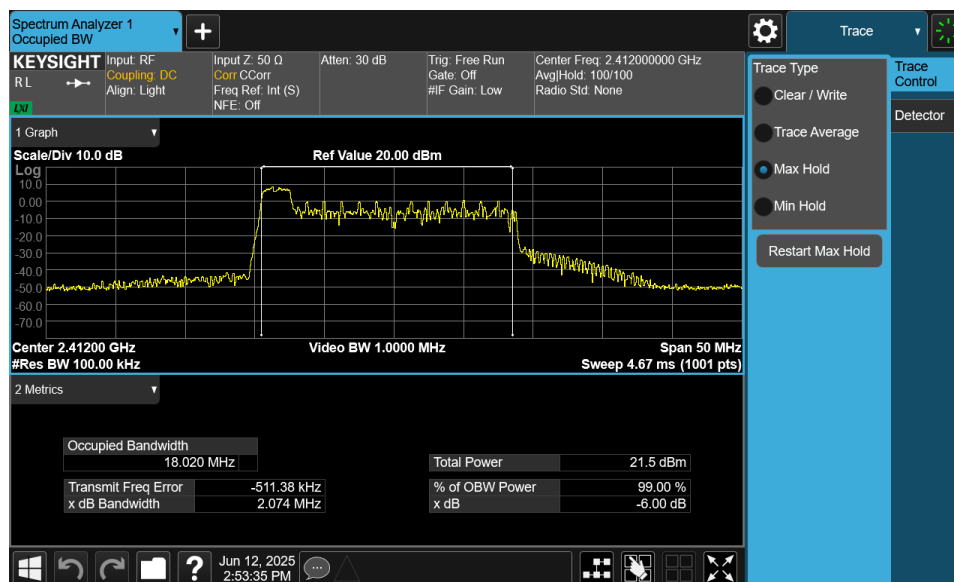
Plot 7-7. 6dB Bandwidth Plot MIMO ANT2 (802.11ax OFDMA – 26 Tones – Ch. 1)
