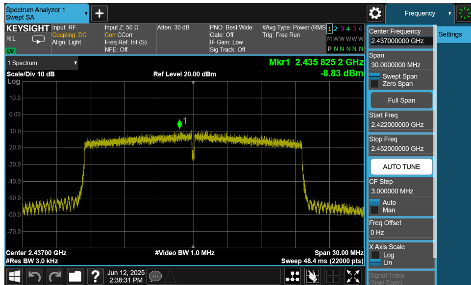
Plot 7-17. Power Spectral Density Plot MIMO ANT1 (802.11ax OFDMA – 242 Tones – Ch. 6)
