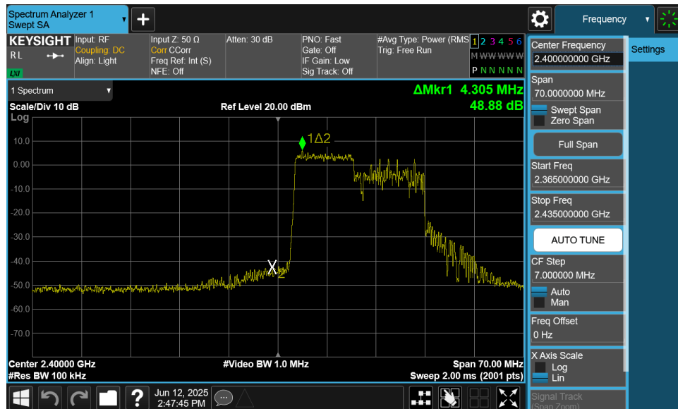
Plot 7-33. Band Edge Plot MIMO ANT2 (802.11ax OFDMA – 106 Tones – Ch. 1)
