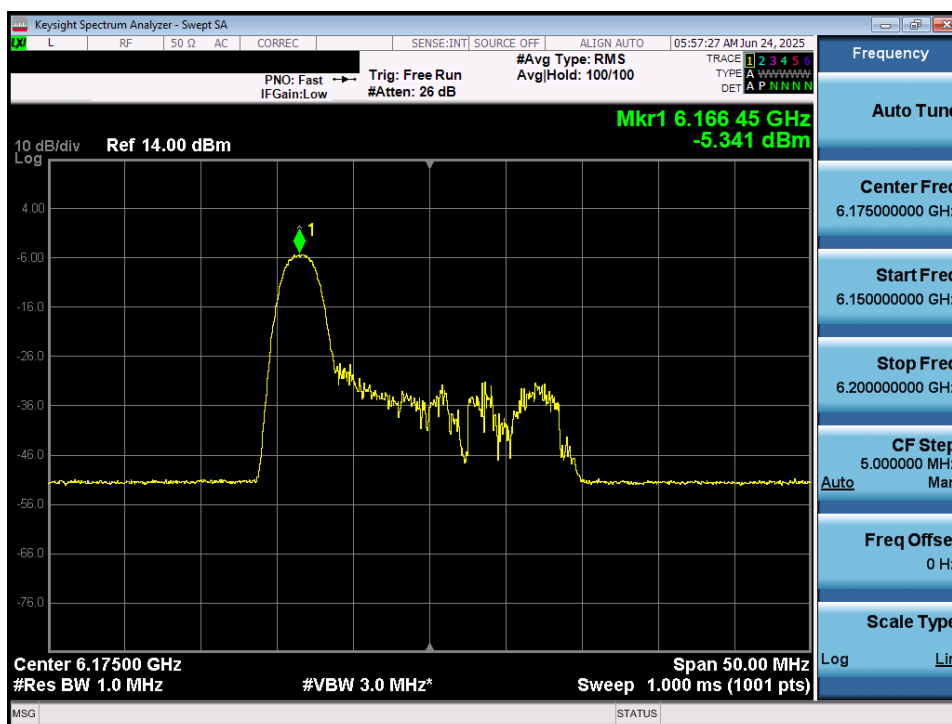
Plot 7-17. Power Spectral Density Plot MIMO ANT1 (20MHz 802.11ax (26 Tones) (UNII Band 5) – Ch. 45) - VLP
