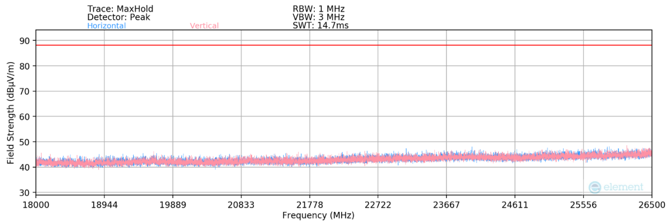
Plot 7-59. Radiated Spurious Plot 18GHz - 26.5GHz (802.11ax) – Ch. 45
