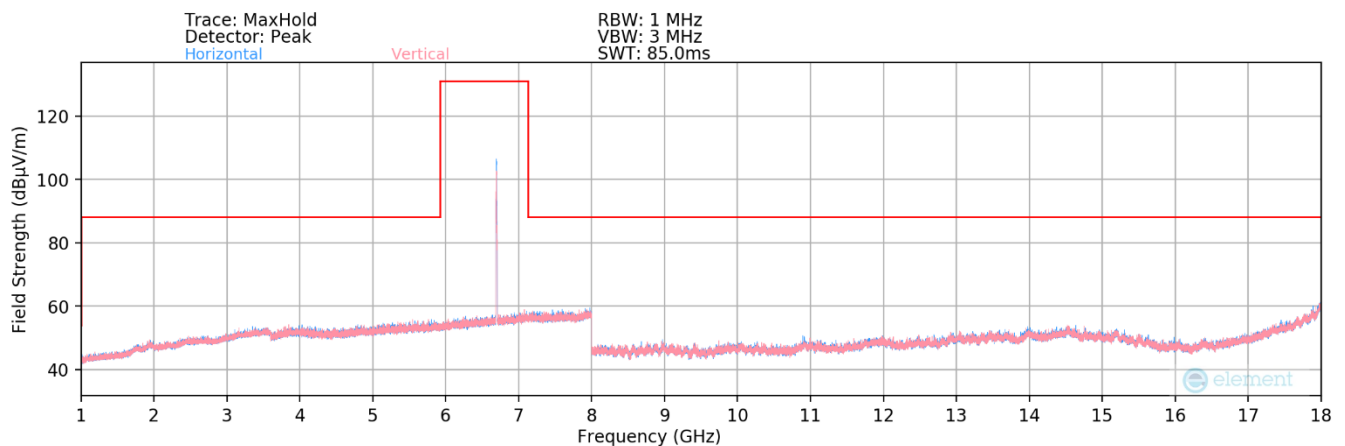
Plot 7-51. Radiated Spurious Plot 1GHz – 18GHz MIMO (802.11ax – UNII Band 7 Ch. 149)
