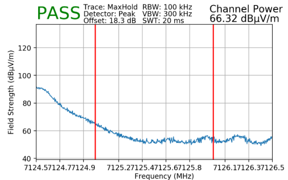
Plot 7-64. Radiated Upper Band Edge Plot MIMO (Peak – UNII Band 8 – 106T)
