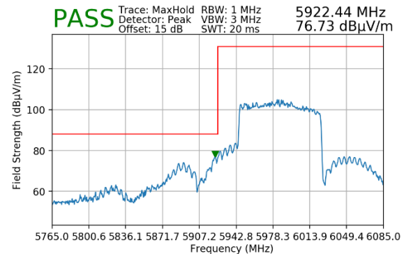
Plot 7-74. Radiated Lower Band Edge Plot MIMO (Peak – UNII Band 5 – 996T)
