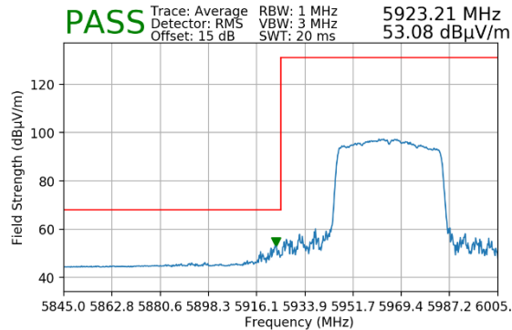
Plot 7-69. Radiated Lower Band Edge Plot MIMO (Average – UNII Band 5 – 484T)
