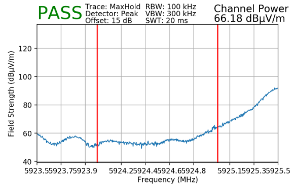
Plot 7-66. Radiated Lower Band Edge Plot MIMO (Peak – UNII Band 5 – 242T)
