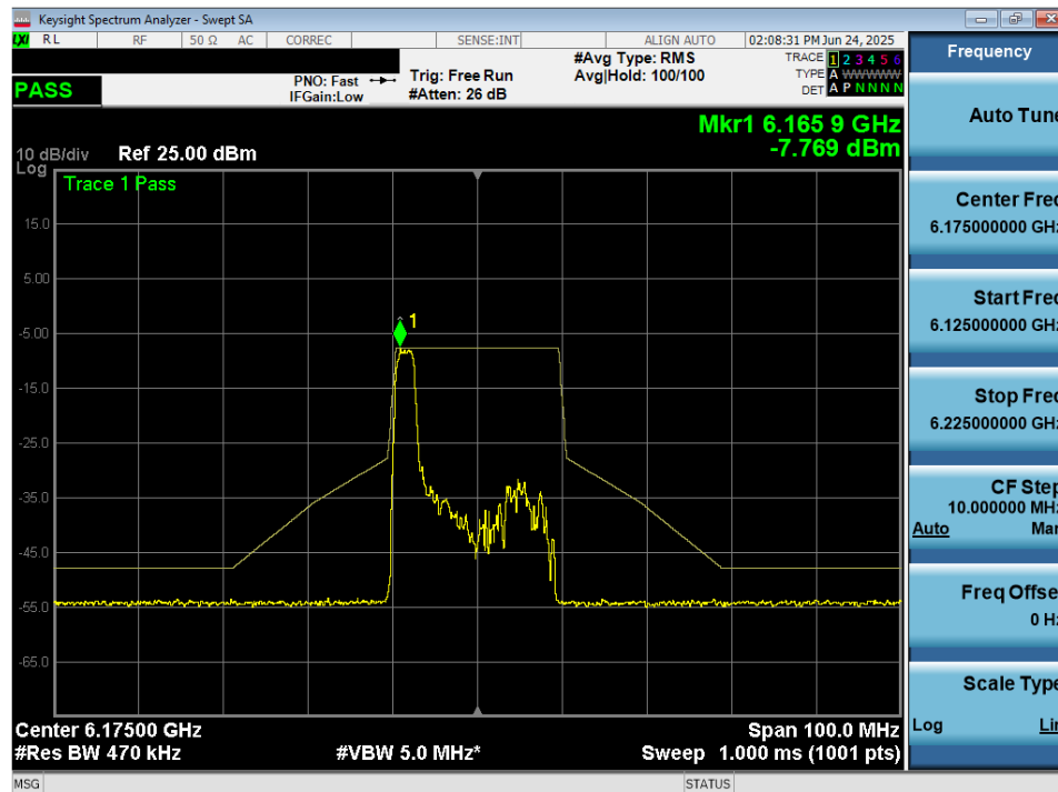
Plot 7-41. In Band Emissions Plot MIMO ANT2 (20MHz 802.11ax (26 Tones) (UNII Band 5) – Ch. 45) - VLP
