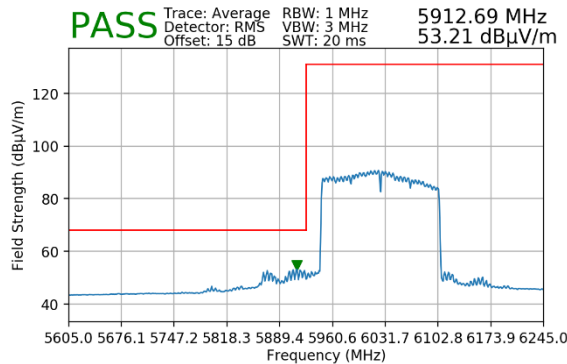
Plot 7-77. Radiated Lower Band Edge Plot MIMO (Average – UNII Band 5 – 2x996T)
