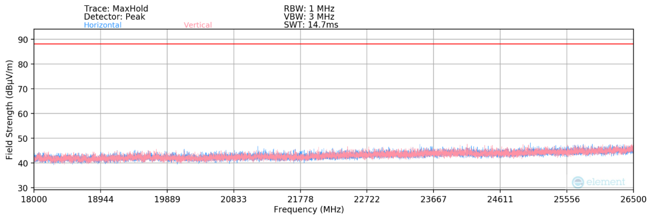
Plot 7-53. Radiated Spurious Plot 18GHz - 26.5GHz (802.11ax) – Ch. 45
