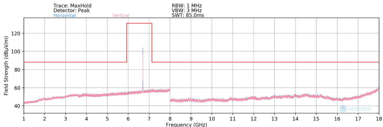
Plot 7-57. Radiated Spurious Plot 1GHz – 18GHz MIMO (802.11ax – UNII Band 7 Ch. 149)
