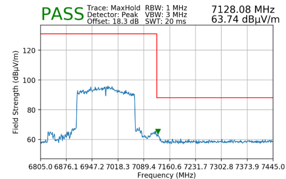
Plot 7-80. Radiated Upper Band Edge Plot MIMO (Peak – UNII Band 8 – 2x996T)
