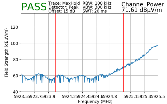
Plot 7-62. Radiated Lower Band Edge Plot MIMO (Peak – UNII Band 5 – 106T)
