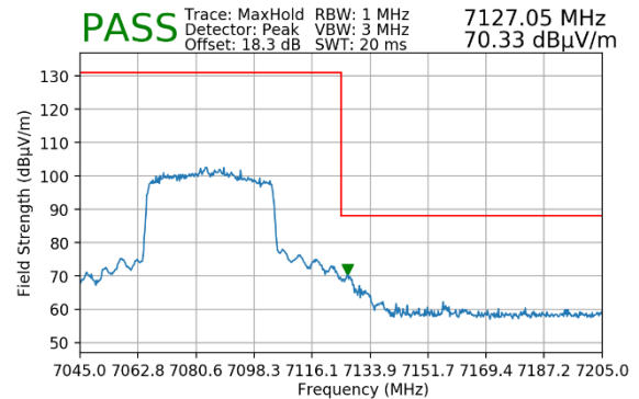
Plot 7-72. Radiated Upper Band Edge Plot MIMO (Peak – UNII Band 8 – 484T)
