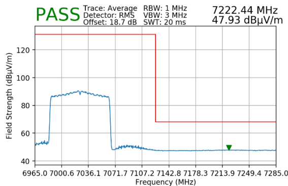
Plot 7-75. Radiated Upper Band Edge Plot MIMO (Average – UNII Band 8 – 996T)
