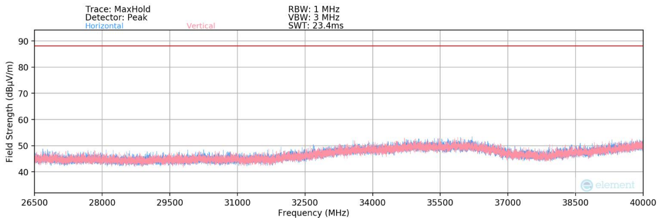
Plot 7-54. Radiated Spurious Plot 26.5GHz - 40GHz (802.11ax) – Ch. 45
