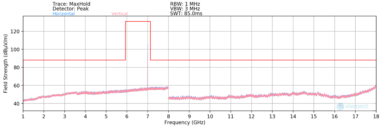
Plot 7-52. Radiated Spurious Plot 1GHz – 18GHz MIMO (802.11ax – UNII Band 8 Ch. 209)
