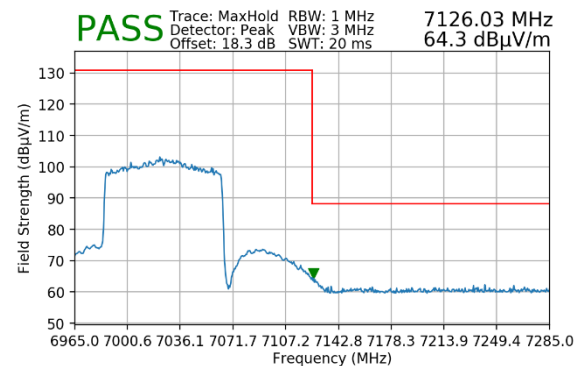
Plot 7-76. Radiated Upper Band Edge Plot MIMO (Peak – UNII Band 8 – 996T)
