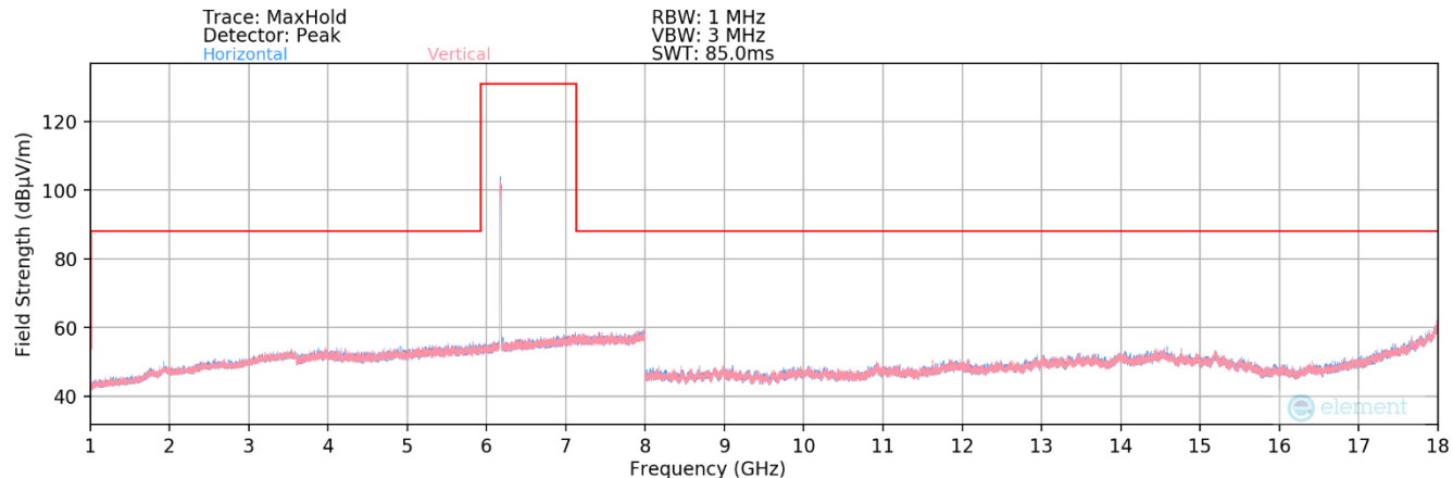
Plot 7-55. Radiated Spurious Plot 1GHz – 18GHz MIMO (802.11ax – UNII Band 5 Ch. 45)
