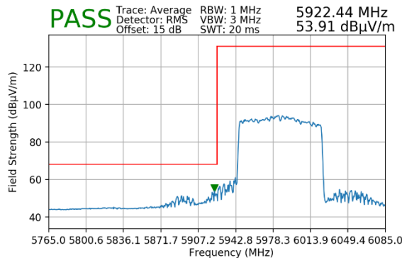
Plot 7-73. Radiated Lower Band Edge Plot MIMO (Average – UNII Band 5 – 996T)
