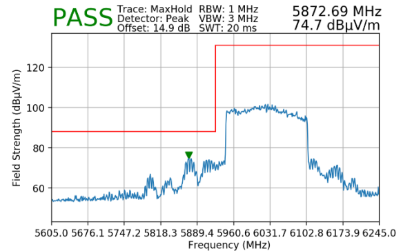
Plot 7-78. Radiated Lower Band Edge Plot MIMO (Peak – UNII Band 5 – 2x996T)
