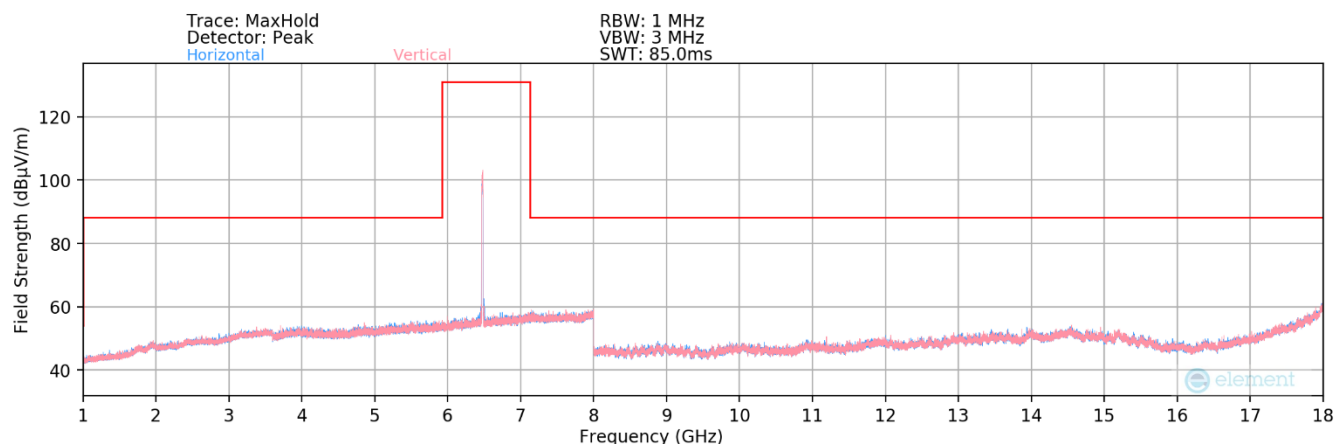
Plot 7-56. Radiated Spurious Plot 1GHz – 18GHz MIMO (802.11ax – UNII Band 6 Ch. 105)
