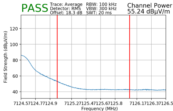
Plot 7-63. Radiated Upper Band Edge Plot MIMO (Average – UNII Band 8 – 106T)
