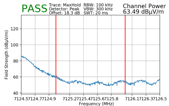
Plot 7-68. Radiated Upper Band Edge Plot MIMO (Peak – UNII Band 8 – 242T)
