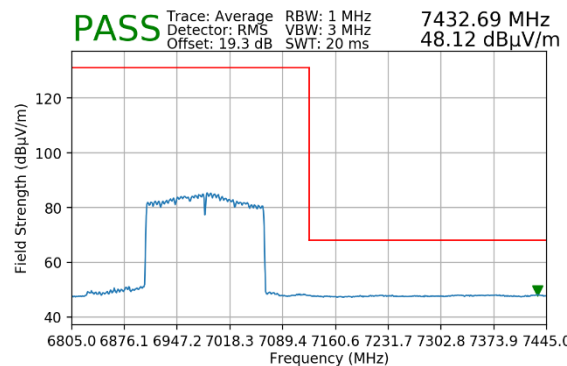
Plot 7-79. Radiated Upper Band Edge Plot MIMO (Average – UNII Band 8 – 2x996T)
