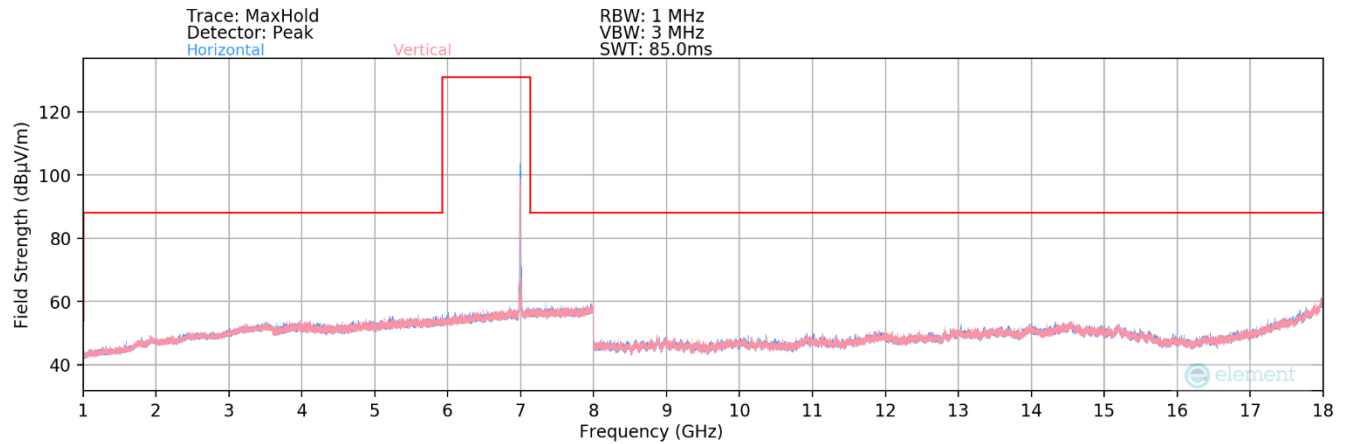
Plot 7-58. Radiated Spurious Plot 1GHz – 18GHz MIMO (802.11ax – UNII Band 8 Ch. 209)
