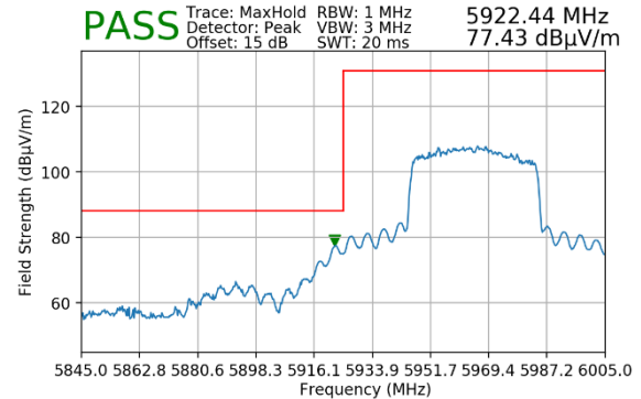
Plot 7-70. Radiated Lower Band Edge Plot MIMO (Peak – UNII Band 5 – 484T)
