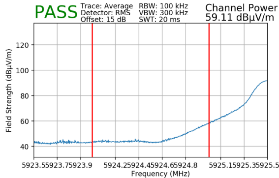
Plot 7-61. Radiated Lower Band Edge Plot MIMO (Average – UNII Band 5 – 106T)
