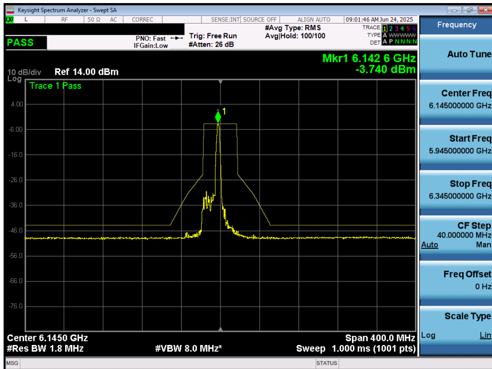
Plot 7-35. In Band Emissions Plot MIMO ANT1 (80MHz 802.11ax (26 Tones) (UNII Band 5) – Ch. 39) - VLP
