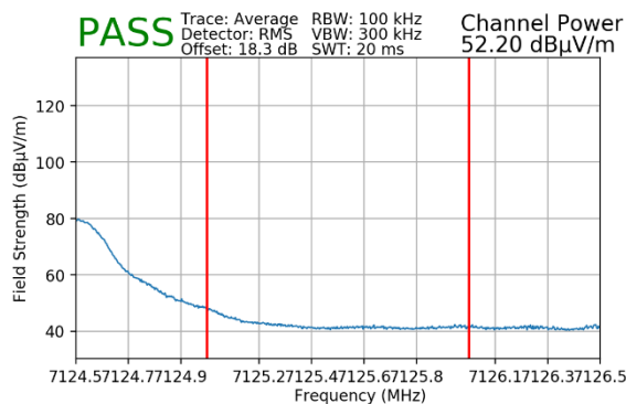
Plot 7-67. Radiated Upper Band Edge Plot MIMO (Average – UNII Band 8 – 242T)
