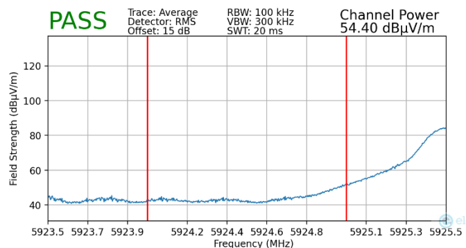
Plot 9-1. Radiated Lower Band Edge Plot MIMO (Average – UNII Band 5 – 242T) (Spot-check)
