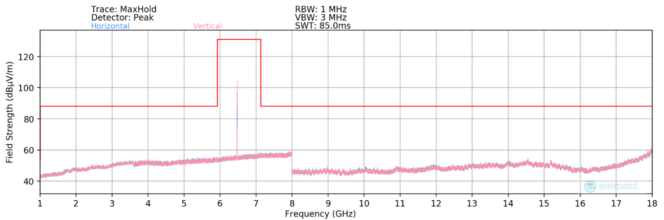
Plot 7-50. Radiated Spurious Plot 1GHz – 18GHz MIMO (802.11ax – UNII Band 6 Ch. 105)
