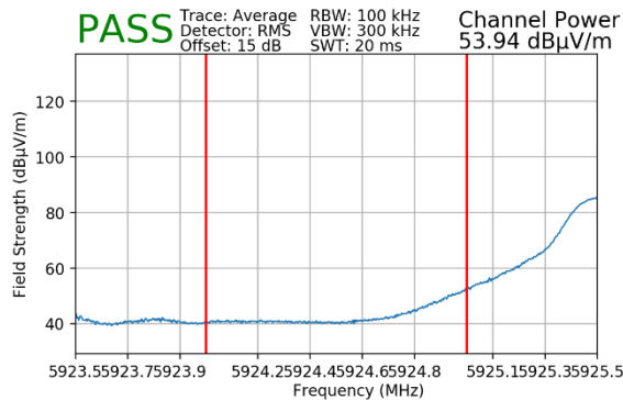
Plot 7-65. Radiated Lower Band Edge Plot MIMO (Average – UNII Band 5 – 242T)
