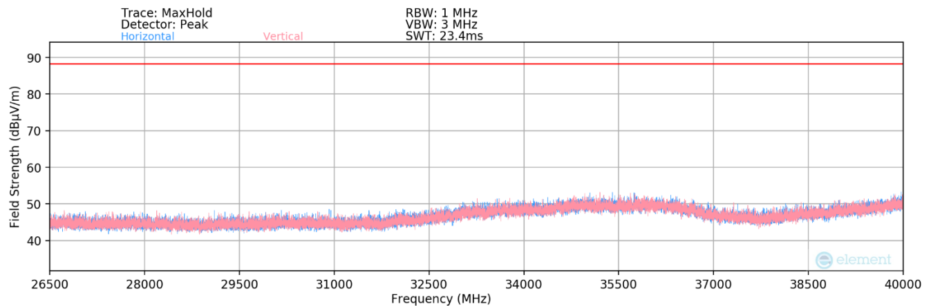
Plot 7-60. Radiated Spurious Plot 26.5GHz - 40GHz (802.11ax) – Ch. 45
