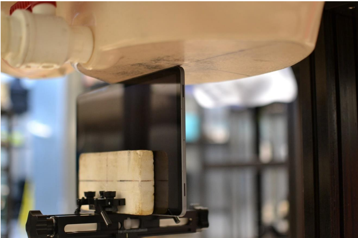
SAR Test Setup Photo 14 – Body, Left Edge at 0mm
