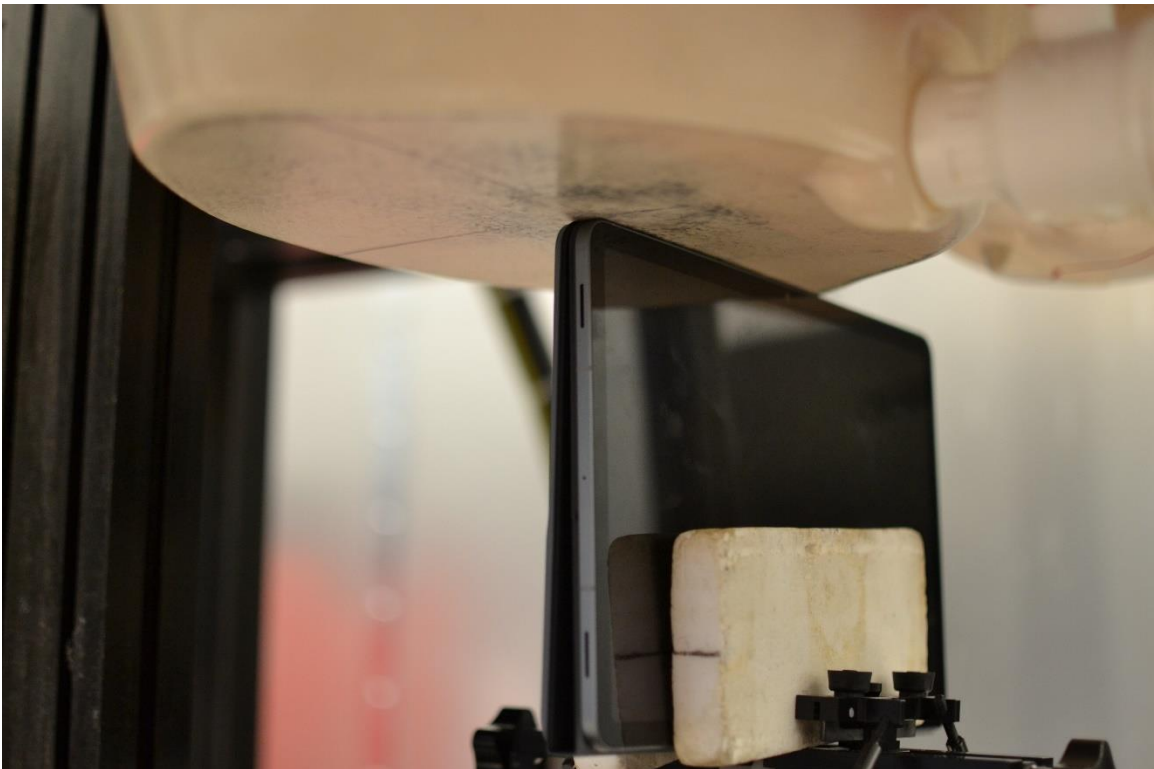
SAR Test Setup Photo 12 – Body with Keyboard, Right Edge at 0mm
