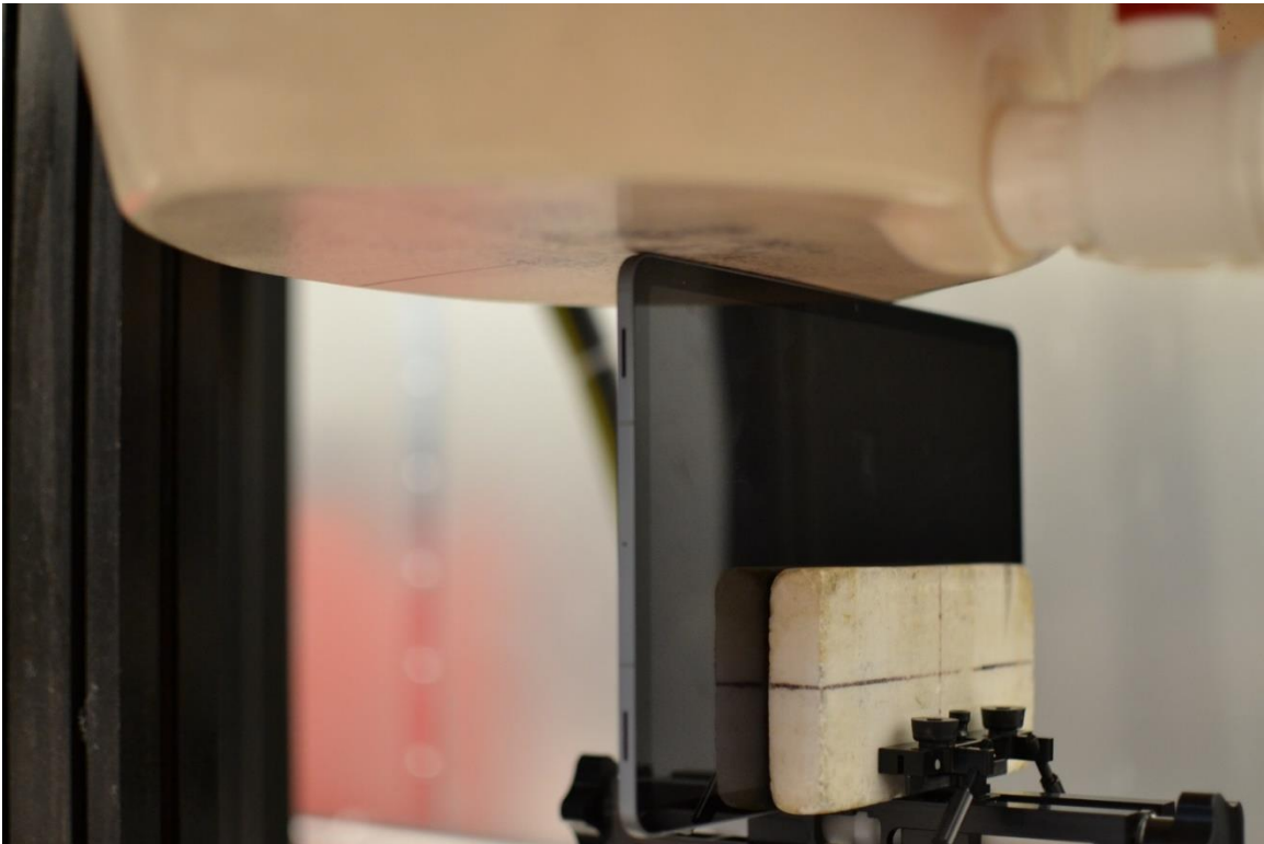
SAR Test Setup Photo 11 –Body, Right Edge at 0mm
