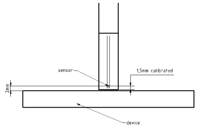
Figure J-5 EUmWVx Probe
