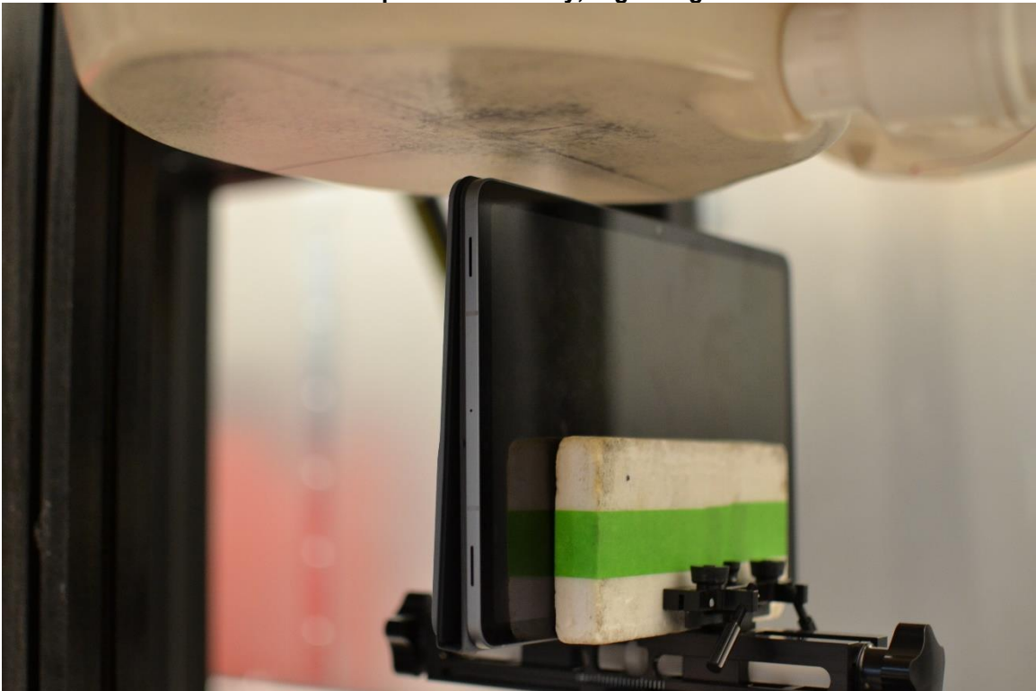
SAR Test Setup Photo 10 – Body with Keyboard, Right Edge at 11mm
