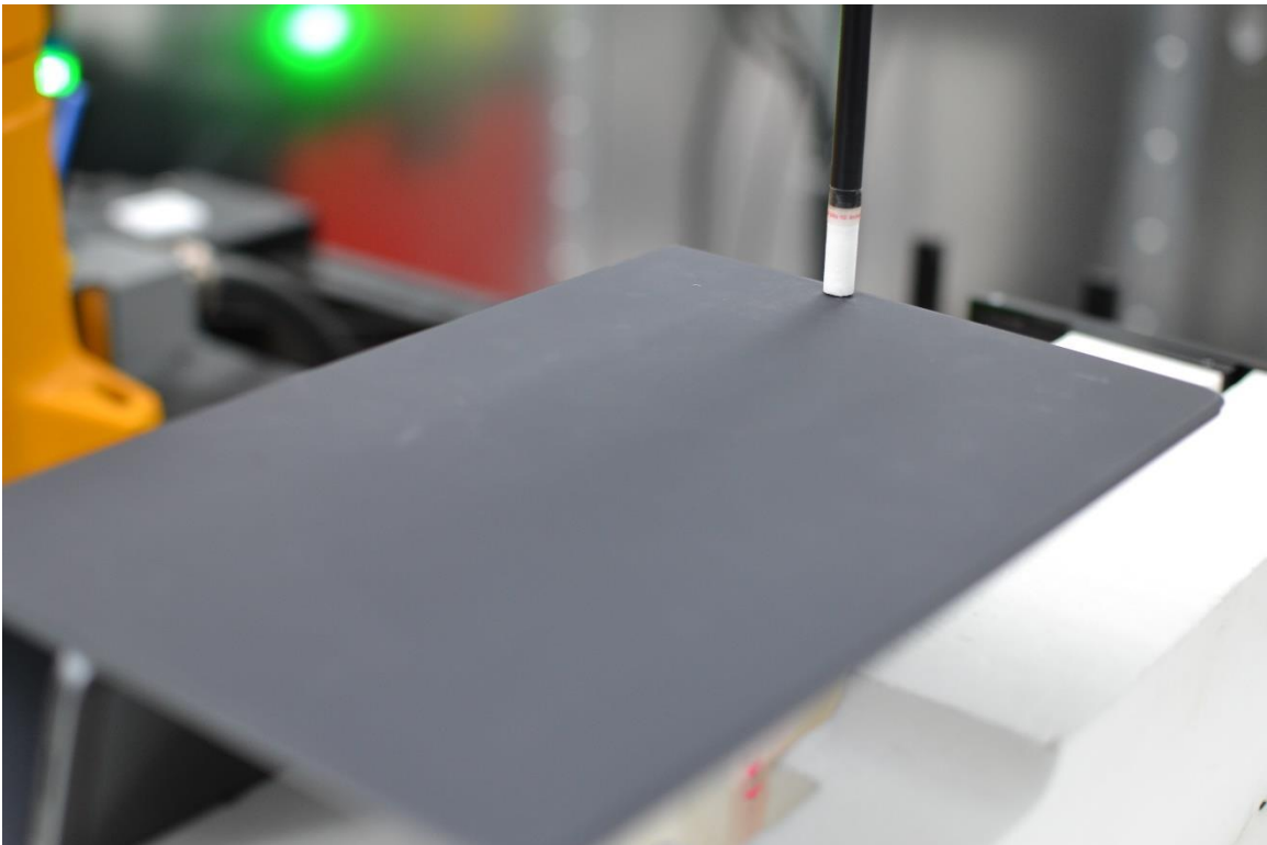
PD Test Setup Photo 21 – Laptop, Bottom Edge at 2mm
