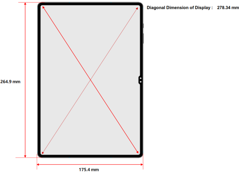
Figure I-2 DUT Dimensions Locations
