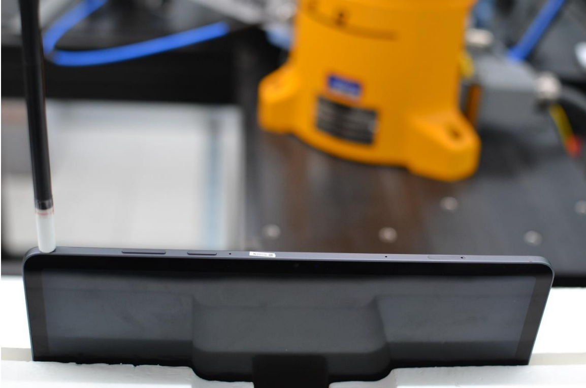
PD Test Setup Photo 18 – Body, Right Edge at 2mm
