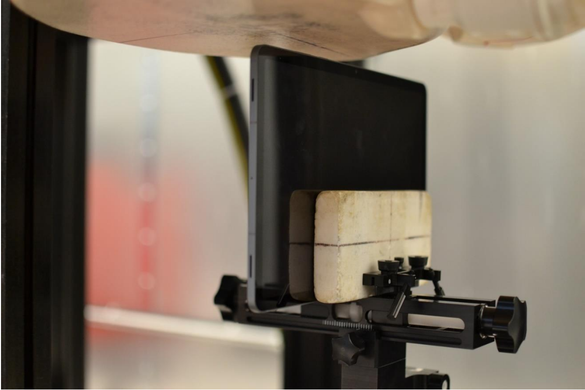
SAR Test Setup Photo 9 – Body, Right Edge at 11mm
