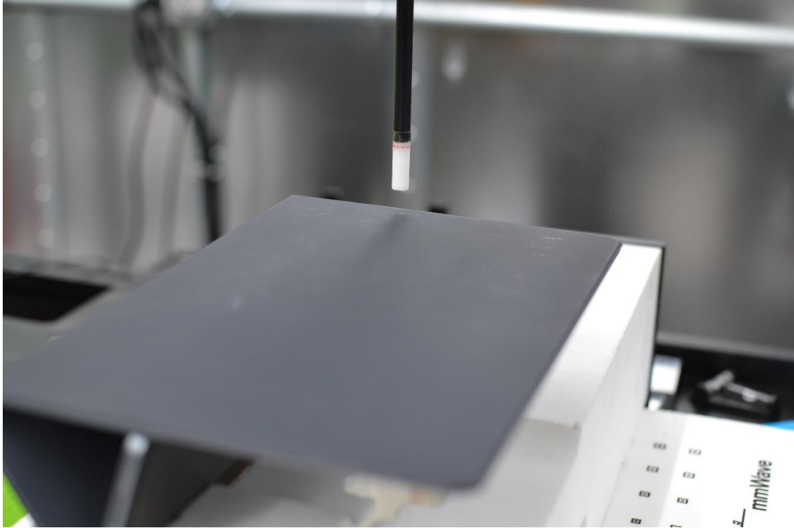
PD Test Setup Photo 22 – Laptop, Bottom Edge at 9.95mm
