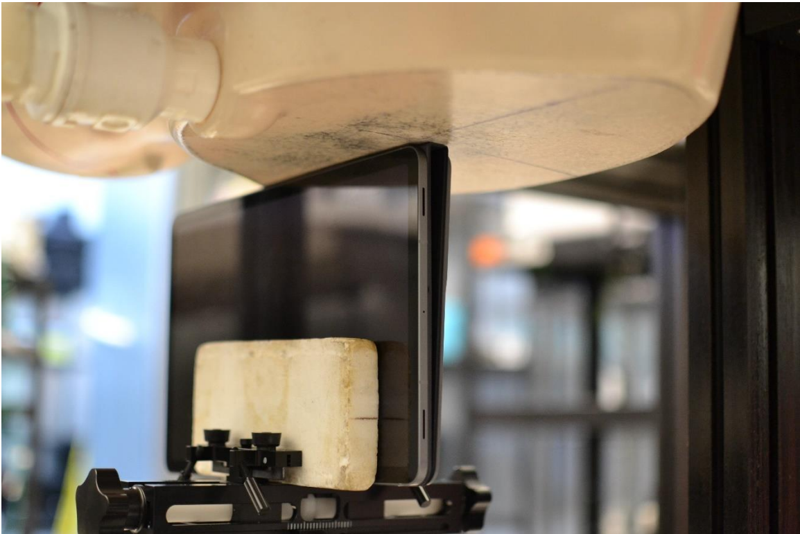
SAR Test Setup Photo 15 – Body with Keyboard, Left Edge at 0mm
