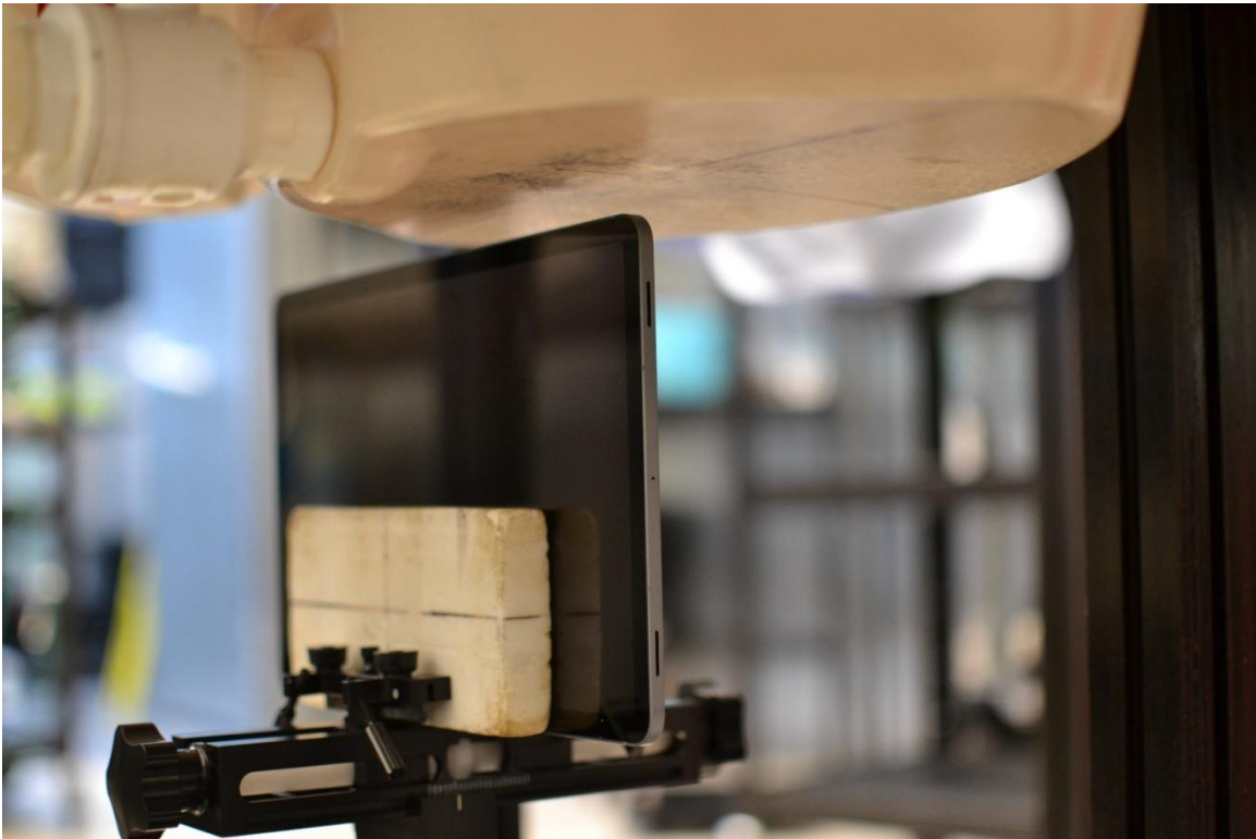
SAR Test Setup Photo 13 – Body, Left Edge at 11mm
