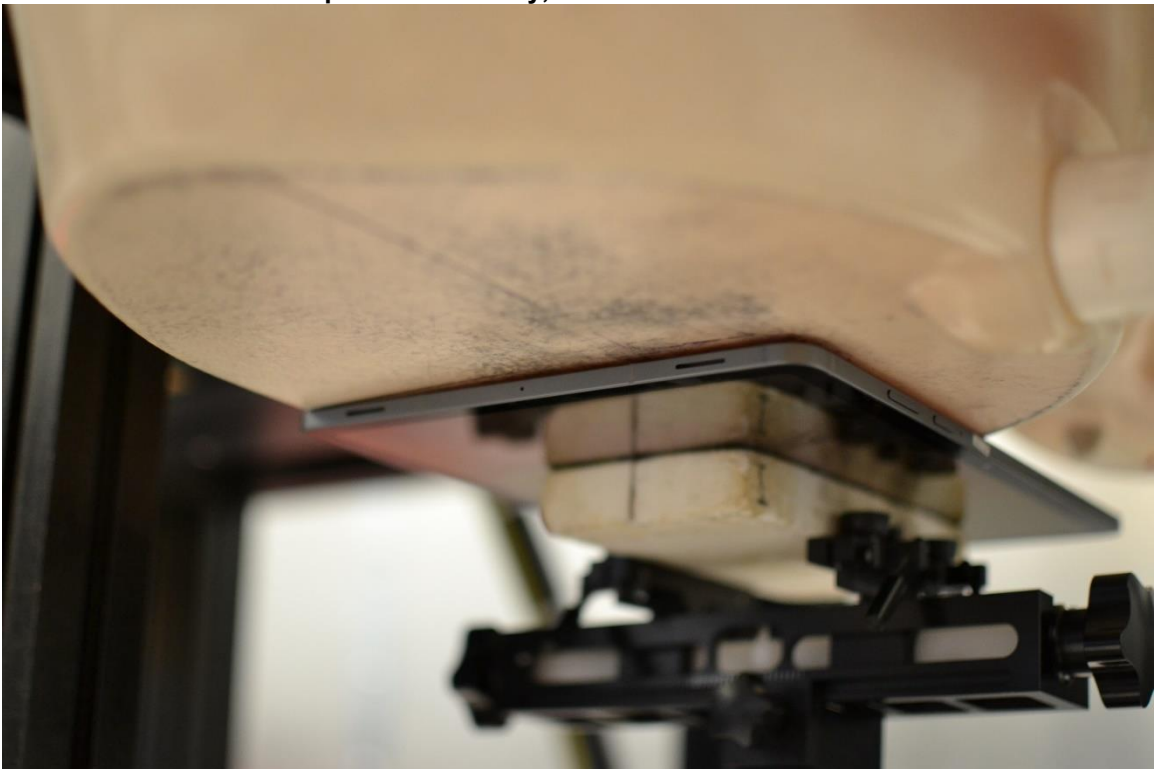
SAR Test Setup Photo 4 – Body, Back Side at 0mm– Antenna WIFI 1
