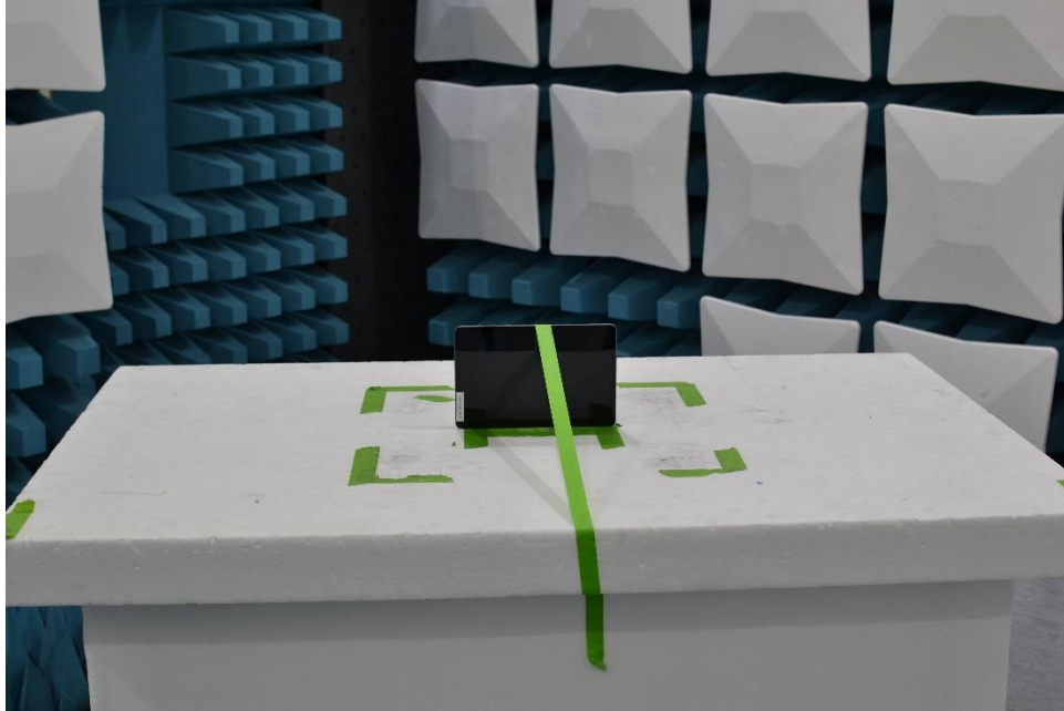
Plot 5. Test Setup – Y Orientation – below 1GHz
