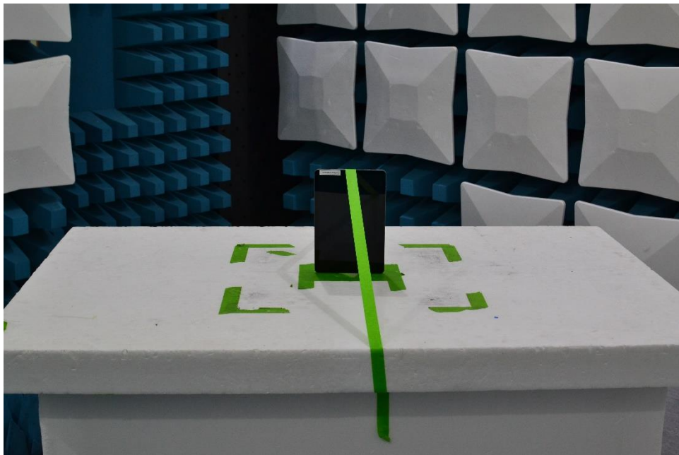
Plot 6. Test Setup – Z Orientation – below 1GHz
