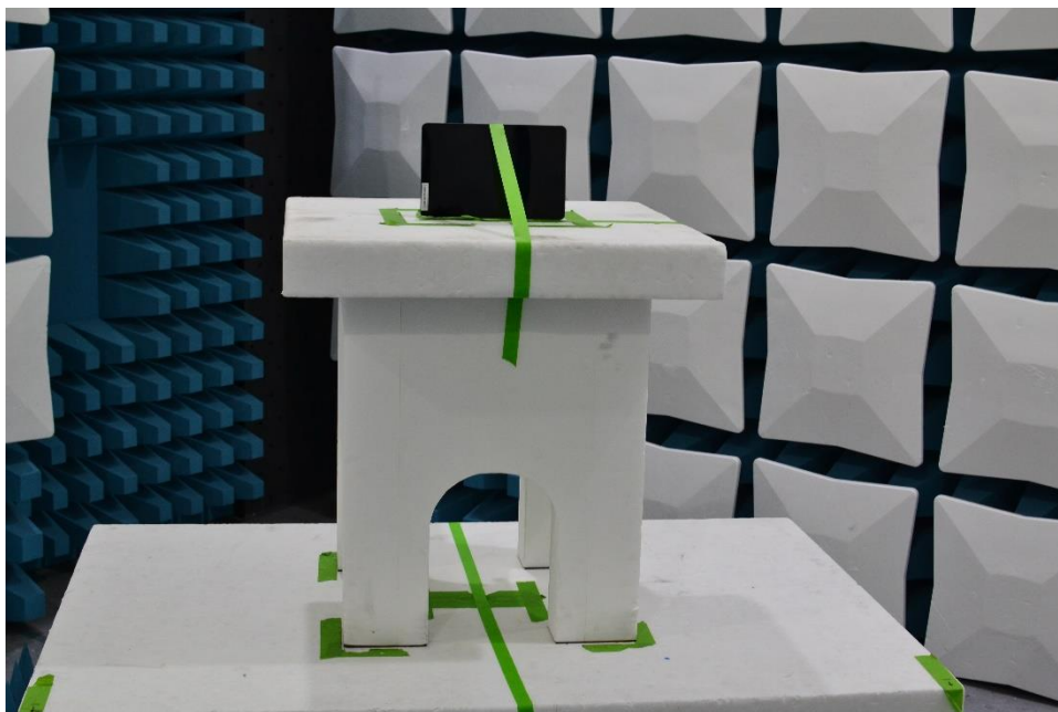
Plot 2. Test Setup – Y Orientation – Above 1GHz
