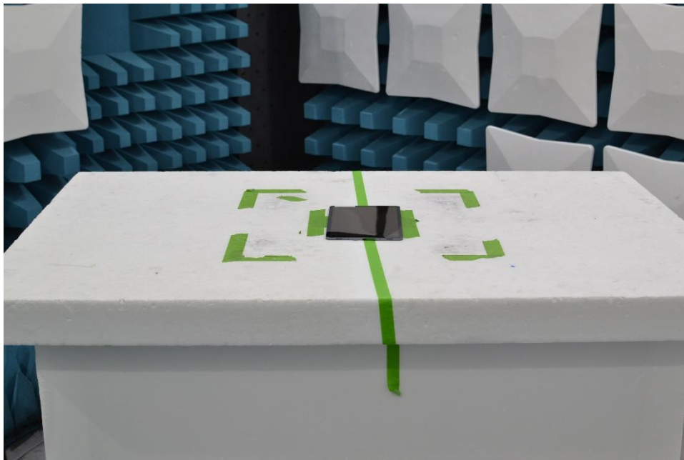
Plot 4. Test Setup – X Orientation – below 1GHz
