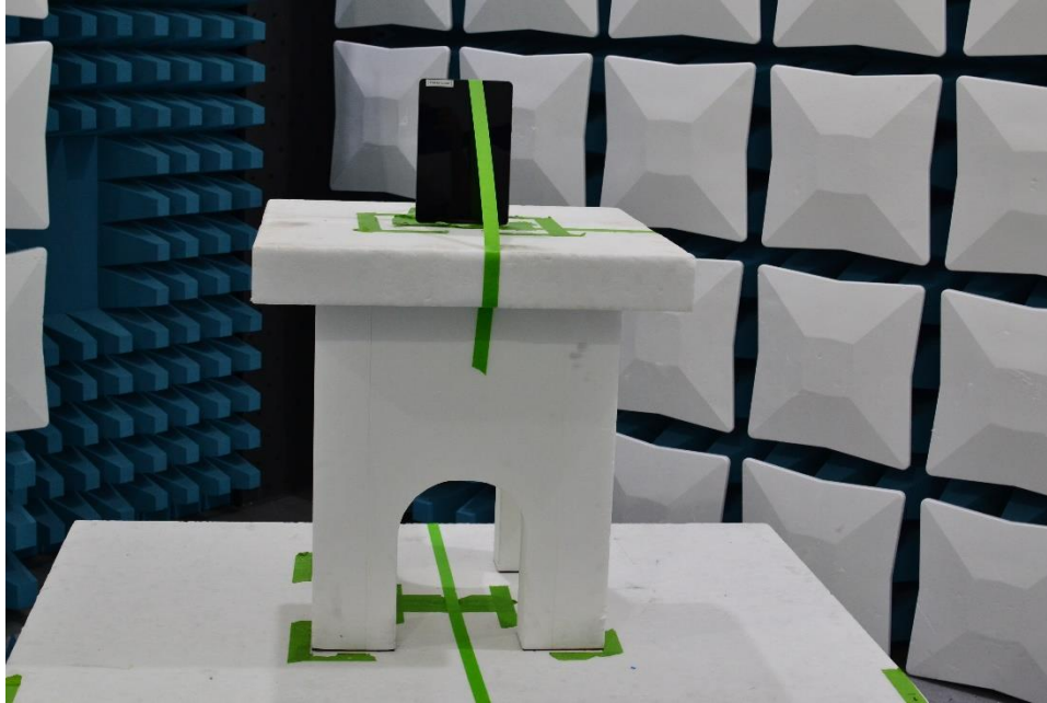
Plot 3. Test Setup – Z Orientation – Above 1GHz
