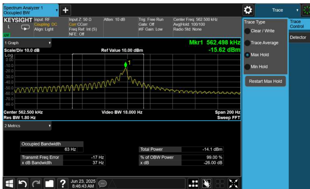
Figure 1-1 Occupied Bandwidth
