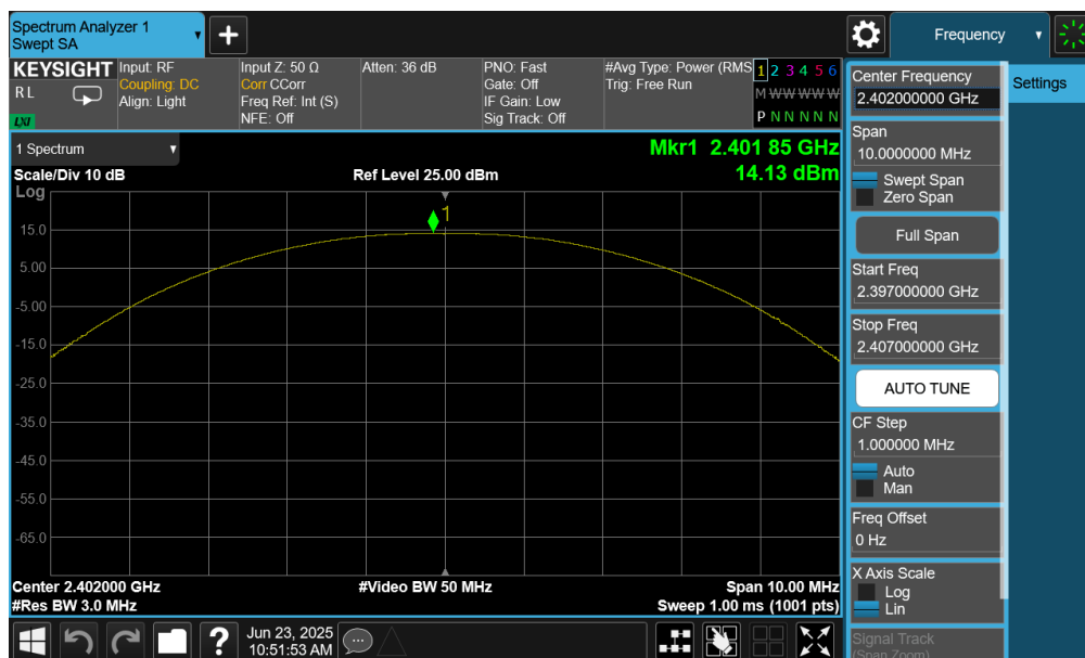
Plot 7-31. Peak Power Plot (Bluetooth (LE), 1Mbps – Ch. 37) – Ant 1
