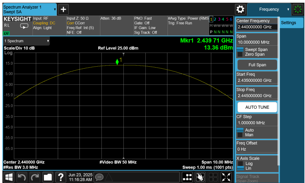
Plot 7-44. Peak Power Plot (Bluetooth (LE), 1Mbps – Ch. 17) – Ant 2
