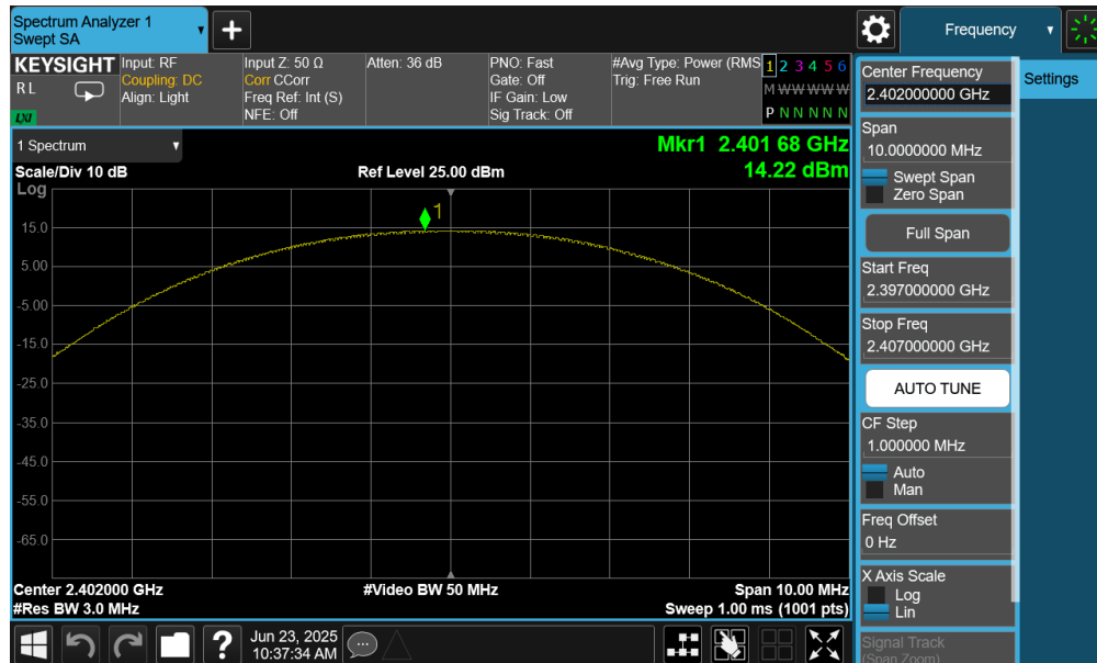
Plot 7-25. Peak Power Plot (Bluetooth (LE), 125kbps – Ch. 37) – Ant 1
