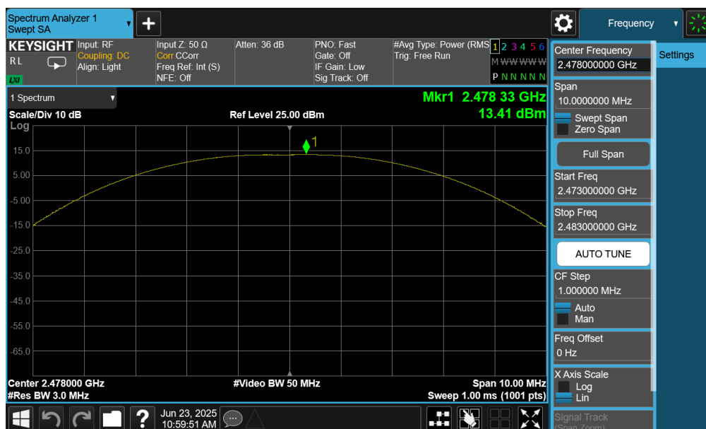
Plot 7-36. Peak Power Plot (Bluetooth (LE), 2Mbps – Ch. 36) – Ant 1
