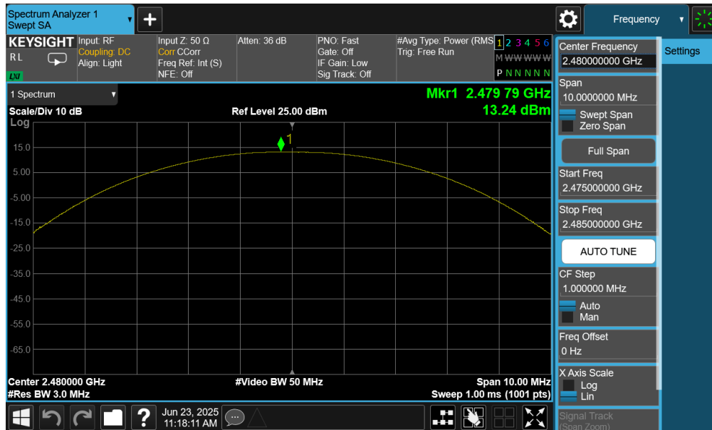
Plot 7-45. Peak Power Plot (Bluetooth (LE), 1Mbps – Ch. 39) – Ant 2
