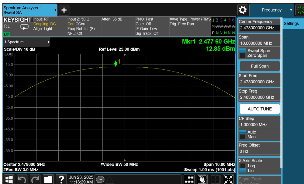
Plot 7-48. Peak Power Plot (Bluetooth (LE), 2Mbps – Ch. 36) – Ant 2
