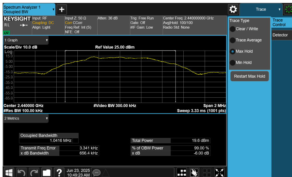
Plot 7-5. 6dB Bandwidth Plot (Bluetooth (LE), 500kbps – Ch. 17) – Ant 1
