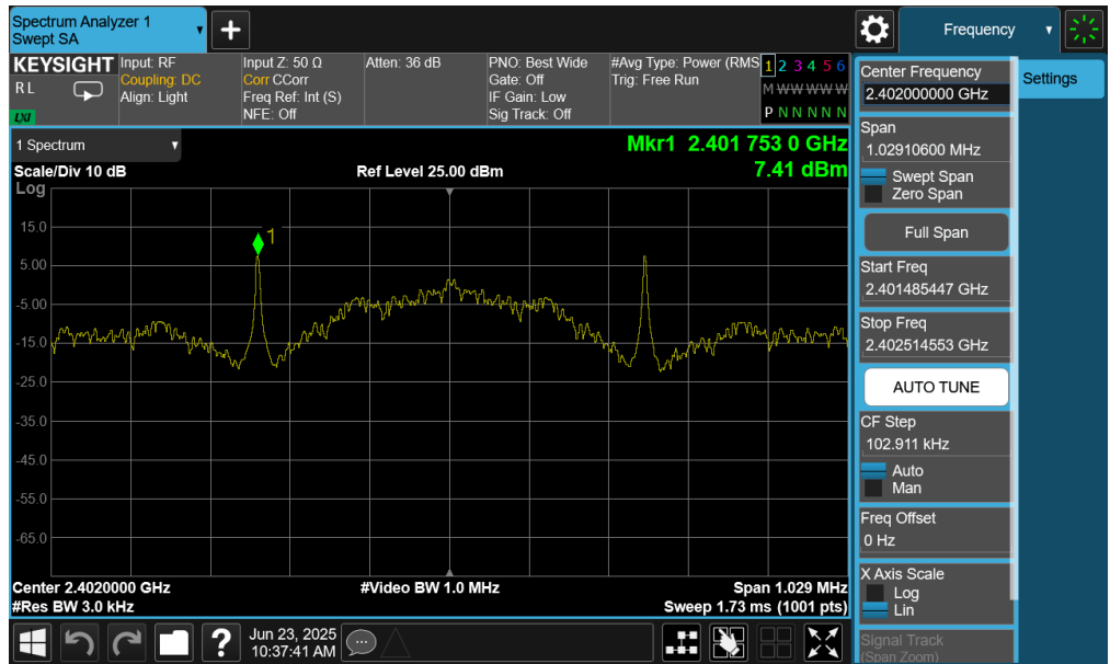
Plot 7-49. Power Spectral Density Plot (Bluetooth (LE), 125kbps – Ch. 37) – Ant 1
