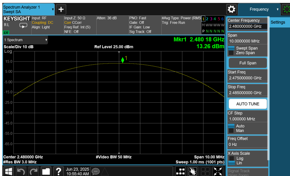
Plot 7-33. Peak Power Plot (Bluetooth (LE), 1Mbps – Ch. 39) – Ant 1
