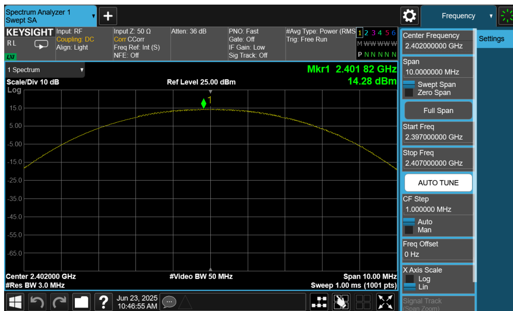
Plot 7-28. Peak Power Plot (Bluetooth (LE), 500kbps – Ch. 37) – Ant 1
