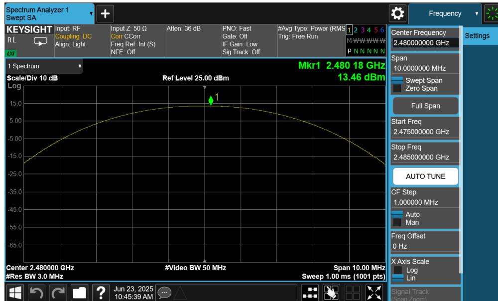
Plot 7-27. Peak Power Plot (Bluetooth (LE), 125kbps – Ch. 39) – Ant 1
