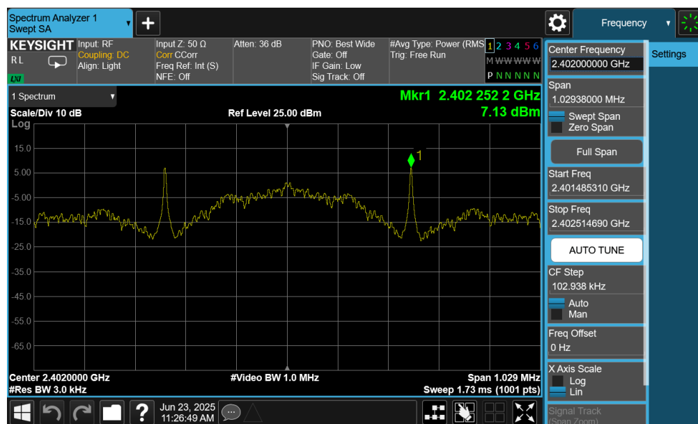
Plot 7-61. Power Spectral Density Plot (Bluetooth (LE), 125kbps – Ch. 37) – Ant 2
