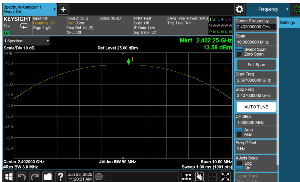
Plot 7-40. Peak Power Plot (Bluetooth (LE), 500kbps – Ch. 37) – Ant 2
