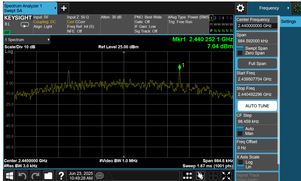
Plot 7-53. Power Spectral Density Plot (Bluetooth (LE), 500kbps – Ch. 17) – Ant 1
