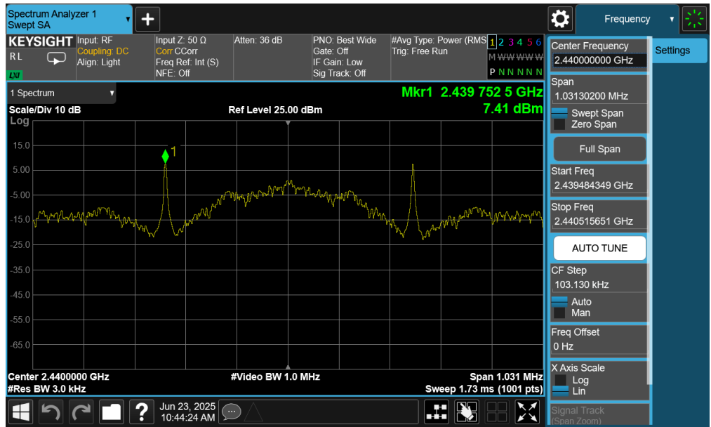
Plot 7-50. Power Spectral Density Plot (Bluetooth (LE), 125kbps – Ch. 17) – Ant 1
