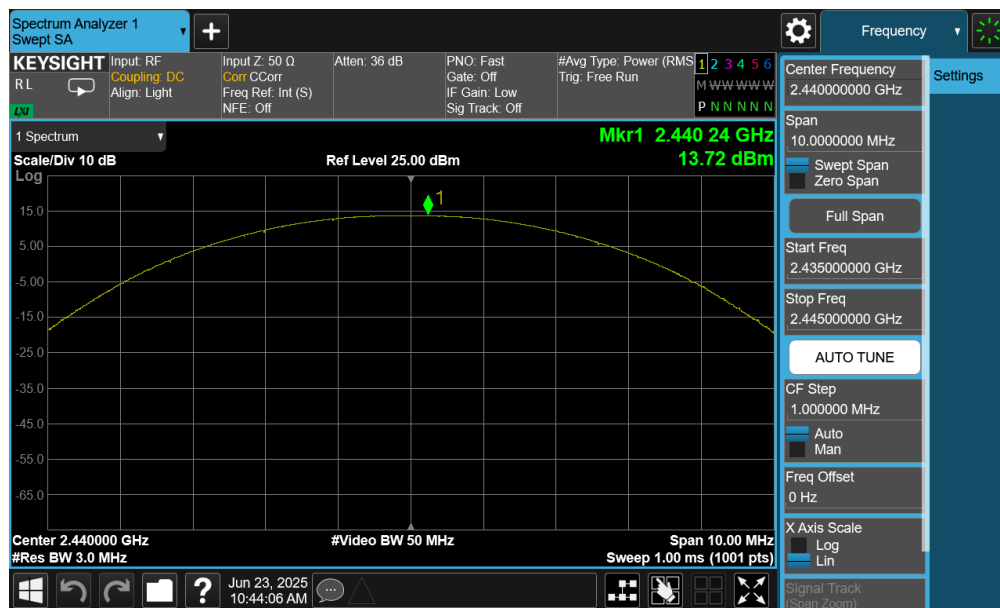
Plot 7-26. Peak Power Plot (Bluetooth (LE), 125kbps – Ch. 17) – Ant 1
