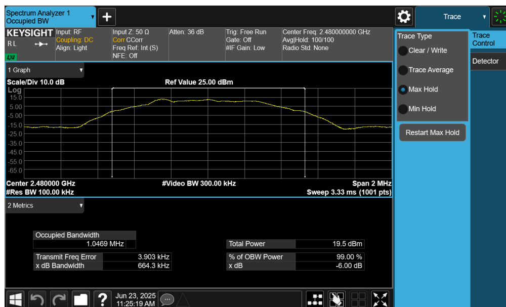
Plot 7-18. 6dB Bandwidth Plot (Bluetooth (LE), 500kbps – Ch. 39) – Ant 2
