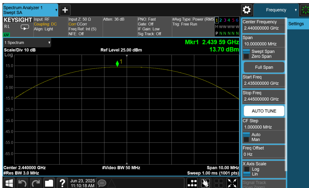
Plot 7-47. Peak Power Plot (Bluetooth (LE), 2Mbps – Ch. 17) – Ant 2
