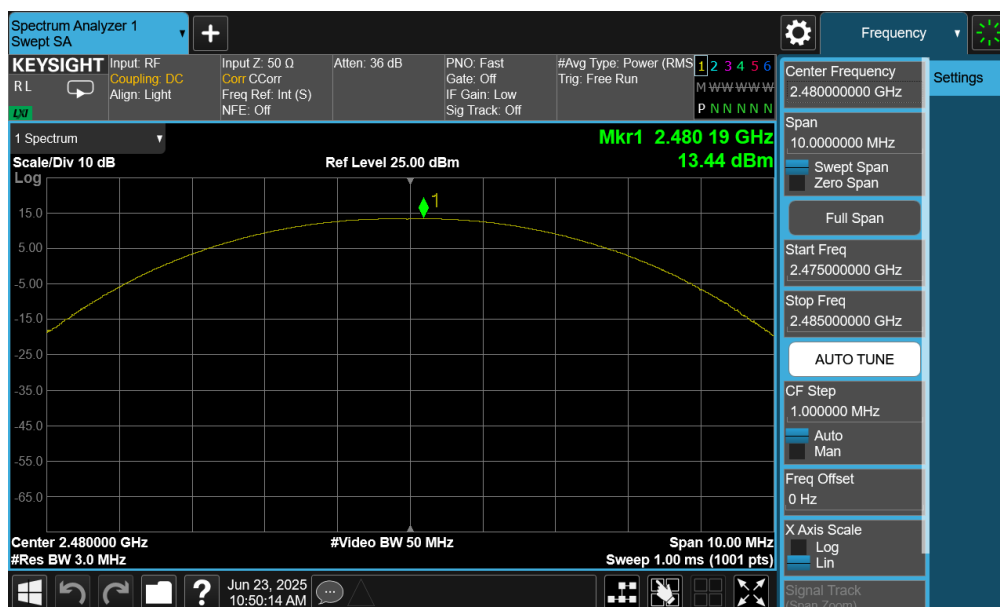
Plot 7-30. Peak Power Plot (Bluetooth (LE), 500kbps – Ch. 39) – Ant 1
