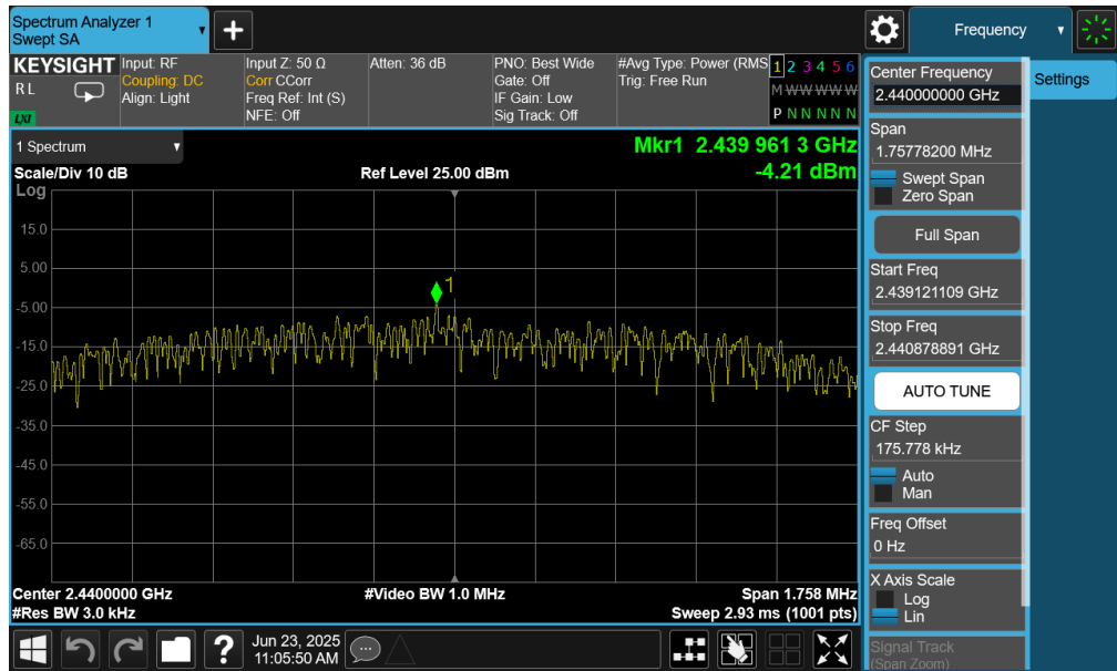
Plot 7-59. Power Spectral Density Plot (Bluetooth (LE), 2Mbps – Ch. 17) – Ant 1
