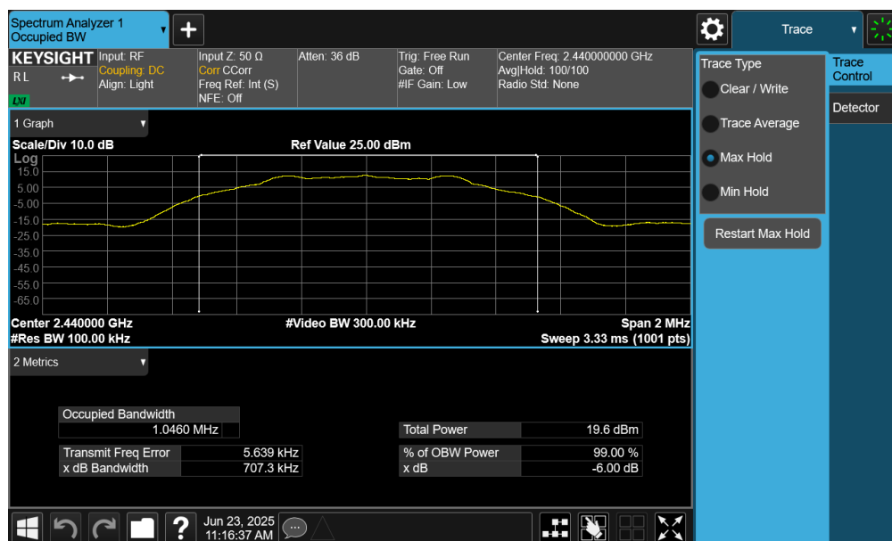
Plot 7-20. 6dB Bandwidth Plot (Bluetooth (LE), 1Mbps – Ch. 17) – Ant 2
