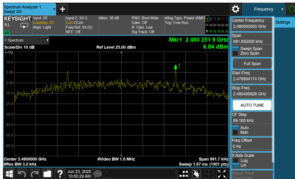
Plot 7-54. Power Spectral Density Plot (Bluetooth (LE), 500kbps – Ch. 39) – Ant 1
