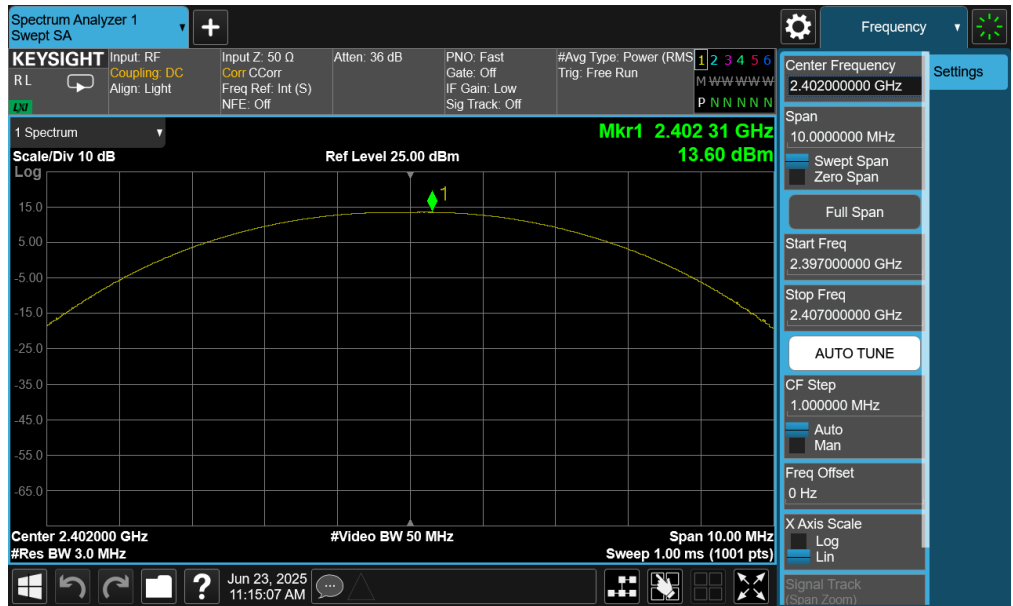
Plot 7-43. Peak Power Plot (Bluetooth (LE), 1Mbps – Ch. 37) – Ant 2
