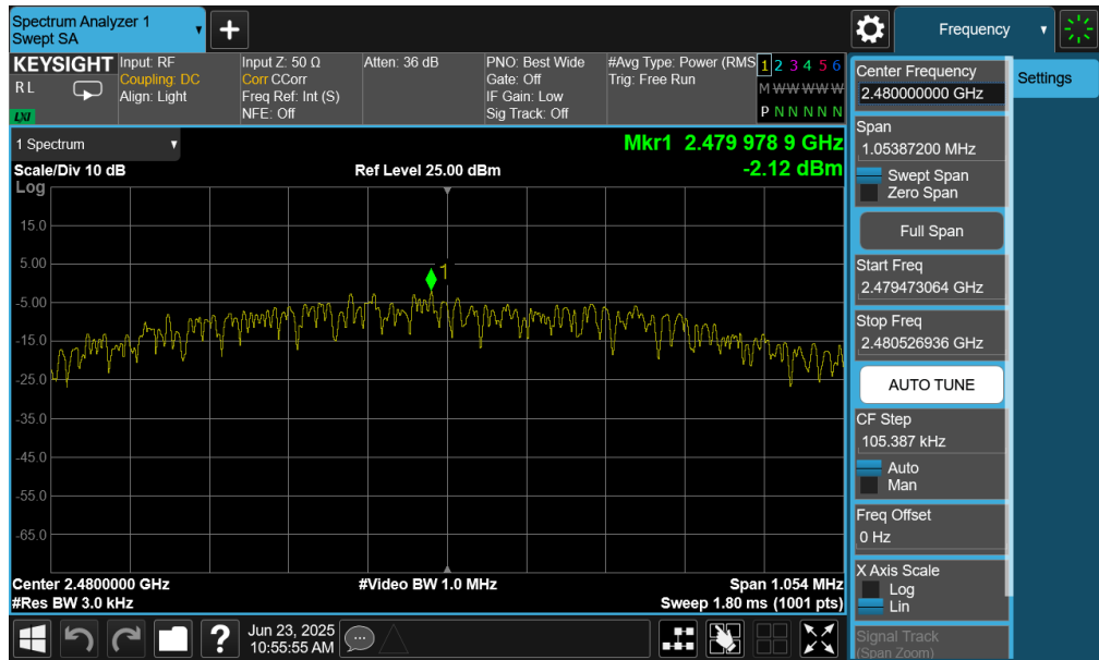
Plot 7-57. Power Spectral Density Plot (Bluetooth (LE), 1Mbps – Ch. 39) – Ant 1
