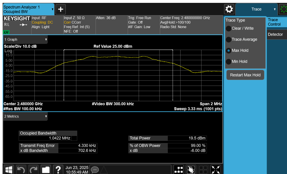
Plot 7-9. 6dB Bandwidth Plot (Bluetooth (LE), 1Mbps – Ch. 39) – Ant 1
