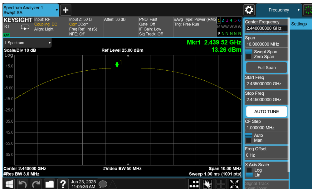
Plot 7-35. Peak Power Plot (Bluetooth (LE), 2Mbps – Ch. 17) – Ant 1
