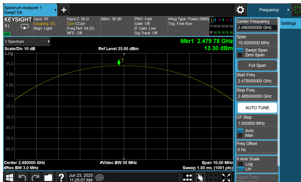
Plot 7-42. Peak Power Plot (Bluetooth (LE), 500kbps – Ch. 39) – Ant 2
