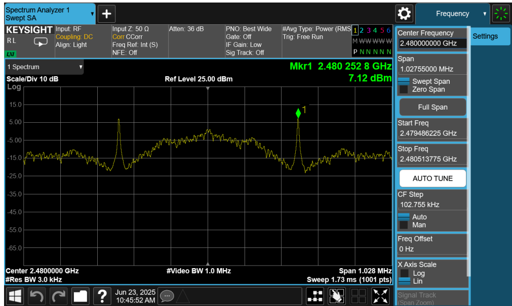
Plot 7-51. Power Spectral Density Plot (Bluetooth (LE), 125kbps – Ch. 39) – Ant 1
