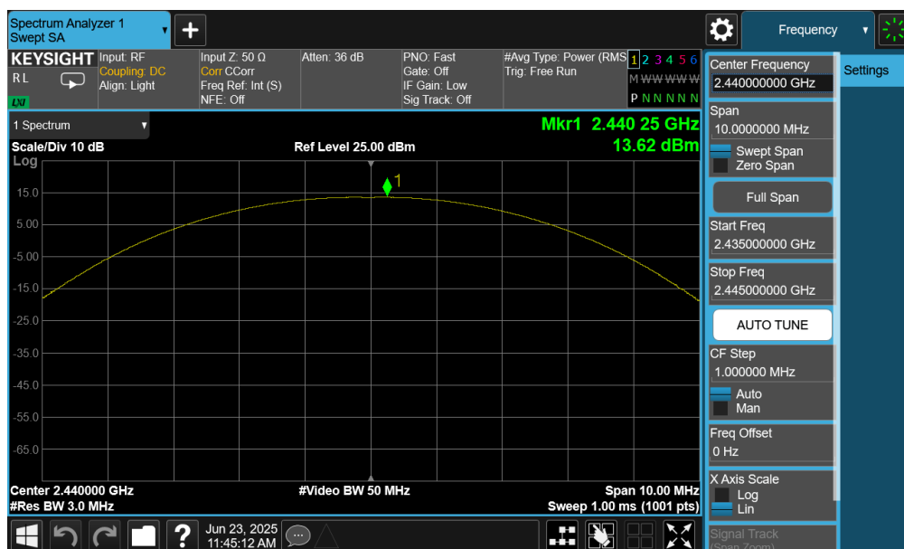
Plot 7-38. Peak Power Plot (Bluetooth (LE), 125kbps – Ch. 17) – Ant 2
