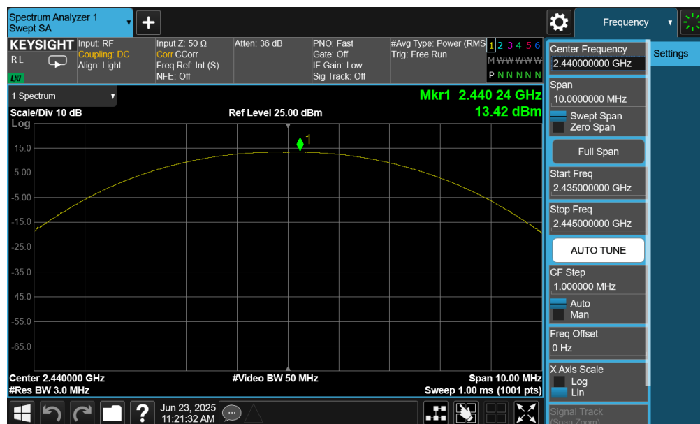
Plot 7-41. Peak Power Plot (Bluetooth (LE), 500kbps – Ch. 17) – Ant 2
