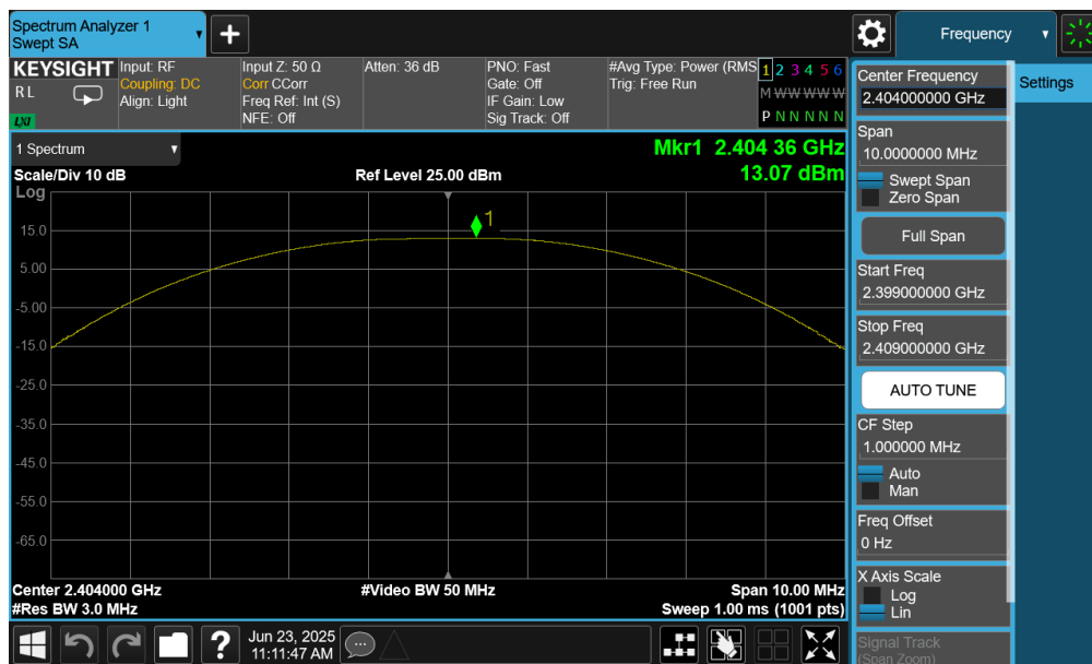
Plot 7-46. Peak Power Plot (Bluetooth (LE), 2Mbps – Ch. 0) – Ant 2
