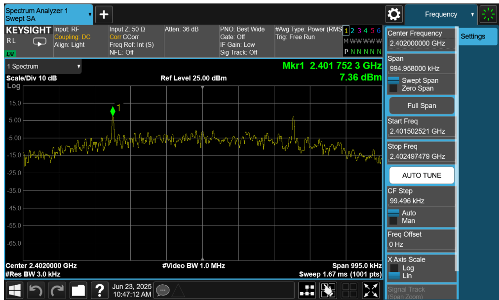
Plot 7-52. Power Spectral Density Plot (Bluetooth (LE), 500kbps – Ch. 37) – Ant 1
