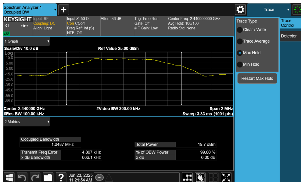
Plot 7-17. 6dB Bandwidth Plot (Bluetooth (LE), 500kbps – Ch. 17) – Ant 2
