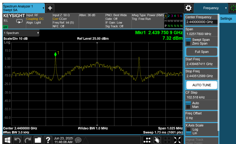
Plot 7-62. Power Spectral Density Plot (Bluetooth (LE), 125kbps – Ch. 17) – Ant 2
