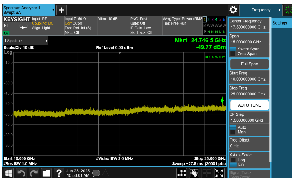
Plot 7-90. Conducted Spurious Plot (Bluetooth (LE), 1Mbps – Ch. 37) – Ant 1
