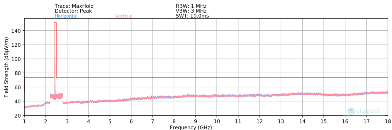
Plot 7-102. Radiated Spurious Plot above 1GHz (Bluetooth (LE) – Ch. 37) – Ant 1
