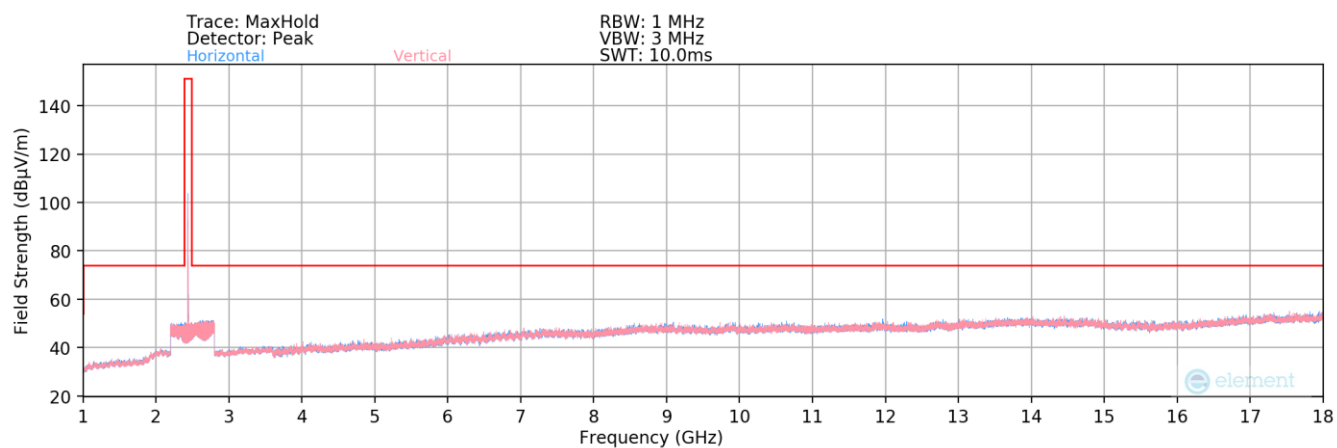
Plot 7-108. Radiated Spurious Plot above 1GHz (Bluetooth (LE) – Ch. 17)
