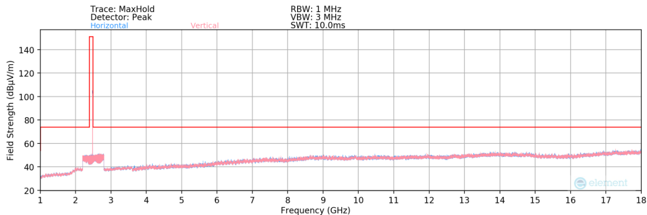
Plot 7-104. Radiated Spurious Plot above 1GHz (Bluetooth (LE) – Ch. 39) – Ant 1
