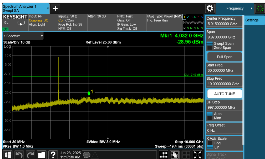
Plot 7-97. Conducted Spurious Plot (Bluetooth (LE), 1Mbps – Ch. 17) – Ant 2
