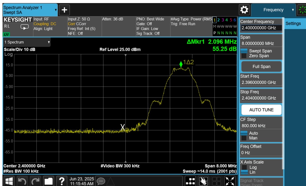
Plot 7-85. Band Edge Plot (Bluetooth (LE), 1Mbps – Ch. 37) – Ant 2
