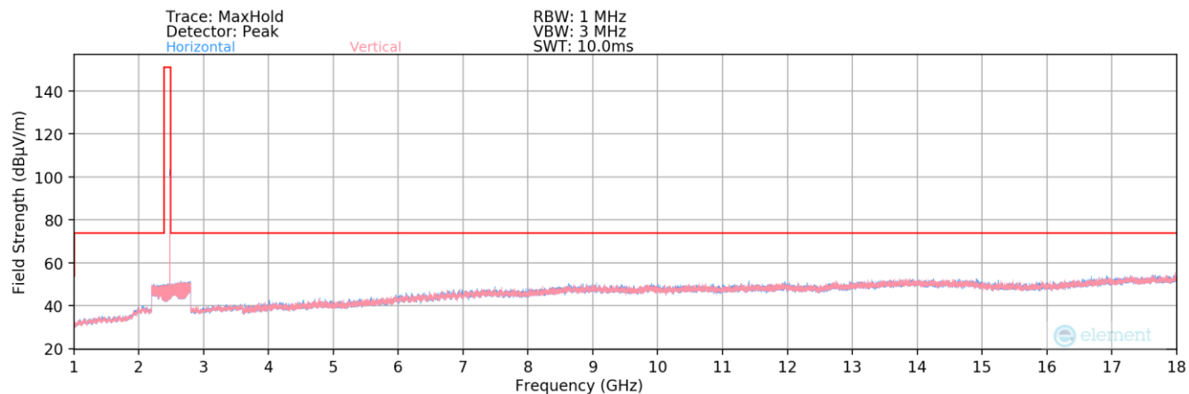
Plot 7-109. Radiated Spurious Plot above 1GHz (Bluetooth (LE) – Ch. 39)
