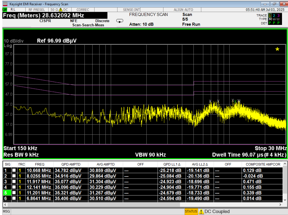
Plot 7-115. Line Conducted Plot with Bluetooth LE (L1)
