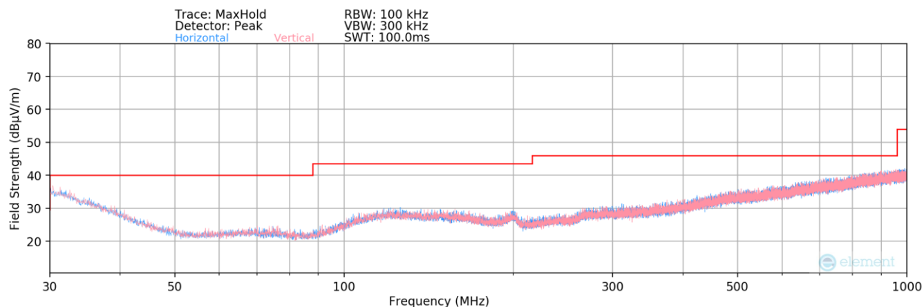
Plot 7-101. Radiated Spurious Plot below 1GHz (Bluetooth (LE) – Ch. 17) – Ant 1
