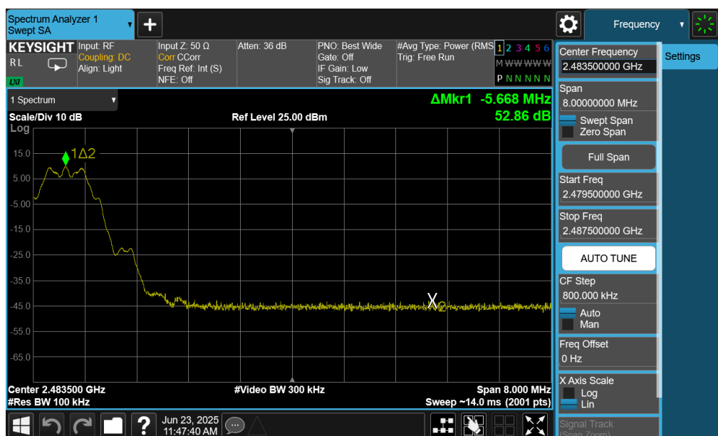
Plot 7-82. Band Edge Plot (Bluetooth (LE), 125kbps – Ch. 39) – Ant 2
