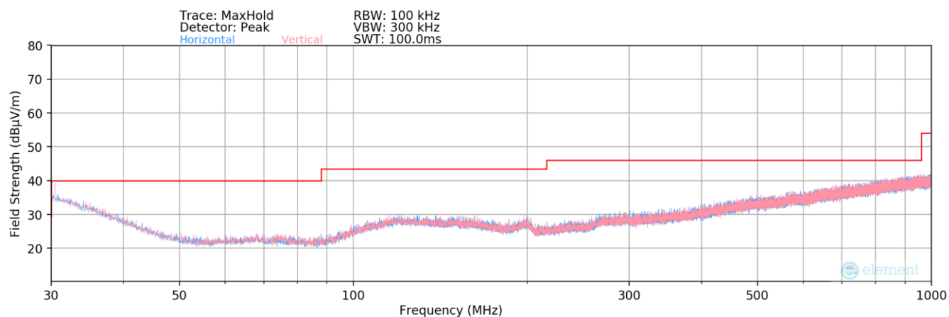
Plot 7-106. Radiated Spurious Plot below 1GHz (Bluetooth (LE) – Ch. 17)
