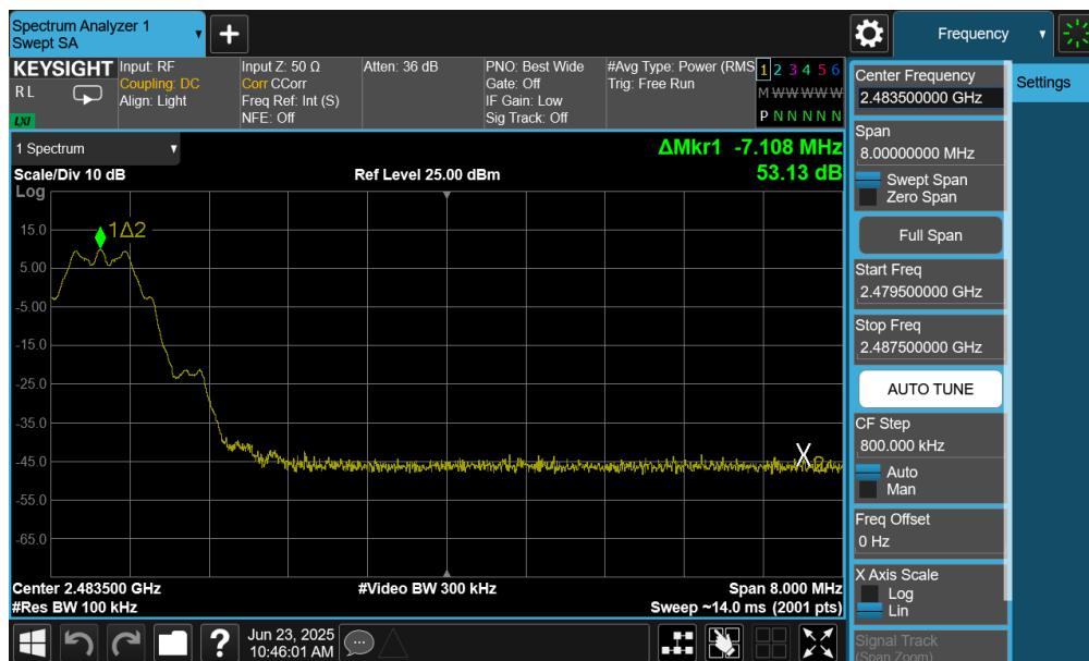
Plot 7-74. Band Edge Plot (Bluetooth (LE), 125kbps – Ch. 39) – Ant 1
