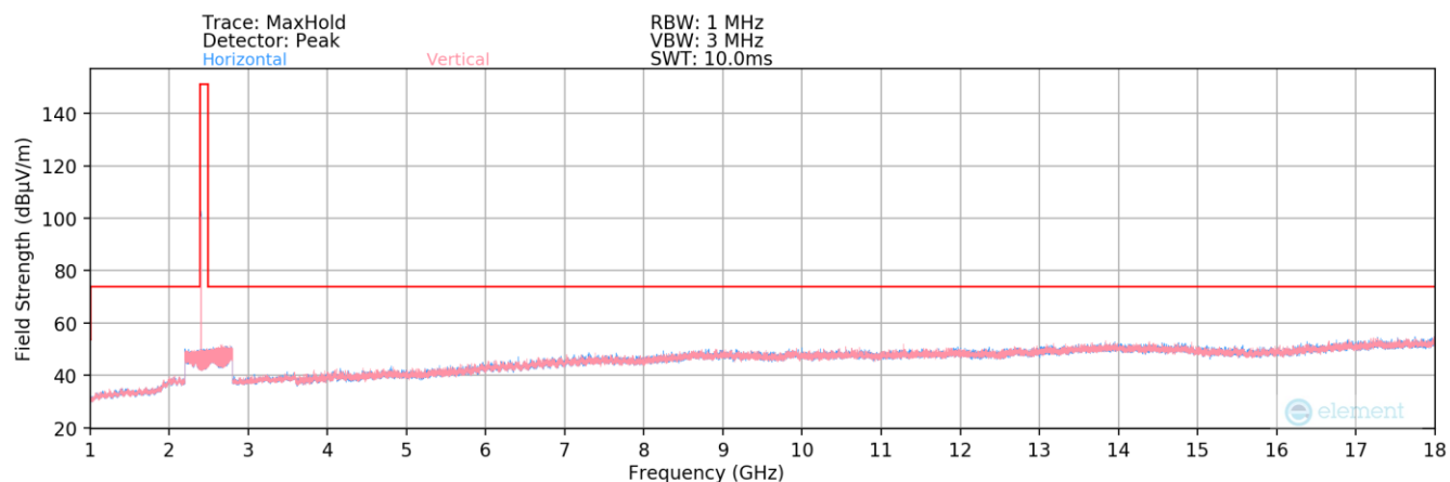
Plot 7-107. Radiated Spurious Plot above 1GHz (Bluetooth (LE) – Ch. 37)
