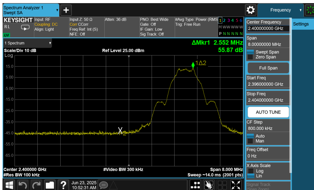
Plot 7-77. Band Edge Plot (Bluetooth (LE), 1Mbps – Ch. 37) – Ant 1
