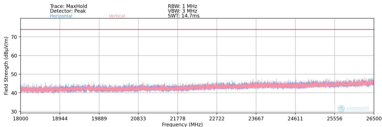
Plot 7-105. Radiated Spurious Plot above 18GHz (Bluetooth (LE) – Ch. 17) – Ant 1
