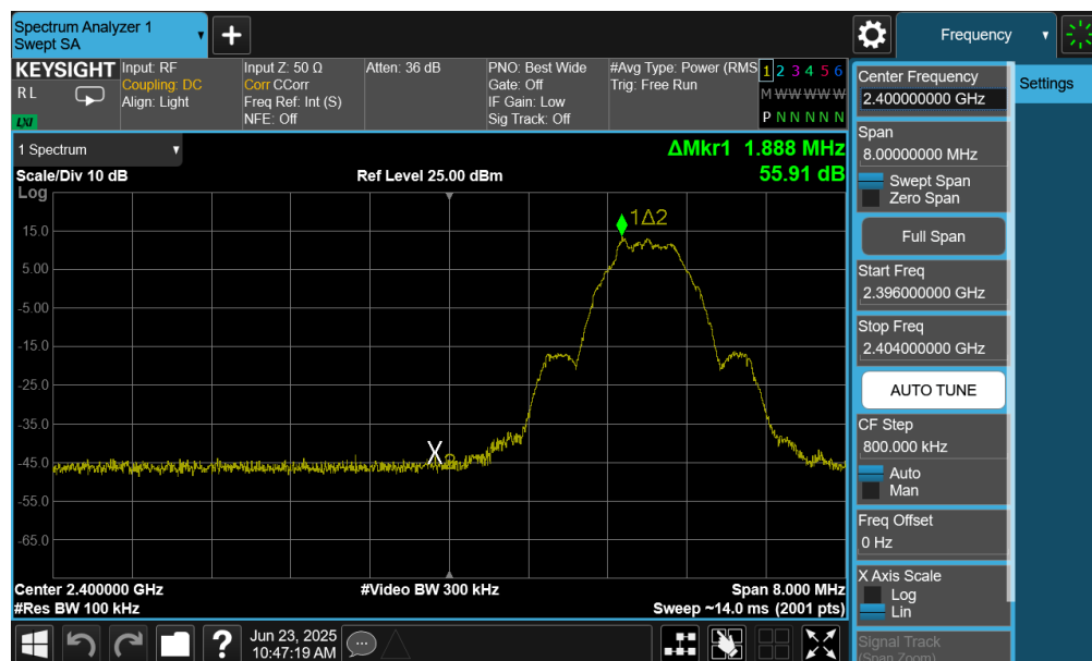
Plot 7-75. Band Edge Plot (Bluetooth (LE), 500kbps – Ch. 37) – Ant 1
