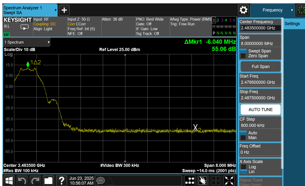
Plot 7-78. Band Edge Plot (Bluetooth (LE), 1Mbps – Ch. 39) – Ant 1
