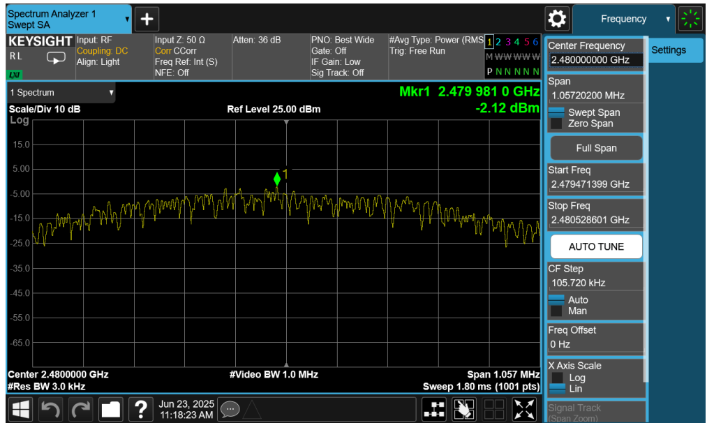
Plot 7-69. Power Spectral Density Plot (Bluetooth (LE), 1Mbps – Ch. 39) – Ant 2
