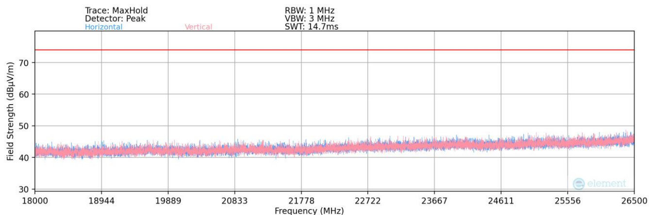
Plot 7-110. Radiated Spurious Plot above 18GHz (Bluetooth (LE) – Ch. 17)
