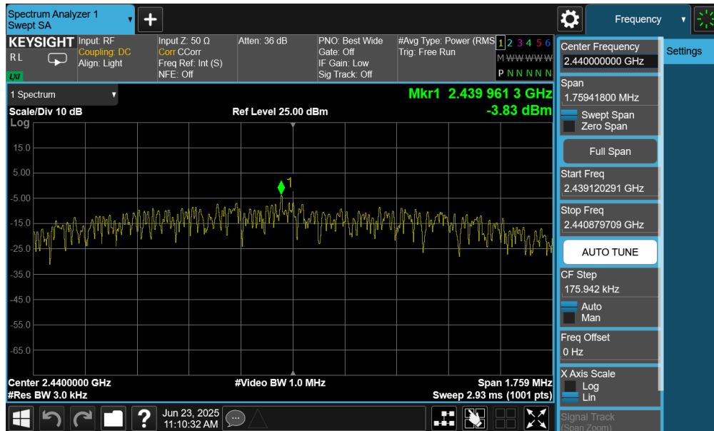
Plot 7-71. Power Spectral Density Plot (Bluetooth (LE), 2Mbps – Ch. 17) – Ant 2
