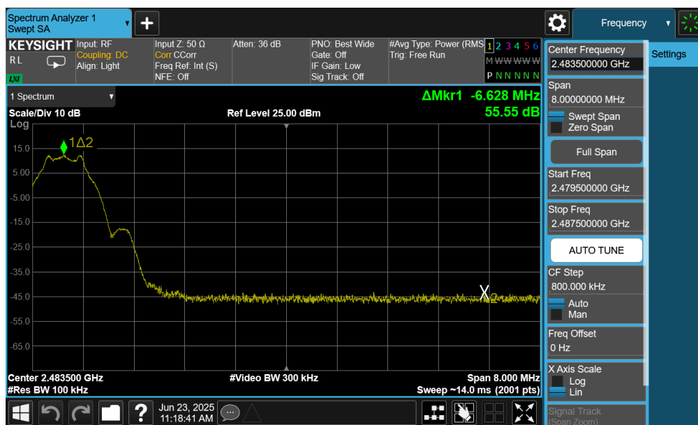
Plot 7-86. Band Edge Plot (Bluetooth (LE), 1Mbps – Ch. 39) – Ant 2
