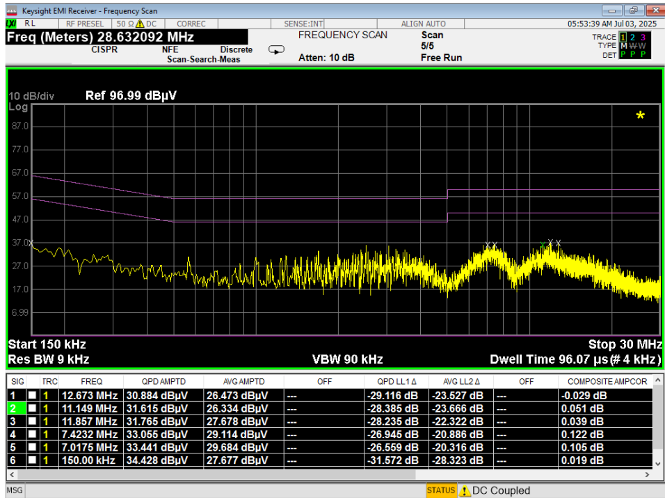
Plot 7-116. Line Conducted Plot with Bluetooth LE (N)
