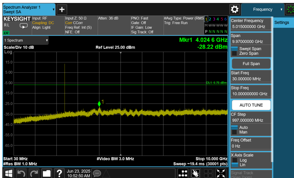
Plot 7-89. Conducted Spurious Plot (Bluetooth (LE), 1Mbps – Ch. 37) – Ant 1
