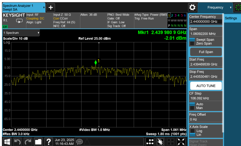
Plot 7-68. Power Spectral Density Plot (Bluetooth (LE), 1Mbps – Ch. 17) – Ant 2
