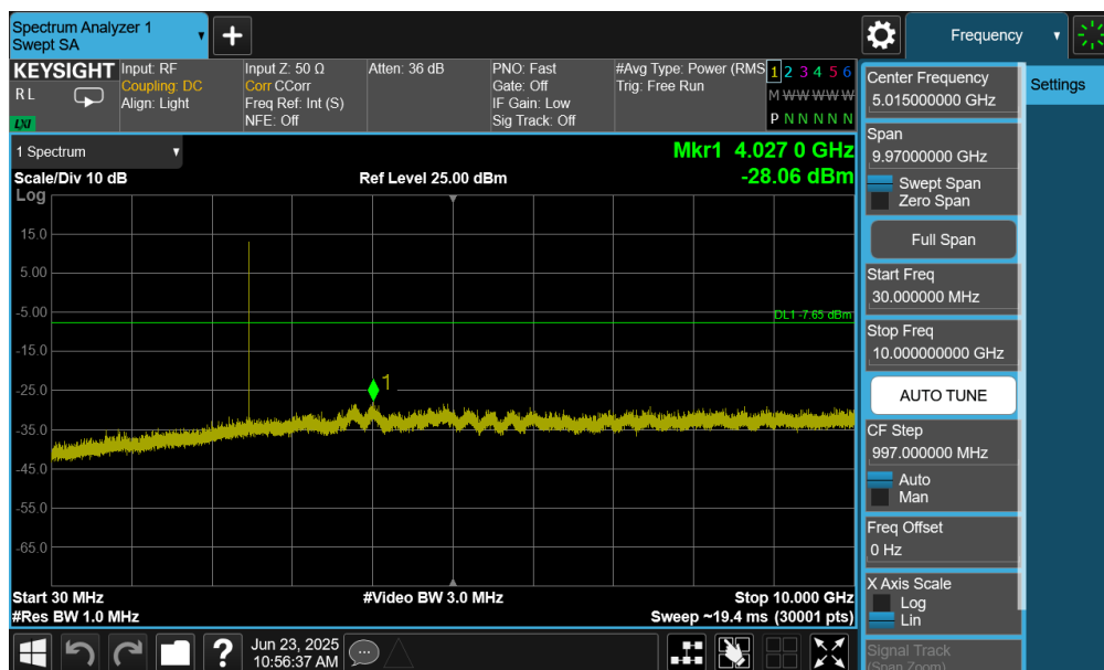
Plot 7-93. Conducted Spurious Plot (Bluetooth (LE), 1Mbps – Ch. 39) – Ant 1
