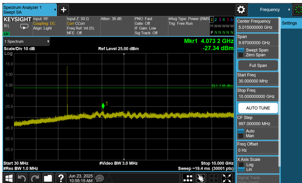
Plot 7-91. Conducted Spurious Plot (Bluetooth (LE), 1Mbps – Ch. 17) – Ant 1
