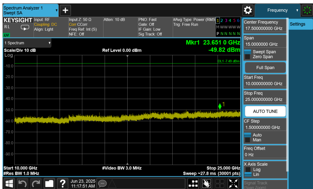
Plot 7-98. Conducted Spurious Plot (Bluetooth (LE), 1Mbps – Ch. 17) – Ant 2
