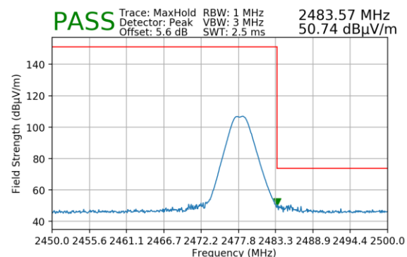
Plot 7-114. Radiated Restricted Upper Band Edge Measurement (Peak) – Ant 2
