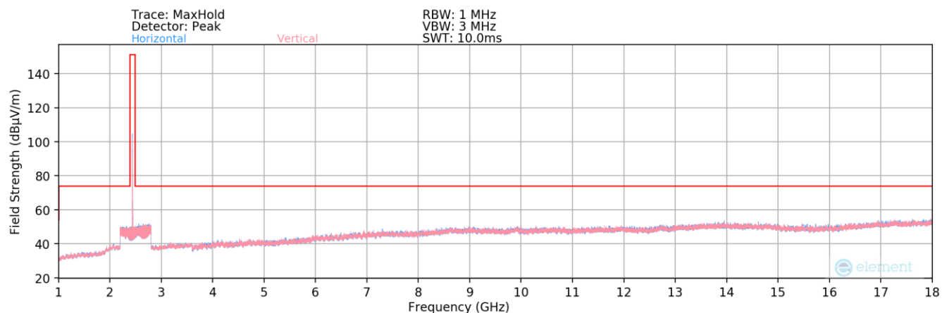
Plot 7-103. Radiated Spurious Plot above 1GHz (Bluetooth (LE) – Ch. 17) – Ant 1
