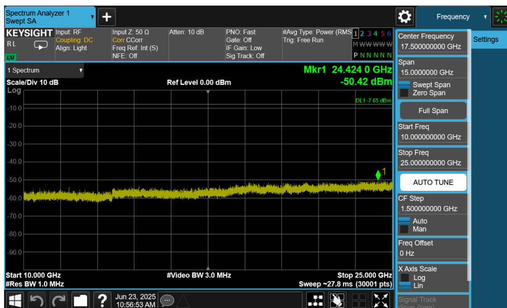
Plot 7-94. Conducted Spurious Plot (Bluetooth (LE), 1Mbps – Ch. 39) – Ant 1
