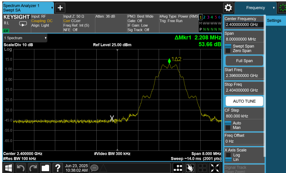
Plot 7-73. Band Edge Plot (Bluetooth (LE), 125kbps – Ch. 37) – Ant 1
