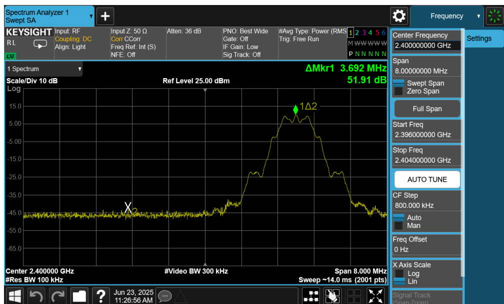
Plot 7-81. Band Edge Plot (Bluetooth (LE), 125kbps – Ch. 37) – Ant 2
