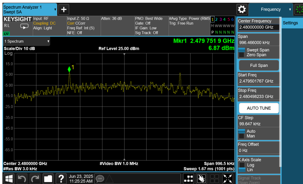
Plot 7-66. Power Spectral Density Plot (Bluetooth (LE), 500kbps – Ch. 39) – Ant 2
