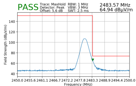
Plot 7-112. Radiated Restricted Upper Band Edge Measurement (Peak) – Ant 1
