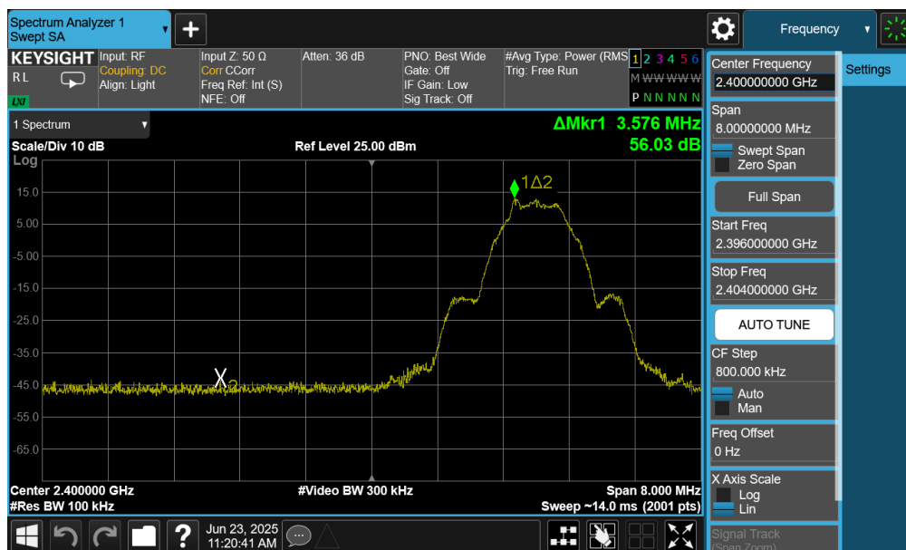
Plot 7-83. Band Edge Plot (Bluetooth (LE), 500kbps – Ch. 37) – Ant 2
