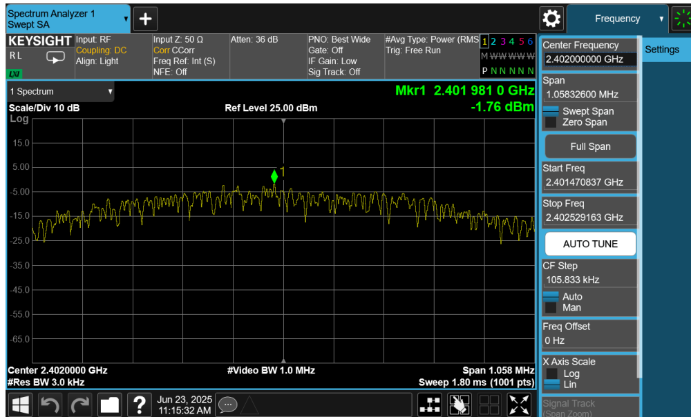
Plot 7-67. Power Spectral Density Plot (Bluetooth (LE), 1Mbps – Ch. 37) – Ant 2
