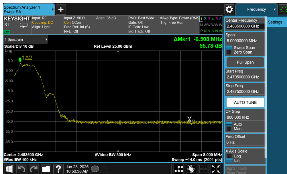
Plot 7-76. Band Edge Plot (Bluetooth (LE), 500kbps – Ch. 39) – Ant 1
