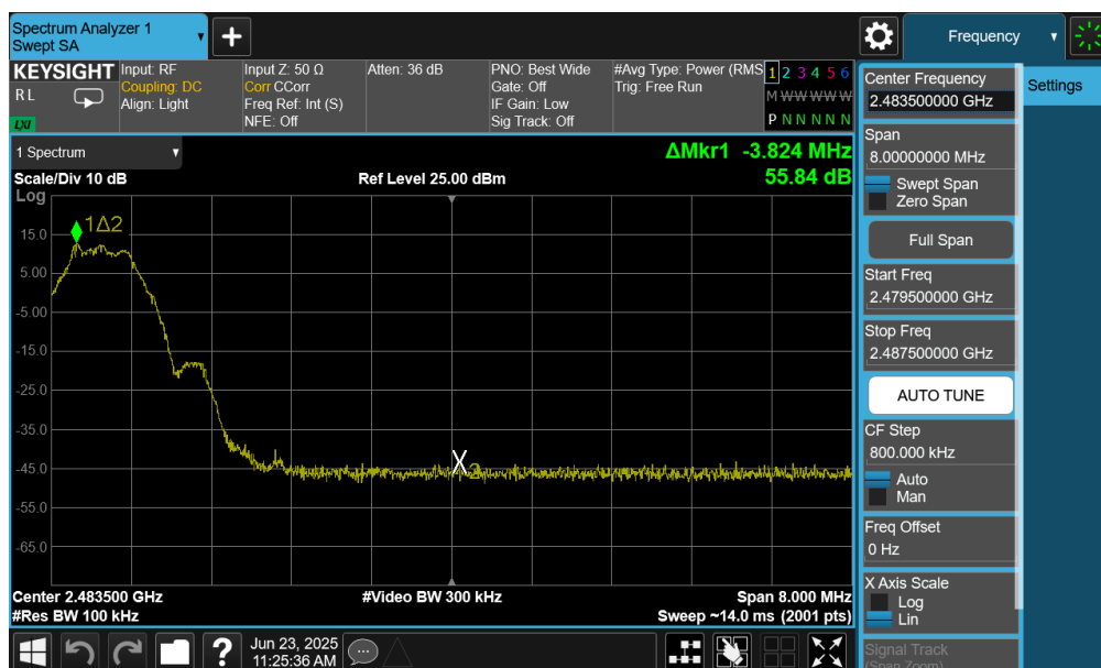
Plot 7-84. Band Edge Plot (Bluetooth (LE), 500kbps – Ch. 39) – Ant 2
