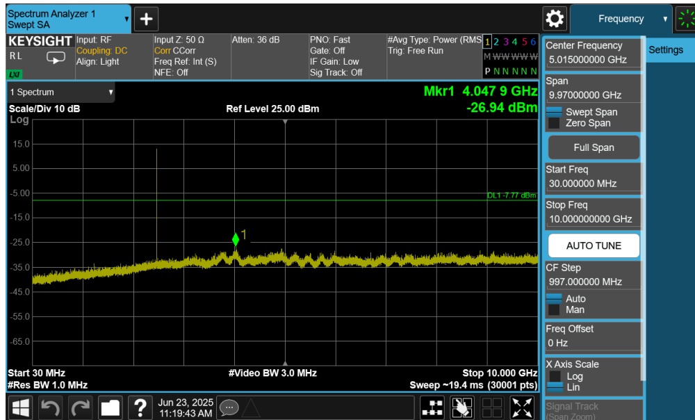
Plot 7-99. Conducted Spurious Plot (Bluetooth (LE), 1Mbps – Ch. 39) – Ant 2
