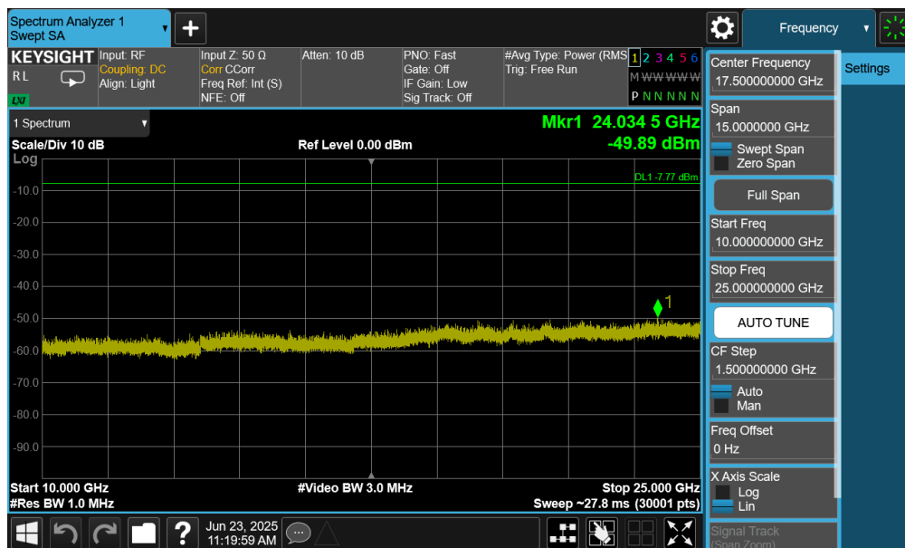
Plot 7-100. Conducted Spurious Plot (Bluetooth (LE), 1Mbps – Ch. 39) – Ant 2
