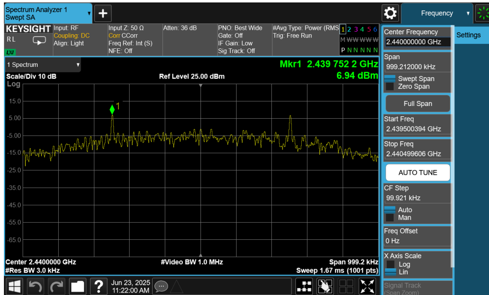
Plot 7-65. Power Spectral Density Plot (Bluetooth (LE), 500kbps – Ch. 17) – Ant 2
