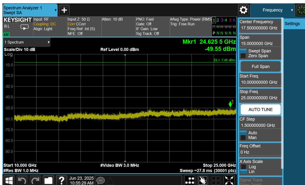
Plot 7-92. Conducted Spurious Plot (Bluetooth (LE), 1Mbps – Ch. 17) – Ant 1
