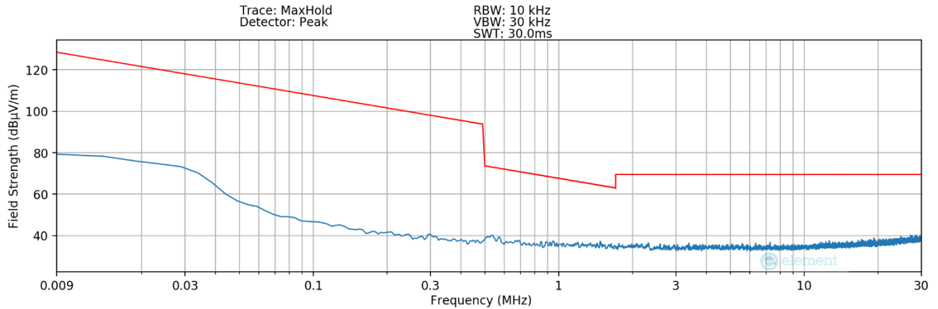
Plot 7-5. Radiated Spurious Plot 9kHz – 30MHz (Pol. X – Click)
