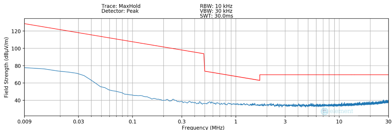
Plot 7-10. Radiated Spurious Plot 9kHz – 30MHz (Pol. Z– Hover)
