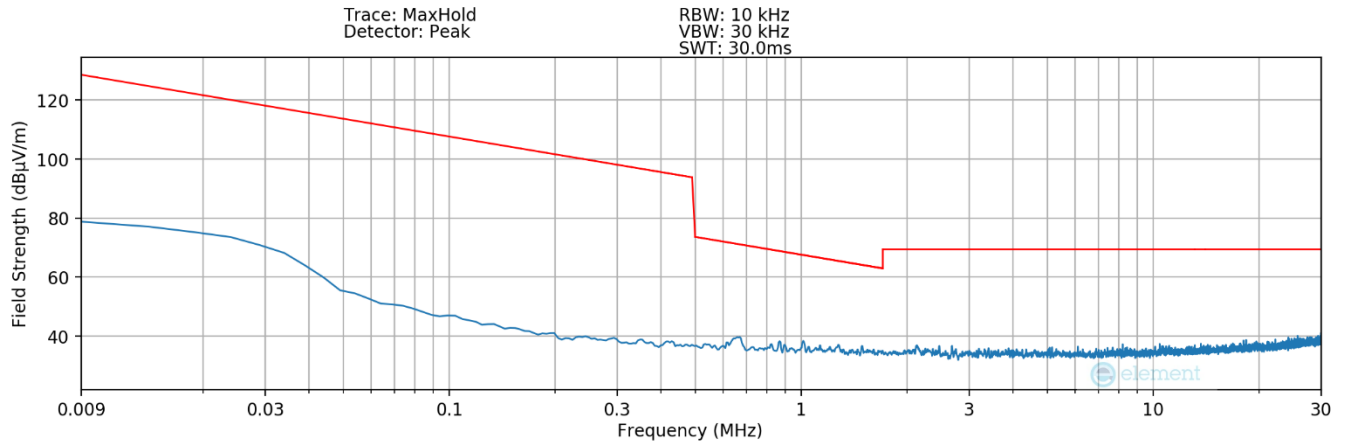
Plot 7-14. Radiated Spurious Plot 9kHz – 30MHz (Pol. X – Keyboard Detection)
