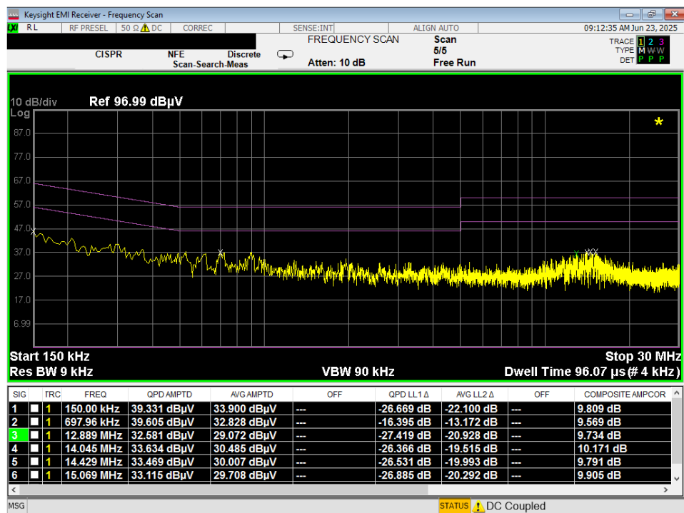
Plot 7-21. Line-Conducted Test Plot (L1) – Eraser
