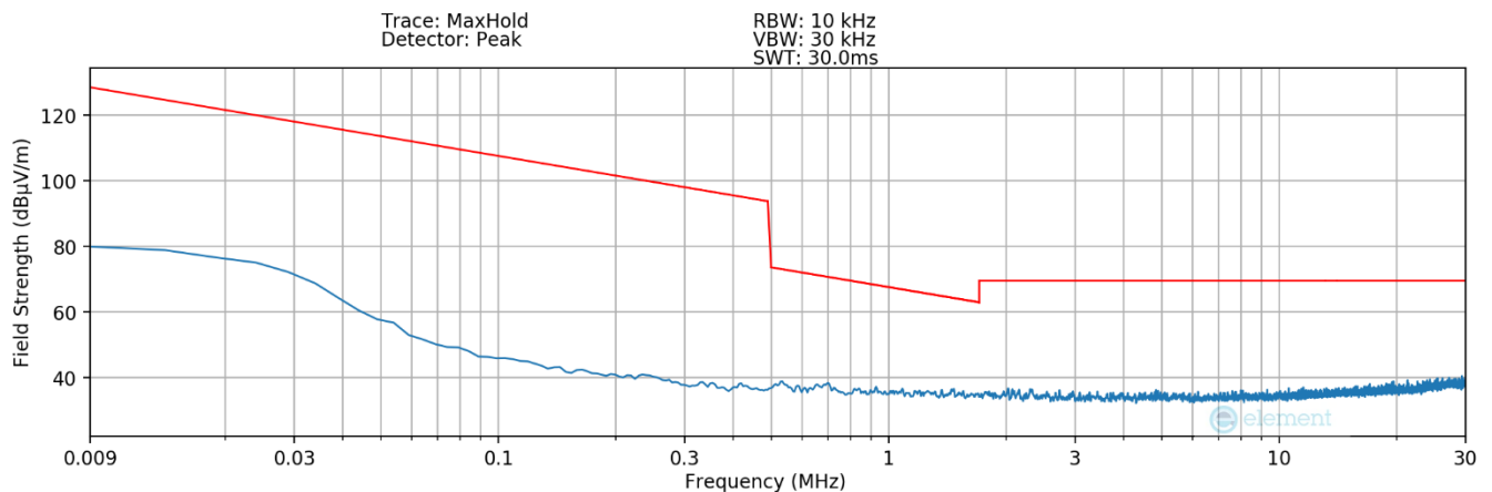
Plot 7-7. Radiated Spurious Plot 9kHz – 30MHz (Pol. Z– Click)
