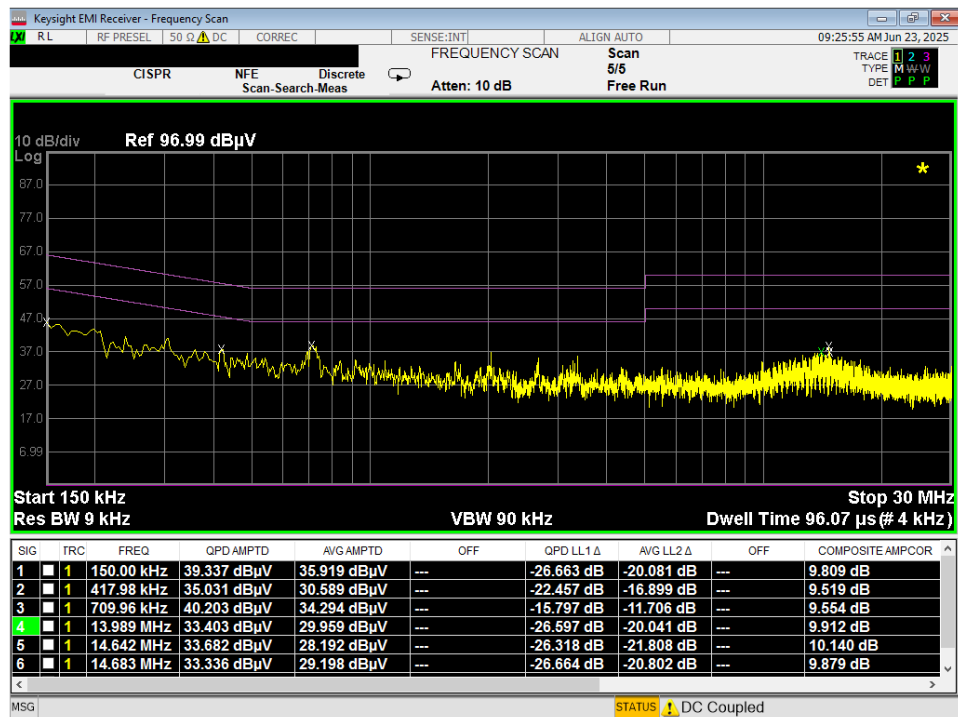
Plot 7-23. Line-Conducted Test Plot (L1) – Keyboard
