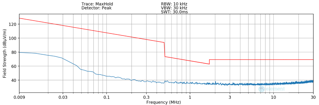
Plot 7-6Radiated Spurious Plot 9kHz – 30MHz (Pol. Y – Click)
