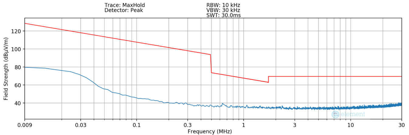
Plot 7-15Radiated Spurious Plot 9kHz – 30MHz (Pol. Y – Keyboard Detection)
