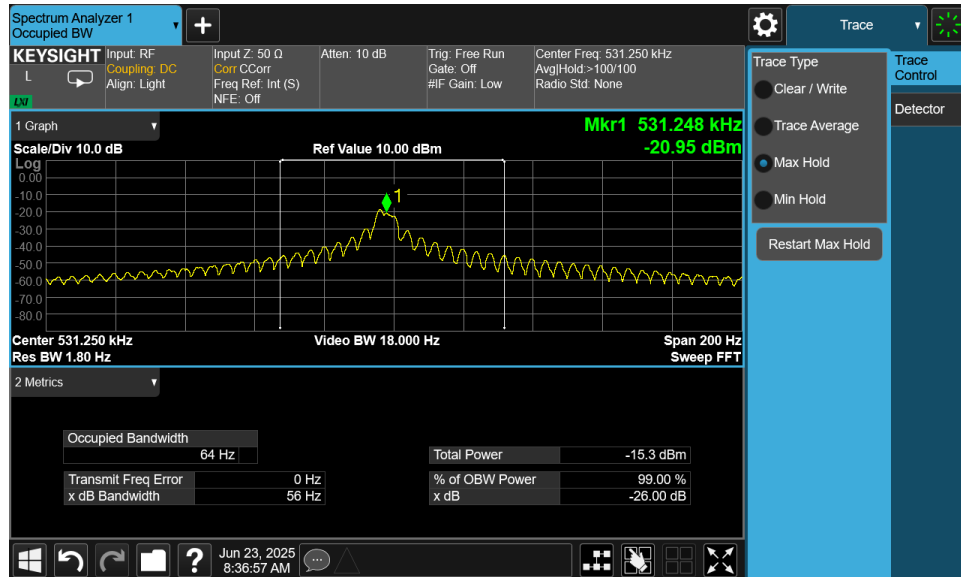
Plot 7-1. Occupied Bandwidth Measurement – Click
