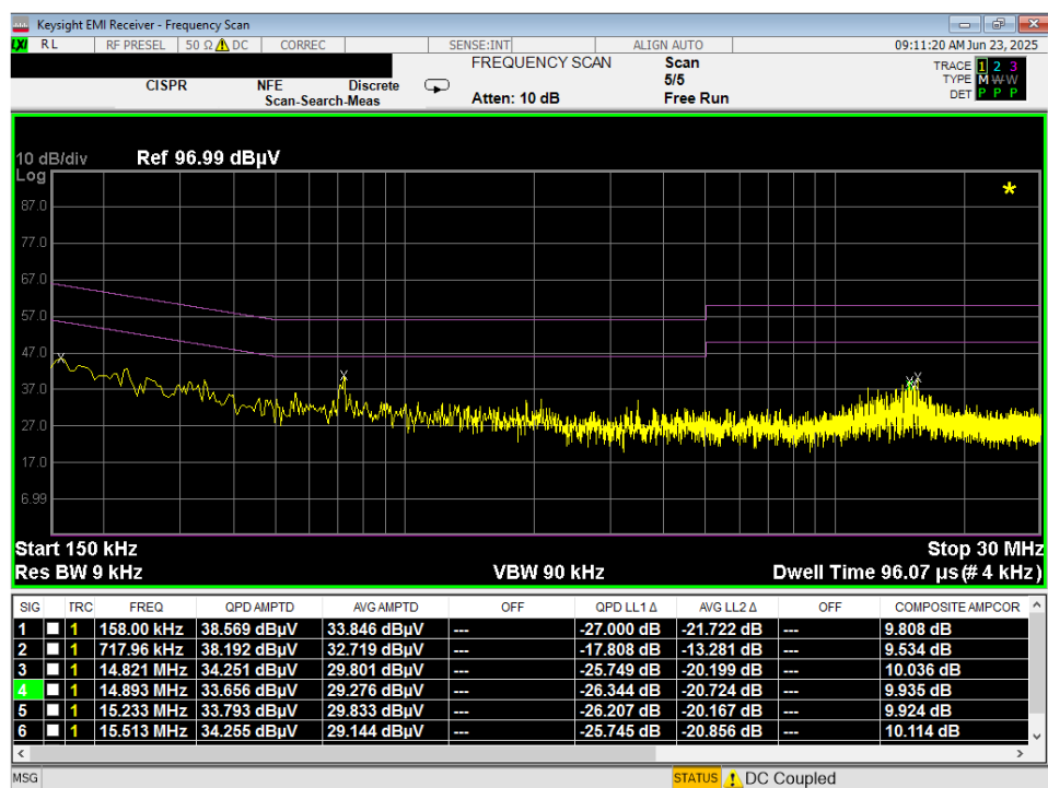
Plot 7-22. Line-Conducted Test Plot (N) – Eraser
