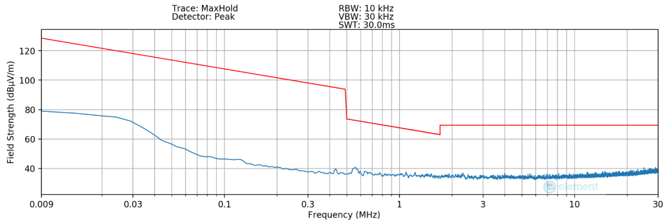
Plot 7-8. Radiated Spurious Plot 9kHz – 30MHz (Pol. X – Hover)
