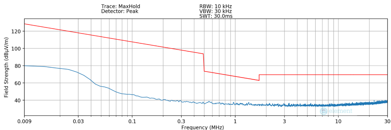
Plot 7-9Radiated Spurious Plot 9kHz – 30MHz (Pol. Y – Hover)
