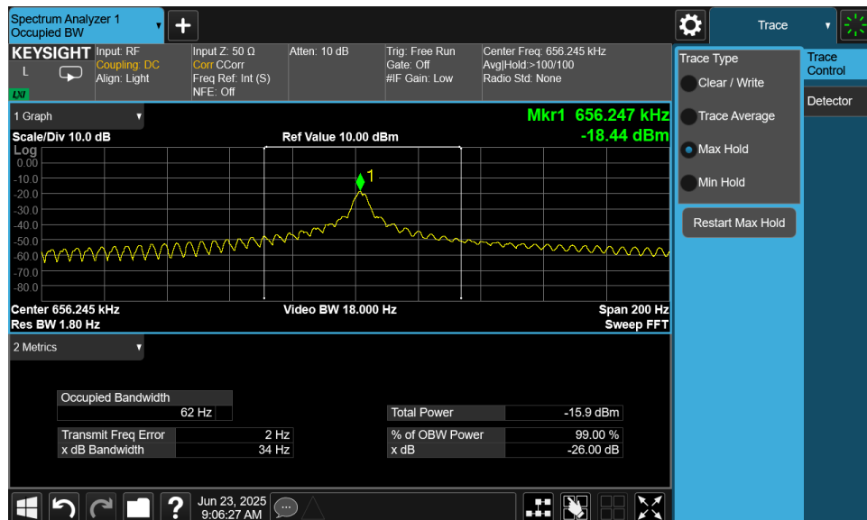
Plot 7-4. Occupied Bandwidth Measurement – Keyboard Detection
