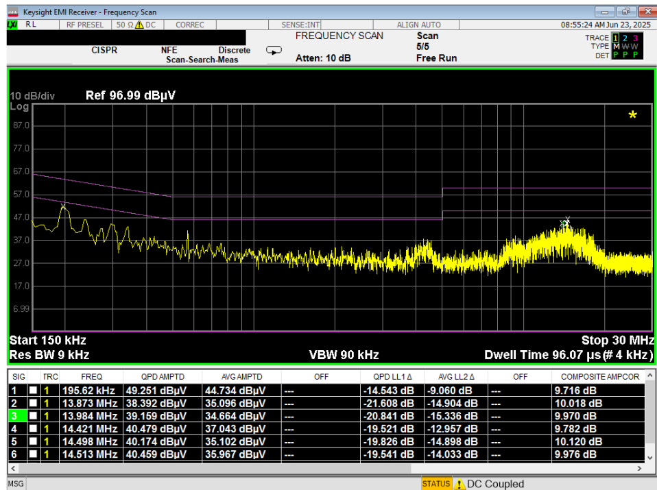
Plot 7-18. Line-Conducted Test Plot (N) – Click
