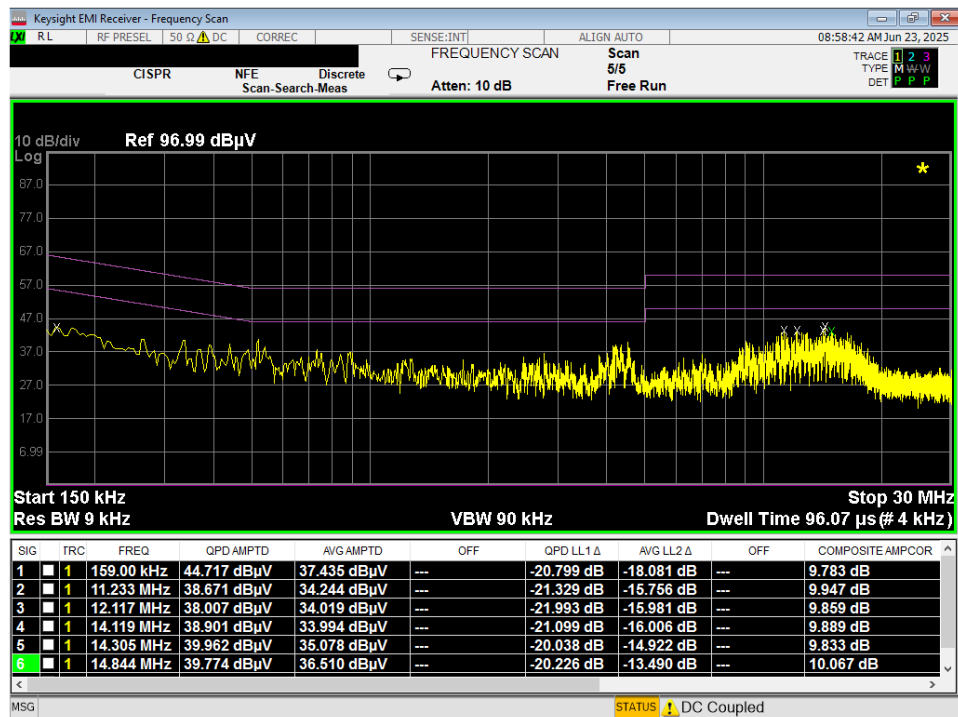
Plot 7-17. Line-Conducted Test Plot (L1) – Click
