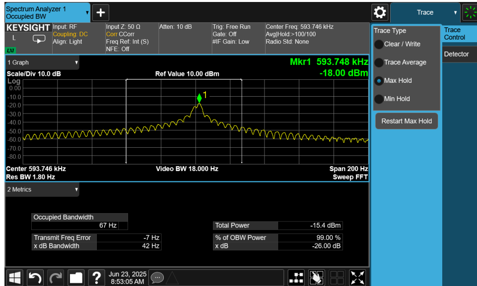
Plot 7-3. Occupied Bandwidth Measurement – Eraser
