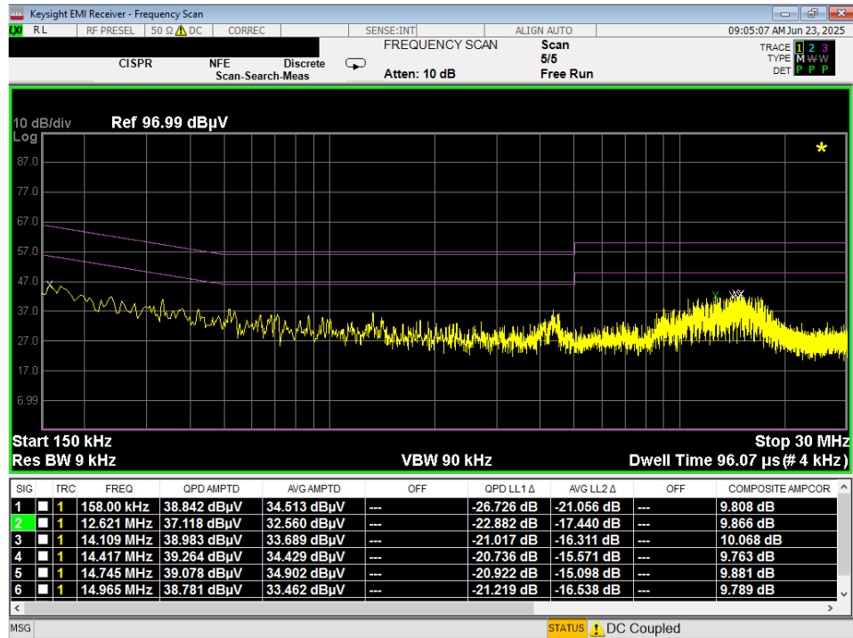
Plot 7-20. Line-Conducted Test Plot (N) – Hover
