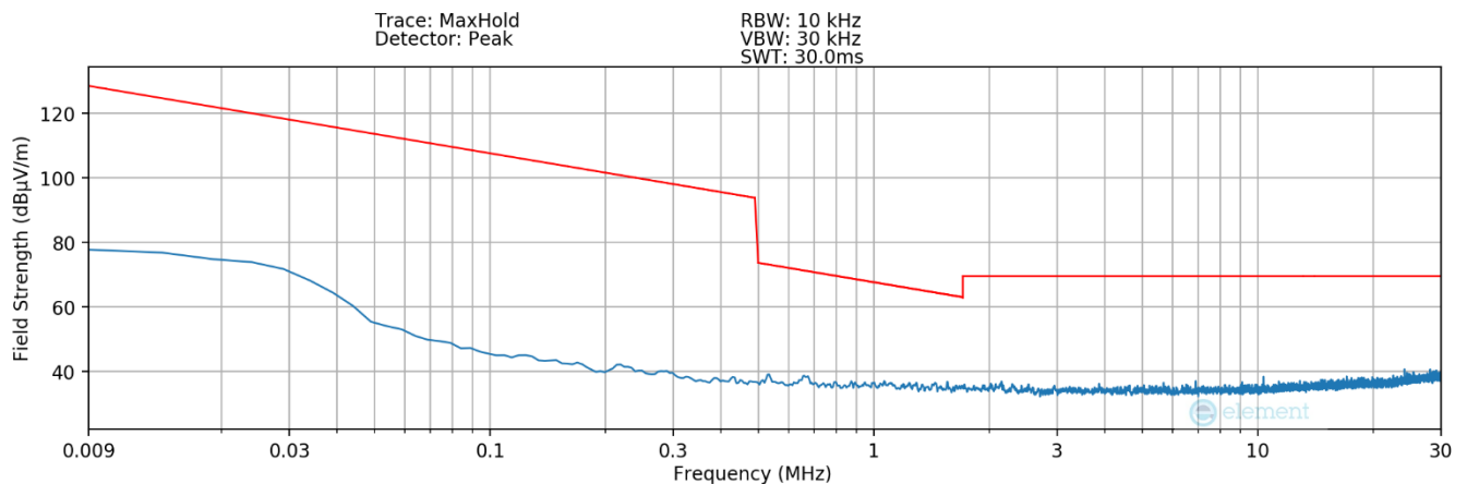
Plot 7-16. Radiated Spurious Plot 9kHz – 30MHz (Pol. Z– Keyboard Detection)
