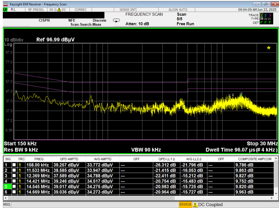
Plot 7-19. Line-Conducted Test Plot (L1) – Hover
