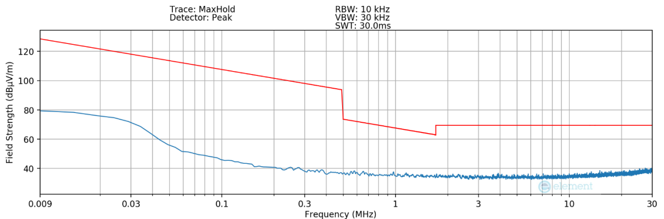
Plot 7-13. Radiated Spurious Plot 9kHz – 30MHz (Pol. Z – Eraser)
