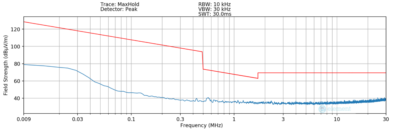
Plot 7-11. Radiated Spurious Plot 9kHz – 30MHz (Pol. X – Eraser)
