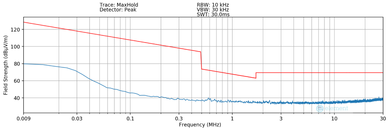
Plot 7-12 Radiated Spurious Plot 9kHz – 30MHz (Pol. Y – Eraser)
