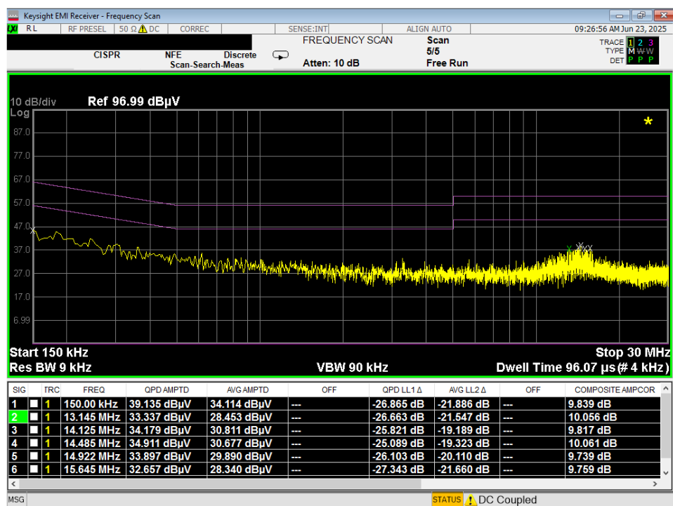
Plot 7-24. Line-Conducted Test Plot (N) – Keyboard
