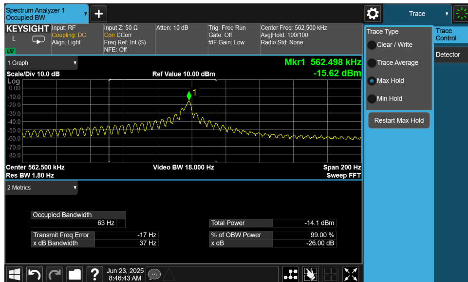
Plot 7-2. Occupied Bandwidth Measurement – Hover
