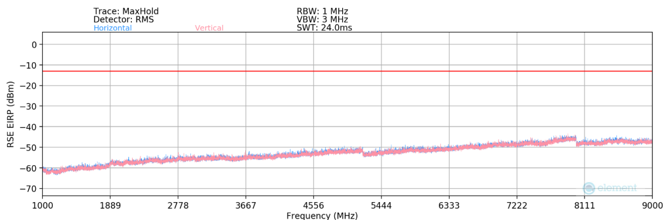
Plot 7-23. Radiated Spurious Plot (LTE Band 26)
