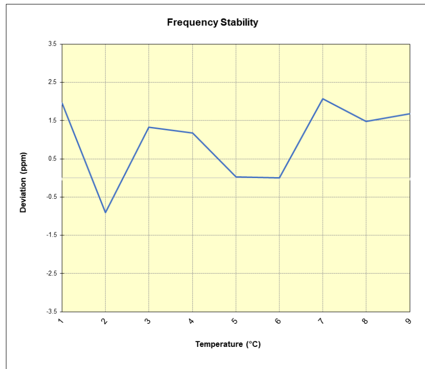
Plot 7-24. LTE Band 26 Frequency Stability Chart
