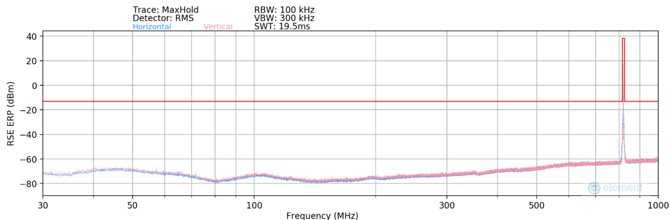
Plot 7-22. Radiated Spurious Plot (LTE Band 26)
