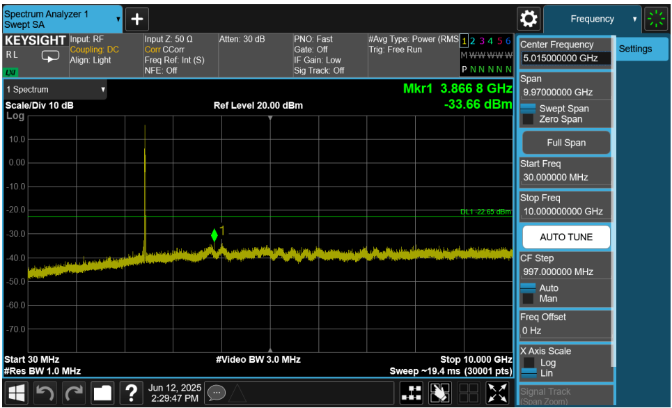
Plot 7-43. Conducted Spurious Plot MIMO ANT1 (802.11ax OFDMA – 26 Tones – Ch. 6)
