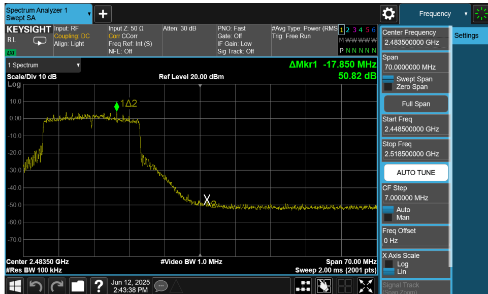
Plot 7-38. Band Edge Plot MIMO ANT2 (802.11ax OFDMA – 242 Tones – Ch. 11)
