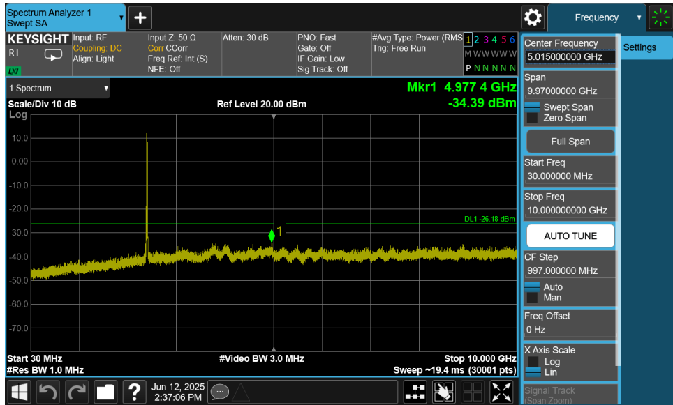
Plot 7-47. Conducted Spurious Plot MIMO ANT1 (802.11ax OFDMA – 242 Tones – Ch. 1)
