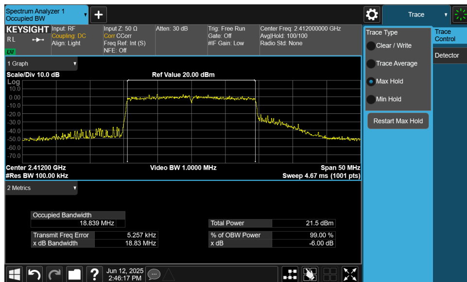
Plot 7-10. 6dB Bandwidth Plot MIMO ANT2 (802.11ax OFDMA – 242 Tones – Ch. 1)
