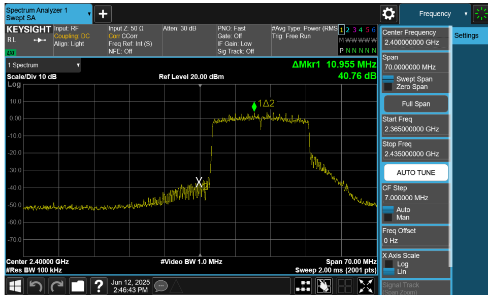
Plot 7-37. Band Edge Plot MIMO ANT2 (802.11ax OFDMA – 242 Tones – Ch. 1)
