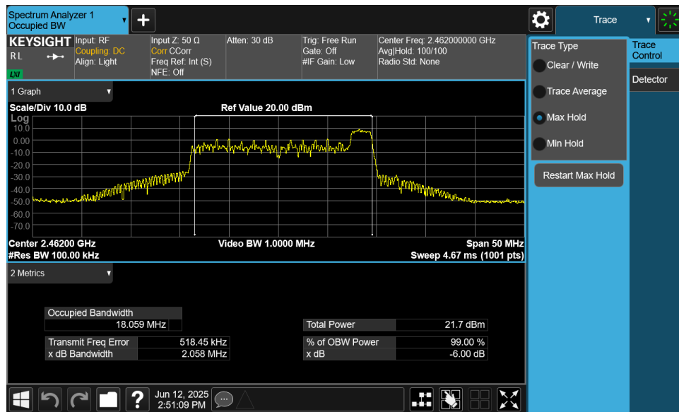
Plot 7-9. 6dB Bandwidth Plot MIMO ANT2 (802.11ax OFDMA – 26 Tones – Ch. 11)
