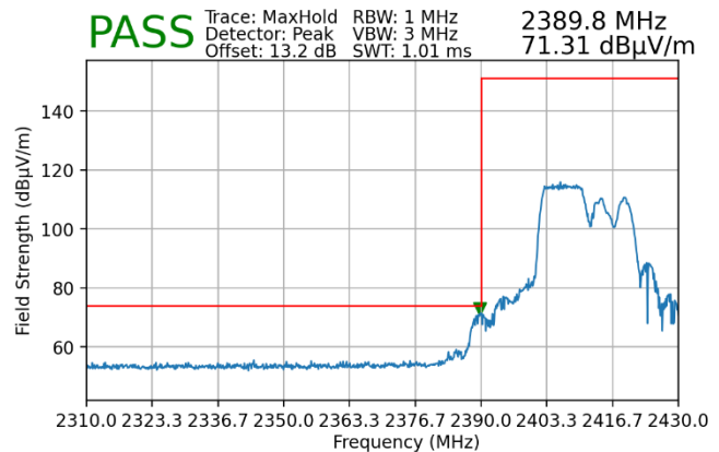
Plot 7-74. Radiated Restricted Lower Band Edge Measurement MIMO (Peak – 106 Tones)
