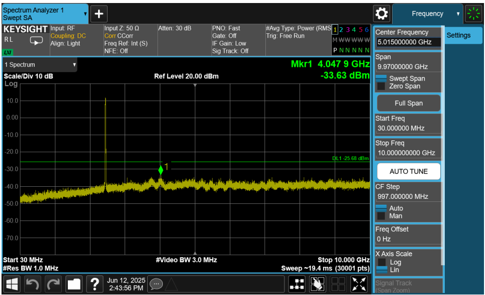
Plot 7-63. Conducted Spurious Plot MIMO ANT2 (802.11ax OFDMA – 242 Tones – Ch. 11)
