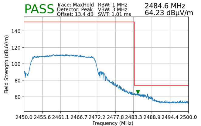
Plot 7-84. Radiated Restricted Upper Band Edge Measurement MIMO (Peak – 242 Tones)
