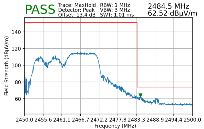
Plot 7-76. Radiated Restricted Upper Band Edge Measurement MIMO (Peak – 106 Tones)
