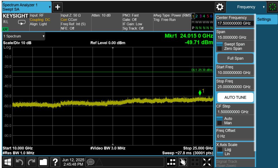
Plot 7-62. Conducted Spurious Plot MIMO ANT2 (802.11ax OFDMA – 242 Tones – Ch. 6)
