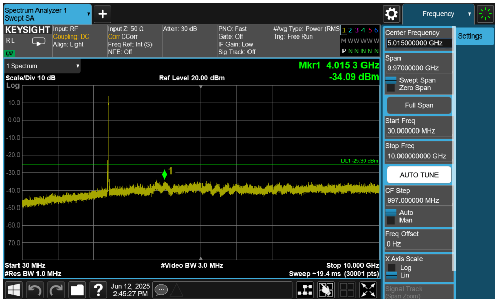
Plot 7-61. Conducted Spurious Plot MIMO ANT2 (802.11ax OFDMA – 242 Tones – Ch. 6)
