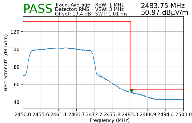
Plot 7-83. Radiated Restricted Upper Band Edge Measurement MIMO (Average – 242 Tones)
