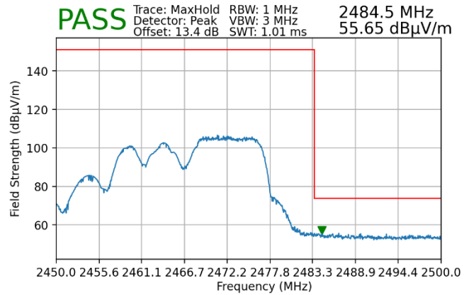
Plot 7-78. Radiated Restricted Upper Band Edge Measurement MIMO (Peak – 106 Tones)
