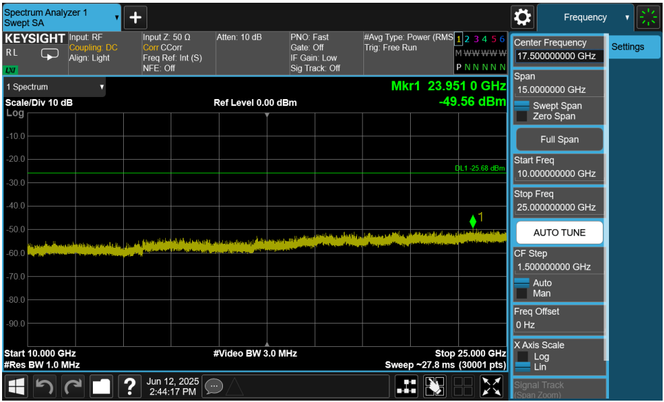
Plot 7-64. Conducted Spurious Plot MIMO ANT2 (802.11ax OFDMA – 242 Tones – Ch. 11)
