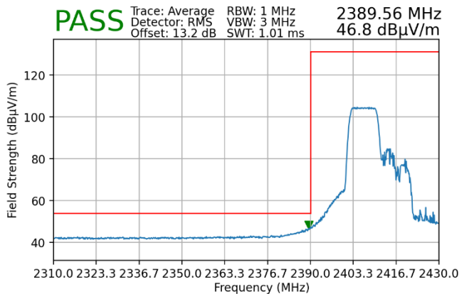
Plot 7-73. Radiated Restricted Lower Band Edge Measurement MIMO (Average – 106 Tones)
