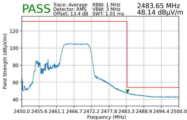
Plot 7-75. Radiated Restricted Upper Band Edge Measurement MIMO (Average – 106 Tones)
