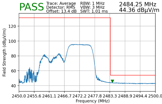
Plot 7-77. Radiated Restricted Upper Band Edge Measurement MIMO (Average – 106 Tones)
