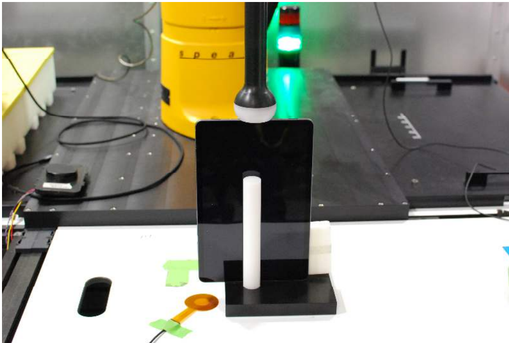
Test Setup Photo 4 Digitizer, Bottom Side, 0mm
