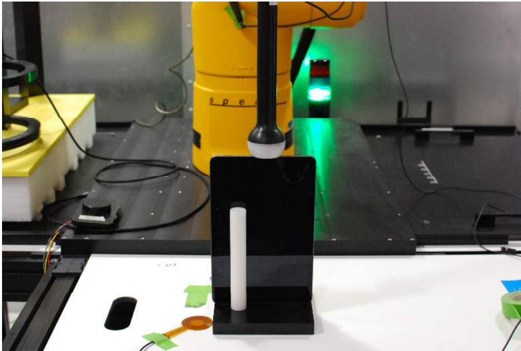
Test Setup Photo 3 Digitizer, Top Side, 0mm
