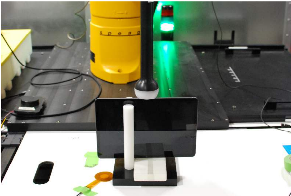
Test Setup Photo 6 Digitizer, Left Side, 0mm
