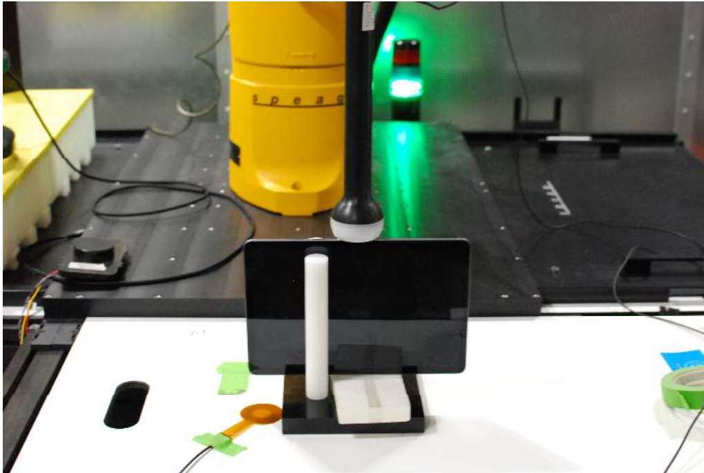
Test Setup Photo 5 Digitizer, Right Side, 0mm
