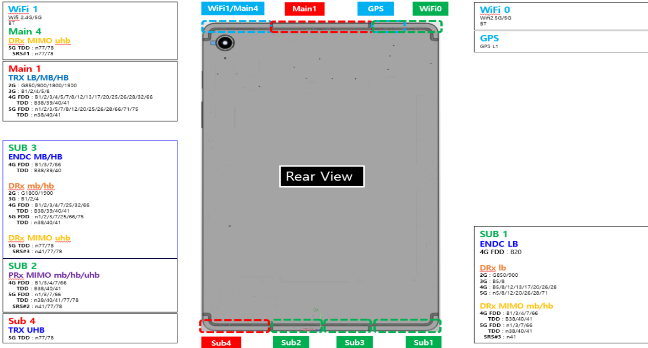
Photograph 11. Antenna position of EUT
