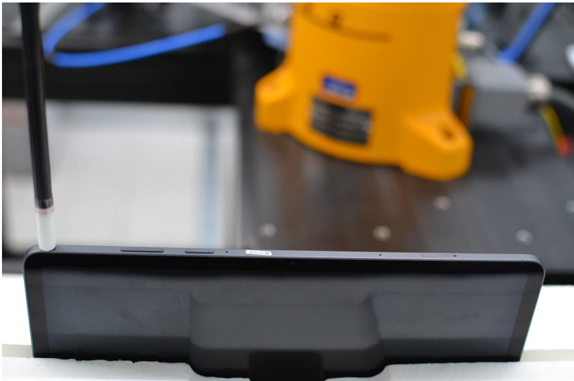
PD Test Setup Photo 36 – Body, Right Edge at 2mm
