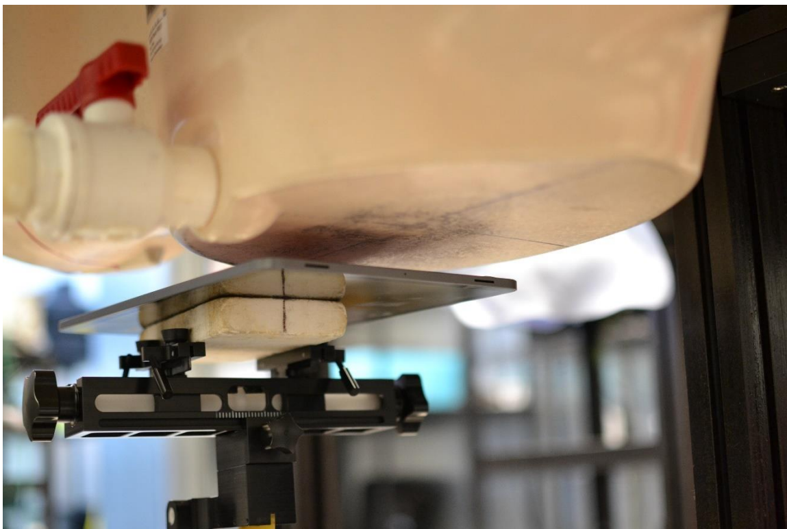
SAR Test Setup Photo 1 – Body, Back Side at 19mm – Antenna M1
