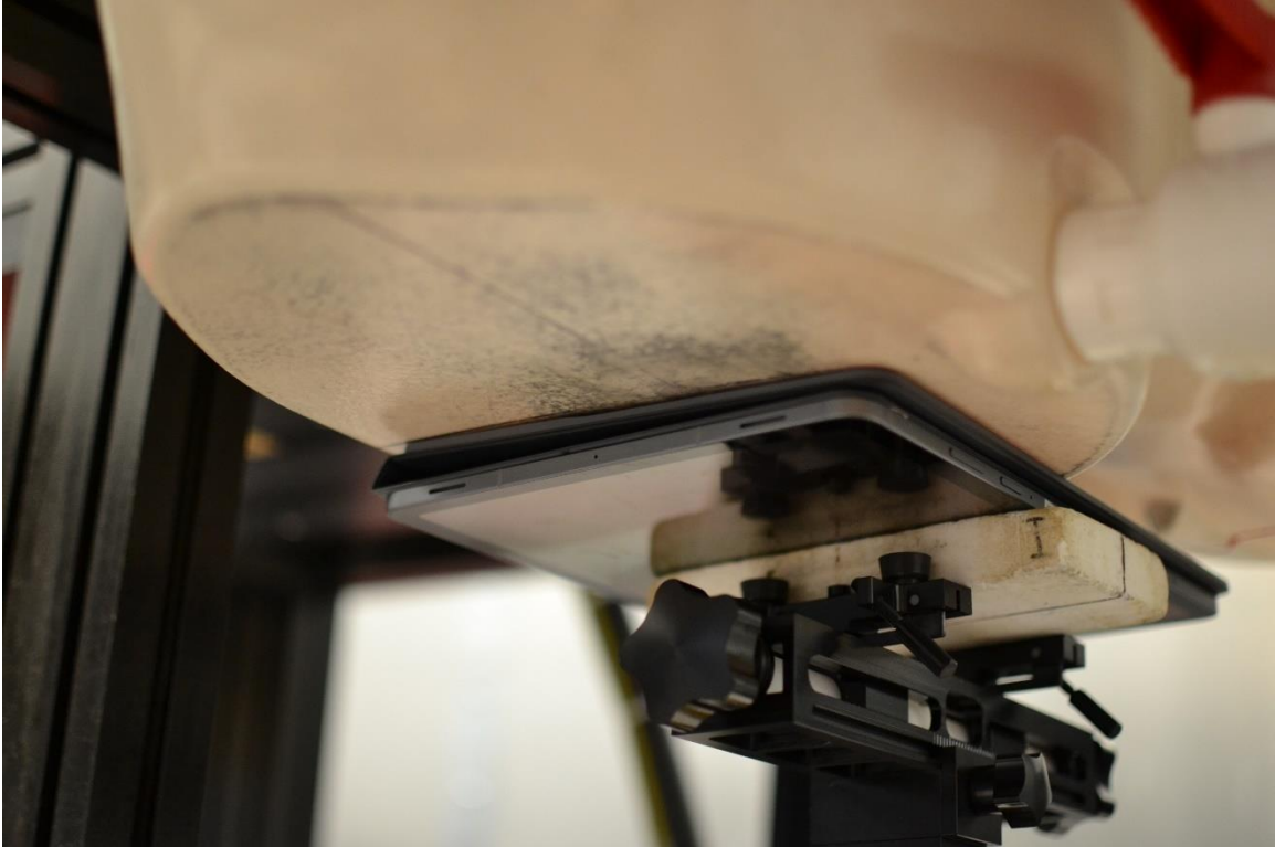
SAR Test Setup Photo 7 – Body with Keyboard, Back Side at 0mm– Antenna WIFI 1 or M4
