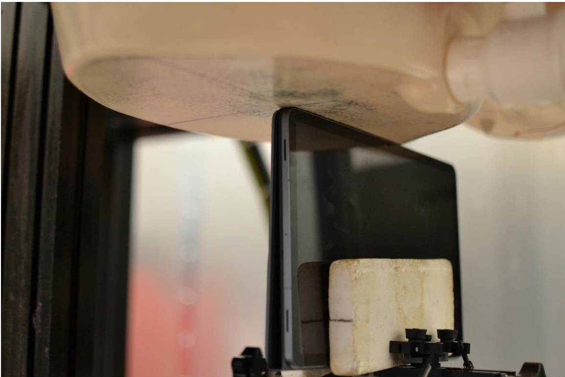
SAR Test Setup Photo 22 – Body with Keyboard, Right Edge at 0mm for M1, M4, WIFI 0, WIFI 1
