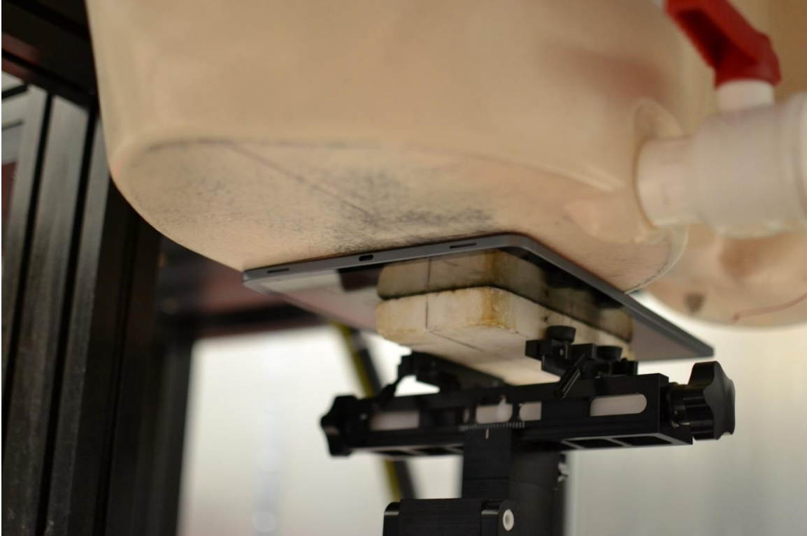
SAR Test Setup Photo 9 – Body, Back Side at 0mm– Antenna S1 or S3
