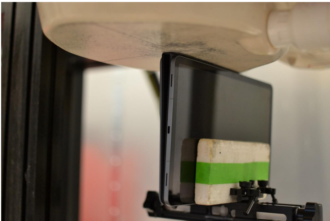
SAR Test Setup Photo 31 – Body with Keyboard, Left Edge at 0mm for S1, S2, S3, S4
