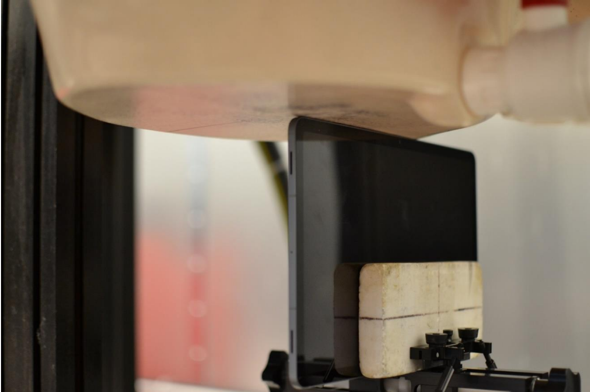
SAR Test Setup Photo 21 –Body, Right Edge at 0mm for M1, M4, WIFI 0, WIFI 1
