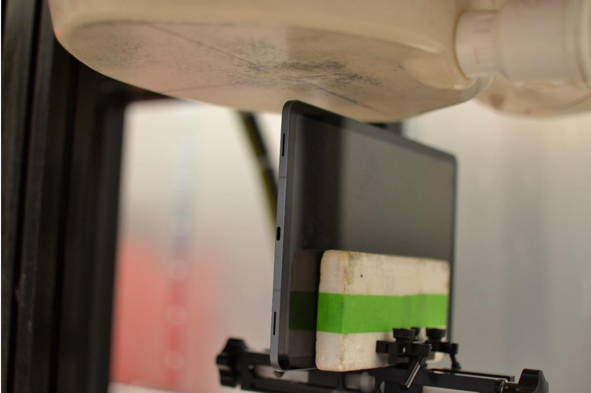
SAR Test Setup Photo 29 – Body, Left Edge at 11mm for S1
