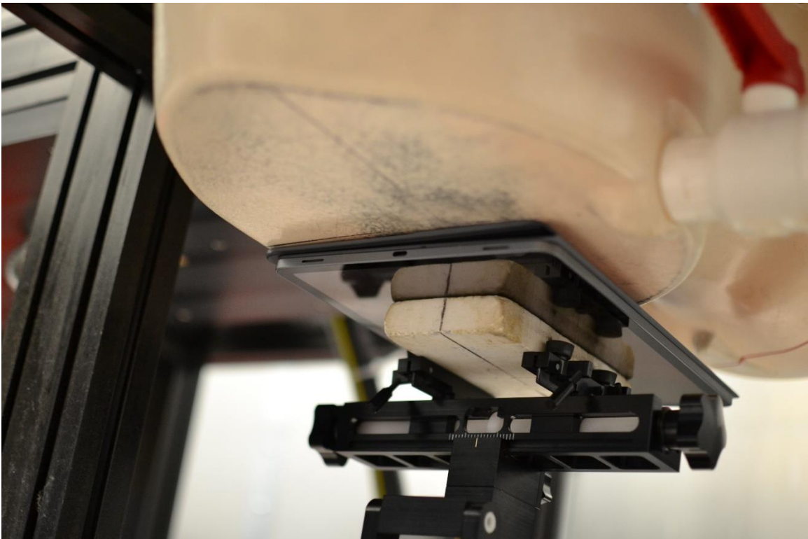
SAR Test Setup Photo 10 – Body with Keyboard, Back Side at 0mm– Antenna S1 or S3
