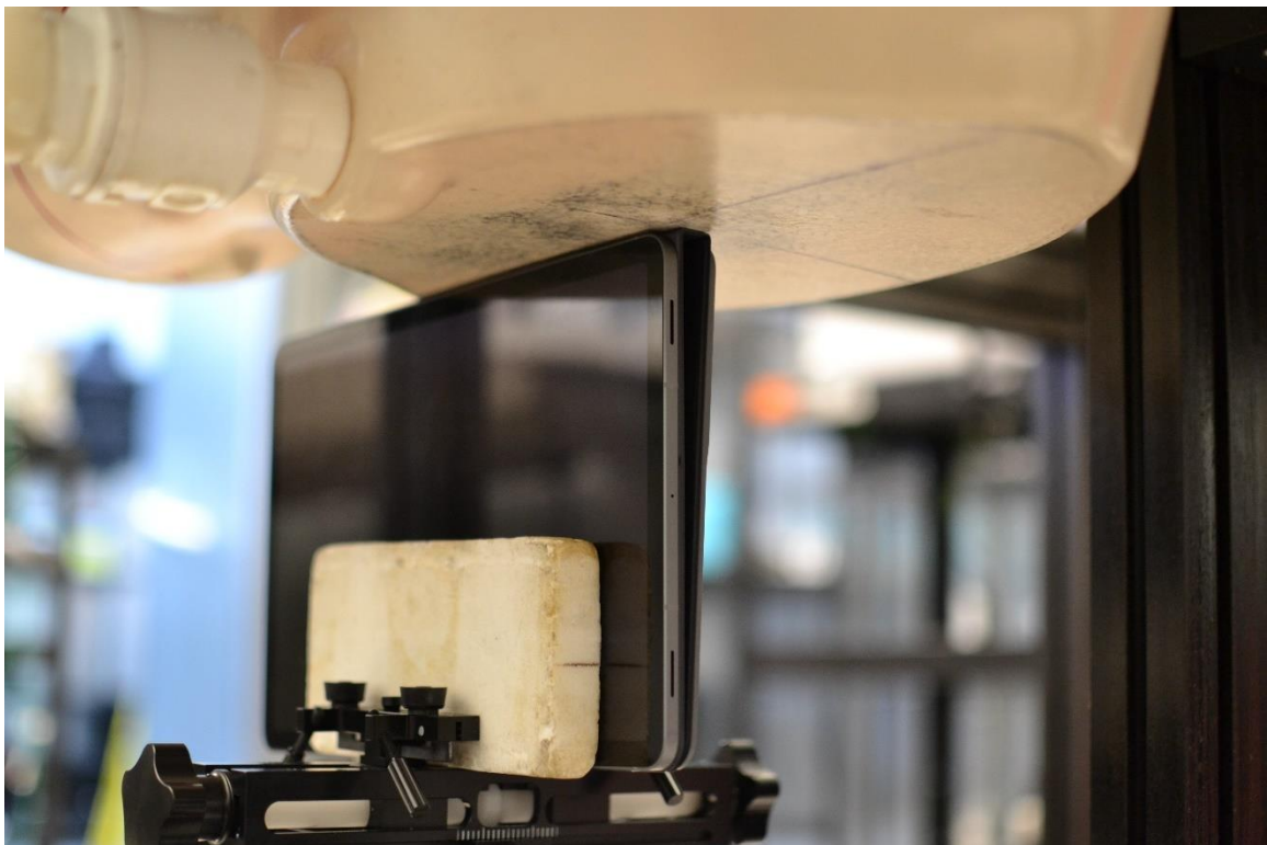
SAR Test Setup Photo 28 – Body with Keyboard, Left Edge at 0mm for M1, M4, WIFI 0, WIFI 1
