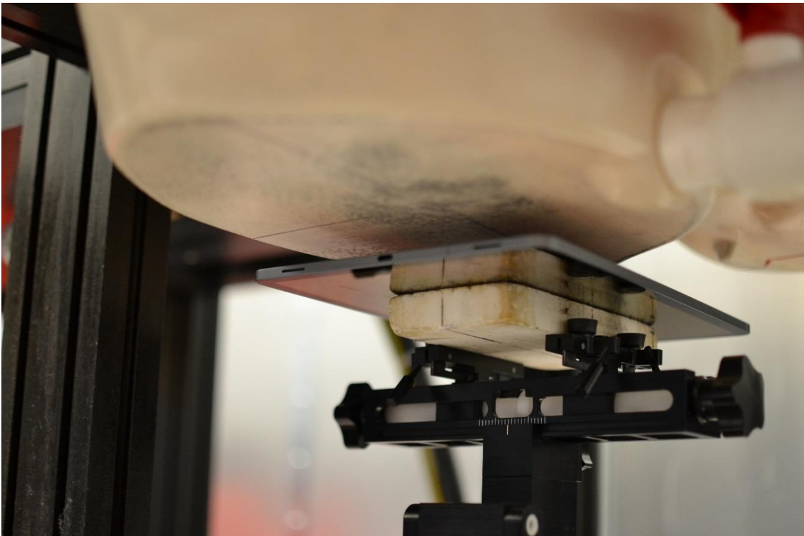
SAR Test Setup Photo 8 – Body, Back Side at 19mm– Antenna S1
