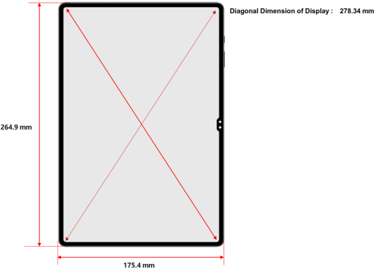
Figure J-2 DUT Dimensions Locations
