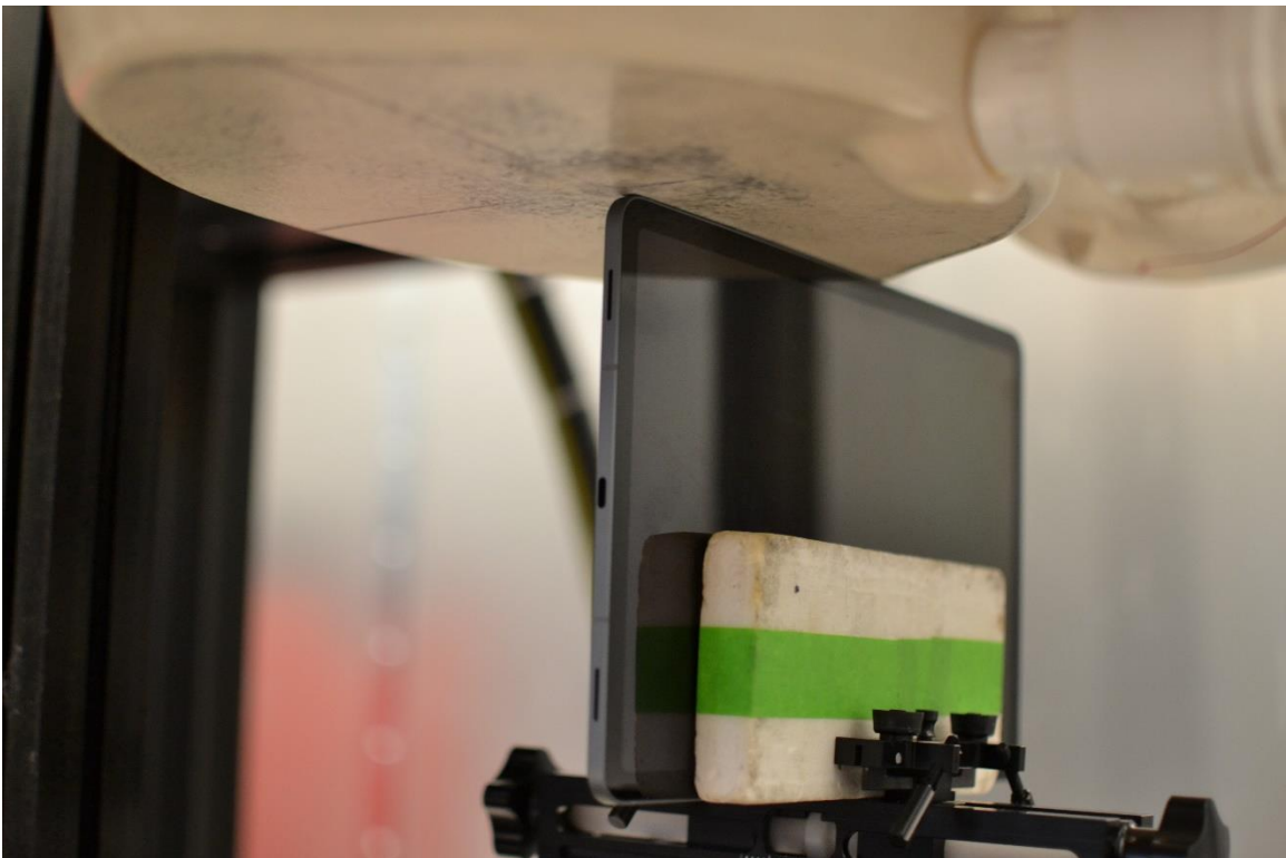
SAR Test Setup Photo 30 – Body, Left Edge at 0mm for S1, S2, S3, S4
