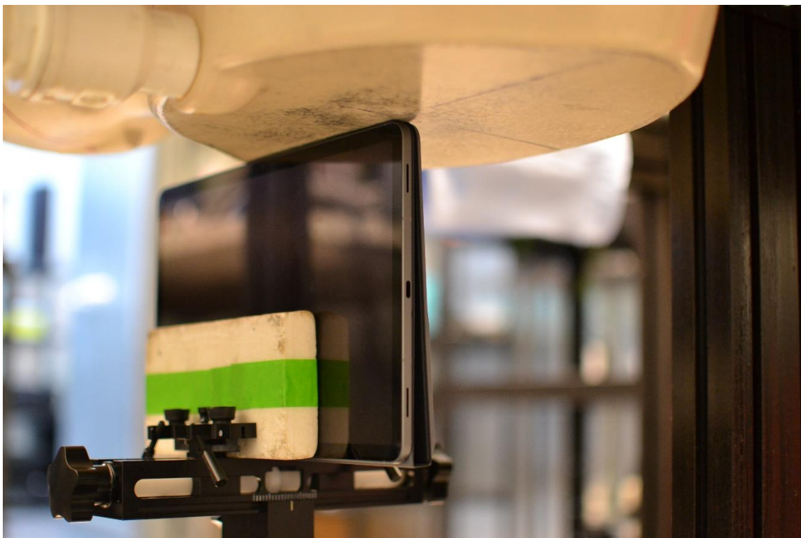
SAR Test Setup Photo 25 – Body with Keyboard, Right Edge at 0mm for S1, S2, S3, S4
