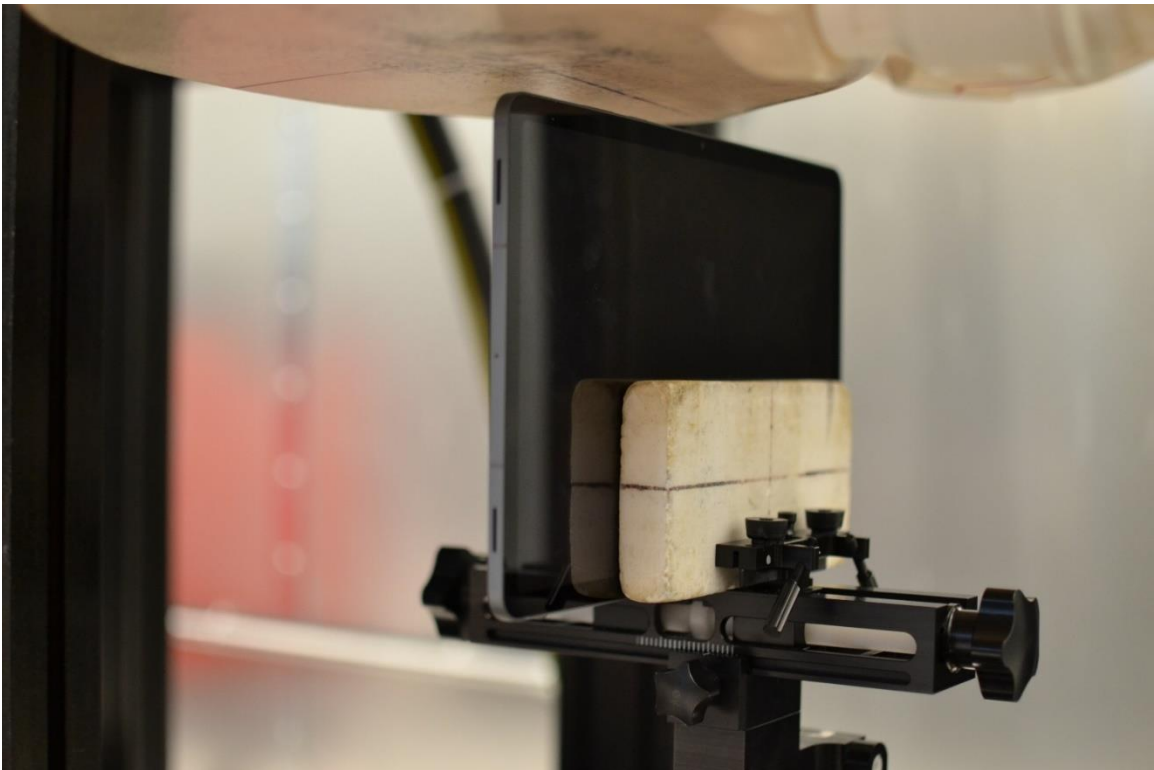
SAR Test Setup Photo 20 – Body, Right Edge at 11mm for M4, WIFI 1
