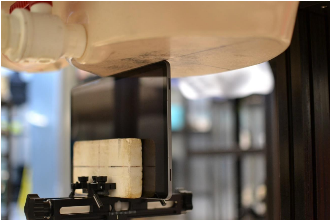
SAR Test Setup Photo 27 – Body, Left Edge at 0mm for M1, M4, WIFI 0, WIFI 1
