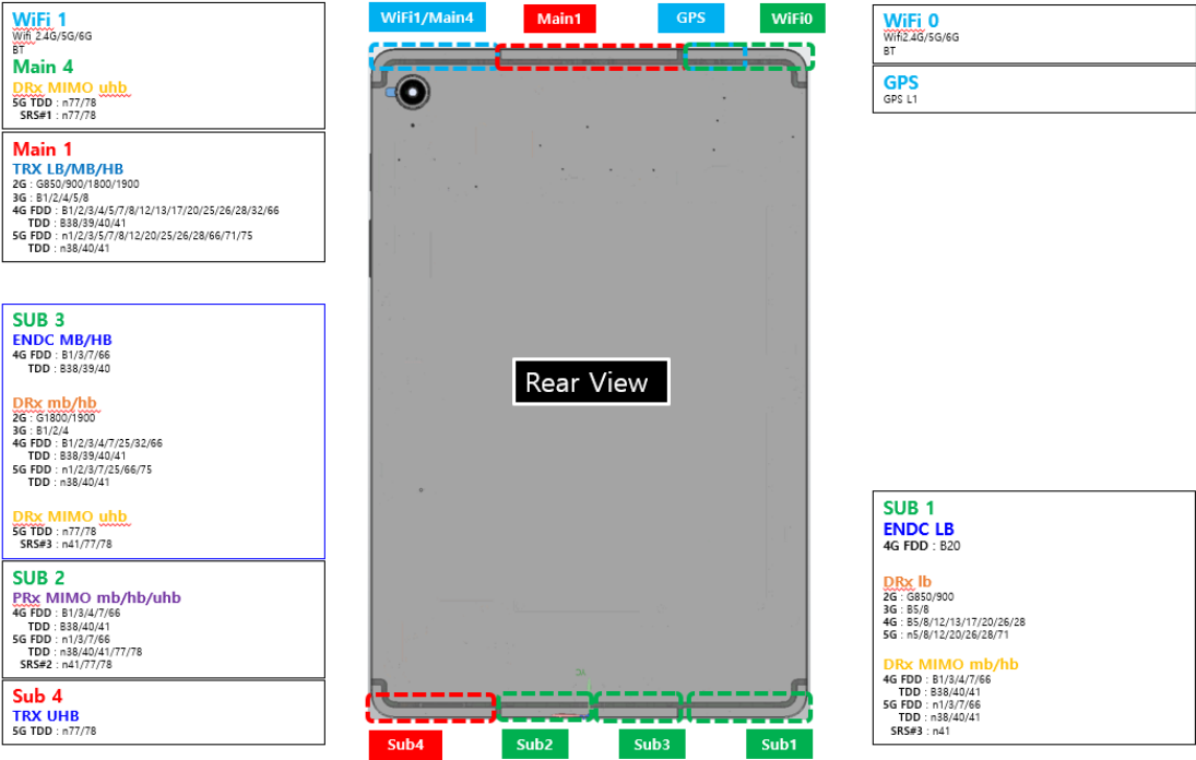
Figure J-1 DUT Antenna Locations
