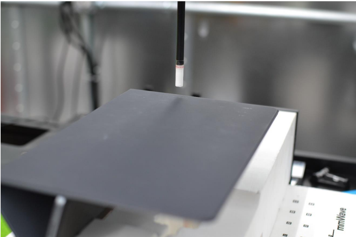
PD Test Setup Photo 40 – Laptop, Bottom Edge at 9.95mm
