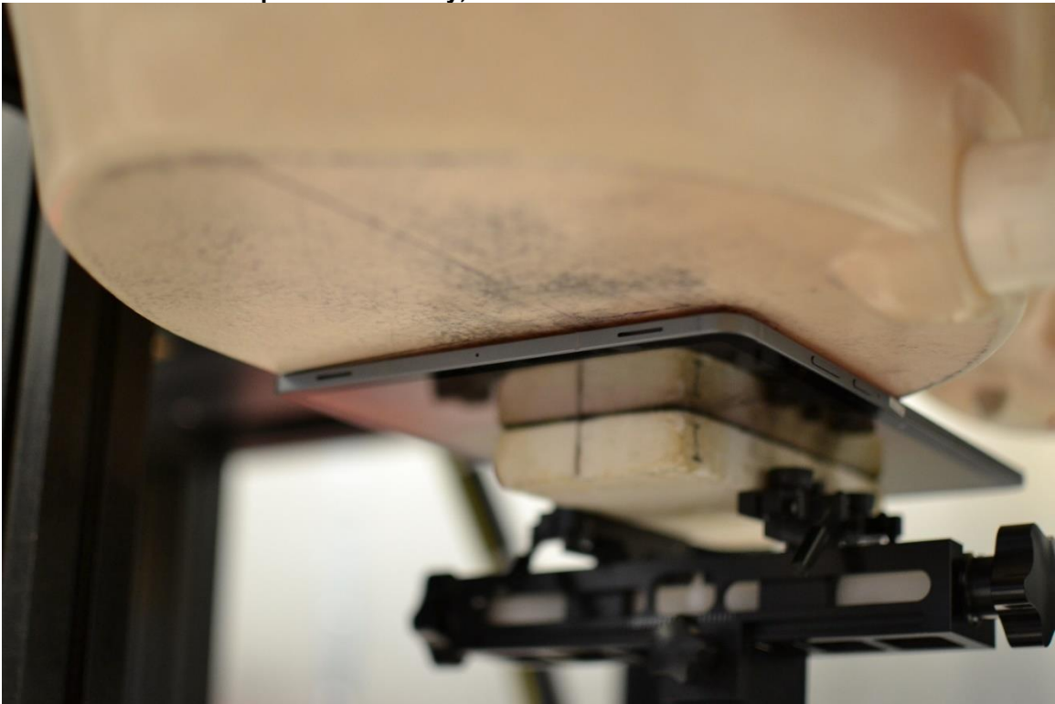
SAR Test Setup Photo 6 – Body, Back Side at 0mm– Antenna WIFI 1 or M4
