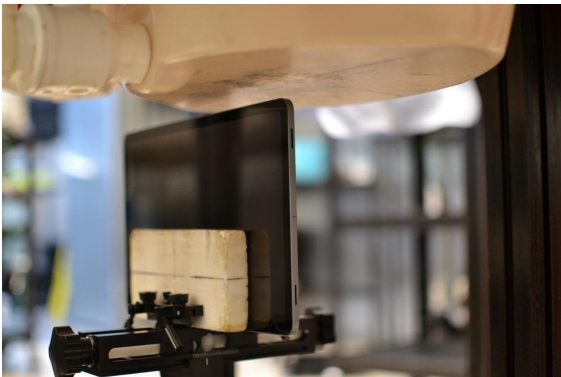
SAR Test Setup Photo 26 – Body, Left Edge at 11mm for WIFI 0
