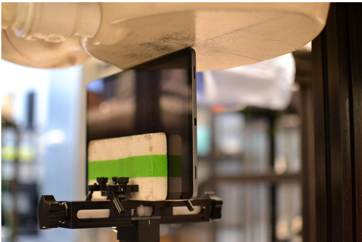
SAR Test Setup Photo 24 – Body, Right Edge at 0mm for S1, S2, S3, S4
