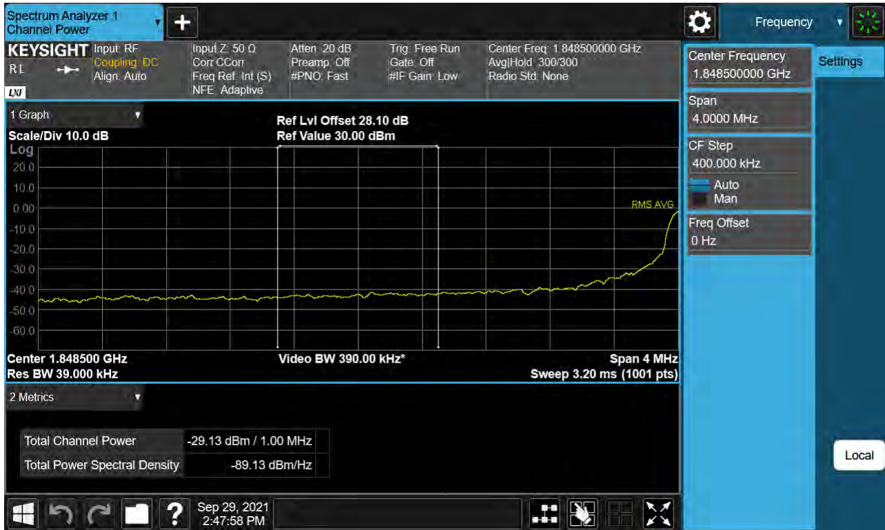
Sub6 n25(2). Lower Extended Band Edge Plot (20 M BW Ch.372000 BPSK_ Full RB) -2
