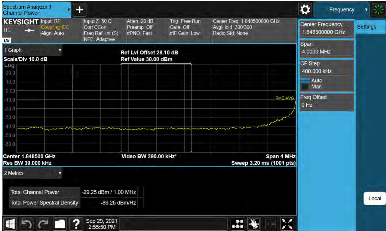
Sub6 n25. Lower Extended Band Edge Plot (25 M BW Ch.372500 BPSK_ Full RB) -2
