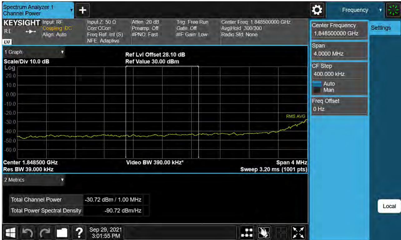
Sub6 n25. Lower Extended Band Edge Plot (30 M BW Ch.373000 BPSK_ Full RB) -2
