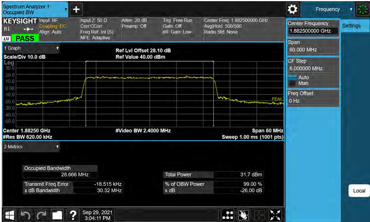
Sub6 n25. Occupied Bandwidth Plot (30 M BW Ch.376500 16QAM _ Full RB _0)
