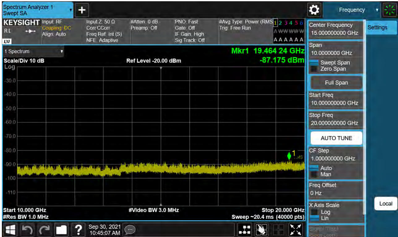
Sub6 n66. Conducted Spurious Plot_2 (343500ch_15 MHz_BPSK_ RB 1_1)
