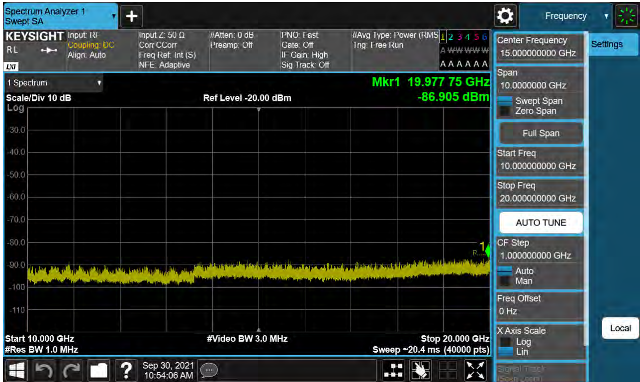
Sub6 n66. Conducted Spurious Plot_2 (349000ch_20 MHz_BPSK_ RB 1_1)
