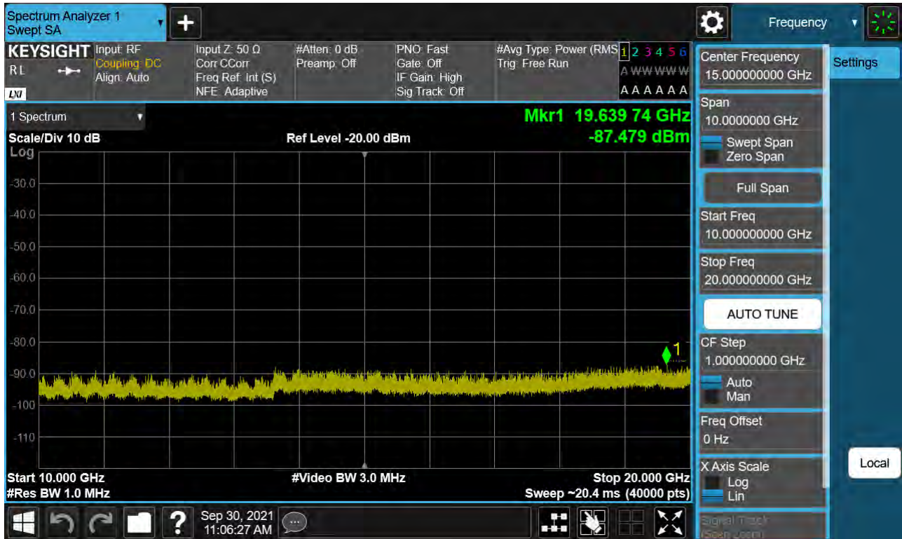
Sub6 n66. Conducted Spurious Plot_2 (346000ch_40 MHz_BPSK_ RB 1_1)
