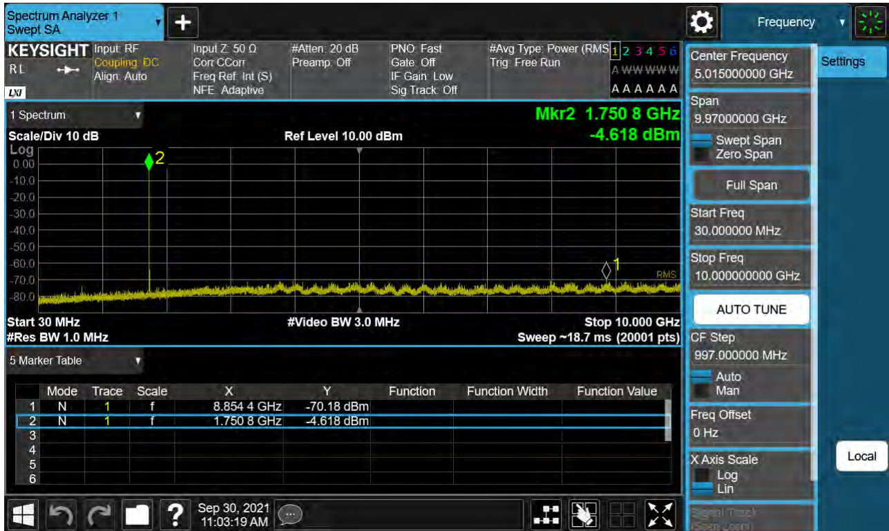
Sub6 n66. Conducted Spurious Plot_1 (353000ch_30 MHz_BPSK_ RB 1_1)
