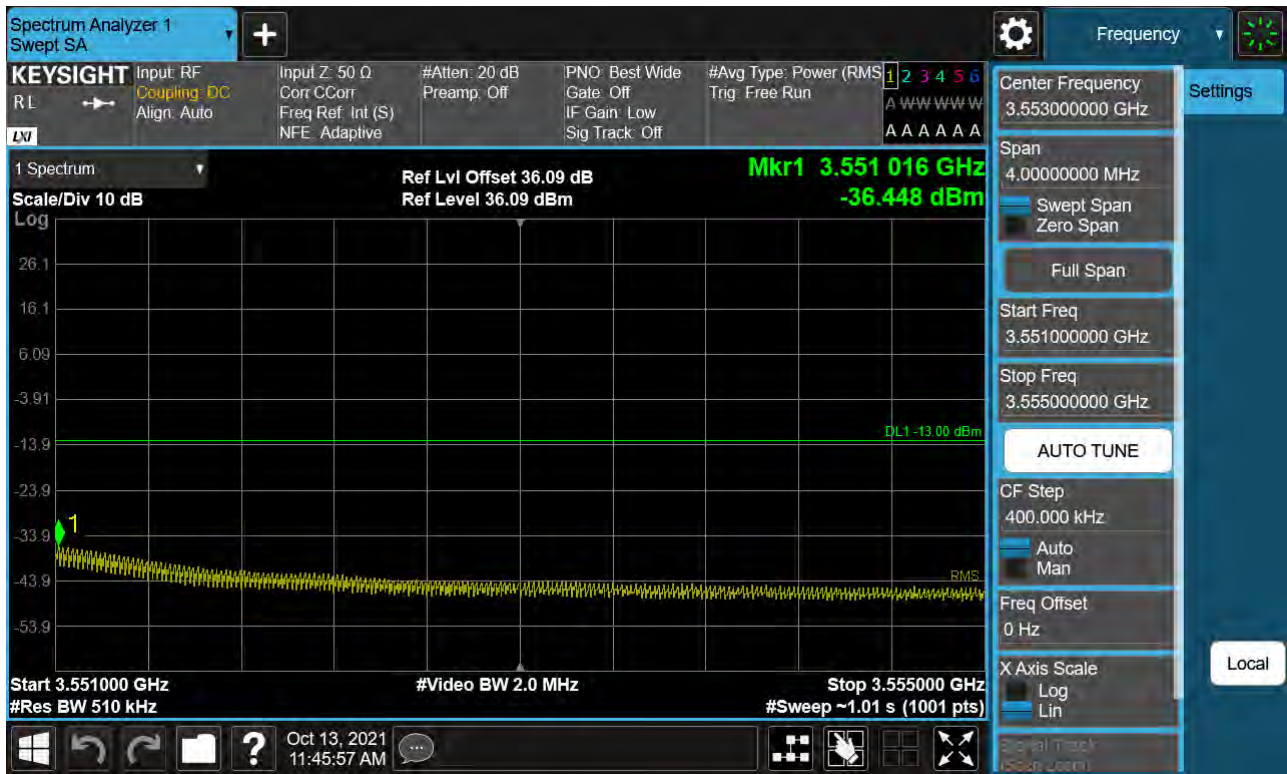
Sub6 n77. High Band Edge Plot (70 M BW Ch.634332 BPSK 1RB)(2)
