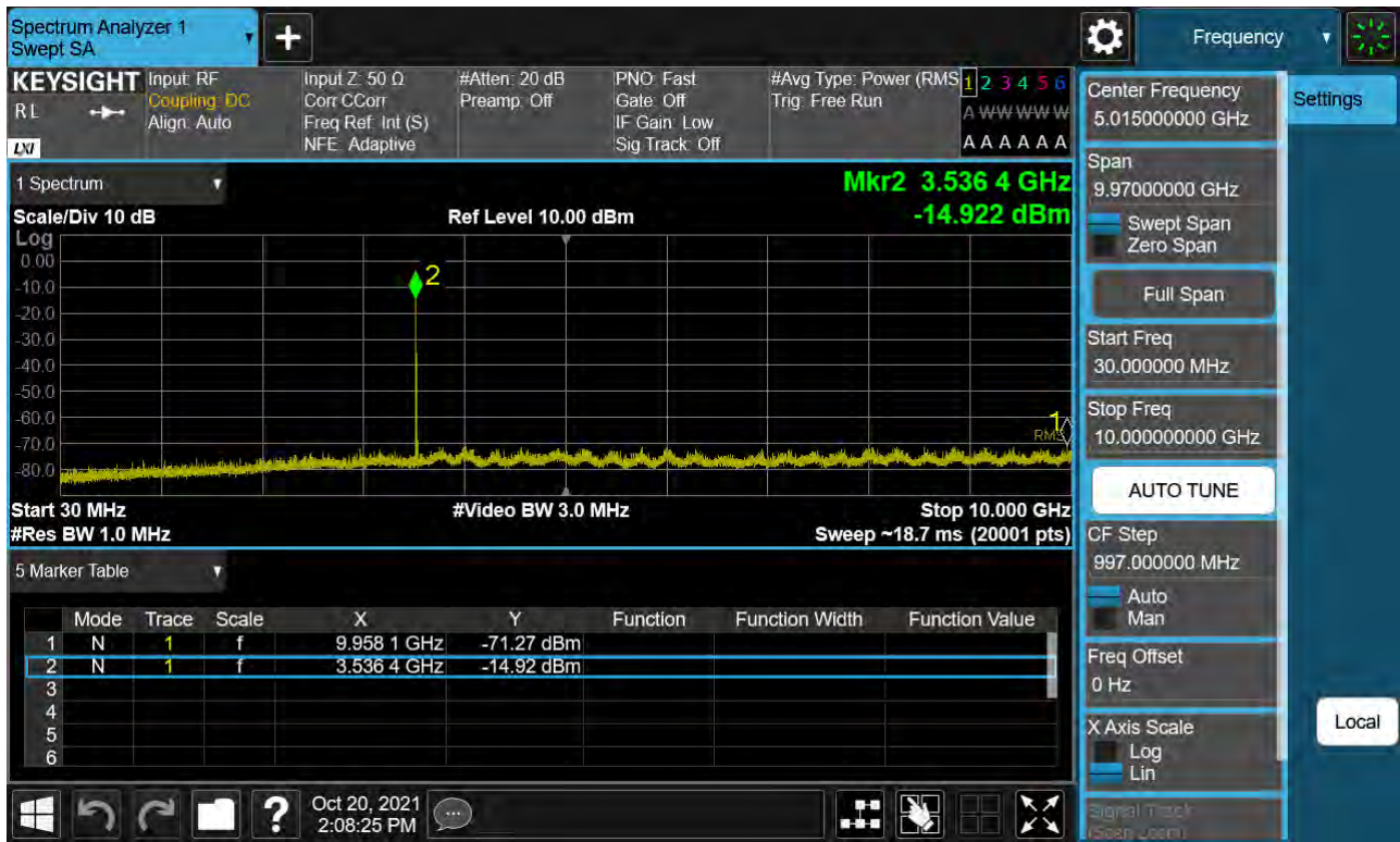
Sub6 n77. Conducted Spurious Plot_1 (636166ch_15 MHz_BPSK)
