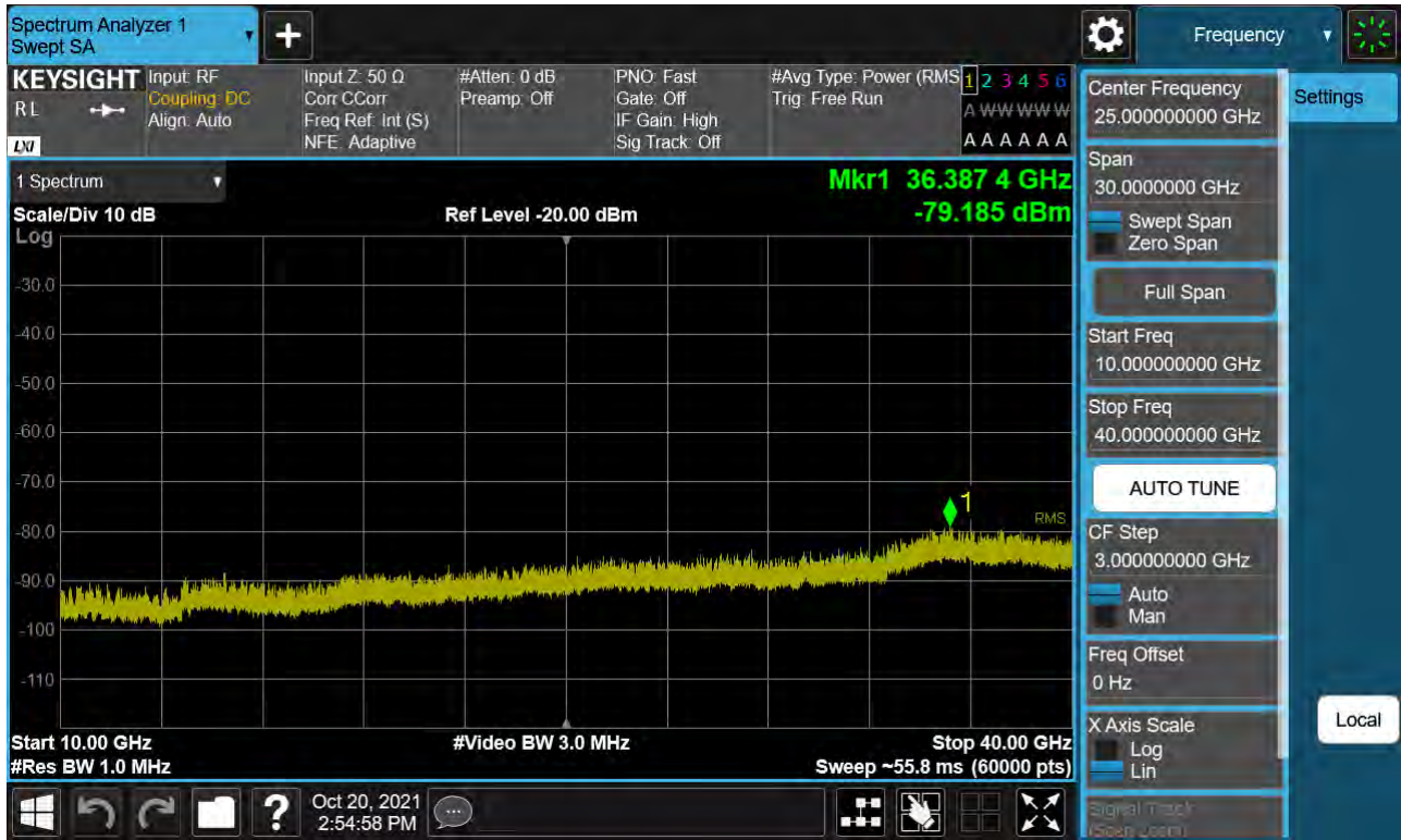
Sub6 n77. Conducted Spurious Plot_2 (633334ch_10 MHz_BPSK)
