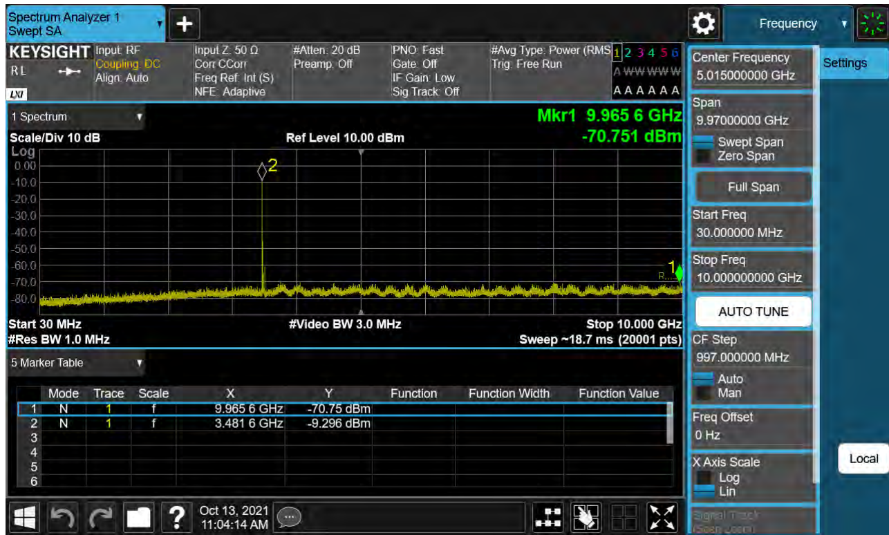
Sub6 n77. Conducted Spurious Plot_1 (633334ch_40 MHz_BPSK)
