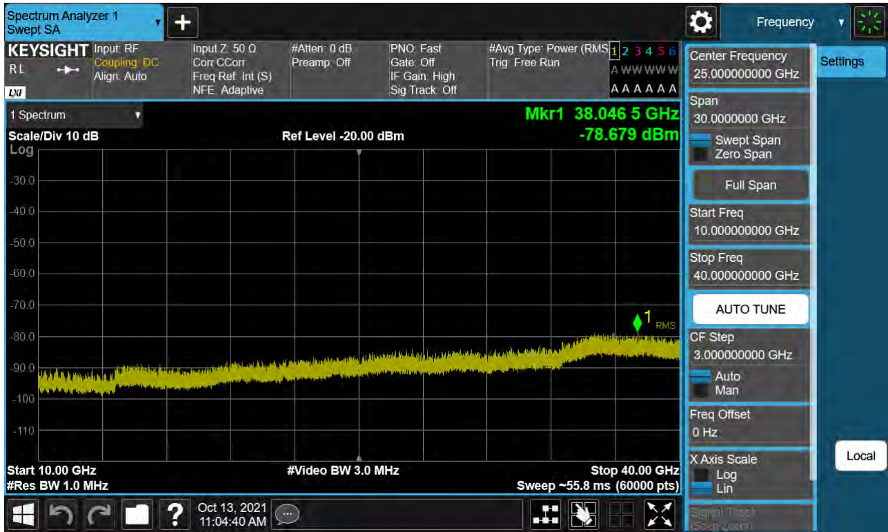
Sub6 n77. Conducted Spurious Plot_2 (633334ch_40 MHz_BPSK)
