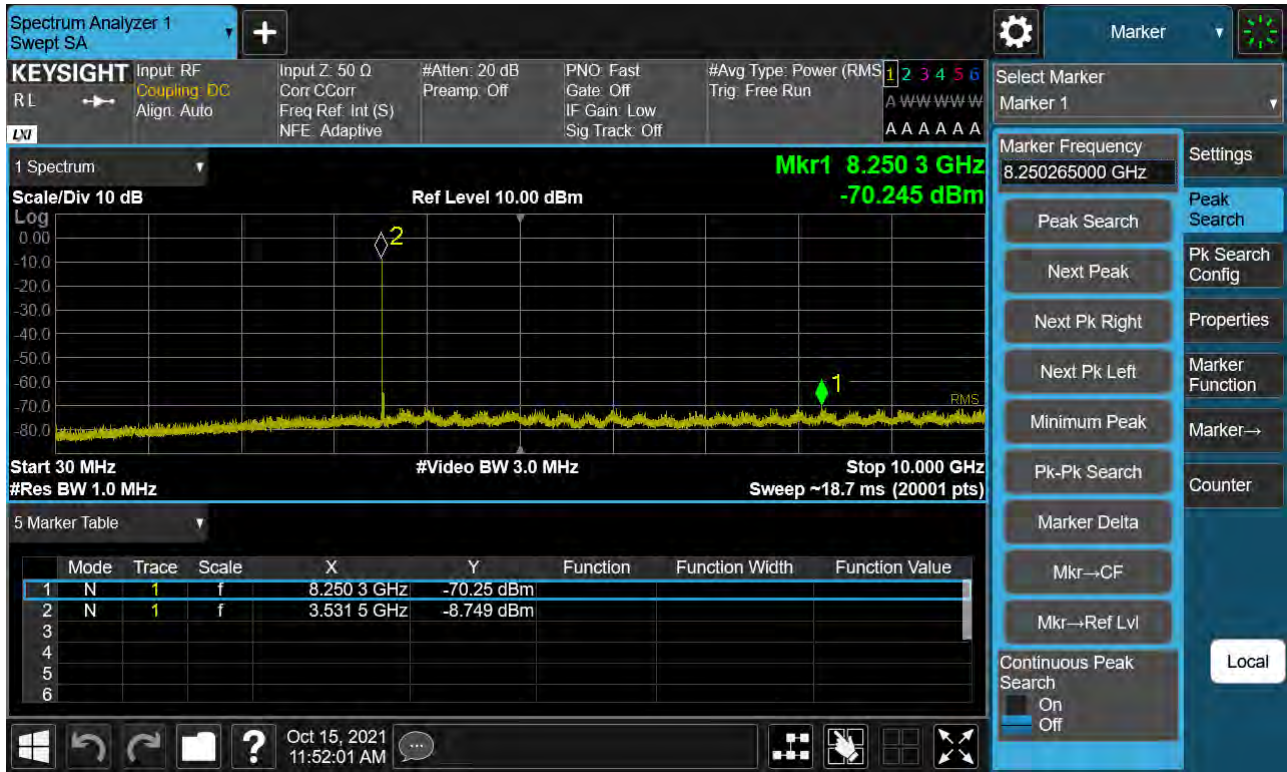
Sub6 n77. Conducted Spurious Plot_1 (636000ch_20 MHz_BPSK)
