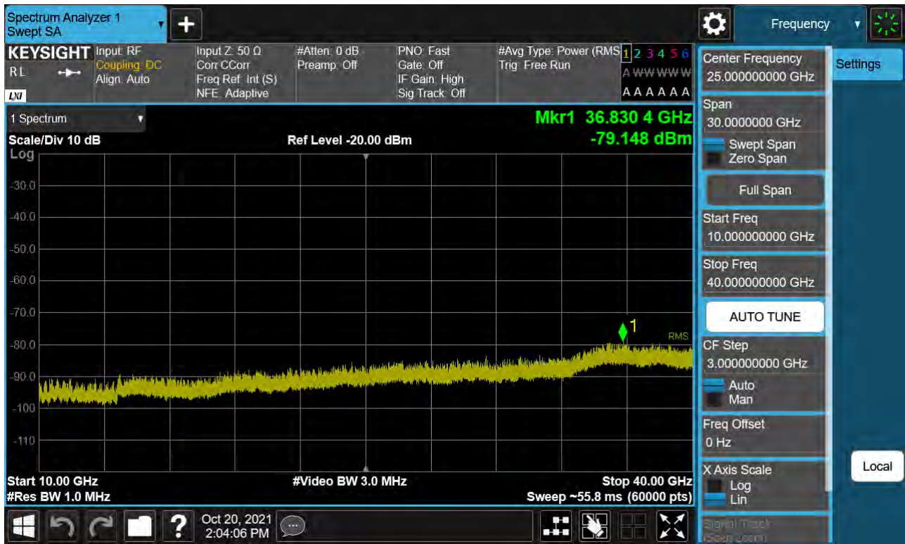
Sub6 n77. Conducted Spurious Plot_2 (633334ch_15 MHz_BPSK)
