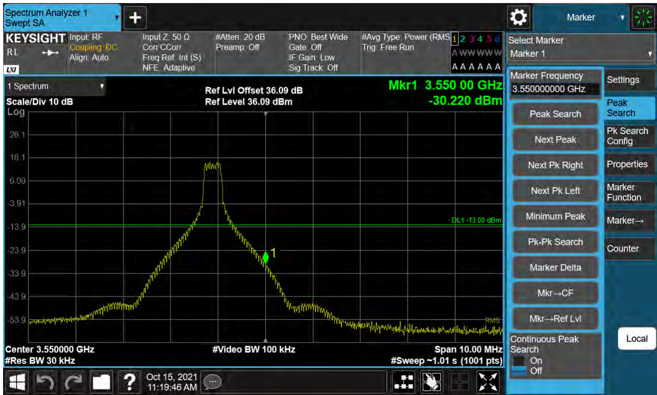
Sub6 n77. High Band Edge Plot (90 M BW Ch.633666 BPSK 1RB)(1)
