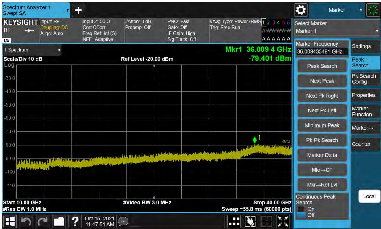
Sub6 n77. Conducted Spurious Plot_2 (633334ch_20 MHz_BPSK)
