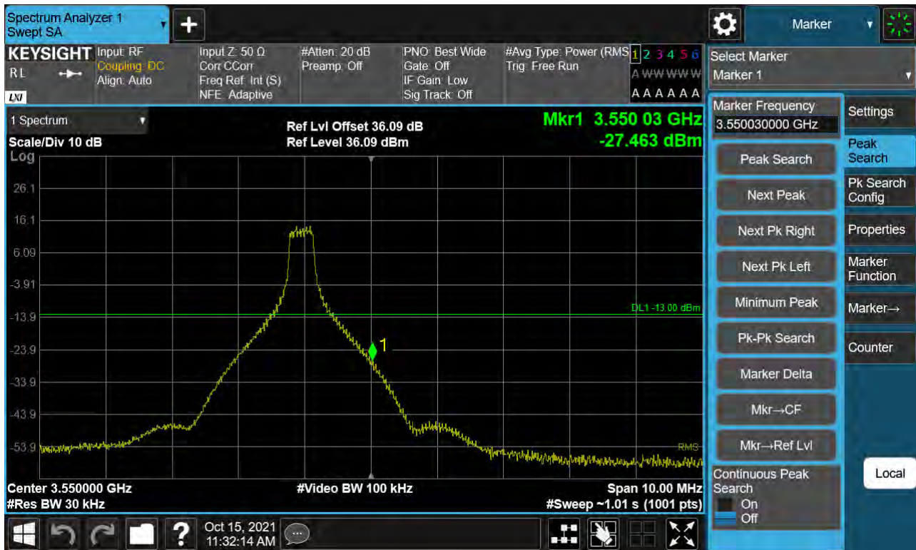
Sub6 n77. High Band Edge Plot (100 M BW Ch.633334 BPSK 1RB)(1)
