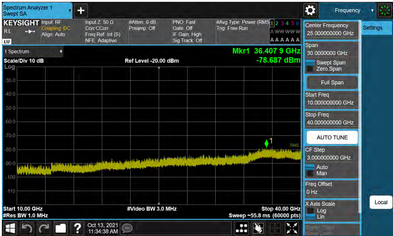
Sub6 n77. Conducted Spurious Plot_2 (634666ch_60 MHz_BPSK)
