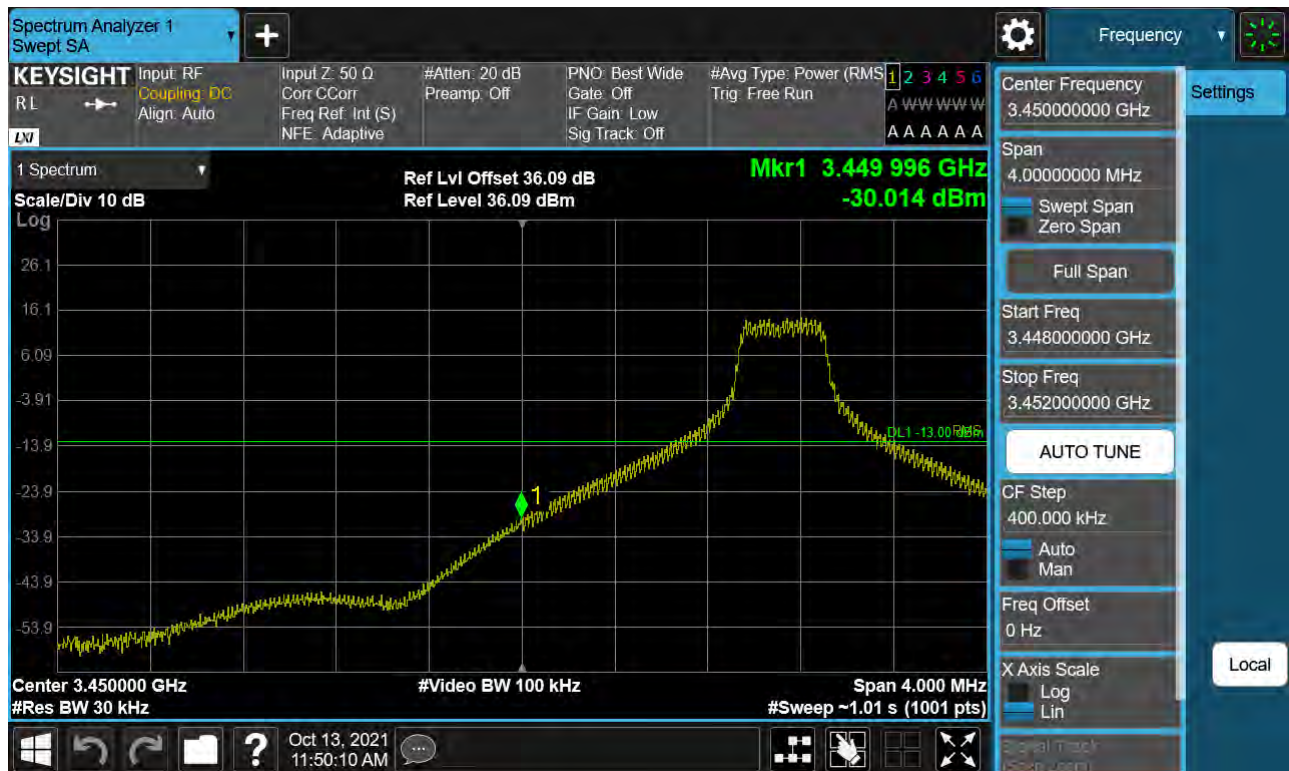
Sub6 n77. Low Band Edge Plot (80 M BW Ch.632668 BPSK 1RB)(1)
