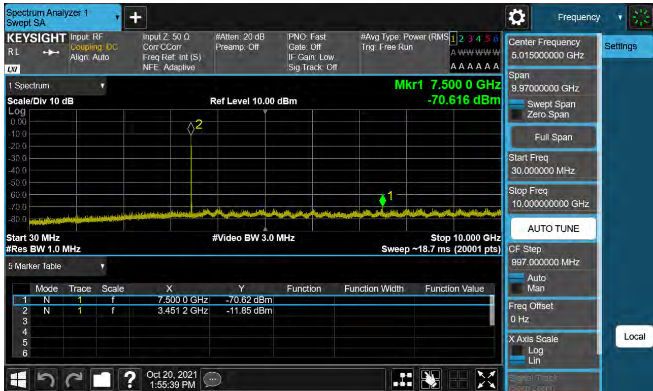
Sub6 n77. Conducted Spurious Plot_1 (630500ch_15 MHz_BPSK)
