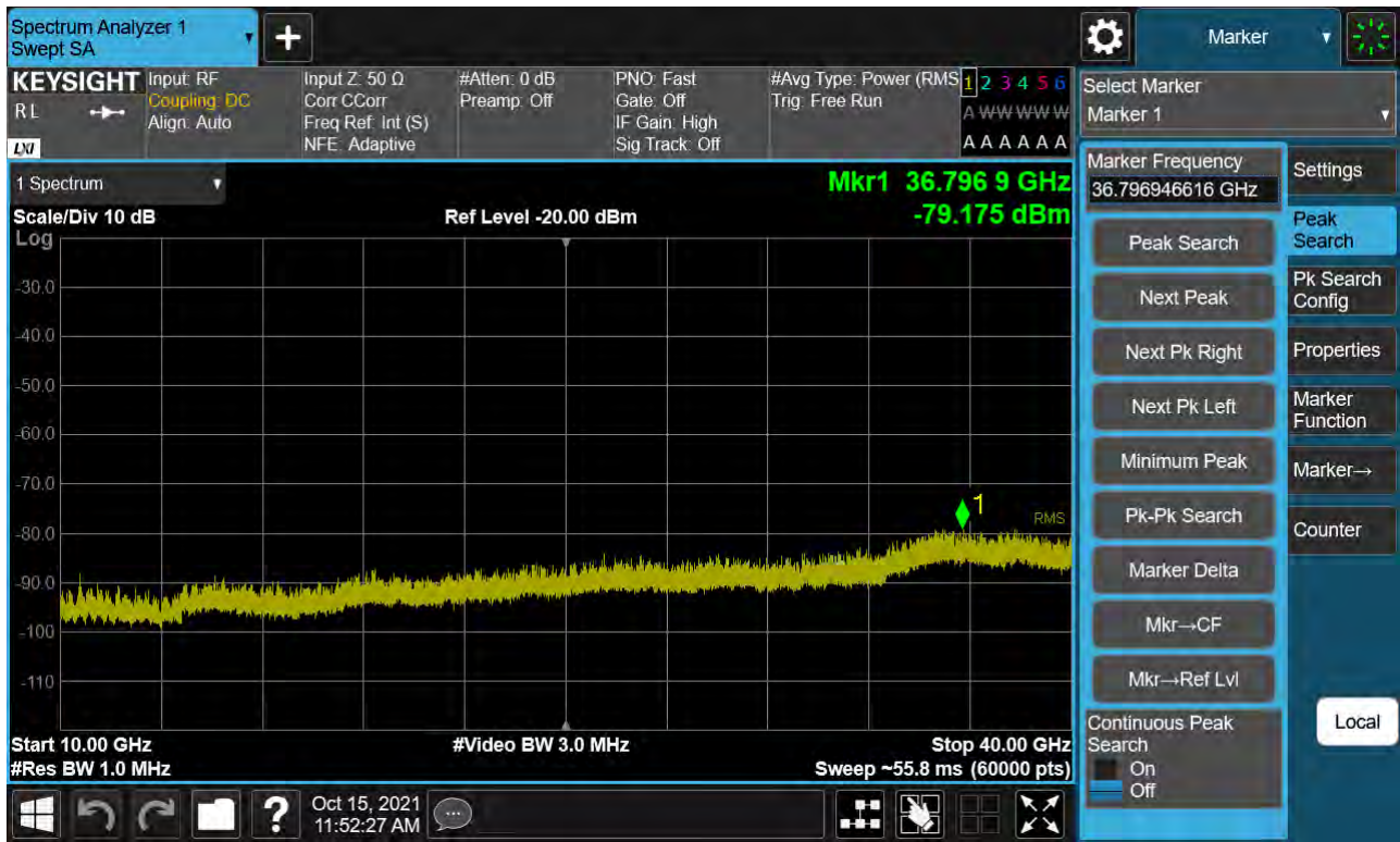
Sub6 n77. Conducted Spurious Plot_2 (636000ch_20 MHz_BPSK)
