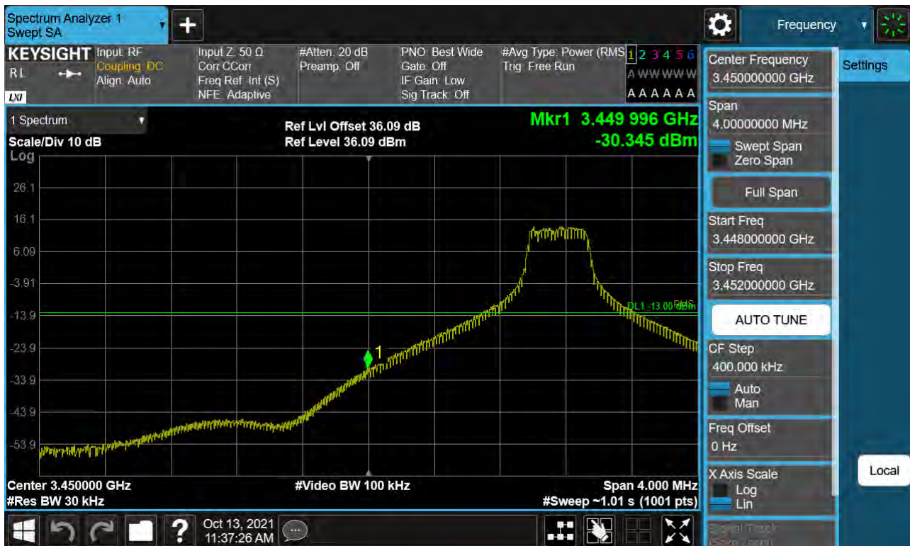
Sub6 n77. Low Band Edge Plot (70 M BW Ch.632334 BPSK 1RB)(1)
