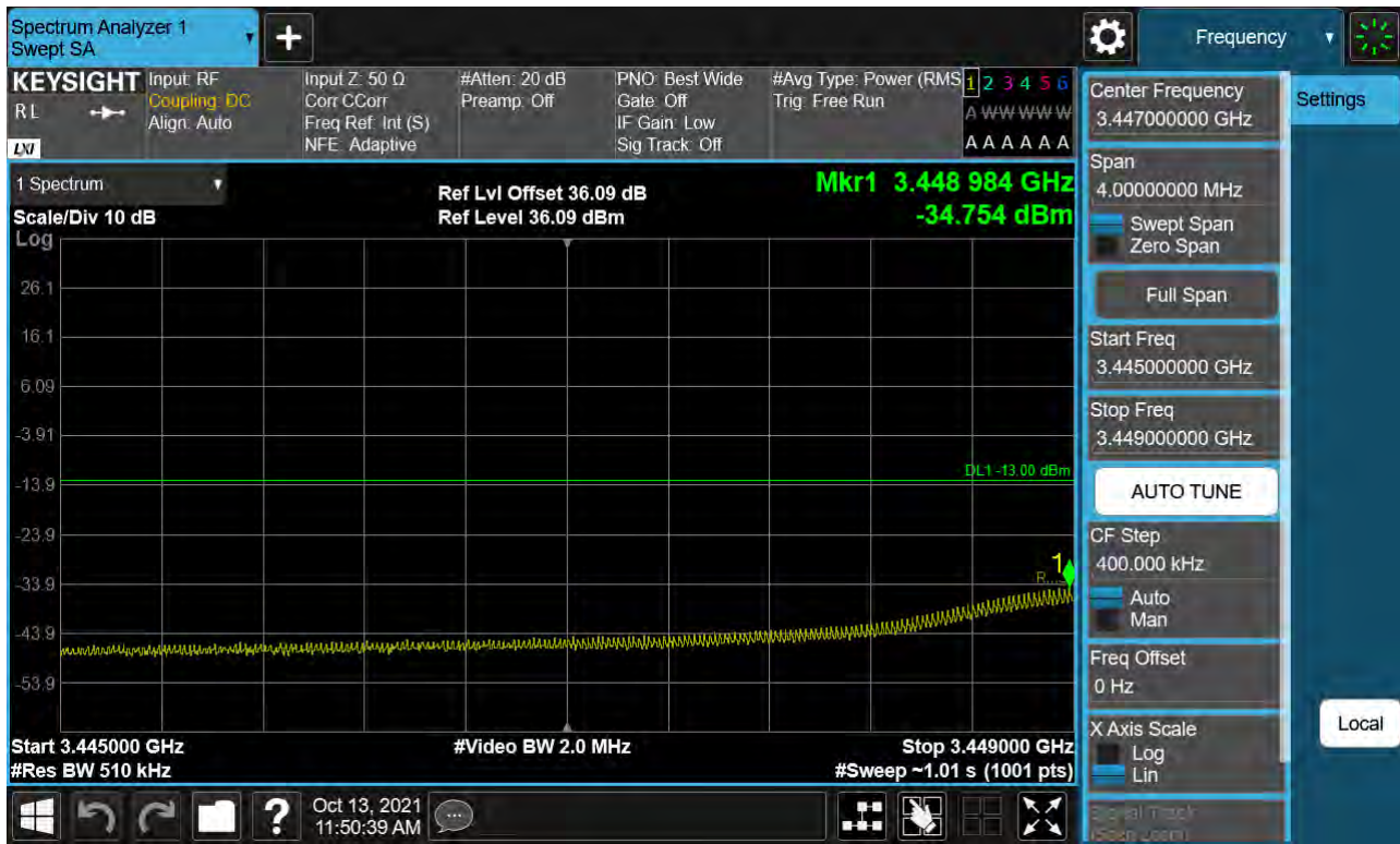
Sub6 n77. Low Band Edge Plot (80 M BW Ch.632668 BPSK 1RB)(2)
