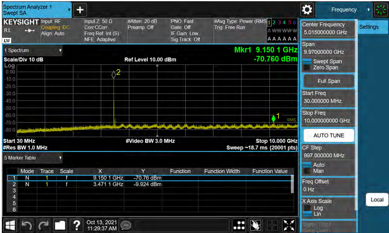
Sub6 n77. Conducted Spurious Plot_1 (633334ch_60 MHz_BPSK)
