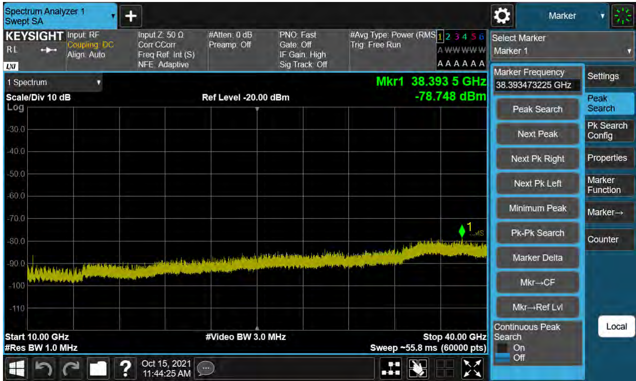
Sub6 n77. Conducted Spurious Plot_2 (630668ch_20 MHz_BPSK)
