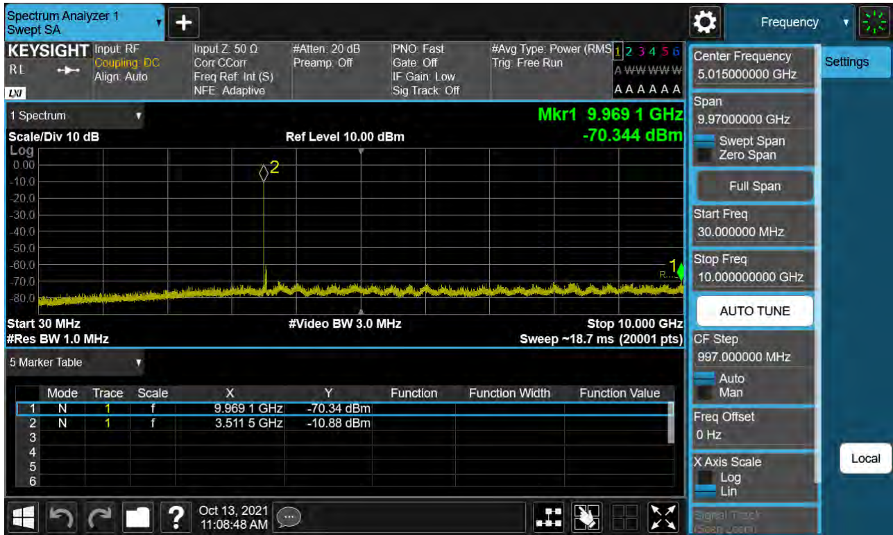
Sub6 n77. Conducted Spurious Plot_1 (635332ch_40 MHz_BPSK)
