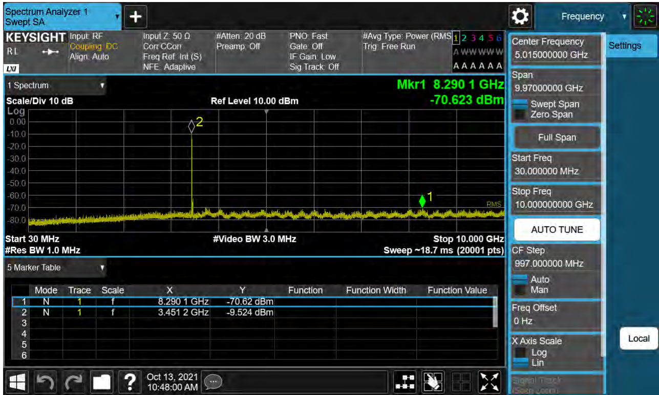
Sub6 n77. Conducted Spurious Plot_1 (631000ch_30 MHz_BPSK)
