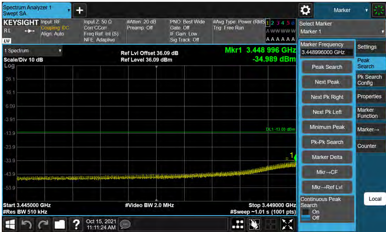
Sub6 n77. Low Band Edge Plot (90 M BW Ch.633000 BPSK 1RB)(2)
