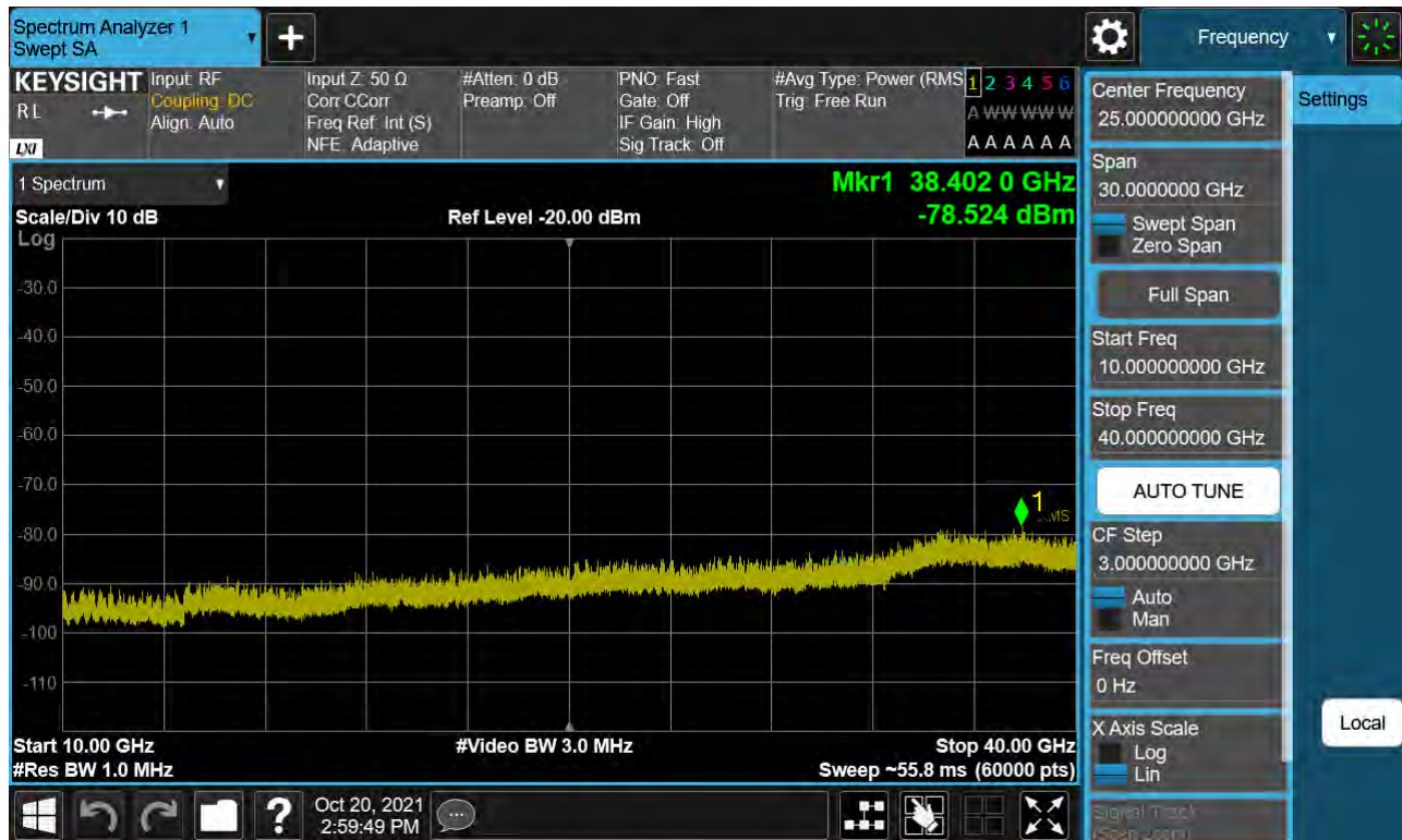
Sub6 n77. Conducted Spurious Plot_2 (636322ch_10 MHz_BPSK)
