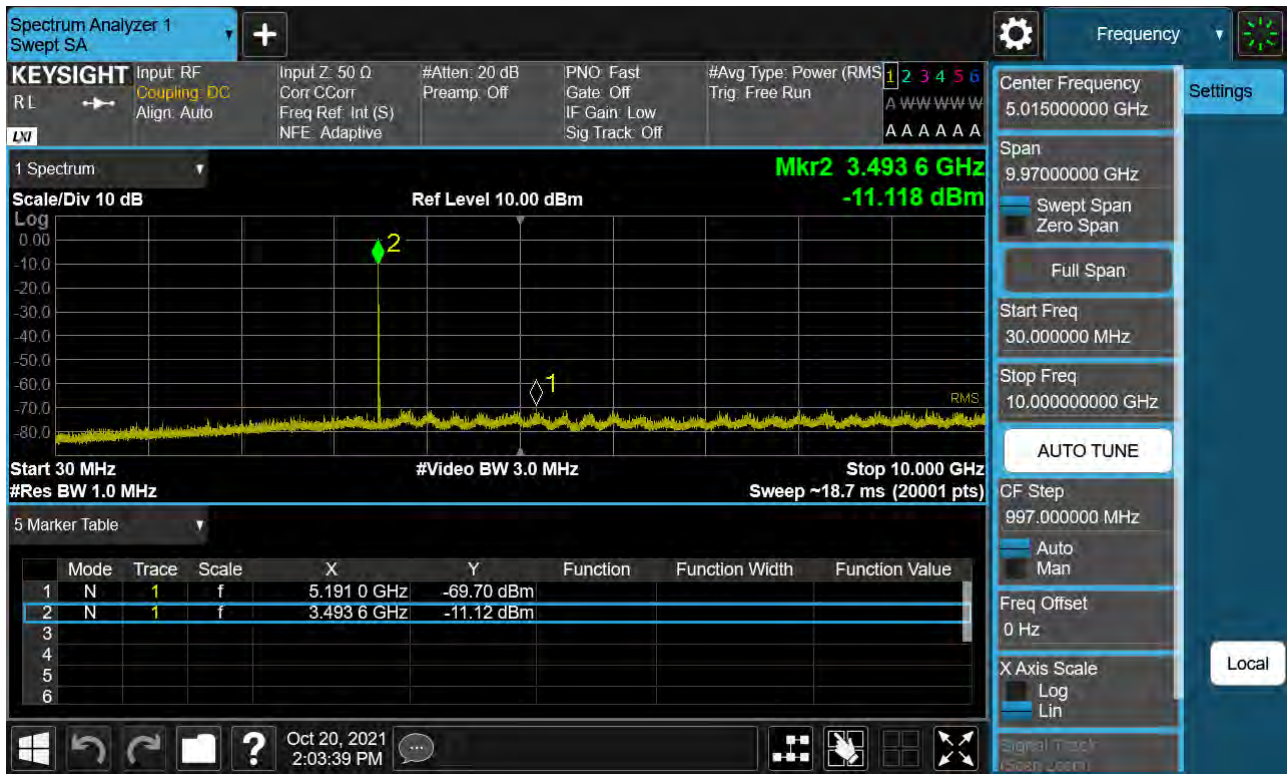
Sub6 n77. Conducted Spurious Plot_1 (633334ch_15 MHz_BPSK)
