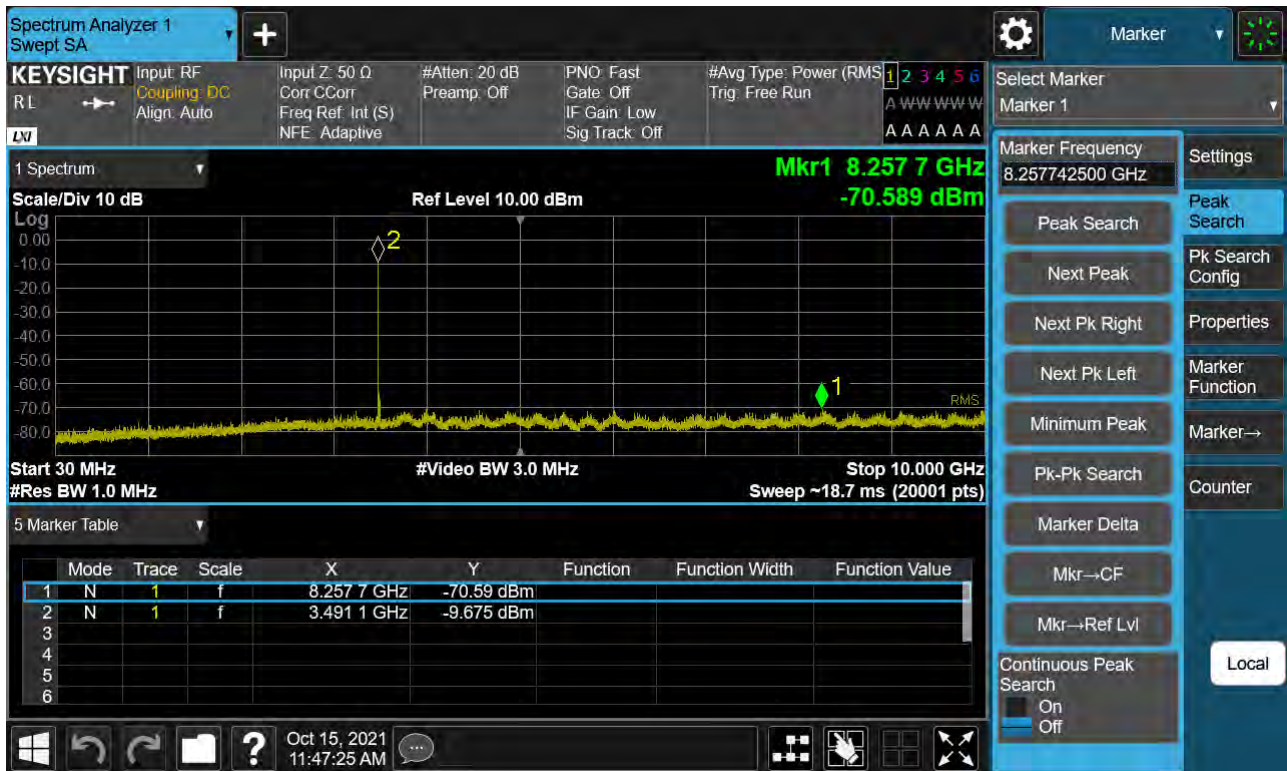
Sub6 n77. Conducted Spurious Plot_1 (633334ch_20 MHz_BPSK)
