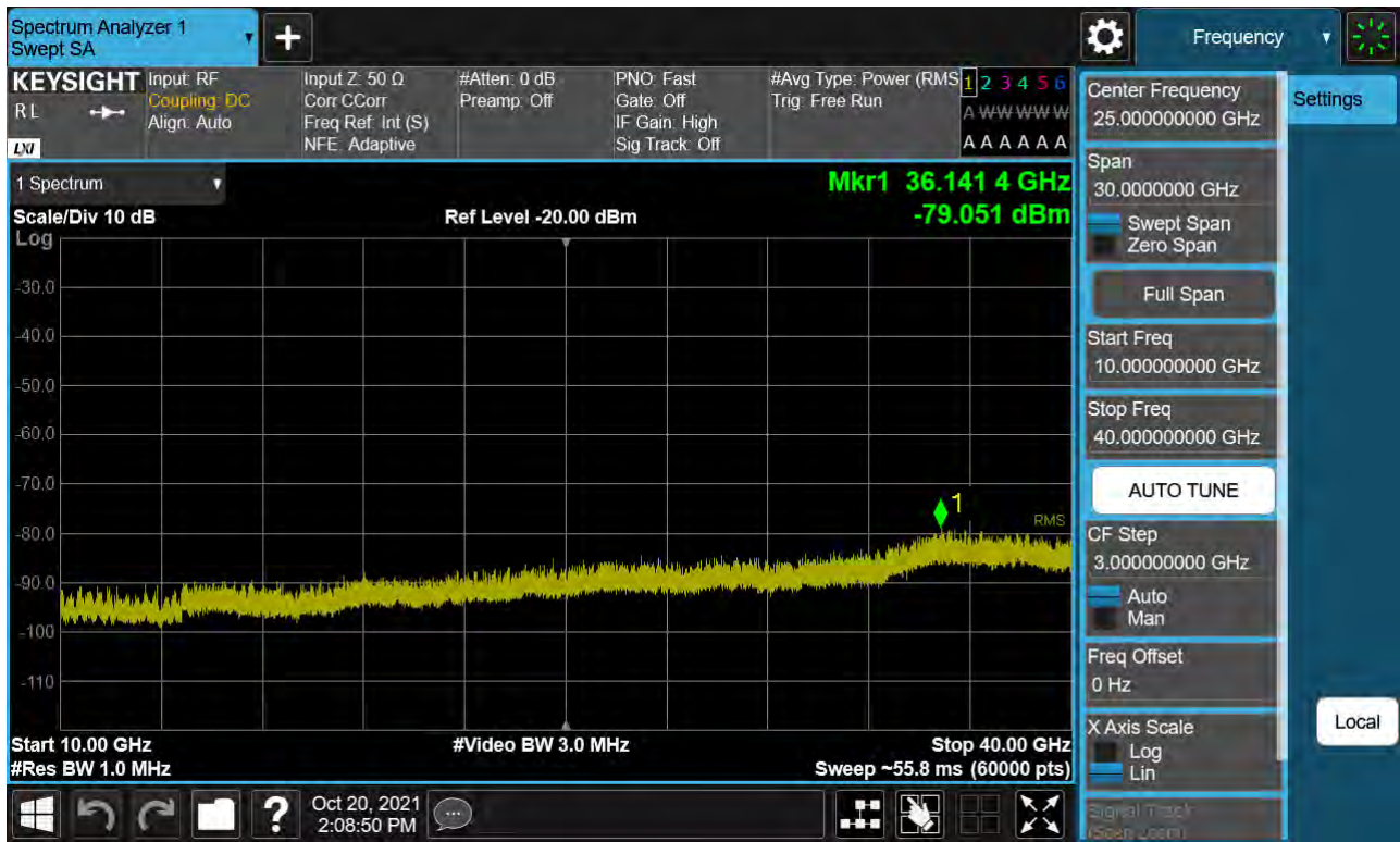
Sub6 n77. Conducted Spurious Plot_2 (636166ch_15 MHz_BPSK)
