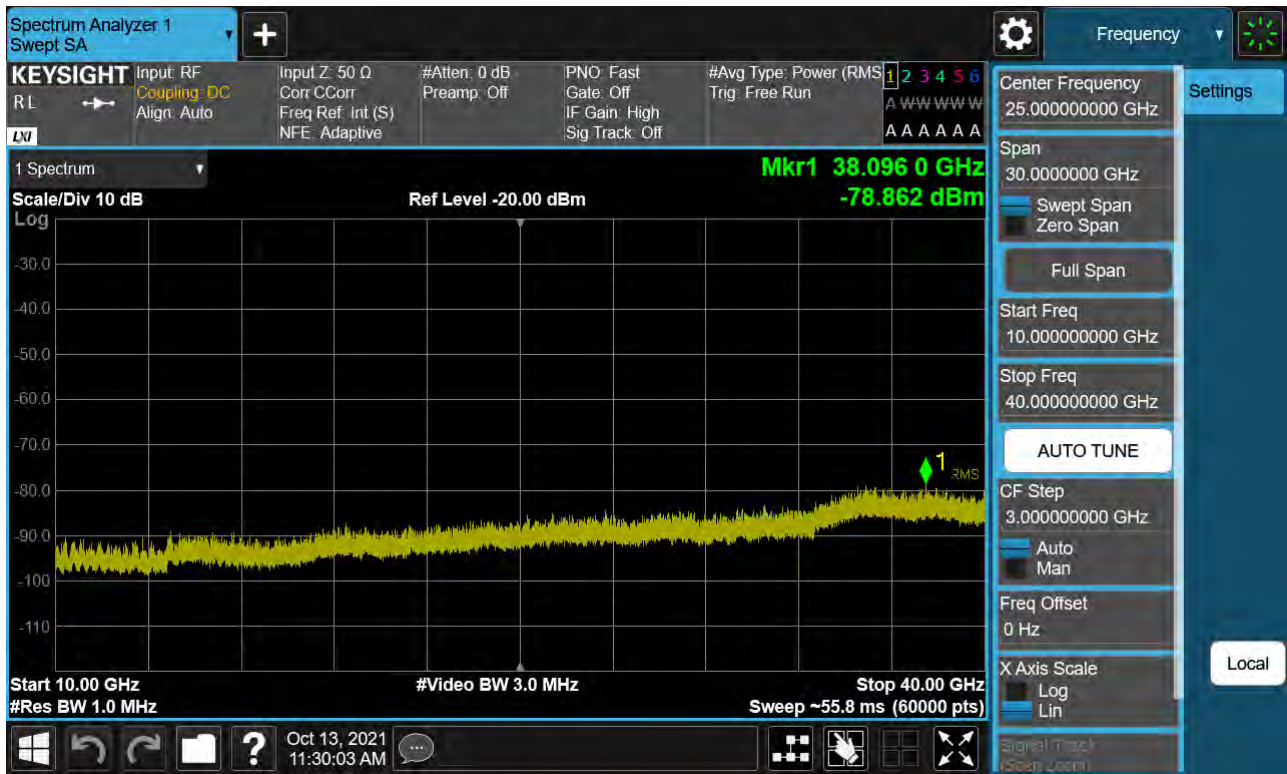
Sub6 n77. Conducted Spurious Plot_2 (633334ch_60 MHz_BPSK)
