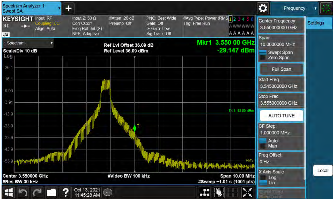
Sub6 n77. High Band Edge Plot (70 M BW Ch.634332 BPSK 1RB)(1)
