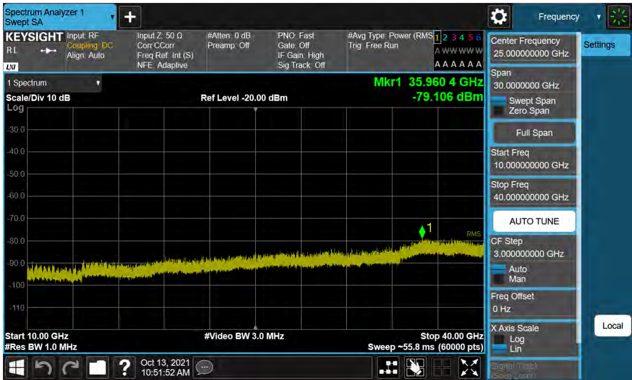
Sub6 n77. Conducted Spurious Plot_2 (633334ch_30 MHz_BPSK)
