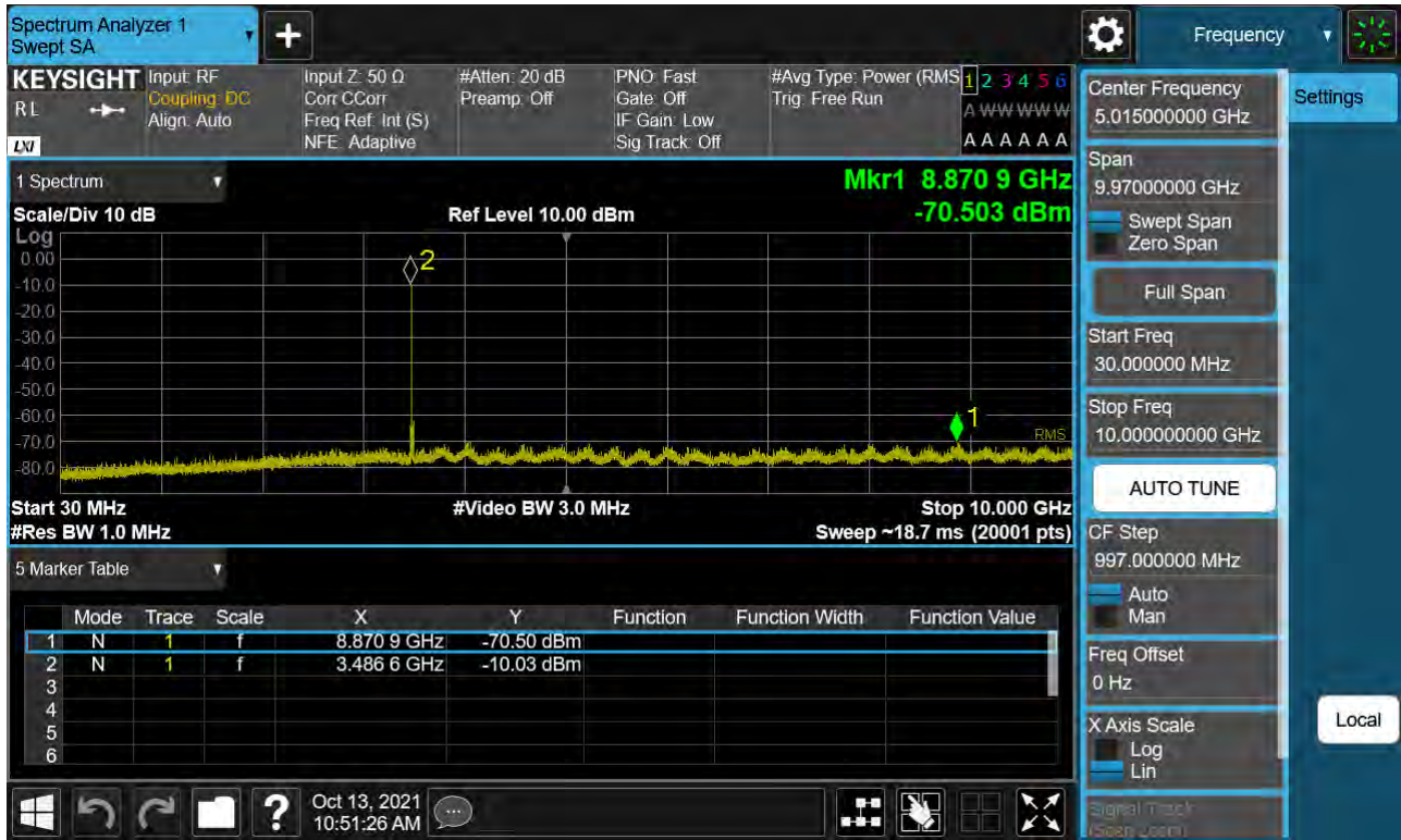
Sub6 n77. Conducted Spurious Plot_1 (633334ch_30 MHz_BPSK)
