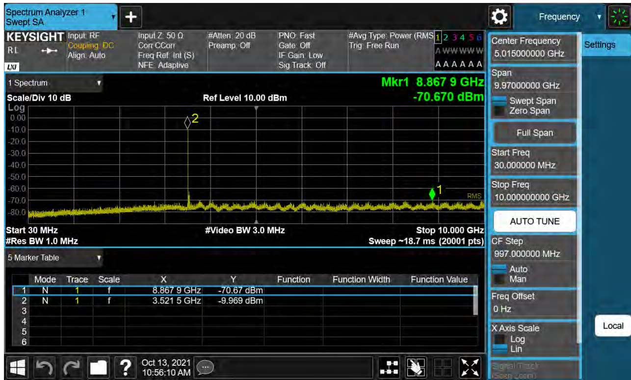
Sub6 n77. Conducted Spurious Plot_1 (635666ch_30 MHz_BPSK)
