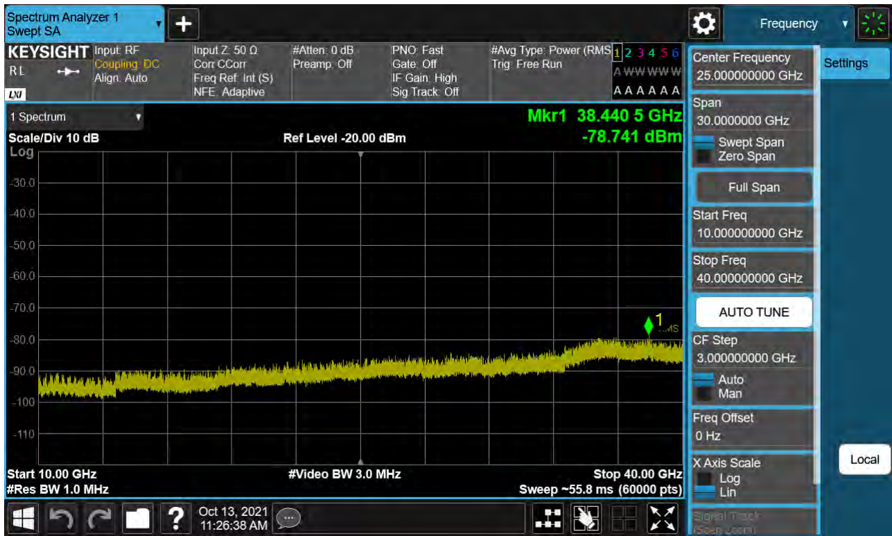
Sub6 n77. Conducted Spurious Plot_2 (632000ch_60 MHz_BPSK)
