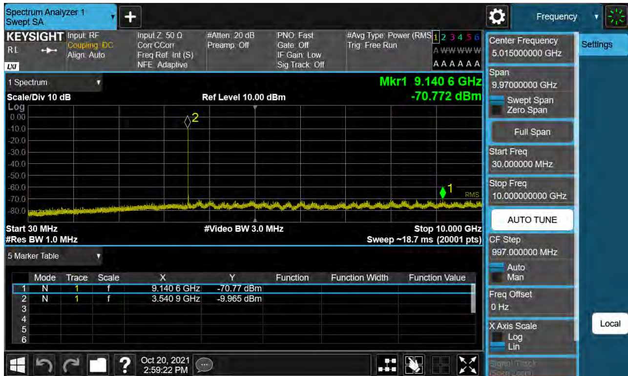
Sub6 n77. Conducted Spurious Plot_1 (636322ch_10 MHz_BPSK)
