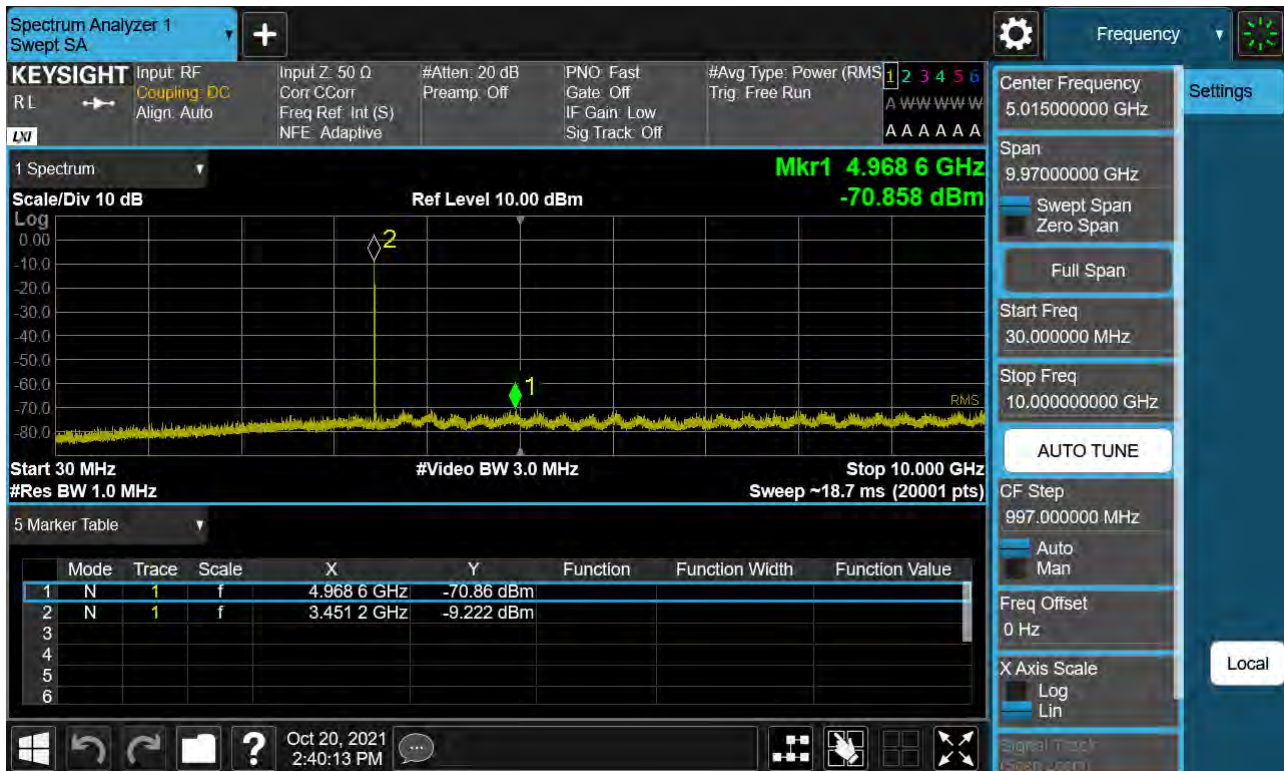
Sub6 n77. Conducted Spurious Plot_1 (630334ch_10 MHz_BPSK)
