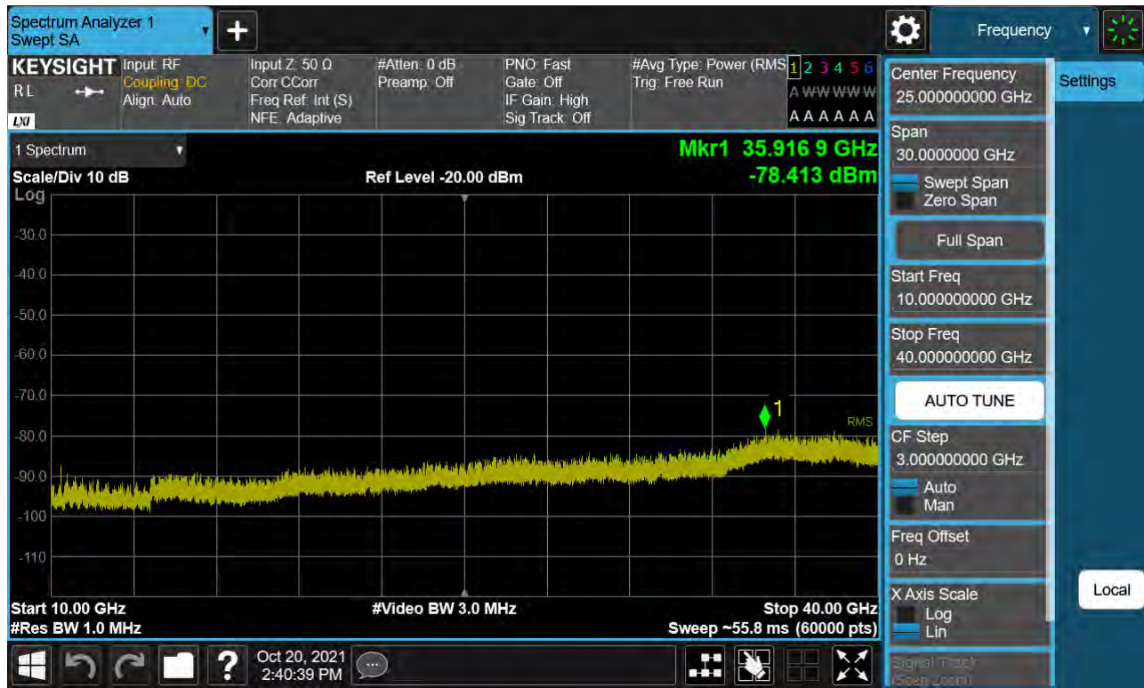
Sub6 n77. Conducted Spurious Plot_2 (630334ch_10 MHz_BPSK)
