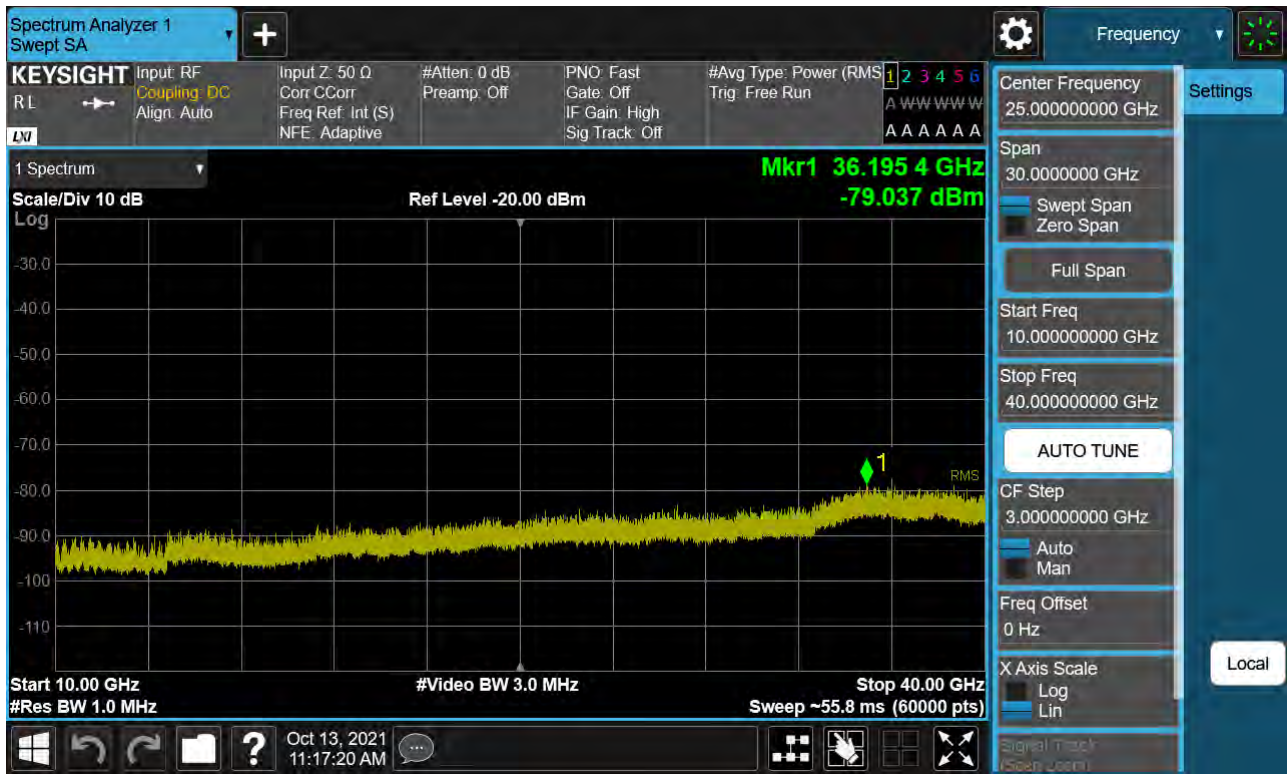
Sub6 n77. Conducted Spurious Plot_2 (633334ch_50 MHz_BPSK)
