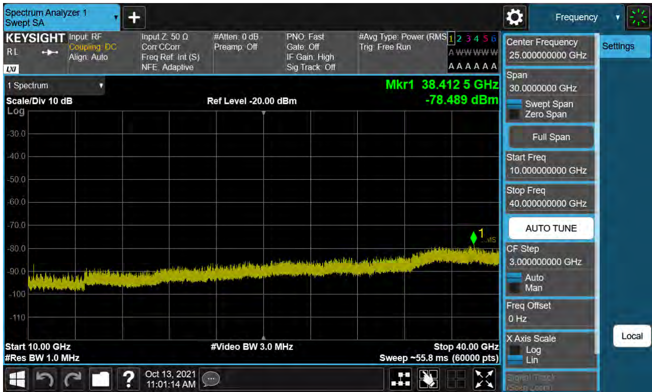
Sub6 n77. Conducted Spurious Plot_2 (631334ch_40 MHz_BPSK)
