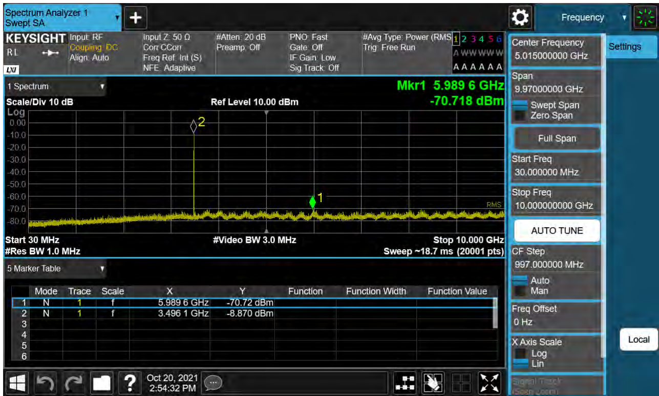
Sub6 n77. Conducted Spurious Plot_1 (633334ch_10 MHz_BPSK)
