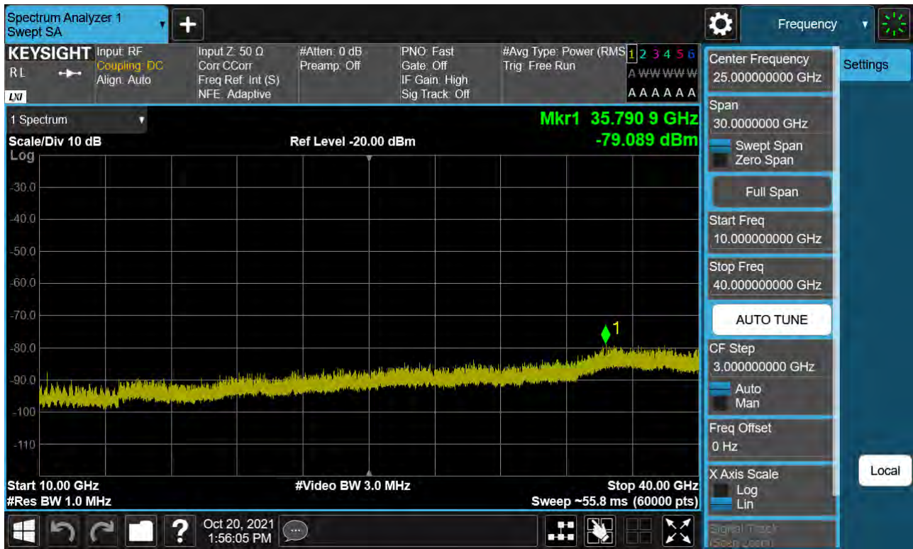
Sub6 n77. Conducted Spurious Plot_2 (630500ch_15 MHz_BPSK)
