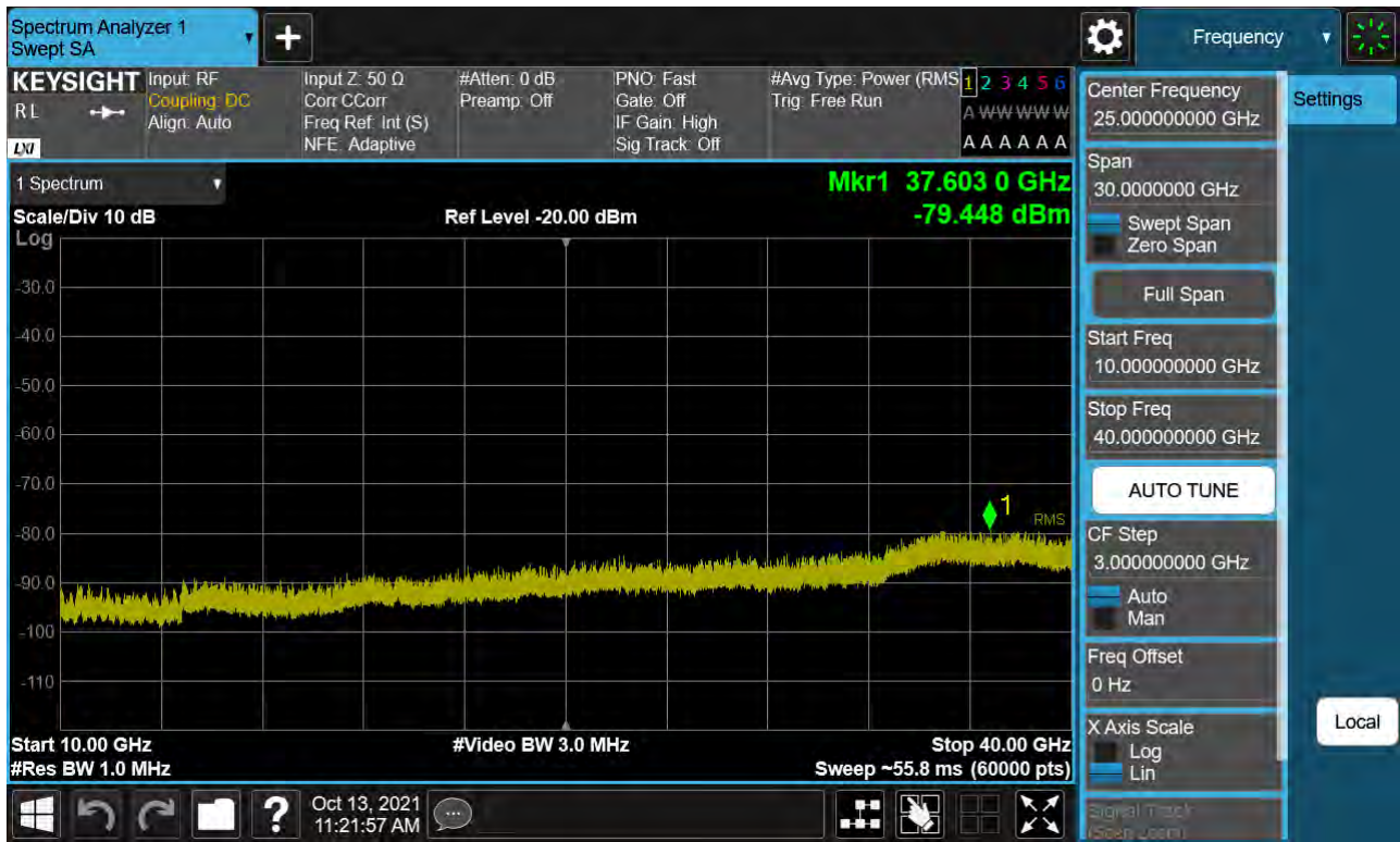
Sub6 n77. Conducted Spurious Plot_2 (635000ch_50 MHz_BPSK)
