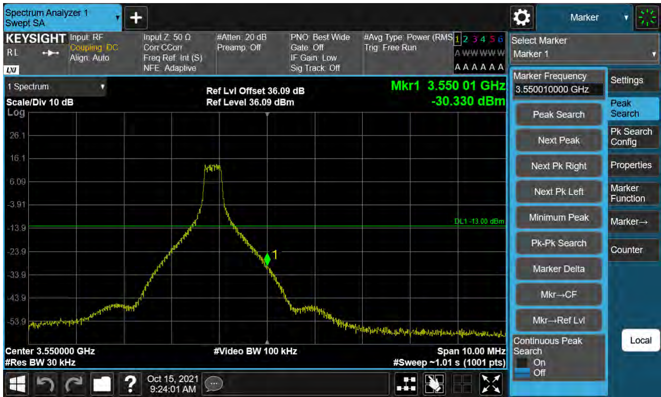
Sub6 n77. High Band Edge Plot (80 M BW Ch.634000 BPSK 1RB)(1)
