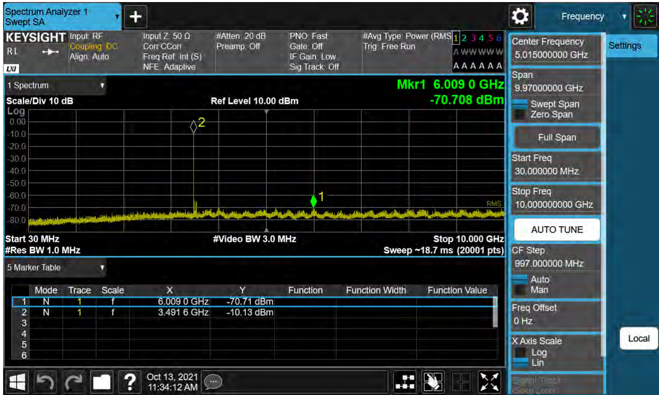
Sub6 n77. Conducted Spurious Plot_1 (634666ch_60 MHz_BPSK)
