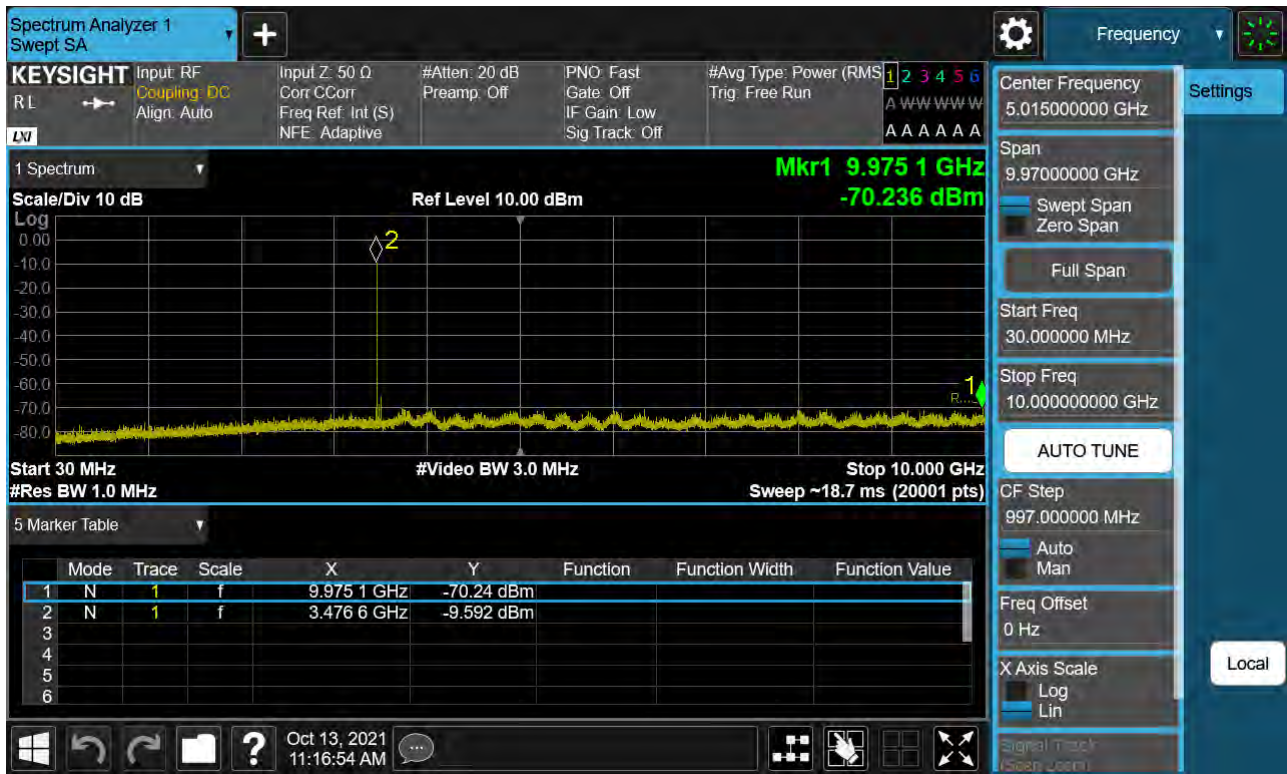
Sub6 n77. Conducted Spurious Plot_1 (633334ch_50 MHz_BPSK)
