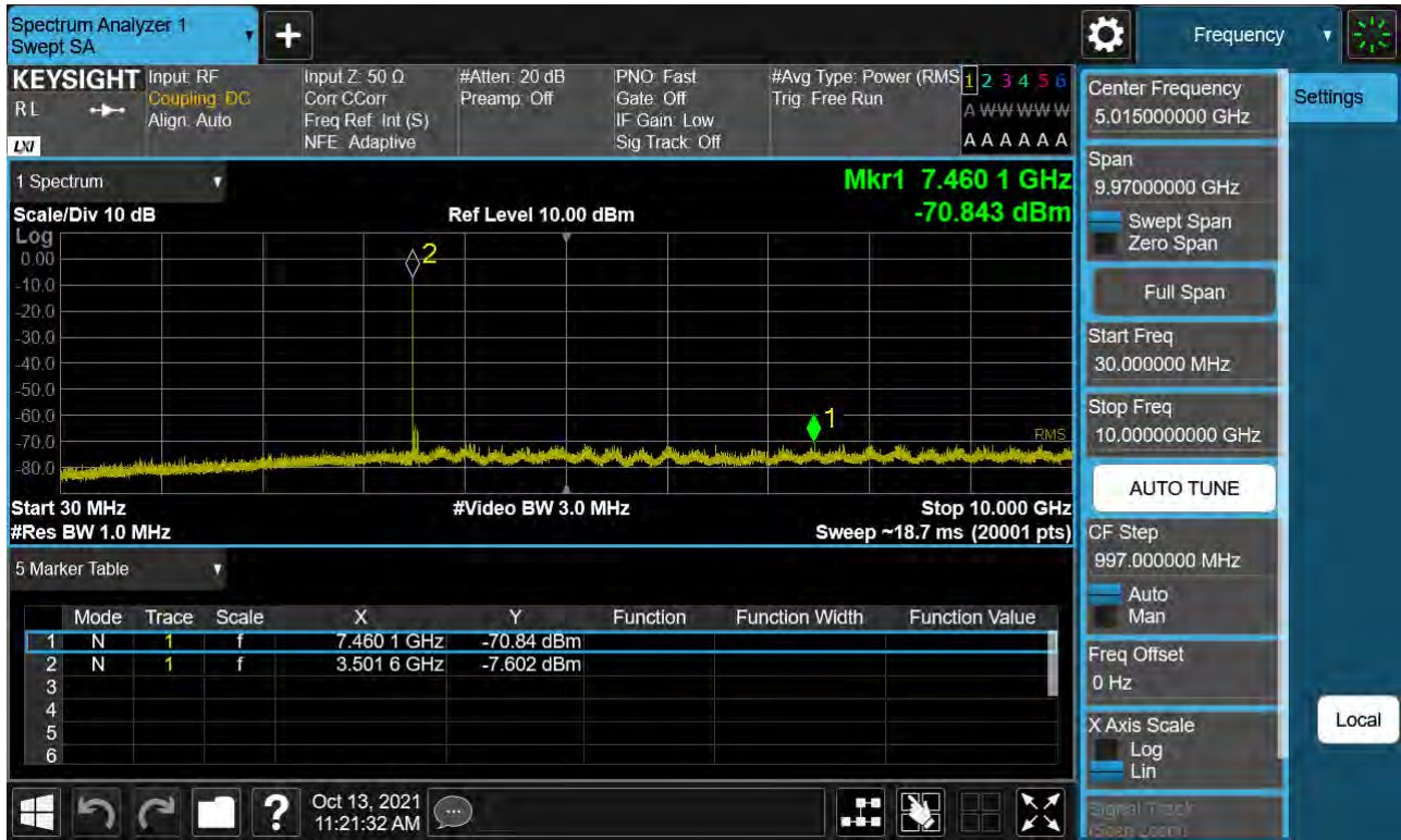
Sub6 n77. Conducted Spurious Plot_1 (635000ch_50 MHz_BPSK)
