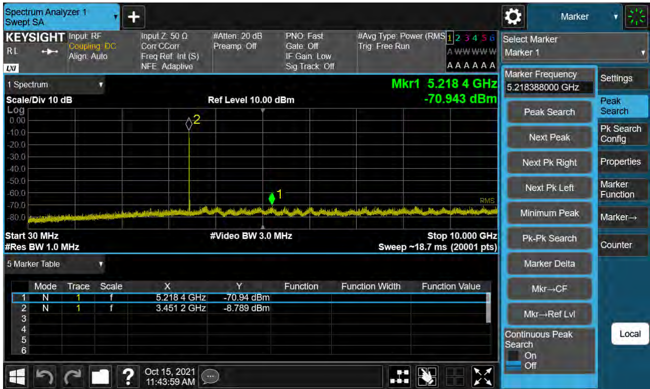
Sub6 n77. Conducted Spurious Plot_1 (630668ch_20 MHz_BPSK)
