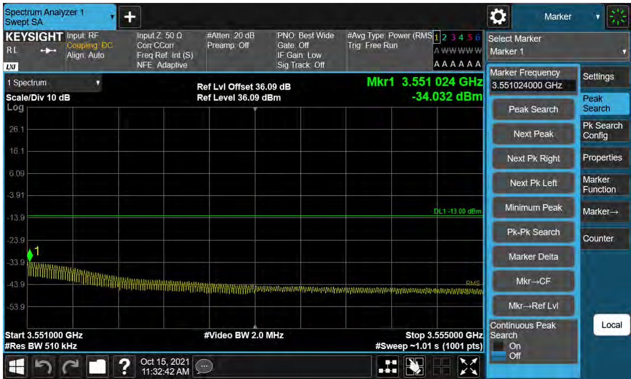
Sub6 n77. High Band Edge Plot (100 M BW Ch.633334 BPSK 1RB)(2)
