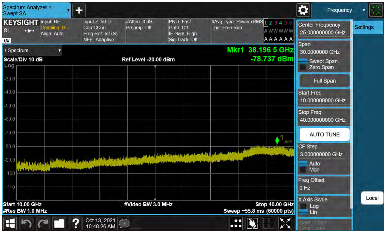
Sub6 n77. Conducted Spurious Plot_2 (631000ch_30 MHz_BPSK)
