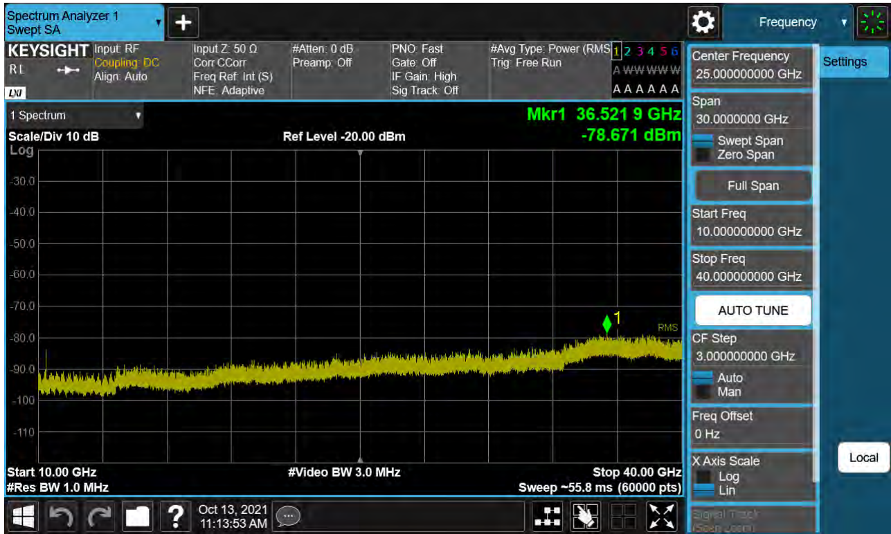
Sub6 n77. Conducted Spurious Plot_2 (631668ch_50 MHz_BPSK)
