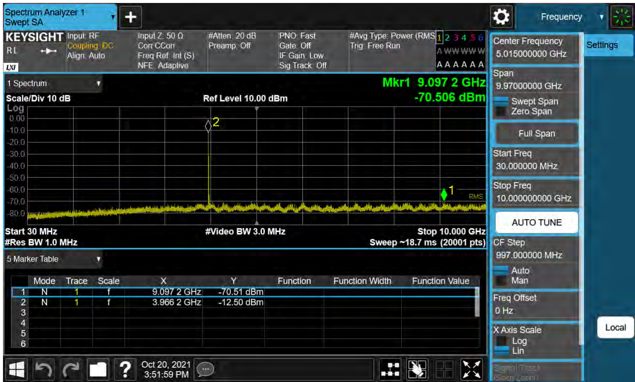
Sub6 n77. Conducted Spurious Plot_1 (664832ch_15 MHz_BPSK)
