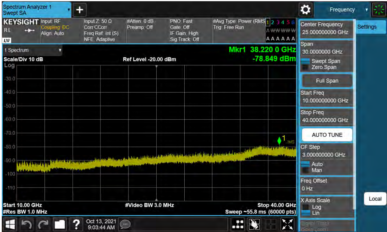
Sub6 n77. Conducted Spurious Plot_2 (648334ch_50 MHz_BPSK)
