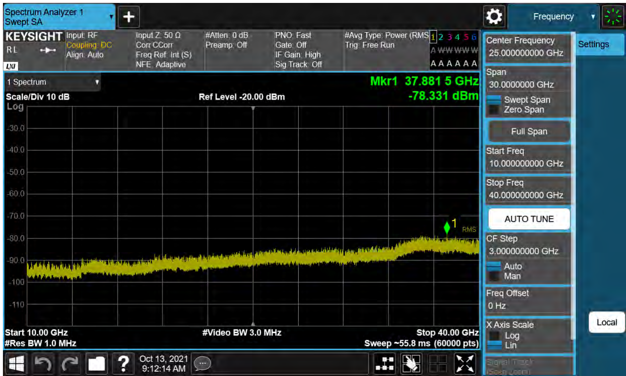
Sub6 n77. Conducted Spurious Plot_2 (663666ch_50 MHz_BPSK)
