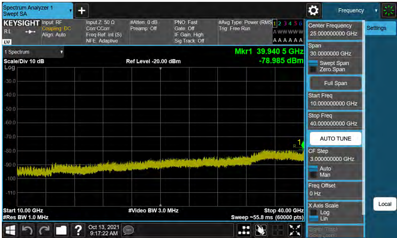
Sub6 n77. Conducted Spurious Plot_2 (648668ch_60 MHz_BPSK)
