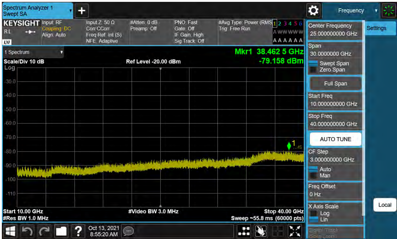
Sub6 n77. Conducted Spurious Plot_2 (664000ch_40 MHz_BPSK)
