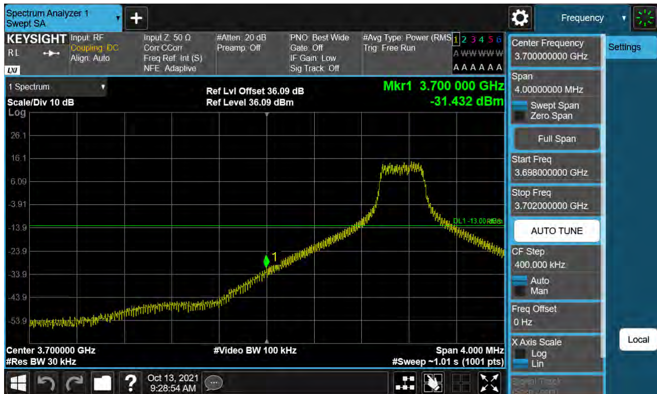
Sub6 n77. Low Band Edge Plot (70 M BW Ch.649000 BPSK 1RB)(1)
