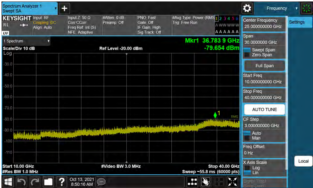
Sub6 n77. Conducted Spurious Plot_2 (656000ch_40 MHz_BPSK)
