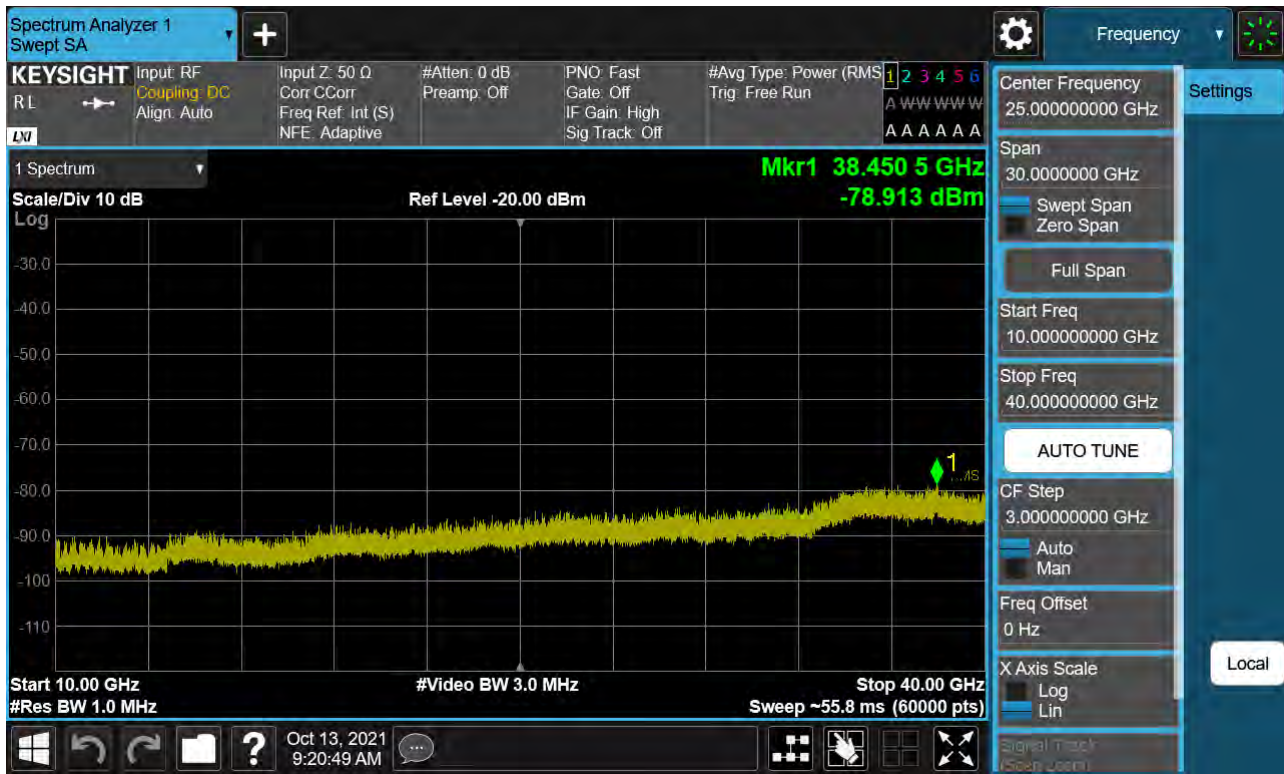
Sub6 n77. Conducted Spurious Plot_2 (656000ch_60 MHz_BPSK)
