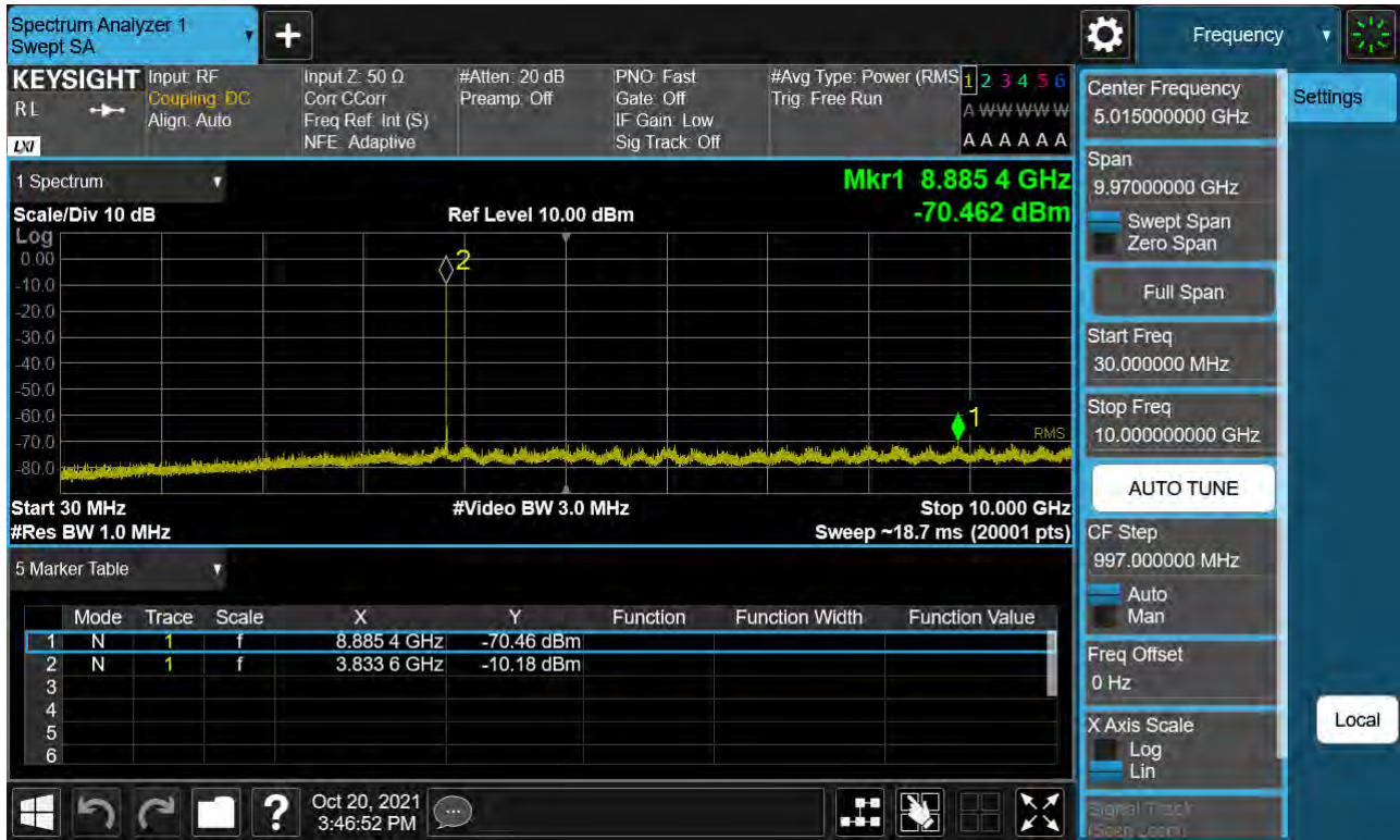
Sub6 n77. Conducted Spurious Plot_1 (656000ch_15 MHz_BPSK)
