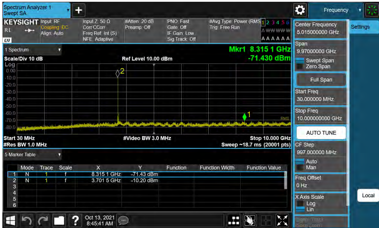
Sub6 n77. Conducted Spurious Plot_1 (648000ch_40 MHz_BPSK)
