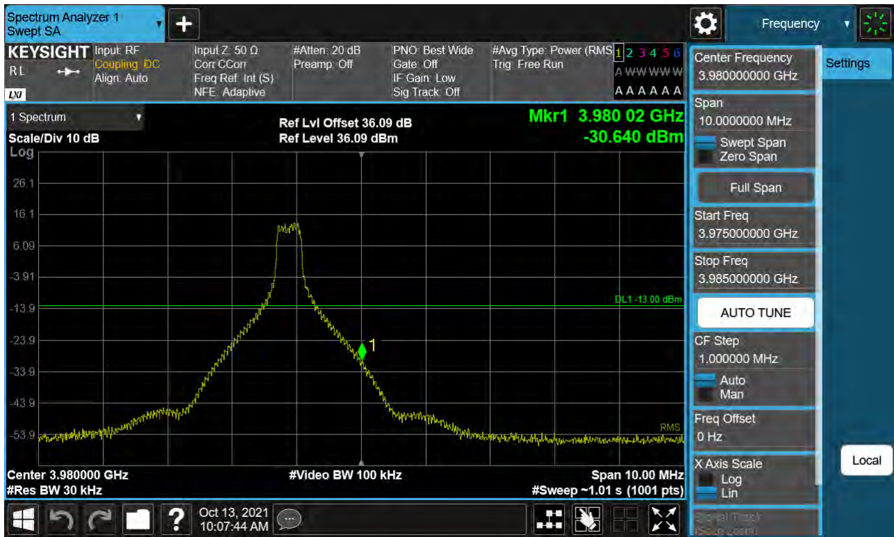
Sub6 n77. High Band Edge Plot (90 M BW Ch.662332 BPSK 1RB)(1)
