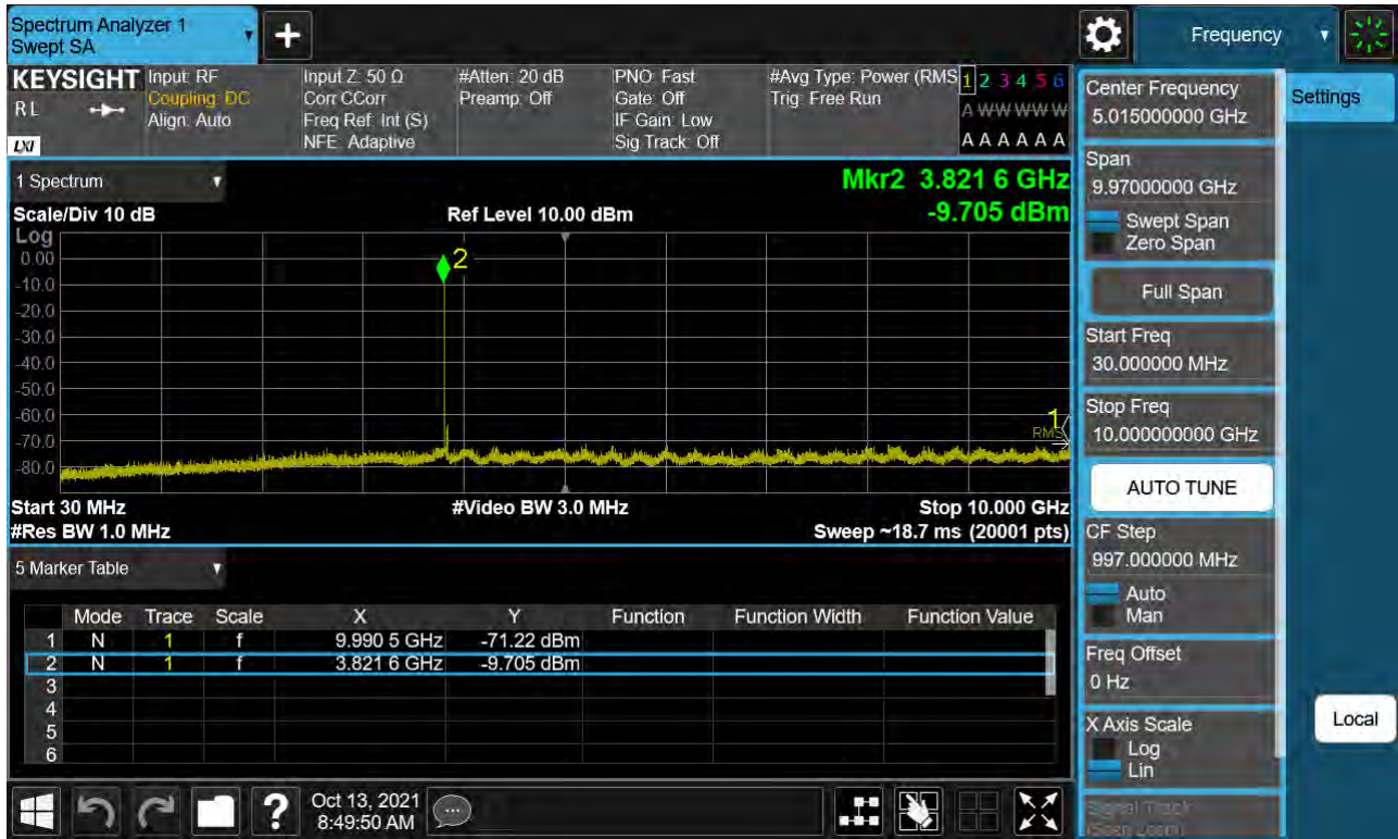
Sub6 n77. Conducted Spurious Plot_1 (656000ch_40 MHz_BPSK)
