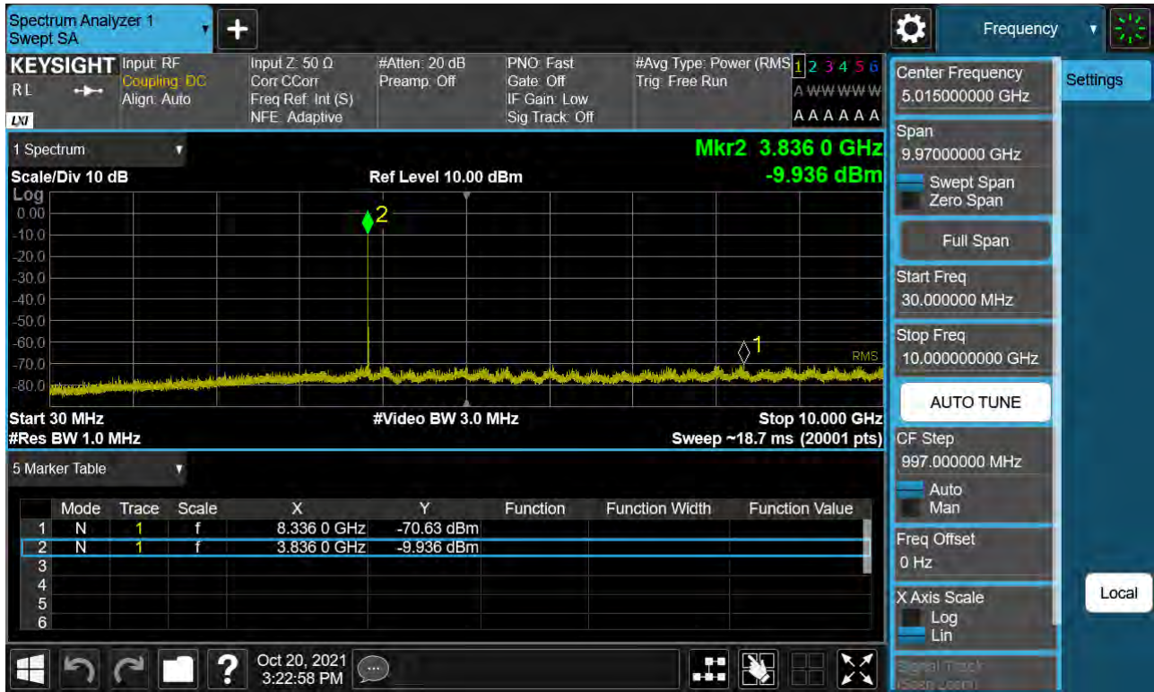
Sub6 n77. Conducted Spurious Plot_1 (656000ch_10 MHz_BPSK)
