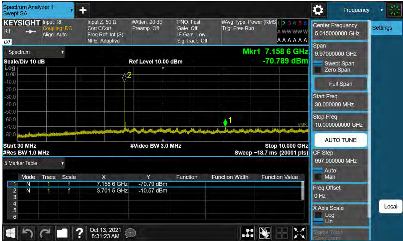
Sub6 n77. Conducted Spurious Plot_1 (647668ch_30 MHz_BPSK)
