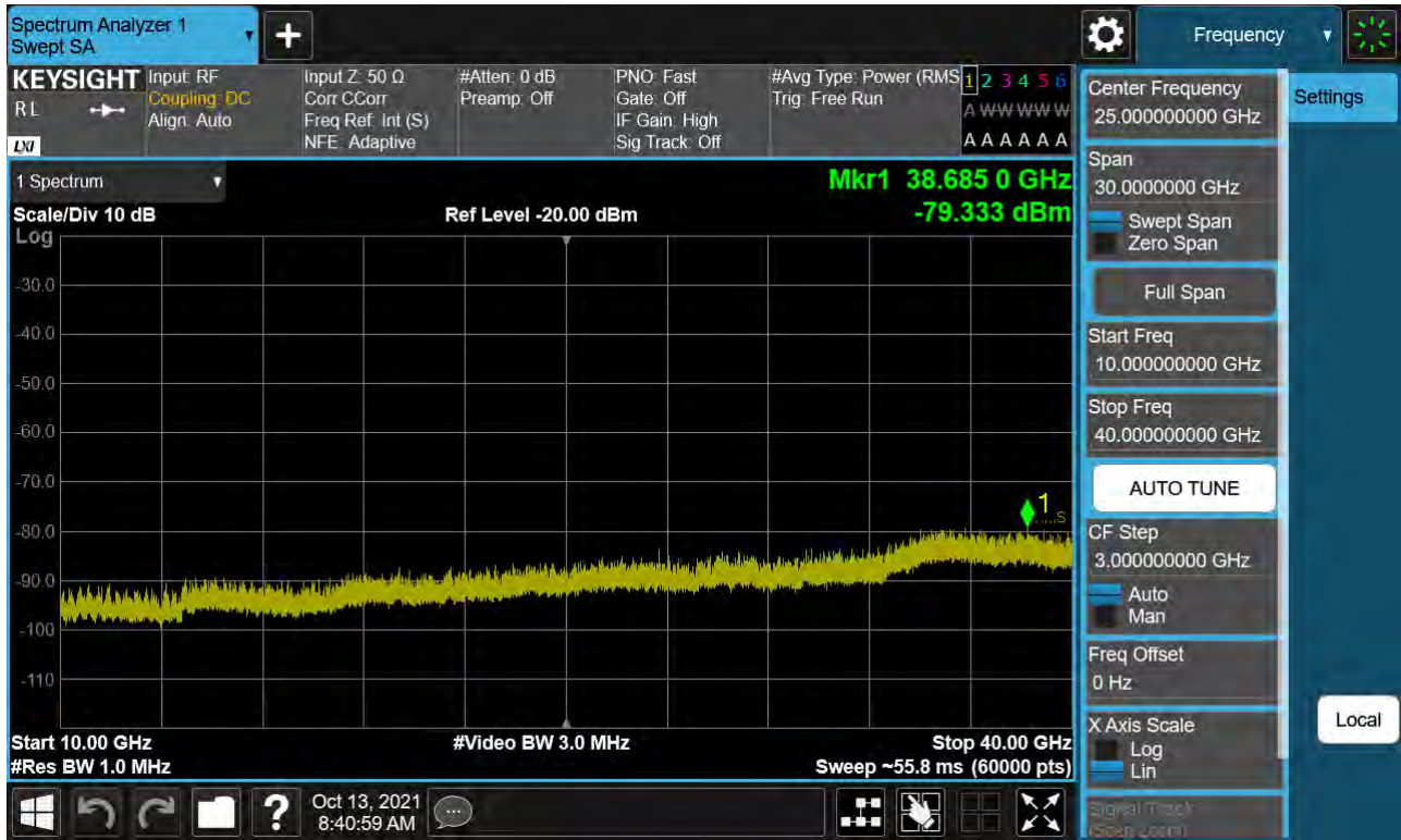
Sub6 n77. Conducted Spurious Plot_2 (664332ch_30 MHz_BPSK)
