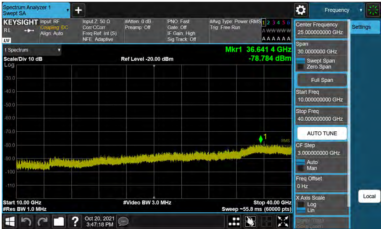
Sub6 n77. Conducted Spurious Plot_2 (656000ch_15 MHz_BPSK)
