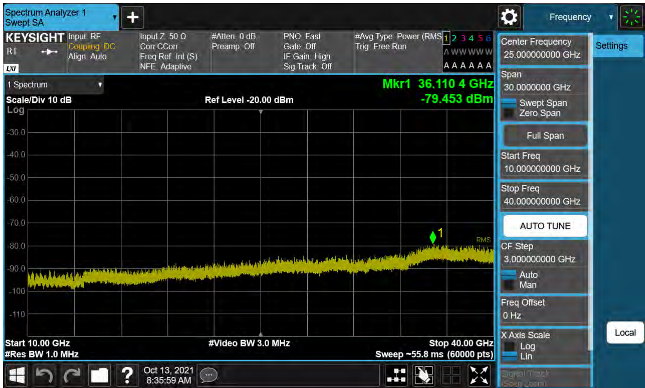
Sub6 n77. Conducted Spurious Plot_2 (656000ch_30 MHz_BPSK)
