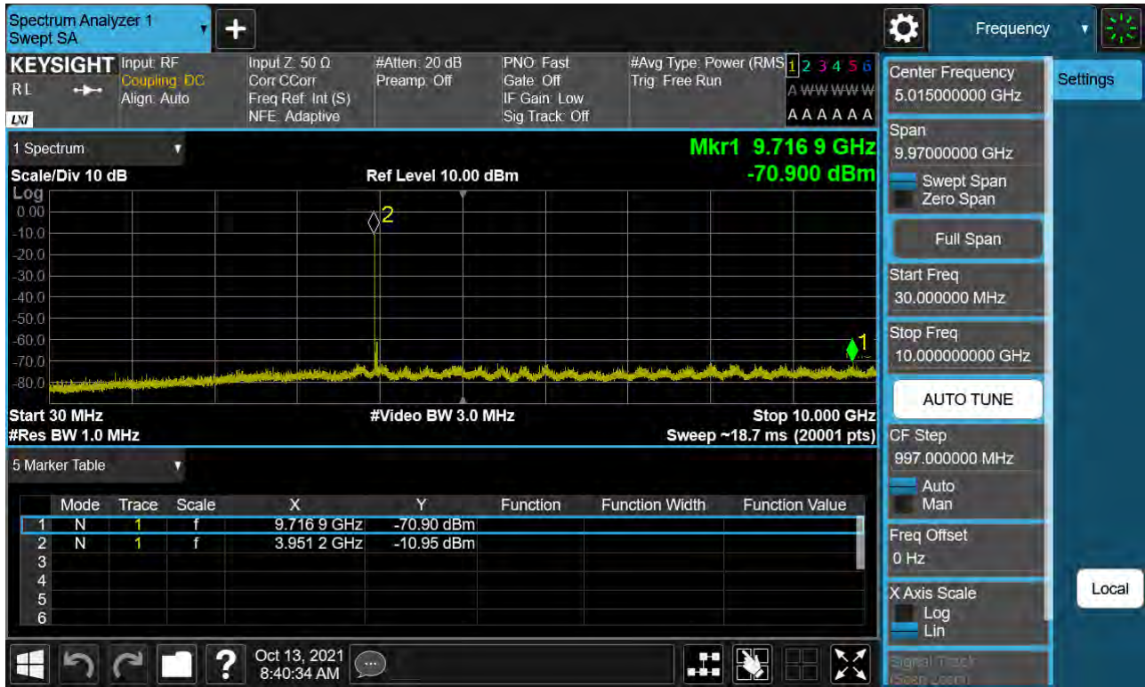
Sub6 n77. Conducted Spurious Plot_1 (664332ch_30 MHz_BPSK)
