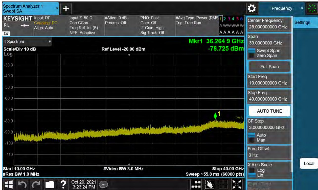
Sub6 n77. Conducted Spurious Plot_2 (656000ch_10 MHz_BPSK)
