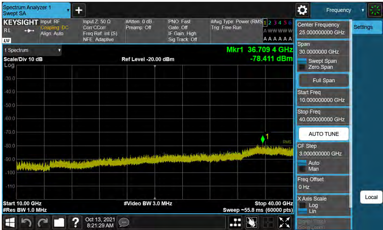
Sub6 n77. Conducted Spurious Plot_2 (664666ch_20 MHz_BPSK)
