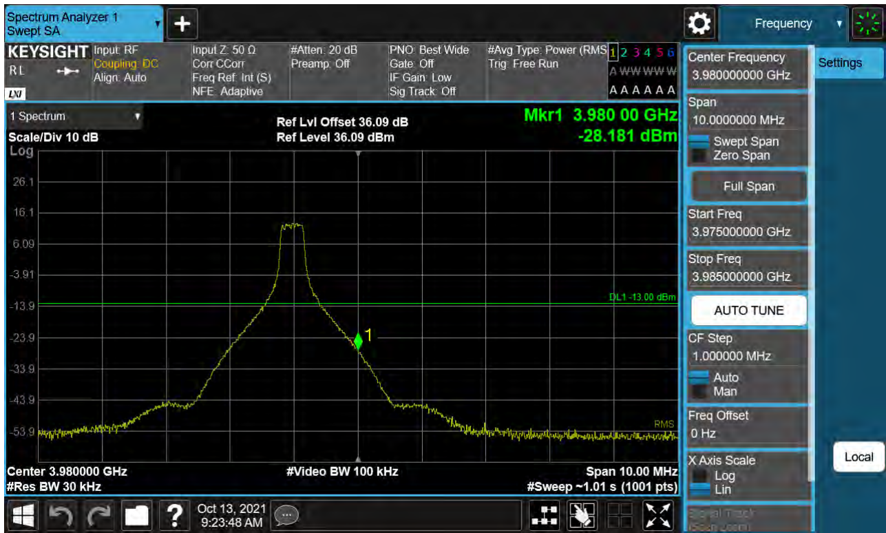
Sub6 n77. High Band Edge Plot (60 M BW Ch.663332 BPSK 1RB)(1)
