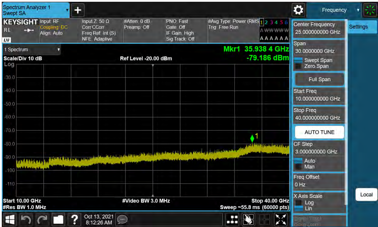
Sub6 n77. Conducted Spurious Plot_2 (647334ch_20 MHz_BPSK)
