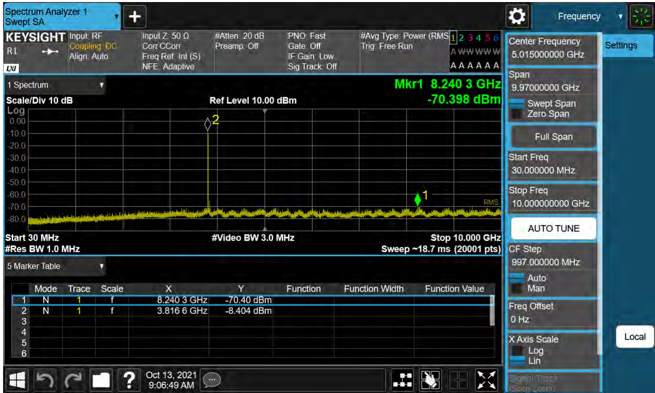
Sub6 n77. Conducted Spurious Plot_1 (656000ch_50 MHz_BPSK)
