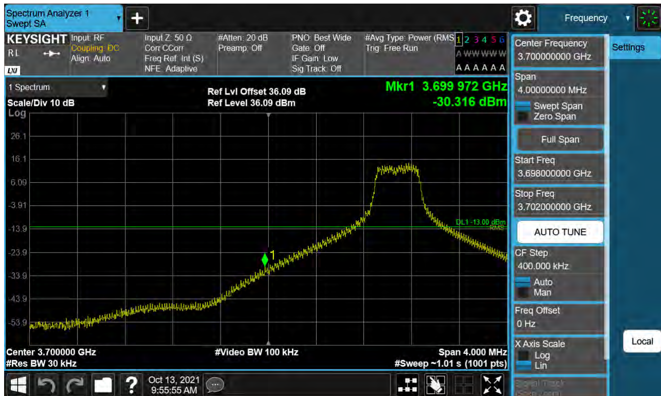
Sub6 n77. Low Band Edge Plot (90 M BW Ch.649668 BPSK 1RB)(1)
