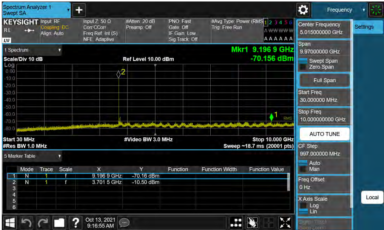
Sub6 n77. Conducted Spurious Plot_1 (648668ch_60 MHz_BPSK)
