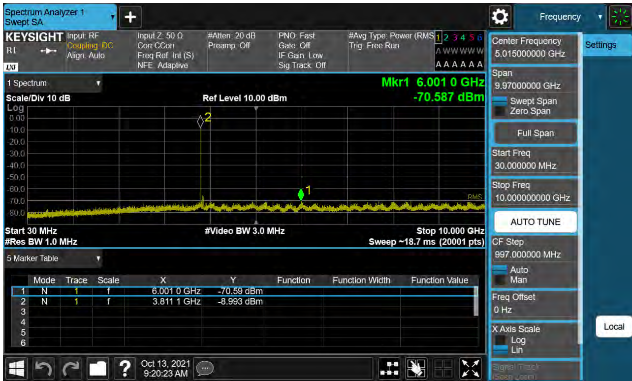
Sub6 n77. Conducted Spurious Plot_1 (656000ch_60 MHz_BPSK)
