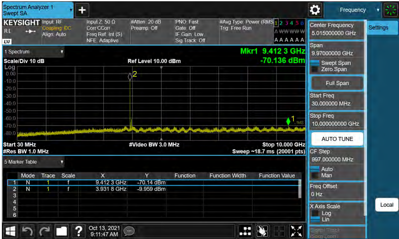
Sub6 n77. Conducted Spurious Plot_1 (663666ch_50 MHz_BPSK)
