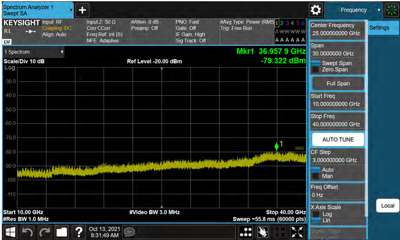
Sub6 n77. Conducted Spurious Plot_2 (647668ch_30 MHz_BPSK)
