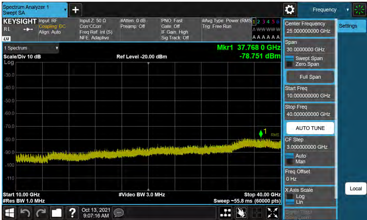
Sub6 n77. Conducted Spurious Plot_2 (656000ch_50 MHz_BPSK)
