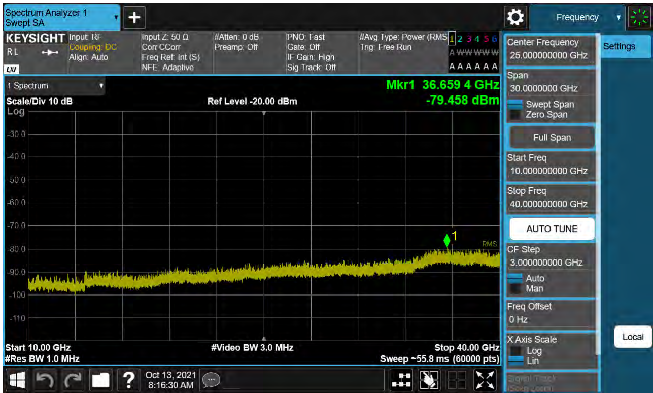
Sub6 n77. Conducted Spurious Plot_2 (656000ch_20 MHz_BPSK)
