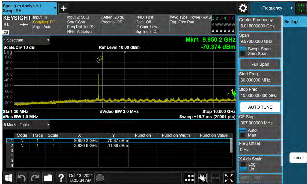
Sub6 n77. Conducted Spurious Plot_1 (656000ch_30 MHz_BPSK)
