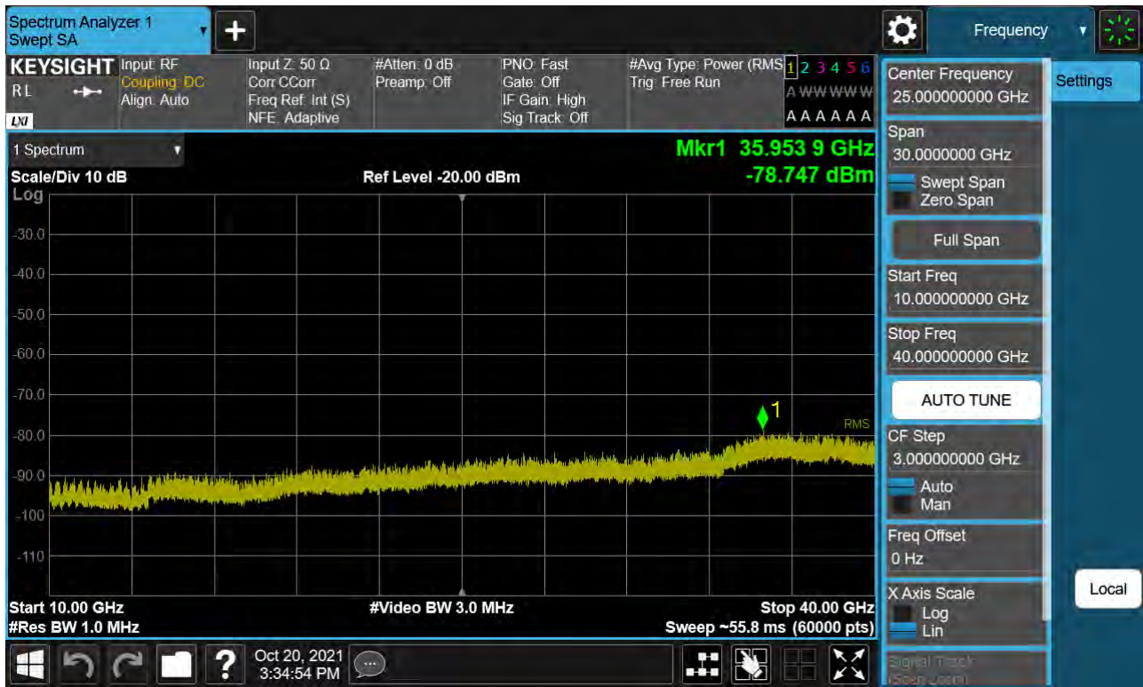
Sub6 n77. Conducted Spurious Plot_2 (665000ch_10 MHz_BPSK)
