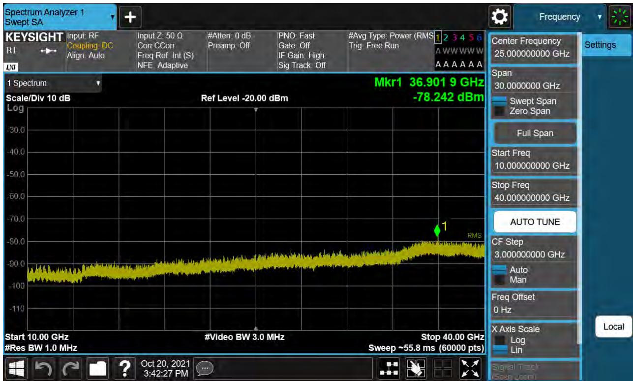
Sub6 n77. Conducted Spurious Plot_2 (647168ch_15 MHz_BPSK)
