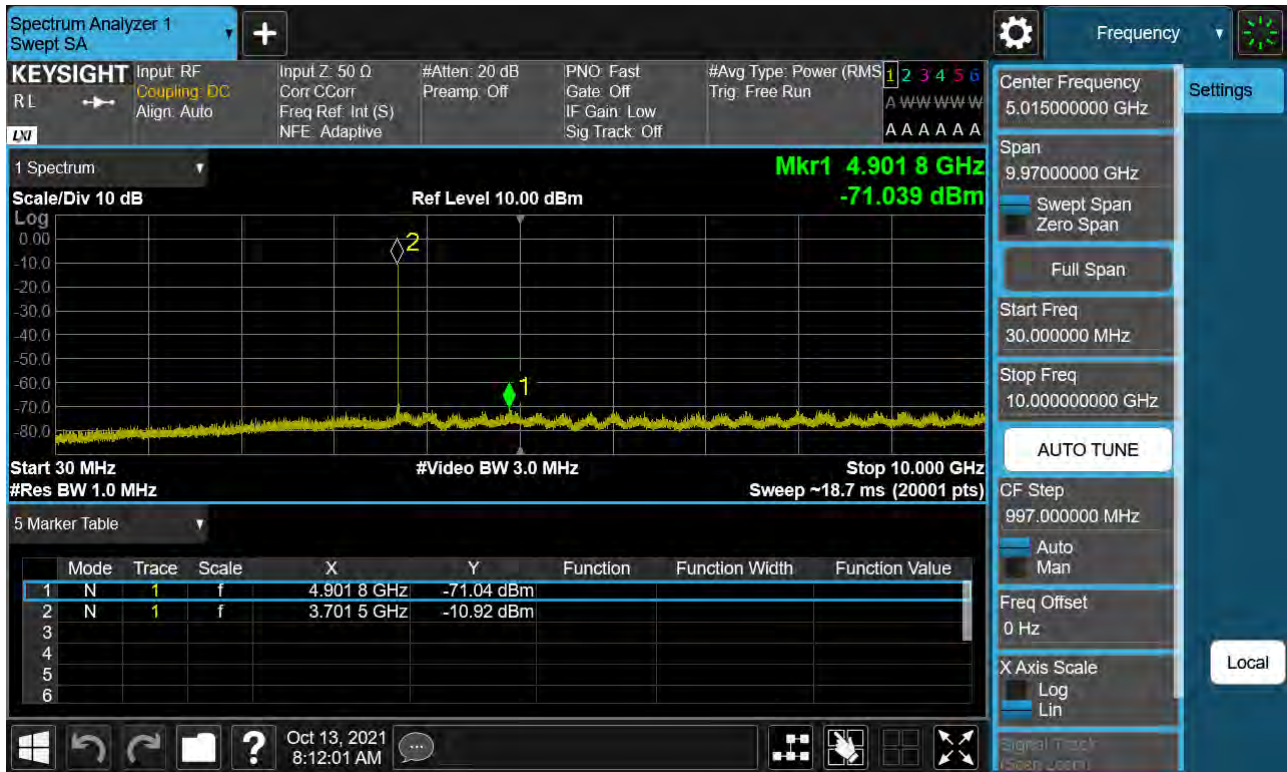
Sub6 n77. Conducted Spurious Plot_1 (647334ch_20 MHz_BPSK)
