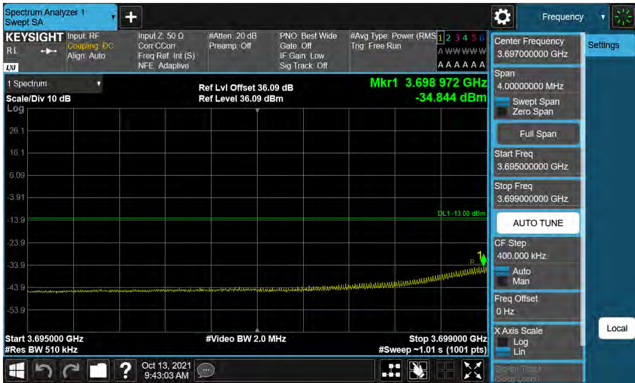
Sub6 n77. Low Band Edge Plot (80 M BW Ch.649334 BPSK 1RB)(2)
