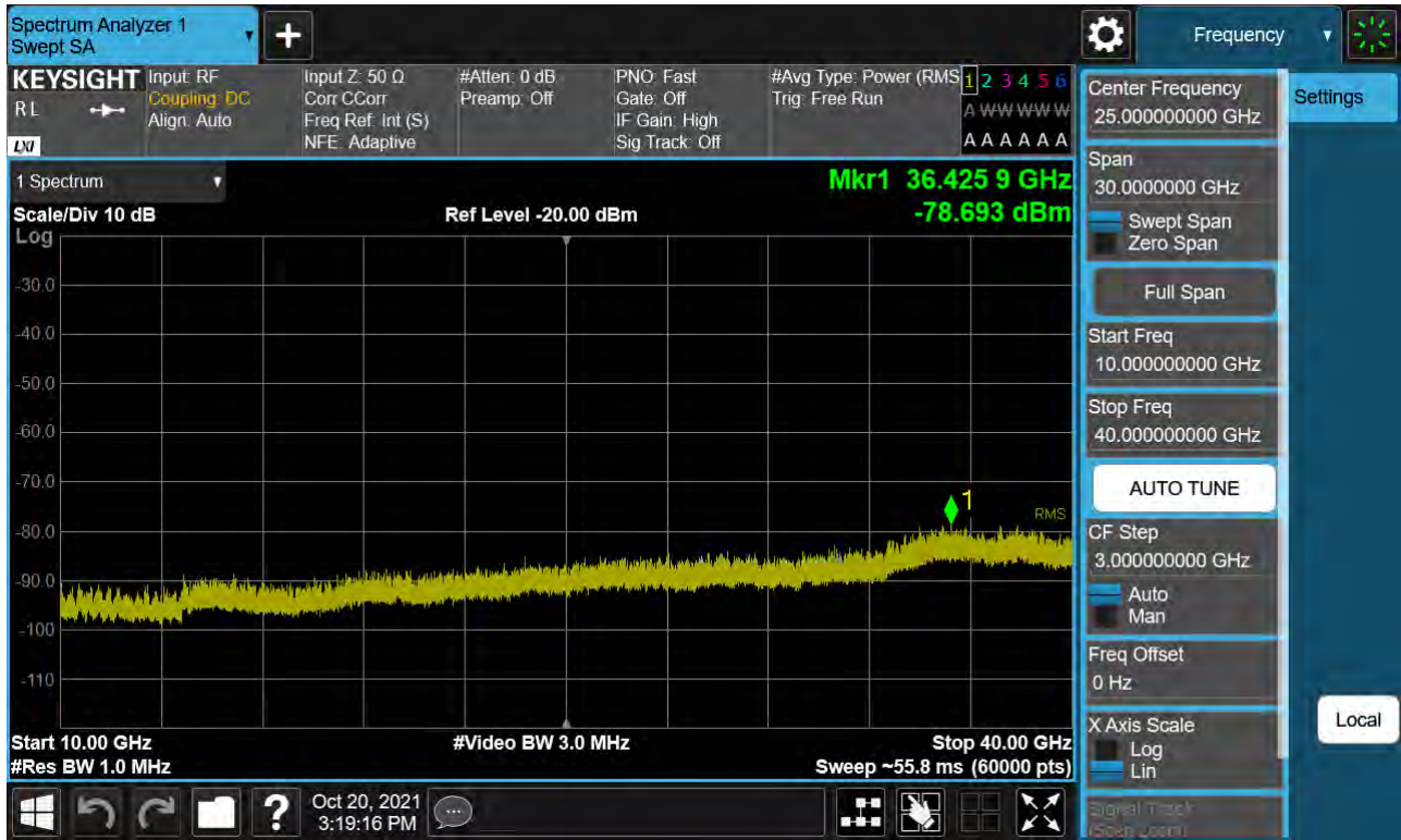
Sub6 n77. Conducted Spurious Plot_2 (647000ch_10 MHz_BPSK)
