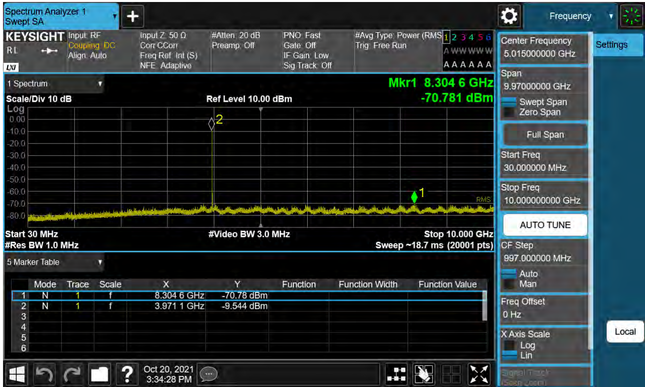
Sub6 n77. Conducted Spurious Plot_1 (665000ch_10 MHz_BPSK)
