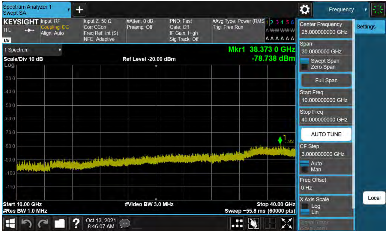
Sub6 n77. Conducted Spurious Plot_2 (648000ch_40 MHz_BPSK)
