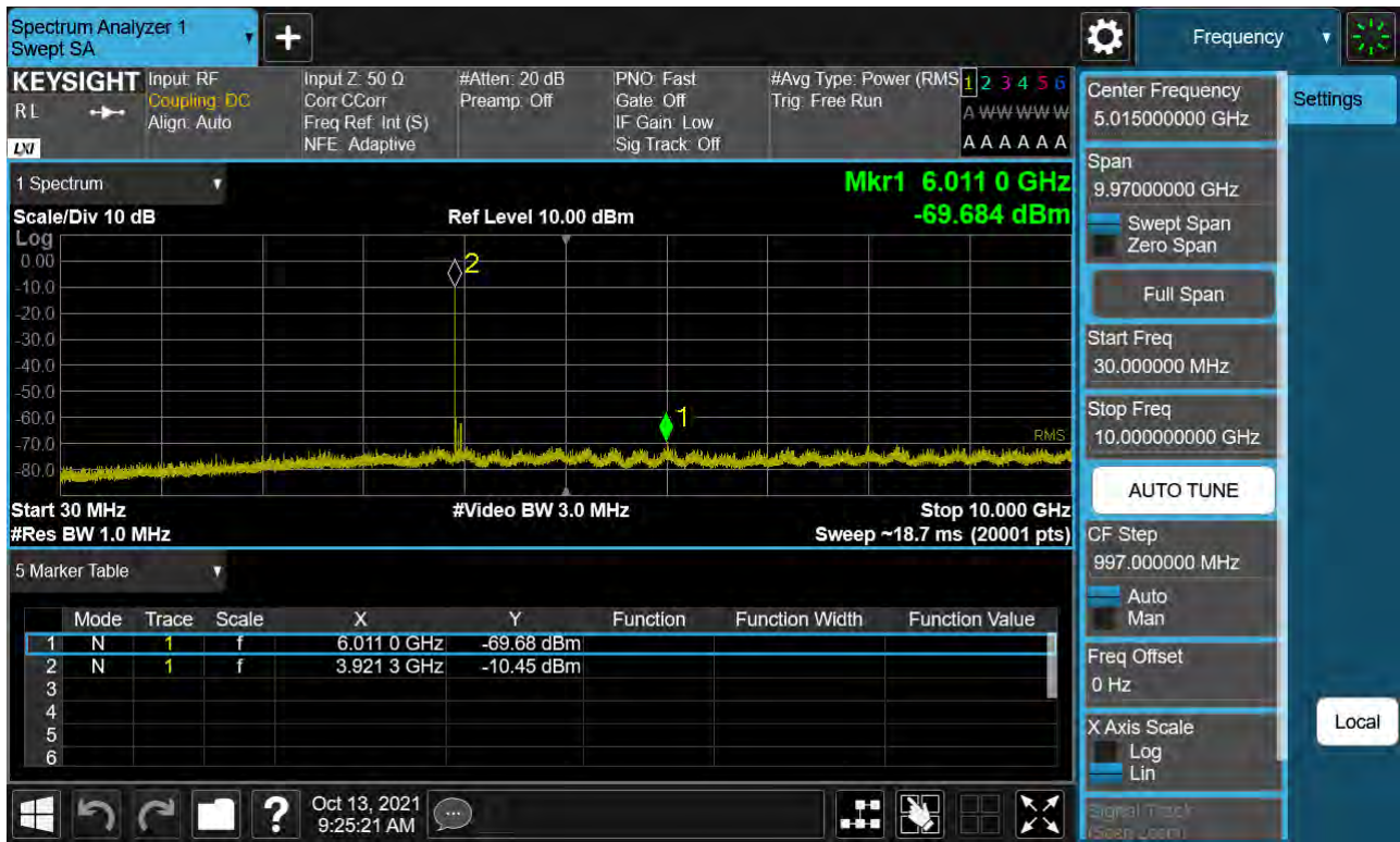
Sub6 n77. Conducted Spurious Plot_1 (663332ch_60 MHz_BPSK)
