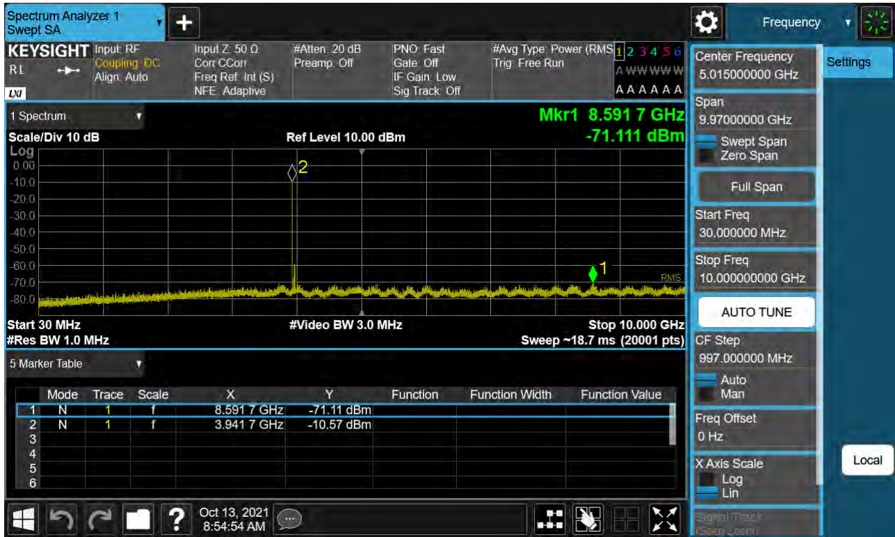
Sub6 n77. Conducted Spurious Plot_1 (664000ch_40 MHz_BPSK)
