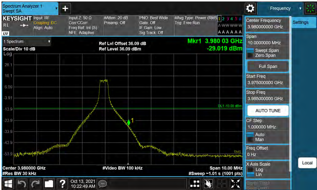
Sub6 n77. High Band Edge Plot (100 M BW Ch.662000 BPSK 1RB)(1)
