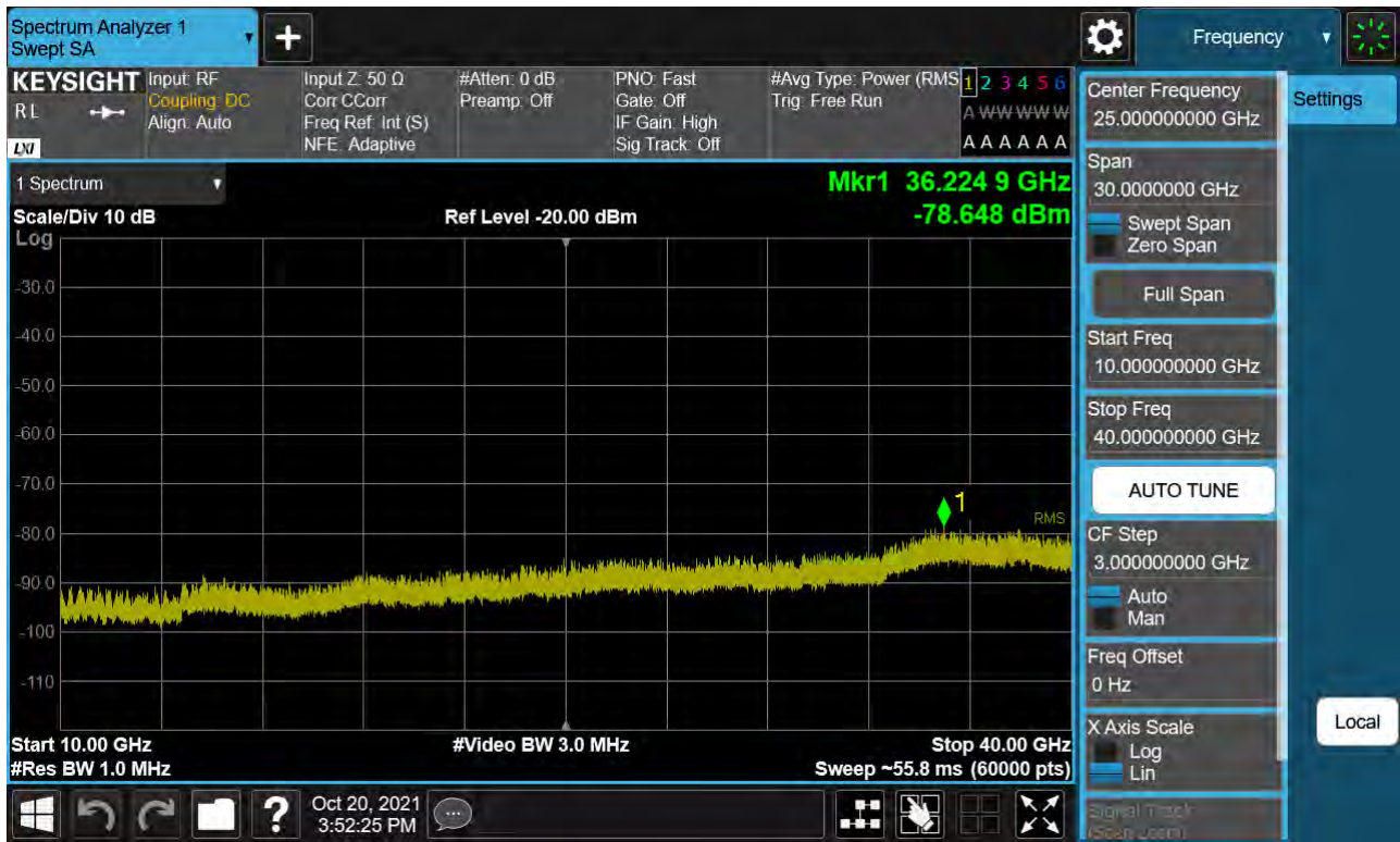
Sub6 n77. Conducted Spurious Plot_2 (664832ch_15 MHz_BPSK)
