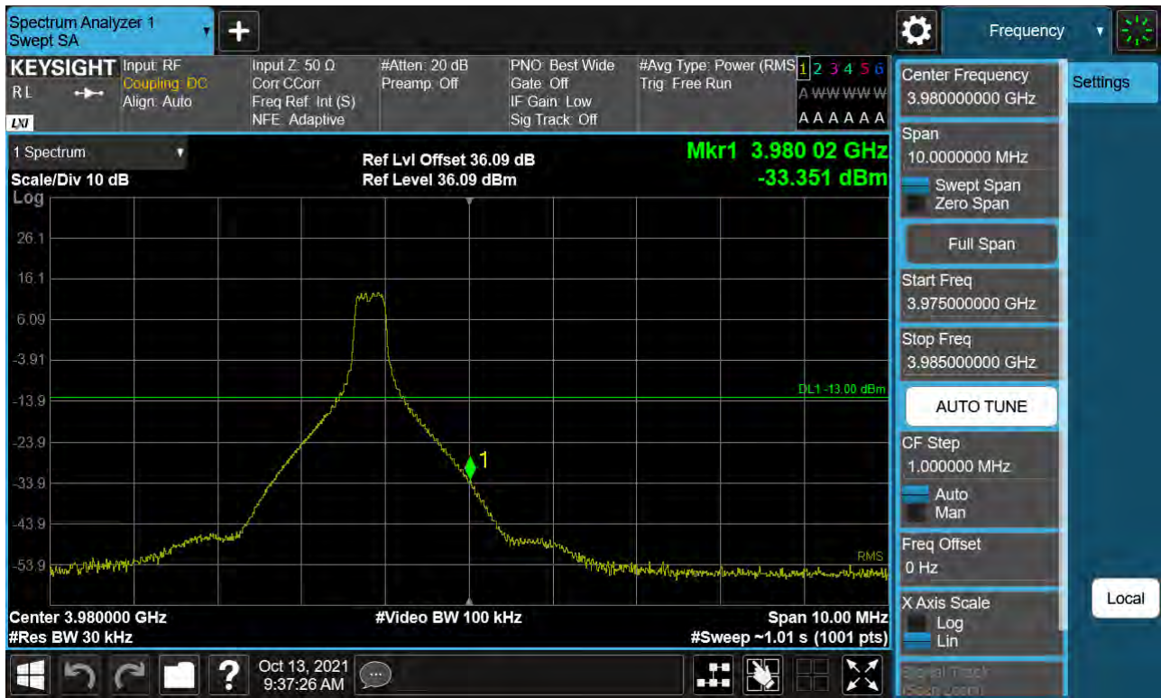
Sub6 n77. High Band Edge Plot (70 M BW Ch.663000 BPSK 1RB)(1)
