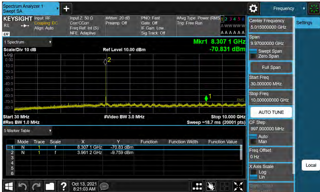
Sub6 n77. Conducted Spurious Plot_1 (664666ch_20 MHz_BPSK)
