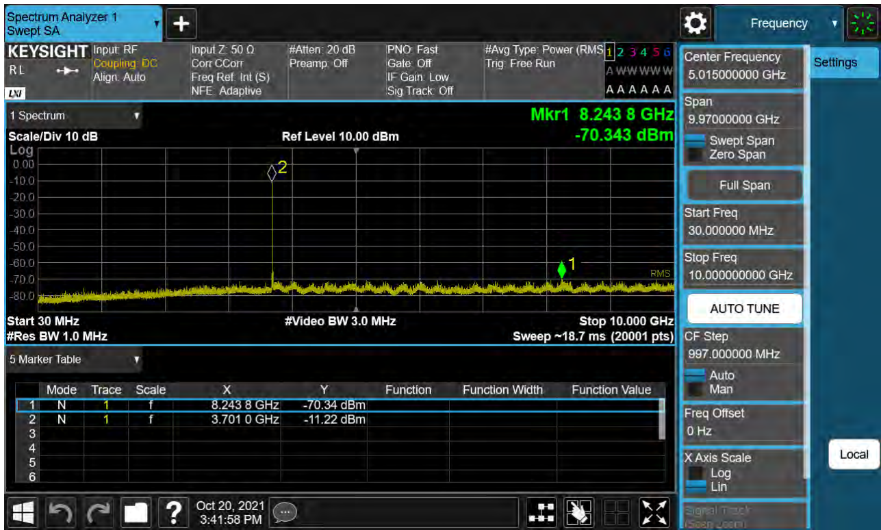
Sub6 n77. Conducted Spurious Plot_1 (647168ch_15 MHz_BPSK)
