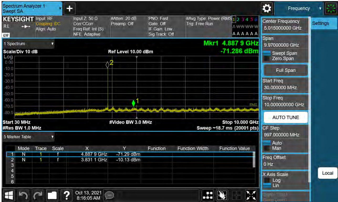
Sub6 n77. Conducted Spurious Plot_1 (656000ch_20 MHz_BPSK)
