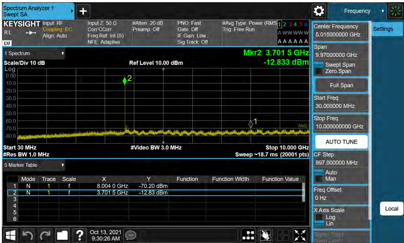
Sub6 n77. Conducted Spurious Plot_1 (649000ch_70 MHz_BPSK)
