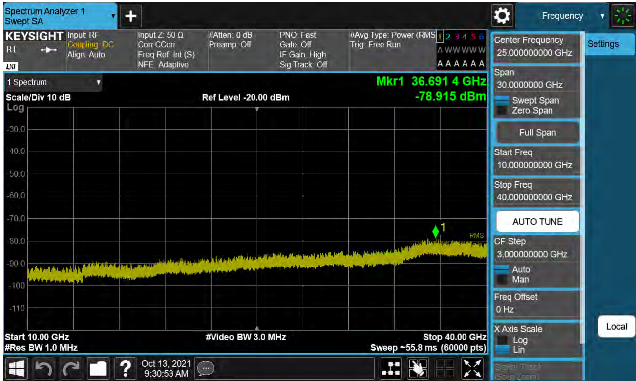
Sub6 n77. Conducted Spurious Plot_2 (649000ch_70 MHz_BPSK)
