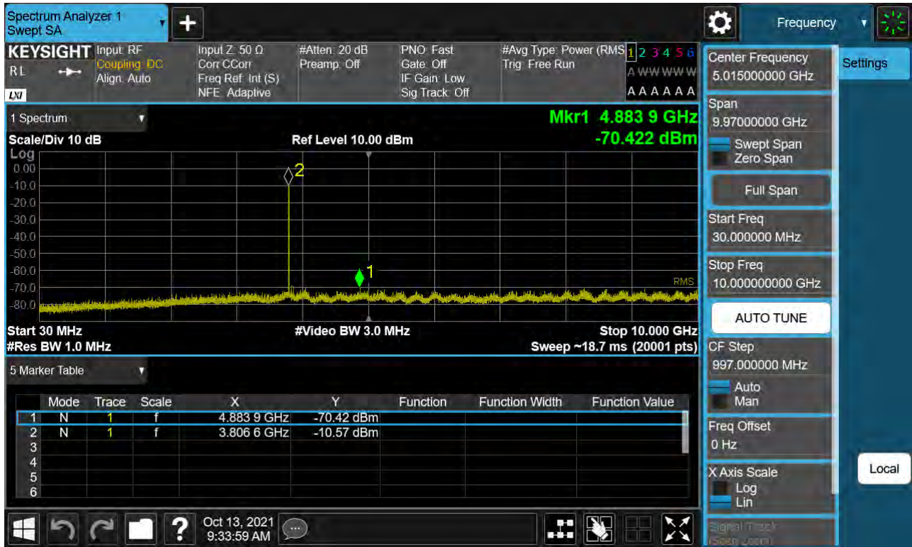
Sub6 n77. Conducted Spurious Plot_1 (656000ch_70 MHz_BPSK)
