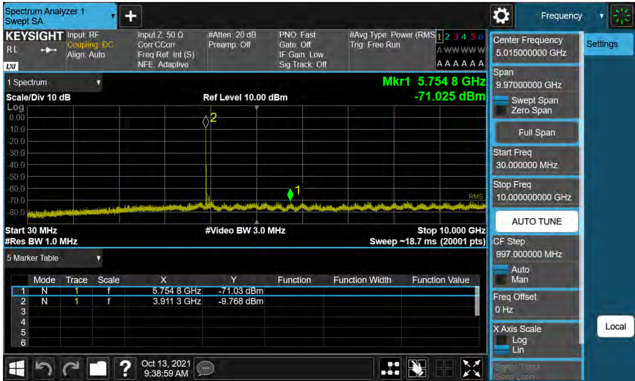
Sub6 n77. Conducted Spurious Plot_1 (663000ch_70 MHz_BPSK)
