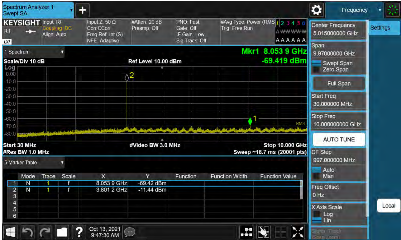
Sub6 n77. Conducted Spurious Plot_1 (656000ch_80 MHz_BPSK)
