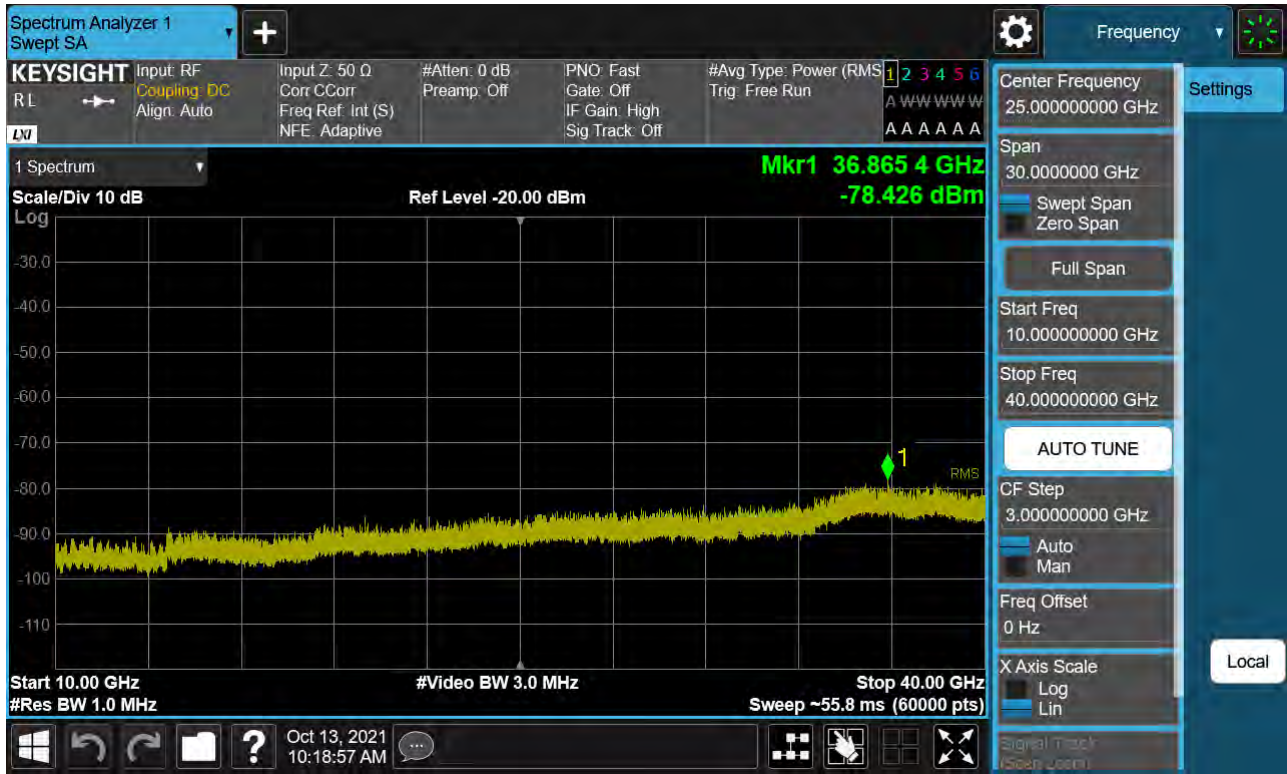
Sub6 n77. Conducted Spurious Plot_2 (656000ch_100 MHz_BPSK)
