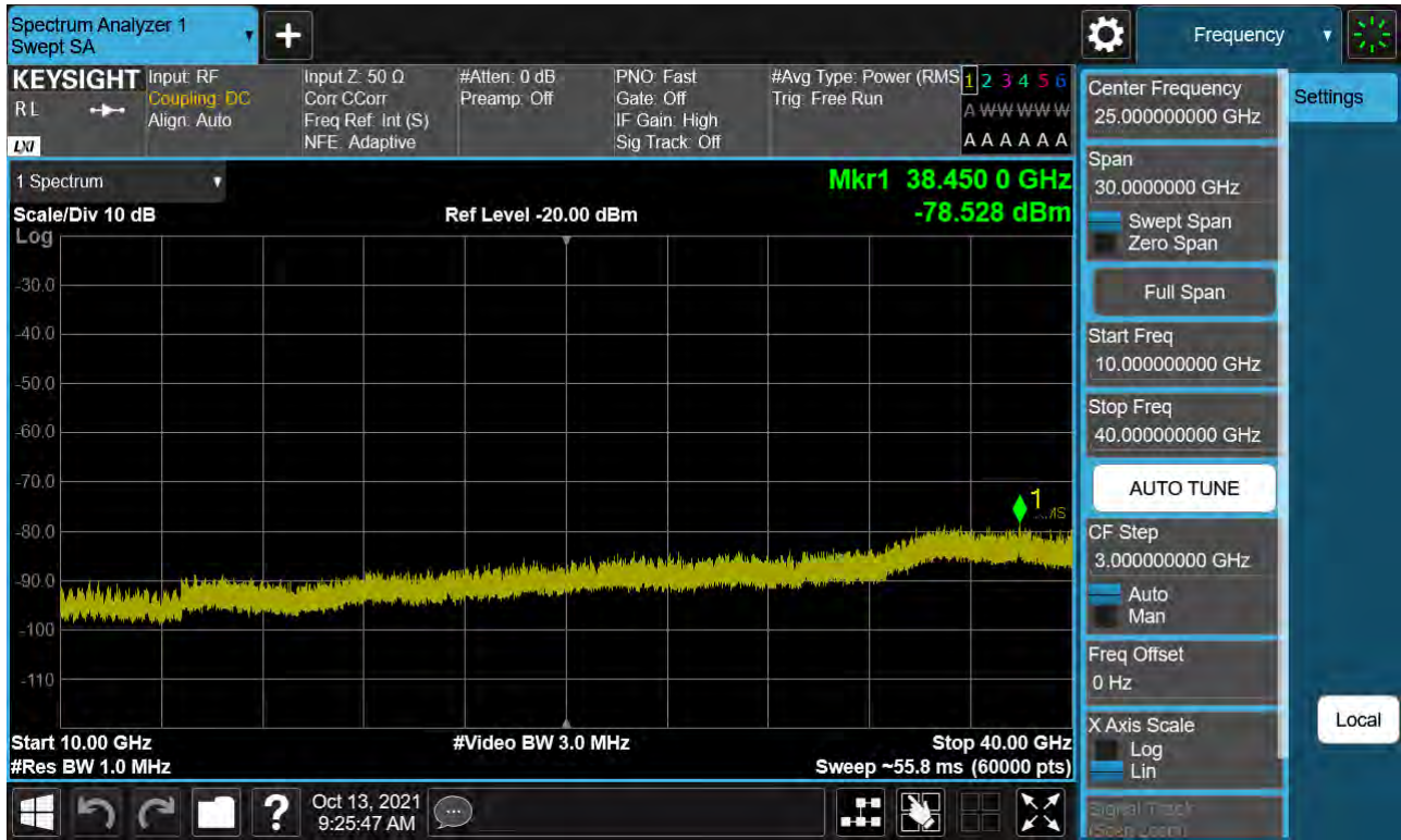
Sub6 n77. Conducted Spurious Plot_2 (663332ch_60 MHz_BPSK)
