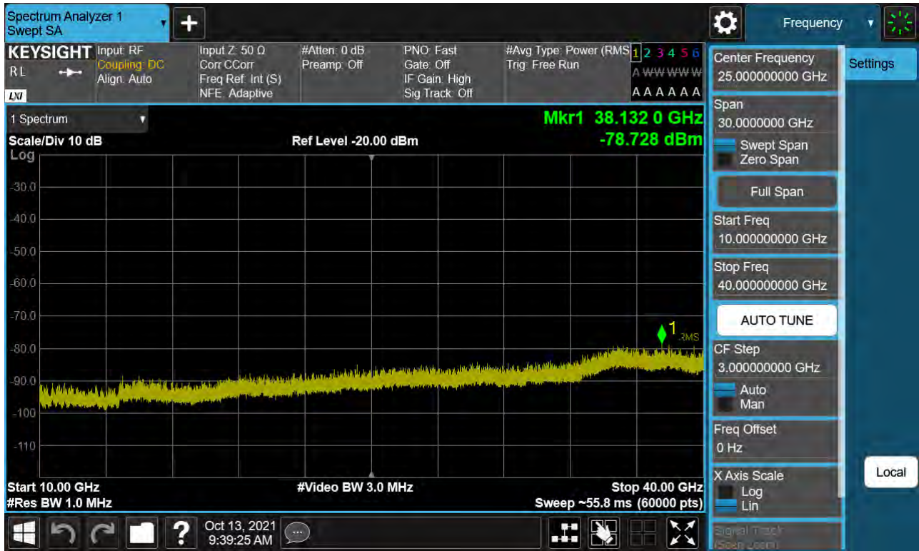
Sub6 n77. Conducted Spurious Plot_2 (663000ch_70 MHz_BPSK)
