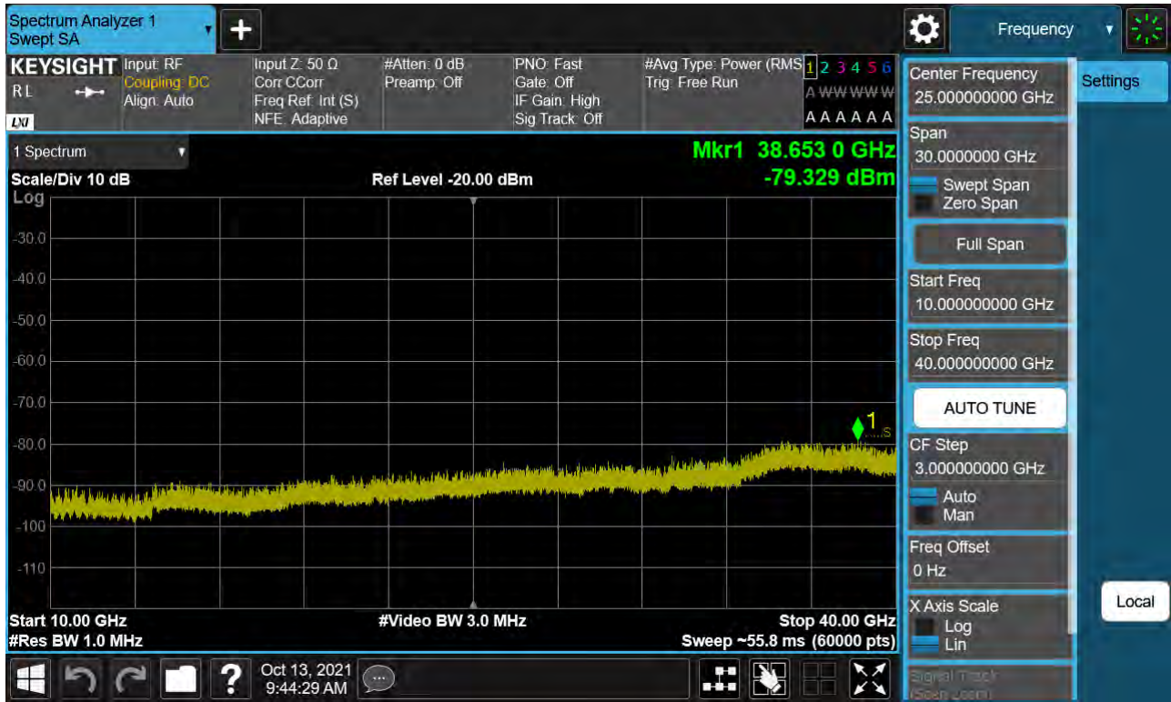
Sub6 n77. Conducted Spurious Plot_2 (649334ch_80 MHz_BPSK)
