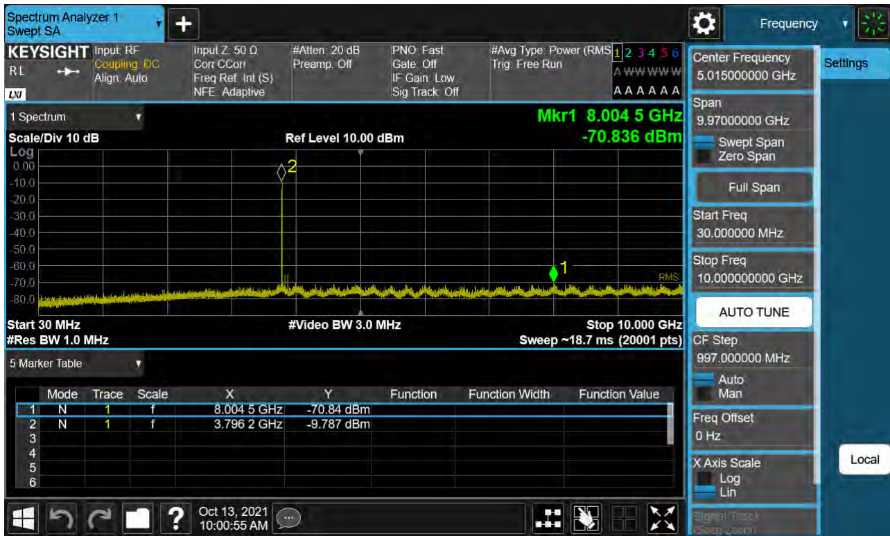
Sub6 n77. Conducted Spurious Plot_1 (656000ch_90 MHz_BPSK)
