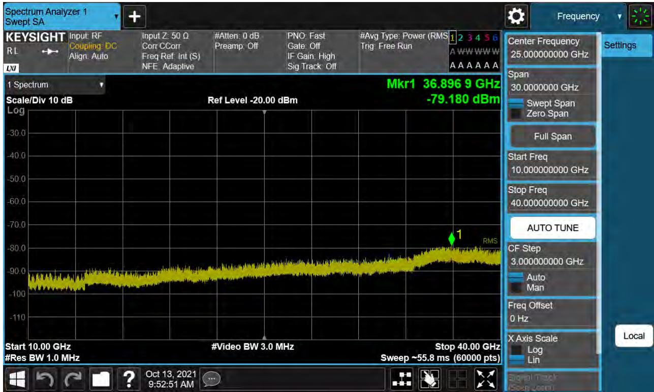
Sub6 n77. Conducted Spurious Plot_2 (662666ch_80 MHz_BPSK)
