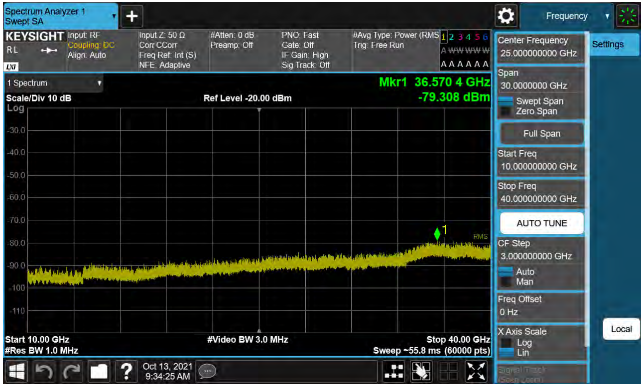
Sub6 n77. Conducted Spurious Plot_2 (656000ch_70 MHz_BPSK)
