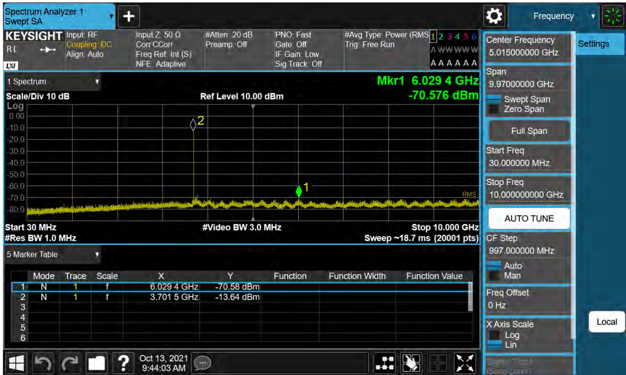
Sub6 n77. Conducted Spurious Plot_1 (649334ch_80 MHz_BPSK)
