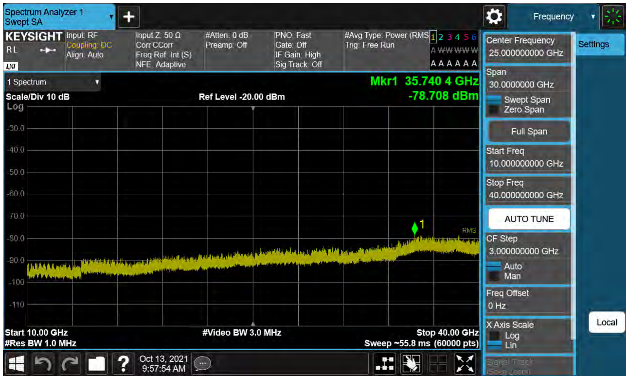
Sub6 n77. Conducted Spurious Plot_2 (649668ch_90 MHz_BPSK)
