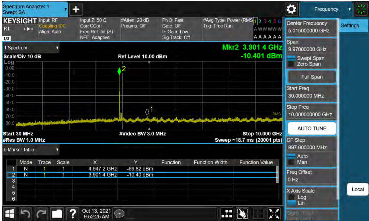
Sub6 n77. Conducted Spurious Plot_1 (662666ch_80 MHz_BPSK)
