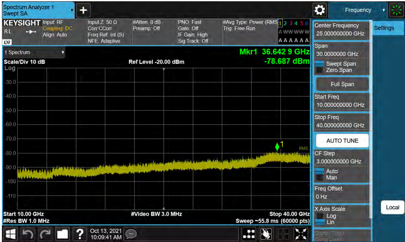
Sub6 n77. Conducted Spurious Plot_2 (662332ch_90 MHz_BPSK)
