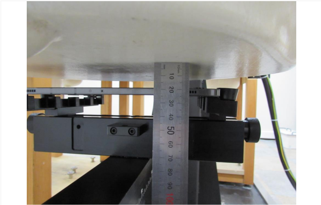
Distance of 19 mm from the EUT
