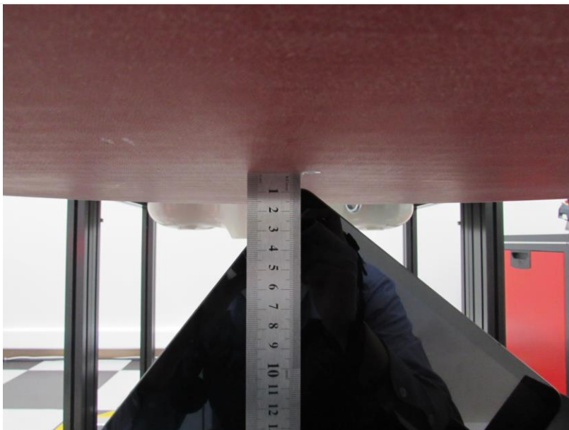
Distance of 8 mm from the EUT
