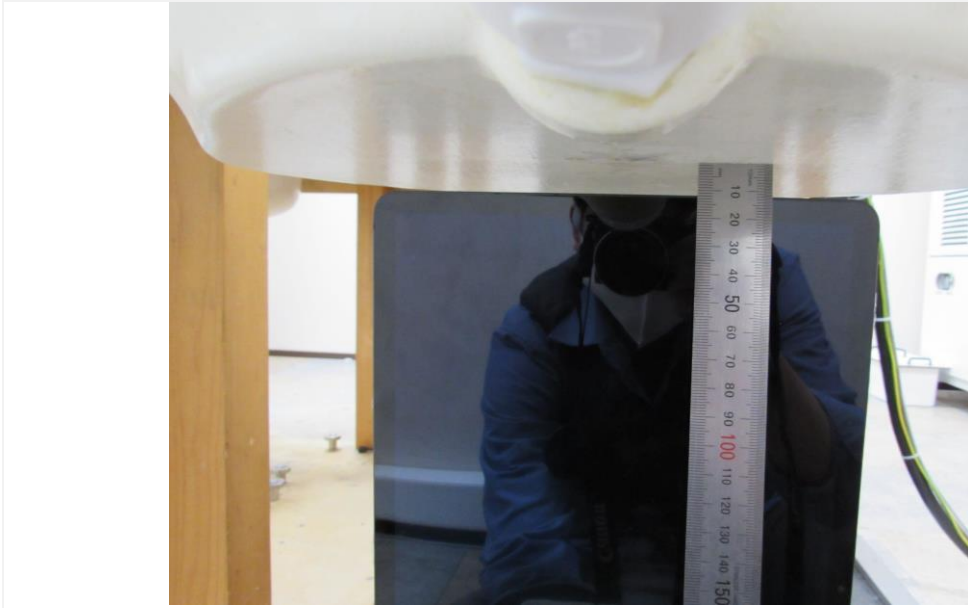
Distance of 12 mm from the EUT
