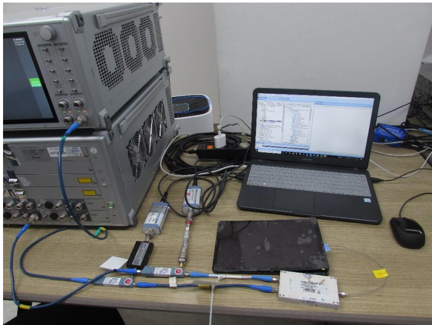
Test setup photo-4 (8-1(c) 5G Sub 6)
