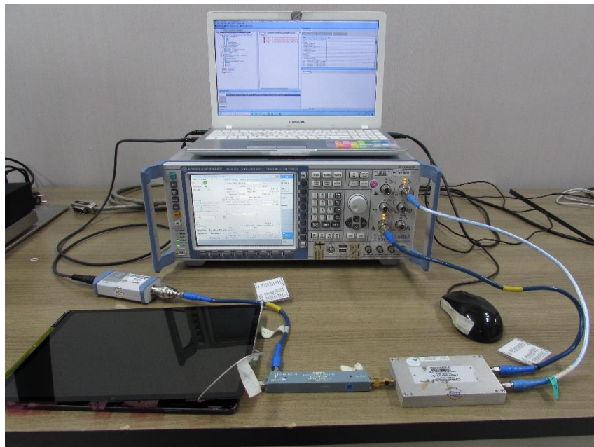
Test setup photo-2 (8-1(b) (Legacy))
