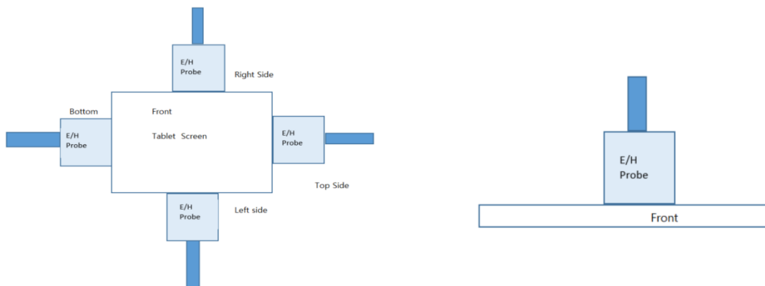
Figure1. H-Field and E-Field Measurement set up
