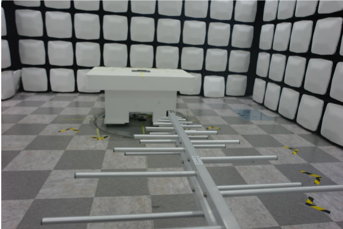
WPS Radiated Test Setup Photo for 30 MHz ~ 1 GHz :
