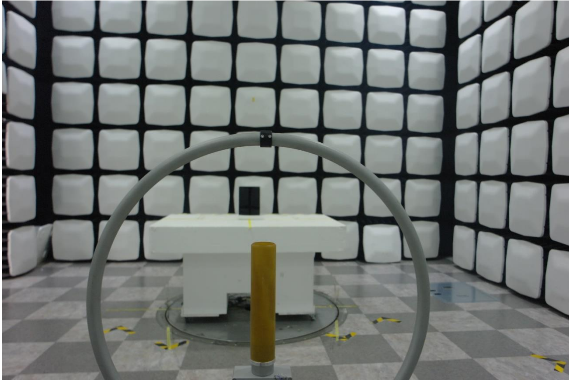
WPS Radiated Test Setup Photo for
