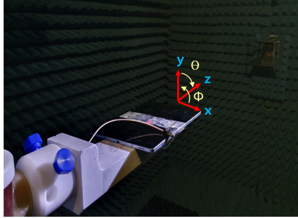
Figure 1: Geometry for SM-X818U for Radiation patterns.
