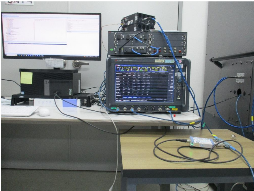
Test setup photo- (9-1(b) mmW NR radiated power measurement)
