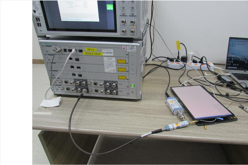
Test setup photo-4 (8-1(c) 5G Sub 6 SA)
