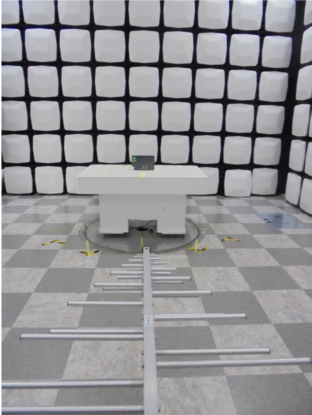
WPS Radiated Test Setup Photo for 30 MHz ~ 1 GHz :
