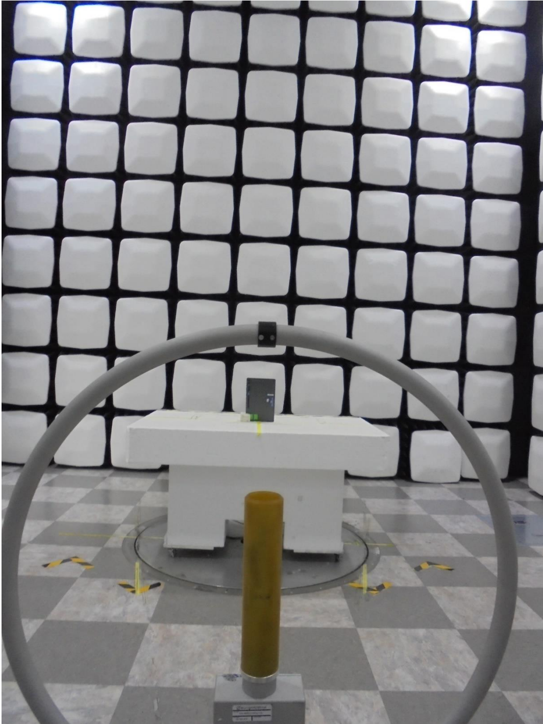
WPS Radiated Test Setup Photo for
