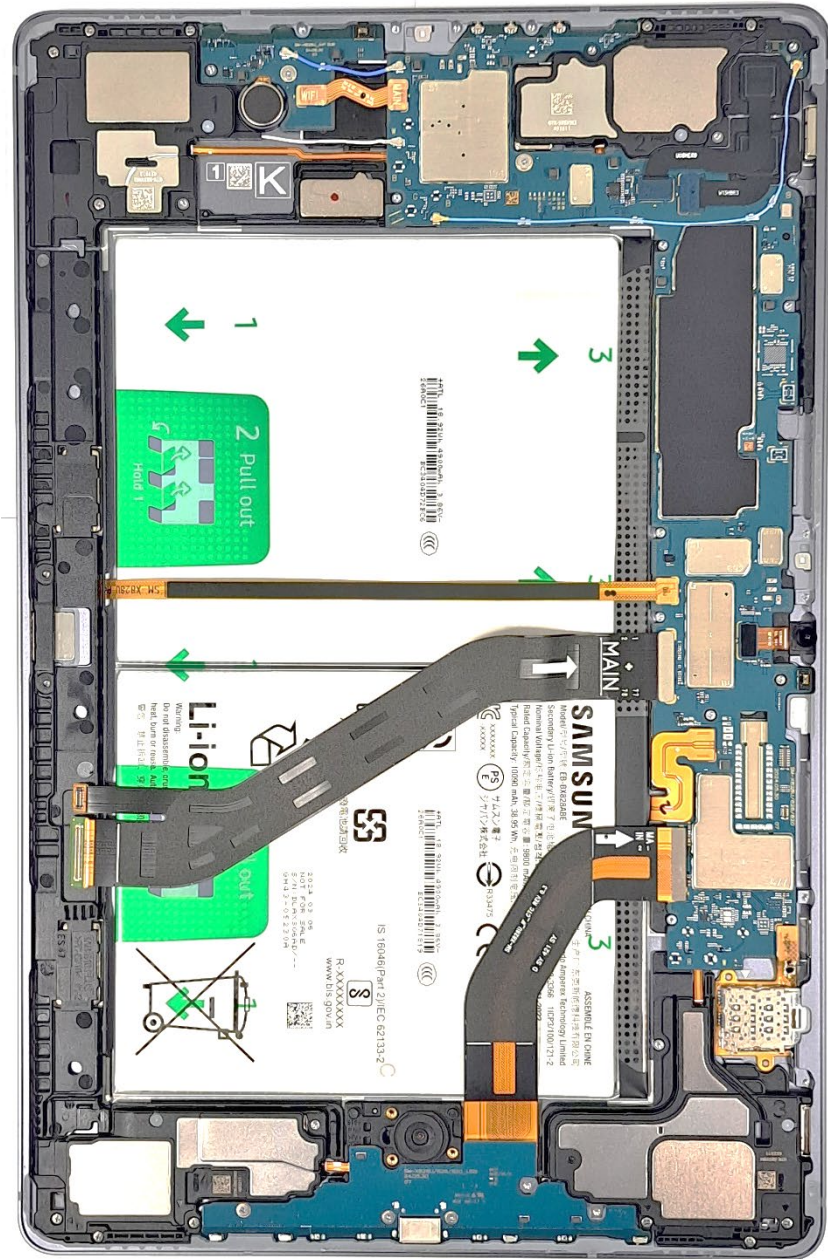
Internal without Bracket
