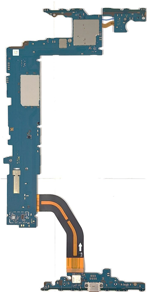
Main and Sub PBAs back
