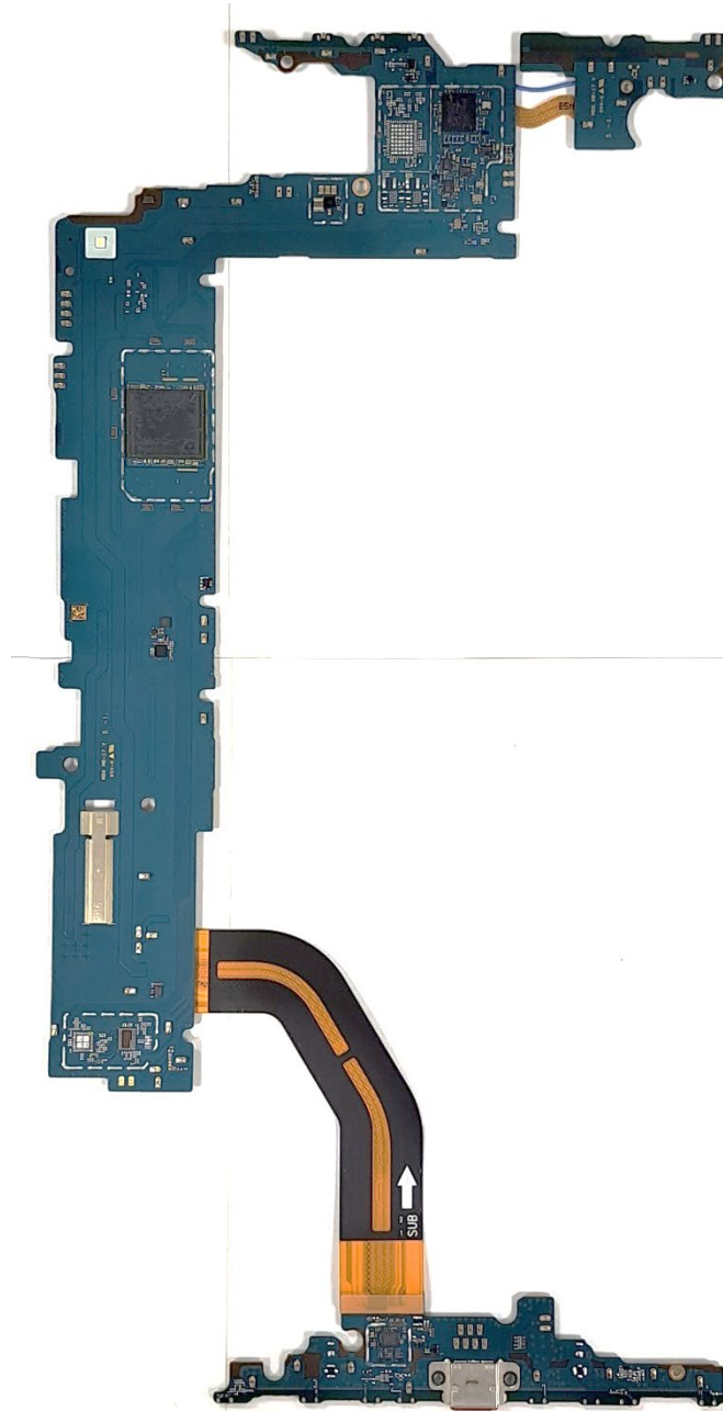
without Shieldcan back
