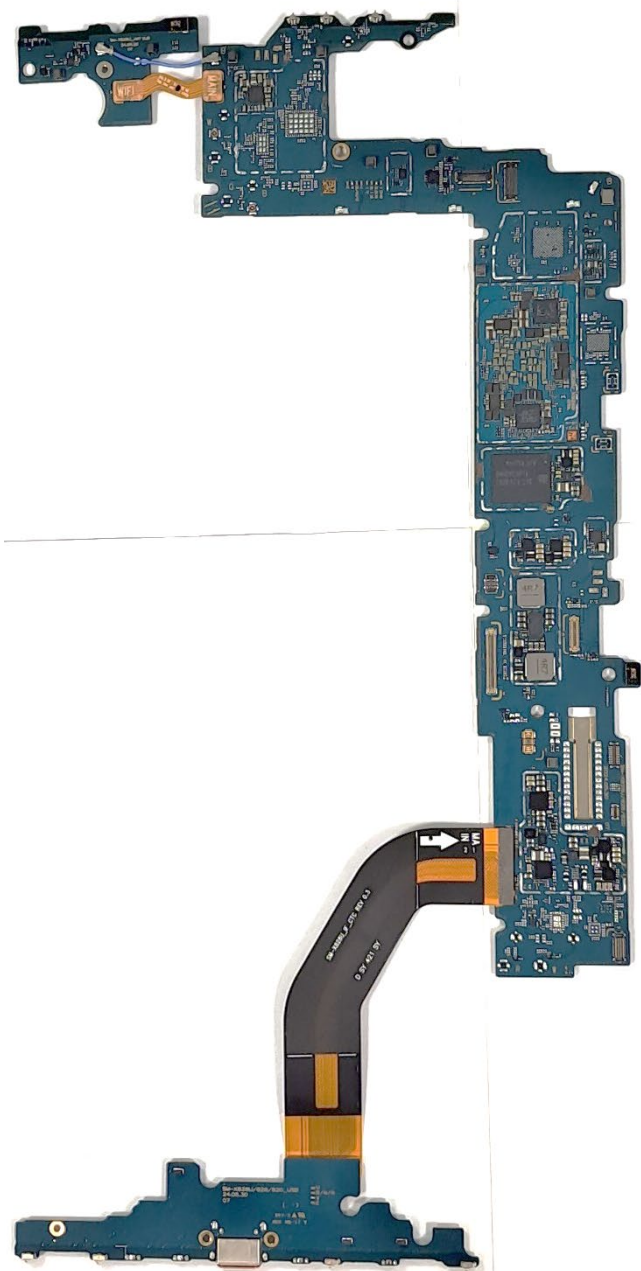
without Shieldcan front
