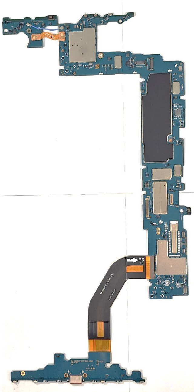
Main and Sub PBAs front
