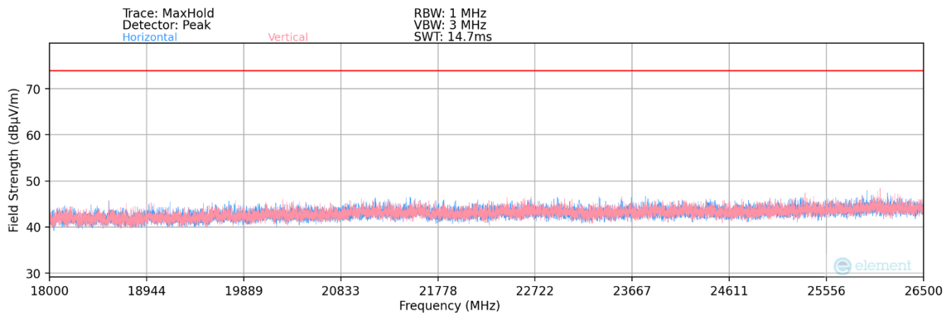
Plot 7-158. Radiated Spurious Plot 18GHz - 26.5GHz (802.11ax)
