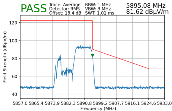
Plot 7-168. Radiated Upper Band Edge Plot MIMO (Average - UNII Band 4 - 106 Tones)
