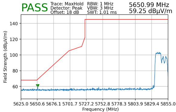
Plot 7-167. Radiated Lower Band Edge Plot MIMO (Peak - UNII Band 4 - 106 Tones)
