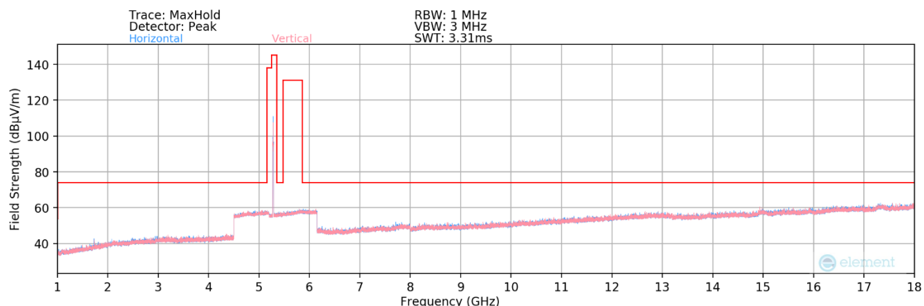
Plot 7-147. Radiated Spurious Plot above 1GHz MIMO (802.11ax – UNII 2A Ch. 56)
