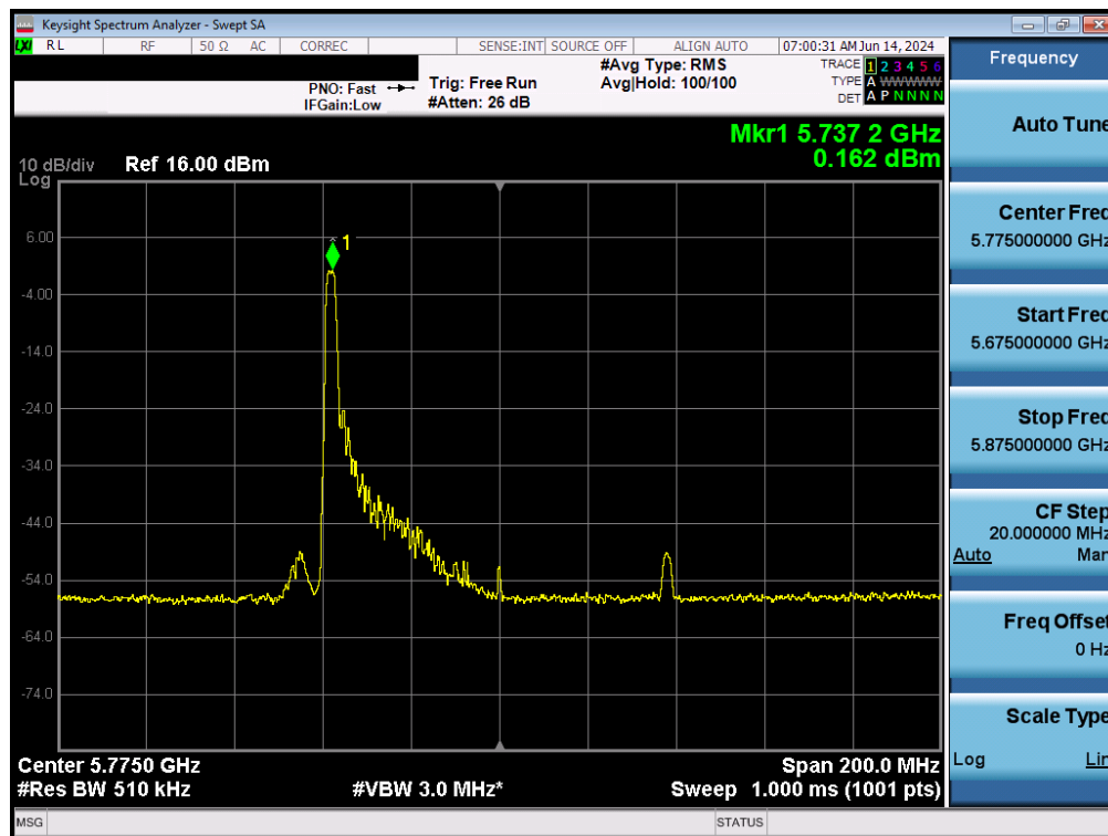
Plot 7-123. Power Spectral Density Plot MIMO ANT2 (80MHz BW 802.11ax – 26 Tones (UNII Band 3) – Ch. 155)
