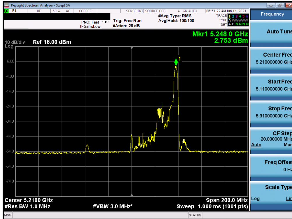
Plot 7-112. Power Spectral Density Plot MIMO ANT2 (80MHz BW 802.11ax – 26 Tones (UNII Band 1) – Ch. 42)
