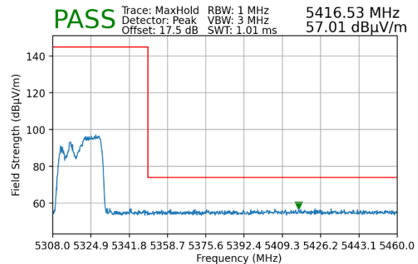
Plot 7-163. Radiated Upper Band Edge Plot MIMO (Peak – UNII Band 2A – 106 Tones)
