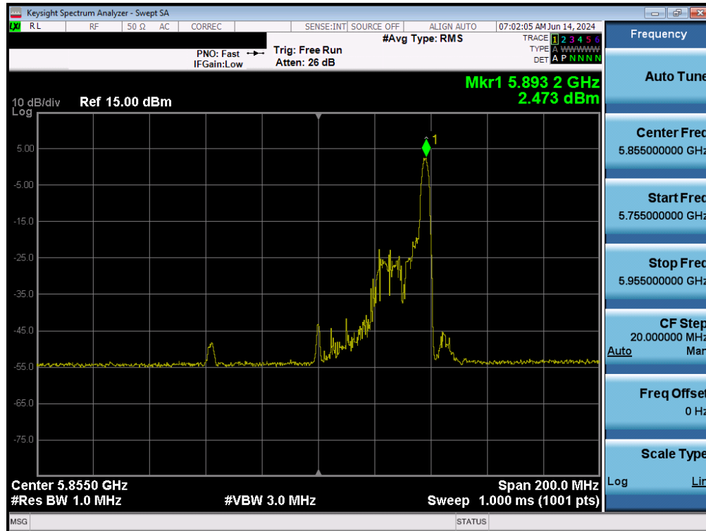
Plot 7-126. Power Spectral Density Plot MIMO ANT2 (80MHz BW 802.11ax – 26 Tones (UNII Band 3/4) – Ch. 171)
