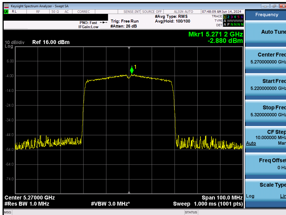
Plot 7-133. Power Spectral Density Plot MIMO ANT2 (40MHz BW 802.11ax – 484 Tones (UNII Band 2A) – Ch. 54)
