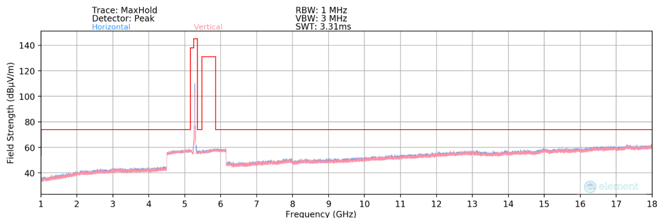
Plot 7-154. Radiated Spurious Plot above 1GHz MIMO (802.11ax – UNII 2A Ch. 56)
