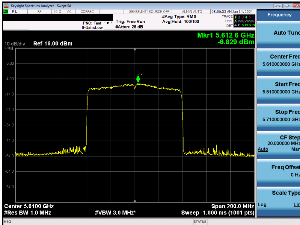
Plot 7-137. Power Spectral Density Plot MIMO ANT2 (80MHz BW 802.11ax – 996 Tones (UNII Band 2C) – Ch. 122)
