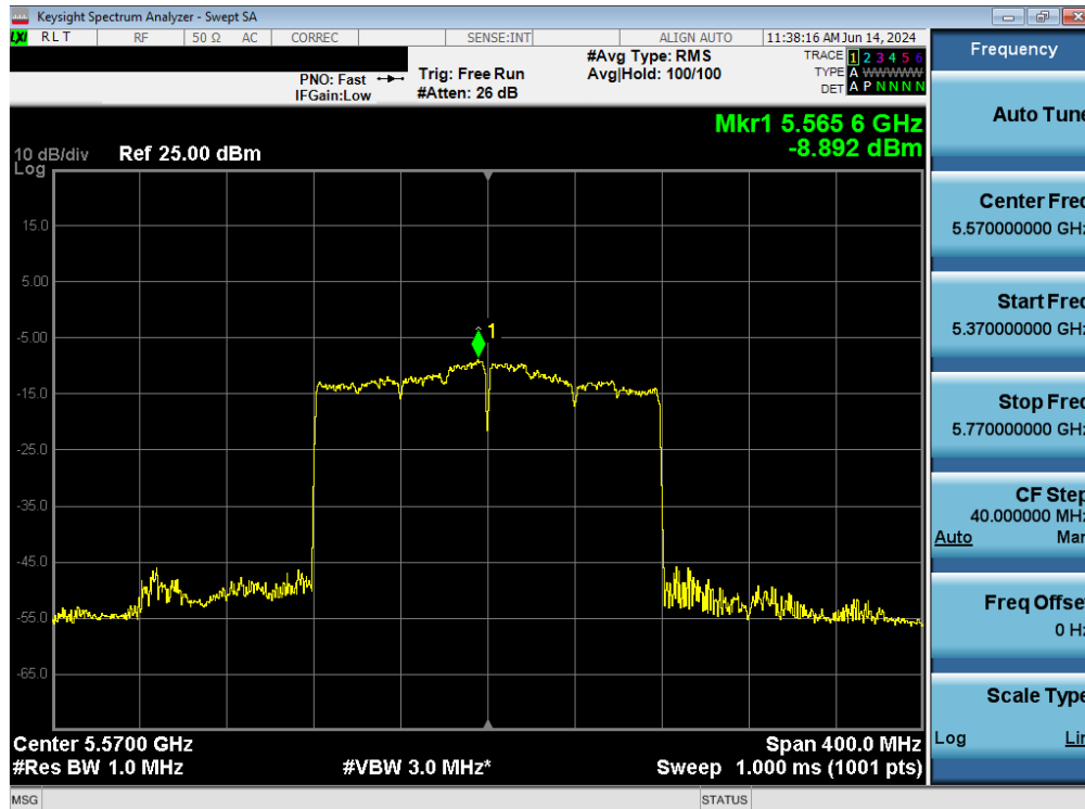
Plot 7-102. Power Spectral Density Plot MIMO ANT1 (160MHz BW 802.11ax – 2x996 Tones (UNII Band 2C) – Ch. 114)
