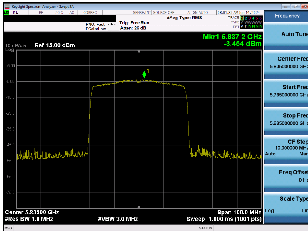
Plot 7-143. Power Spectral Density Plot MIMO ANT2 (40MHz BW 802.11ax – 484 Tones (UNII Band 3/4) – Ch. 167)
