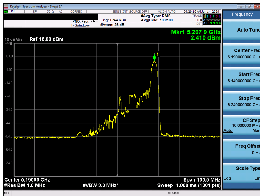
Plot 7-111. Power Spectral Density Plot MIMO ANT2 (40MHz BW 802.11ax – 26 Tones (UNII Band 1) – Ch. 38)
