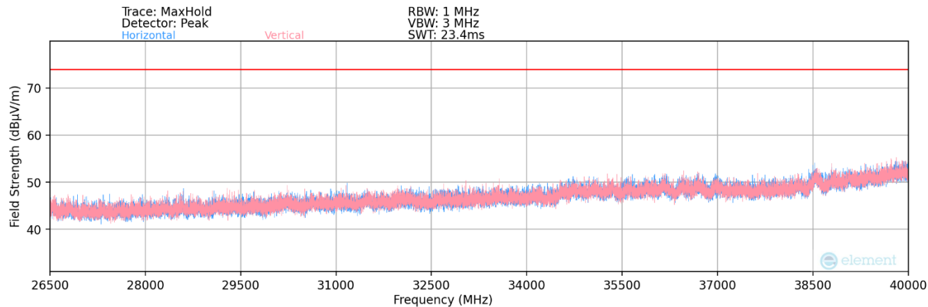
Plot 7-159. Radiated Spurious Plot 26.5GHz - 40GHz (802.11ax)
