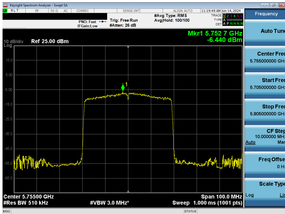
Plot 7-104. Power Spectral Density Plot MIMO ANT1 (40MHz BW 802.11ax – 484 Tones (UNII Band 3) – Ch. 151)
