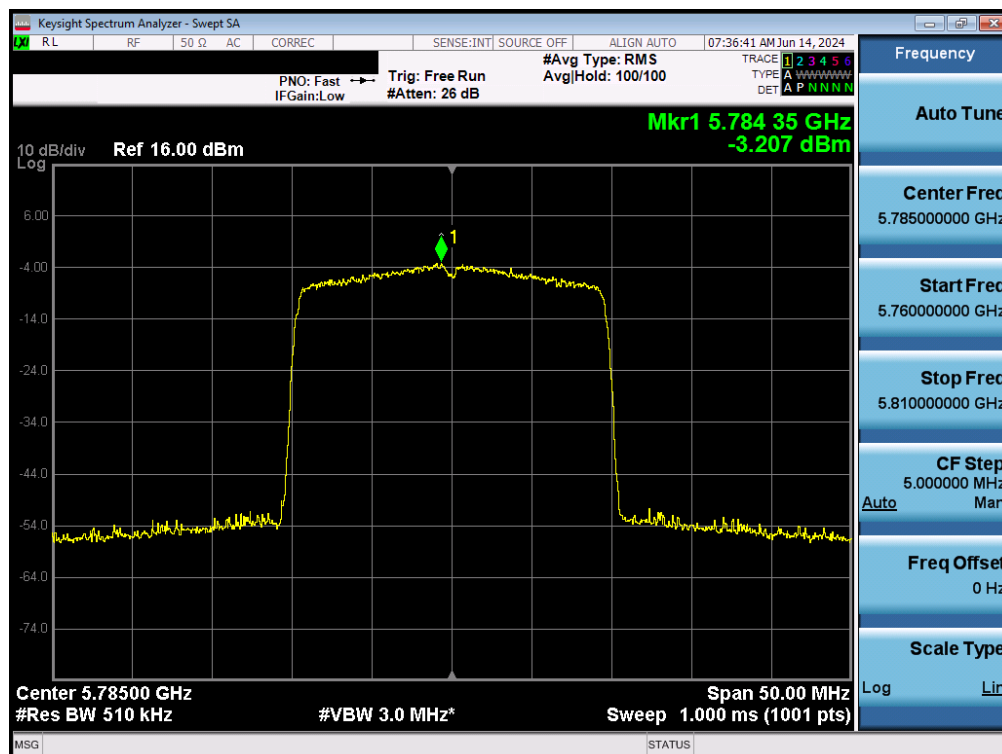
Plot 7-139. Power Spectral Density Plot MIMO ANT2 (20MHz BW 802.11ax – 242 Tones (UNII Band 3) – Ch. 157)
