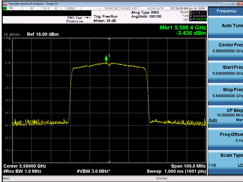
Plot 7-136. Power Spectral Density Plot MIMO ANT2 (40MHz BW 802.11ax – 484 Tones (UNII Band 2C) – Ch. 118)
