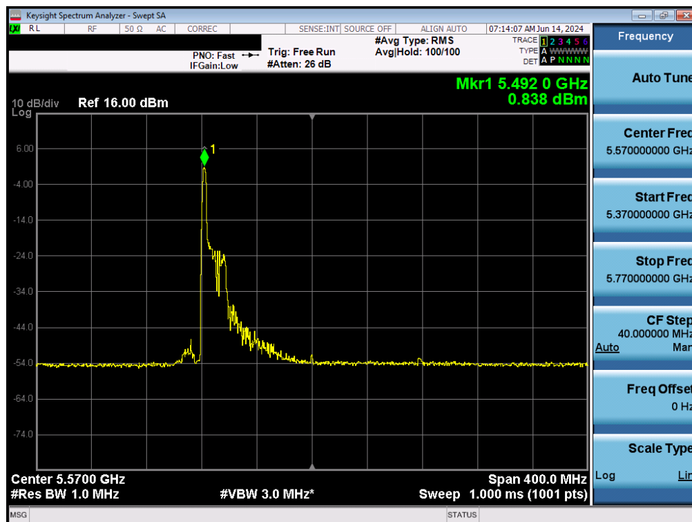
Plot 7-120. Power Spectral Density Plot MIMO ANT2 (160MHz BW 802.11ax – 26 Tones (UNII Band 2C) – Ch. 114)
