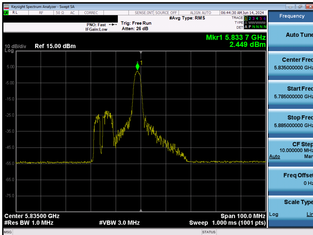
Plot 7-125. Power Spectral Density Plot MIMO ANT2 (40MHz BW 802.11ax – 26 Tones (UNII Band 3/4) – Ch. 167)
