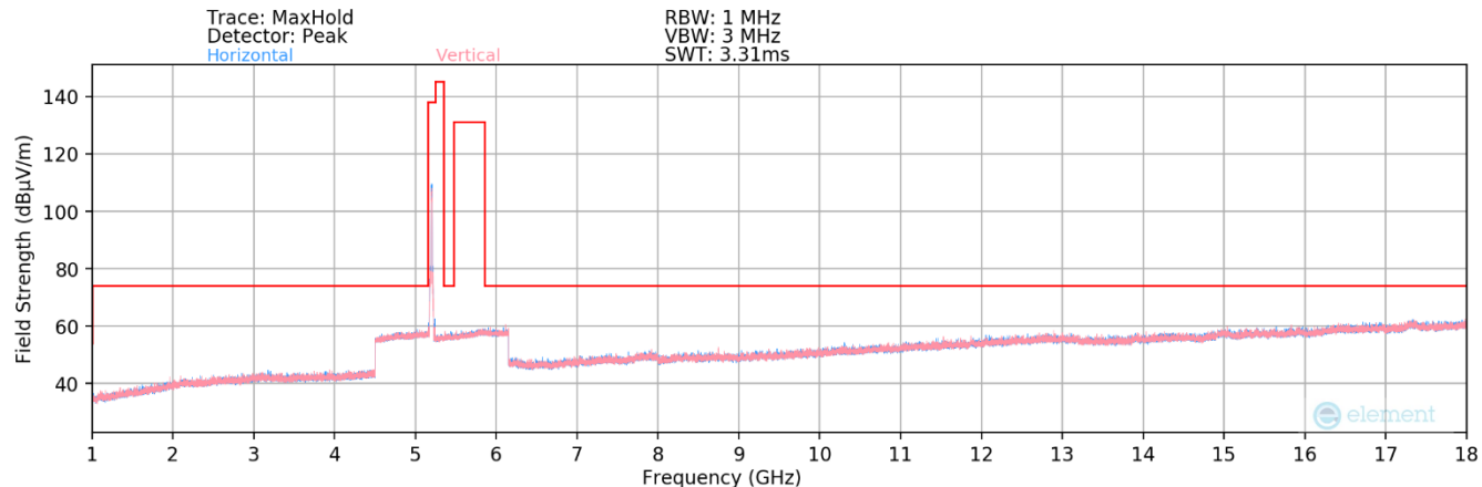
Plot 7-153. Radiated Spurious Plot above 1GHz MIMO (802.11ax – UNII 1 Ch. 40)
