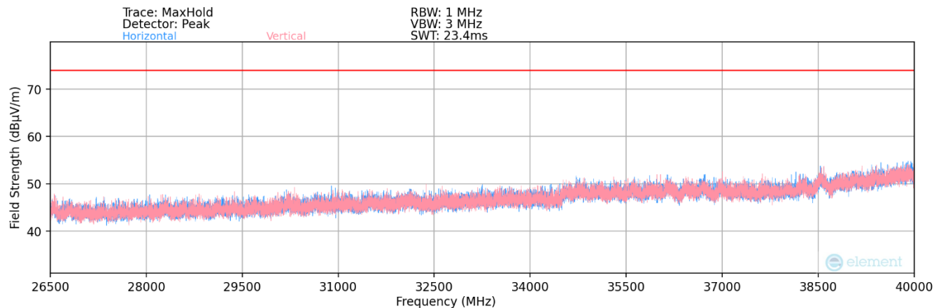
Plot 7-152. Radiated Spurious Plot 26.5GHz - 40GHz (802.11ax)
