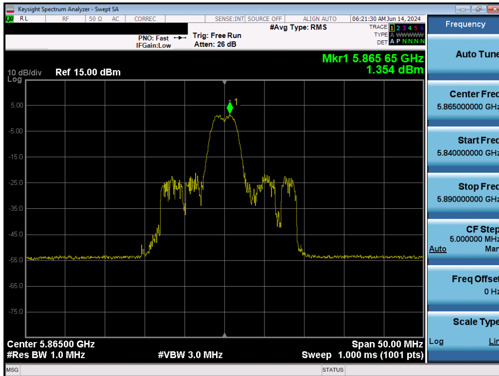
Plot 7-124. Power Spectral Density Plot MIMO ANT2 (20MHz BW 802.11ax – 26 Tones (UNII Band 4) – Ch. 173)
