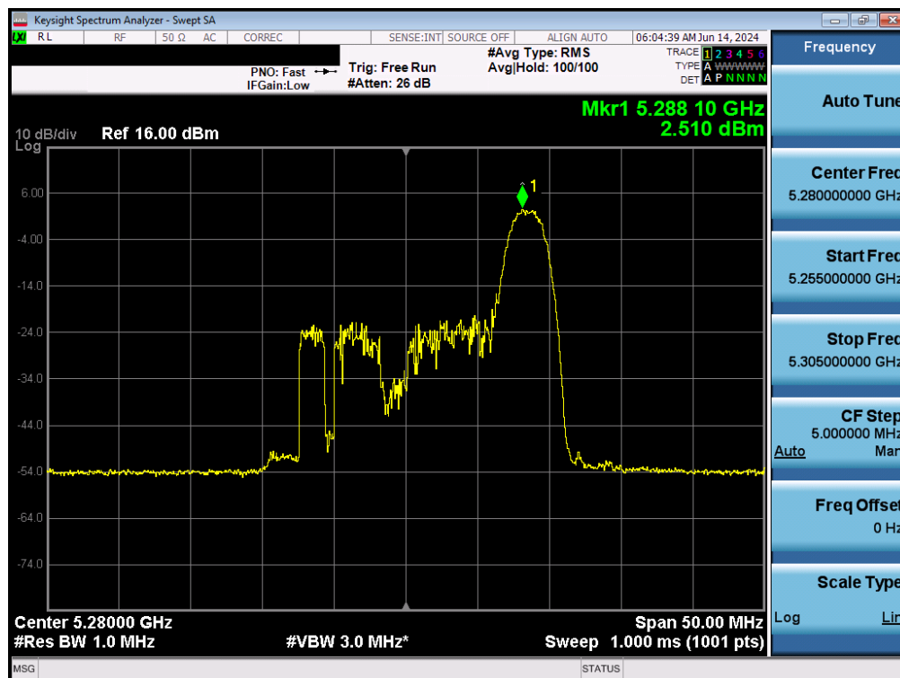
Plot 7-114. Power Spectral Density Plot MIMO ANT2 (20MHz BW 802.11ax – 26 Tones (UNII Band 2A) – Ch. 56)
