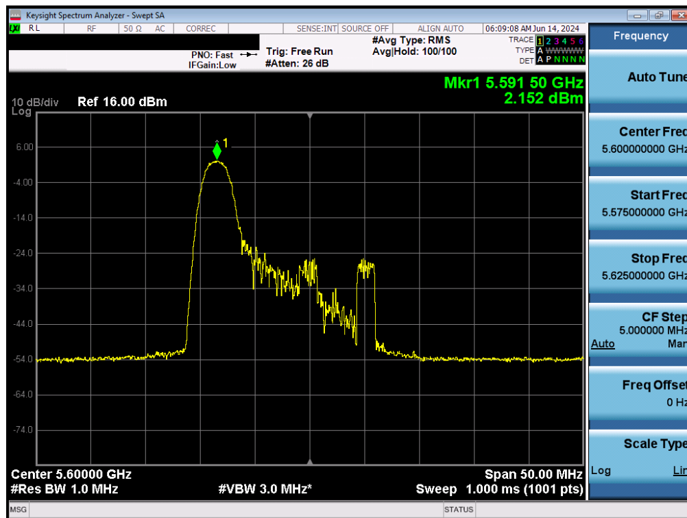
Plot 7-117. Power Spectral Density Plot MIMO ANT2 (20MHz BW 802.11ax – 26 Tones (UNII Band 2C) – Ch. 120)
