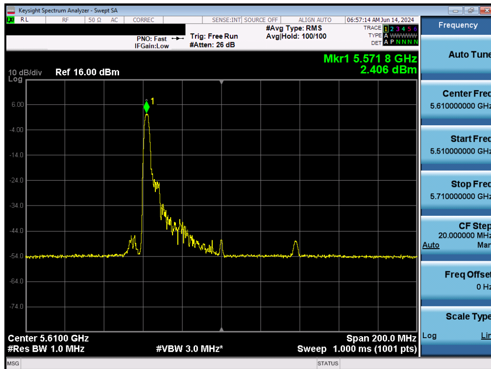
Plot 7-119. Power Spectral Density Plot MIMO ANT2 (80MHz BW 802.11ax – 26 Tones (UNII Band 2C) – Ch. 122)
