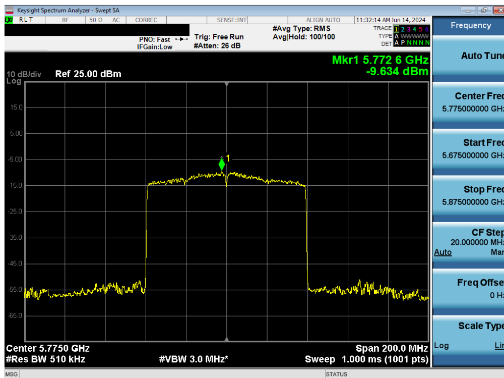
Plot 7-105. Power Spectral Density Plot MIMO ANT1 (80MHz BW 802.11ax – 996 Tones (UNII Band 3) – Ch. 155)
