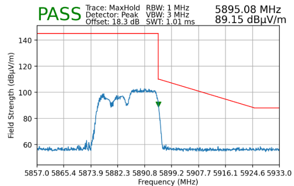
Plot 7-169. Radiated Upper Band Edge Plot MIMO (Peak - UNII Band 4 - 106 Tones)
