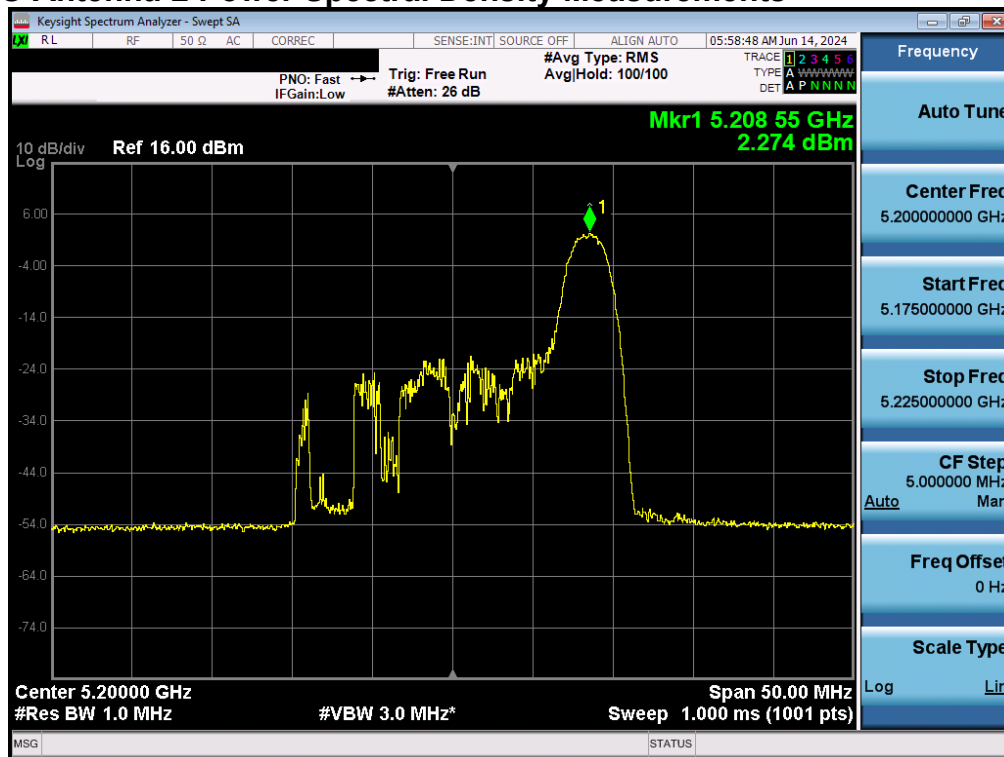
Plot 7-110. Power Spectral Density Plot MIMO ANT2 (20MHz BW 802.11ax – 26 Tones (UNII Band 1) – Ch. 40)
