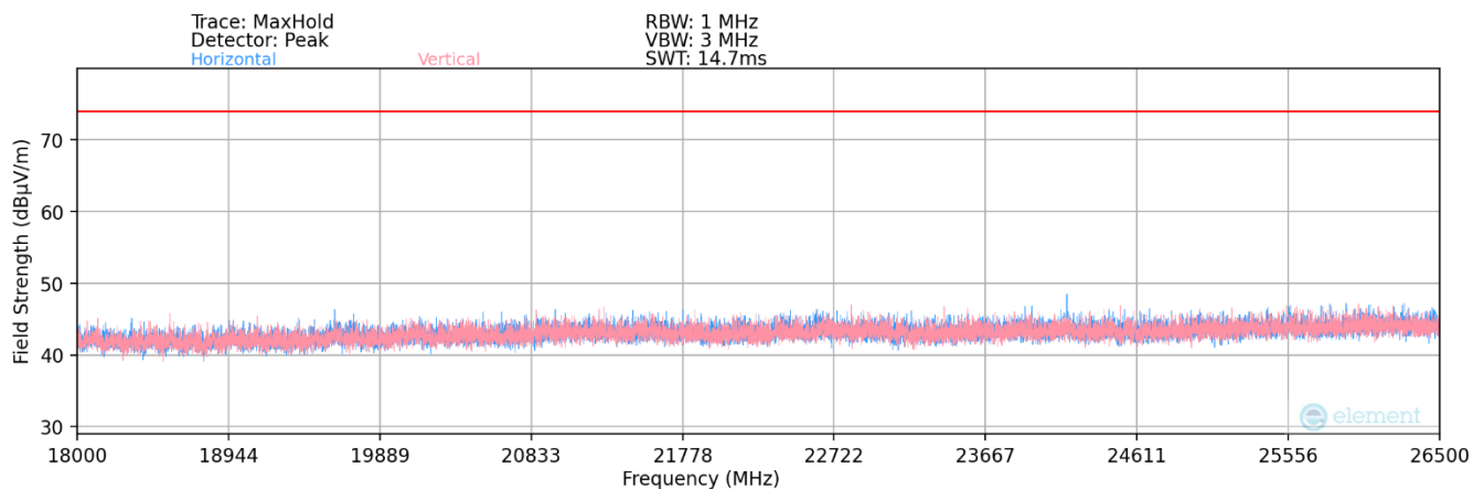
Plot 7-151. Radiated Spurious Plot 18GHz - 26.5GHz (802.11ax)
