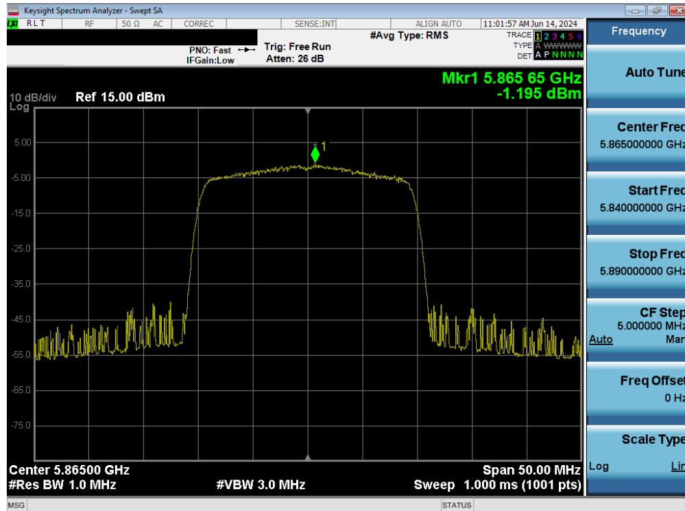
Plot 7-106. Power Spectral Density Plot MIMO ANT1 (20MHz BW 802.11ax – 242 Tones (UNII Band 4) – Ch. 173)
