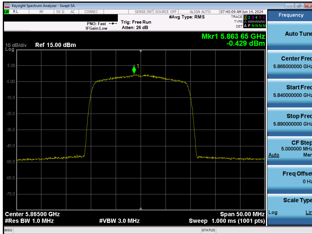
Plot 7-142. Power Spectral Density Plot MIMO ANT2 (20MHz BW 802.11ax – 242 Tones (UNII Band 4) – Ch. 173)
