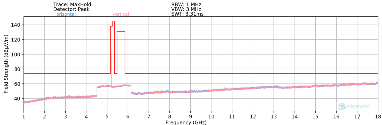
Plot 7-146. Radiated Spurious Plot above 1GHz MIMO (802.11ax – UNII 1 Ch. 40)
