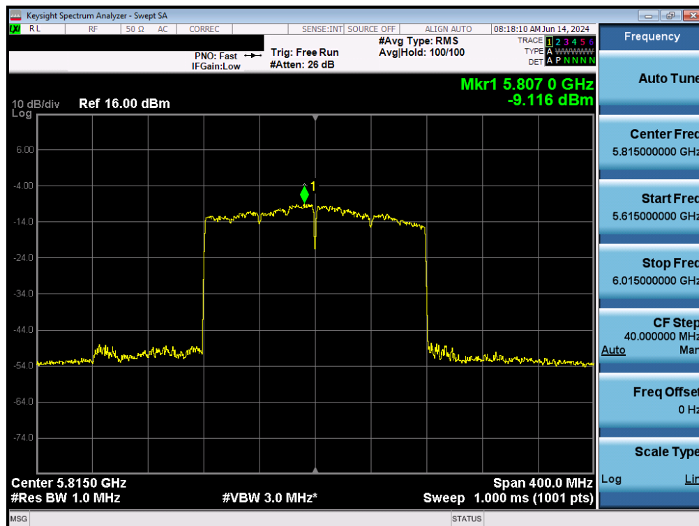
Plot 7-145. Power Spectral Density Plot MIMO ANT2 (160MHz BW 802.11ax – 996*2 Tones (UNII Band 3/4) – Ch. 163)
