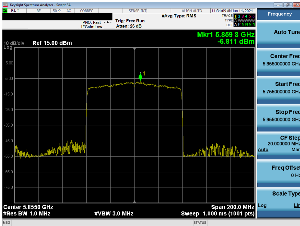
Plot 7-108. Power Spectral Density Plot MIMO ANT1 (80MHz BW 802.11ax – 996 Tones (UNII Band 3/4) – Ch. 171)
