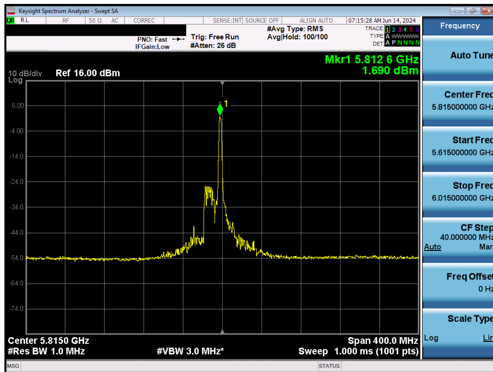
Plot 7-127. Power Spectral Density Plot MIMO ANT2 (160MHz BW 802.11ax – 26 Tones (UNII Band 3/4) – Ch. 163)
