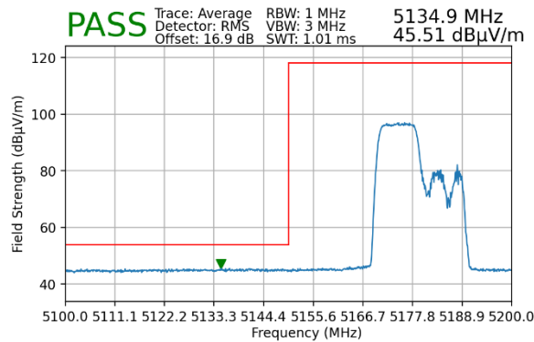
Plot 7-160. Radiated Lower Band Edge Plot MIMO (Average – UNII Band 1 – 106 Tones)
