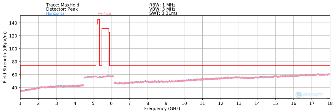
Plot 7-150. Radiated Spurious Plot above 1GHz MIMO (802.11ax – UNII 4 Ch. 173)
