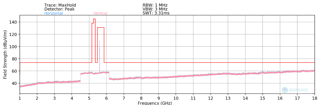
Plot 7-148. Radiated Spurious Plot above 1GHz MIMO (802.11ax – UNII 2C Ch. 120)
