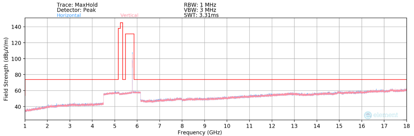
Plot 7-149. Radiated Spurious Plot above 1GHz MIMO (802.11ax – UNII 3 Ch. 157)
