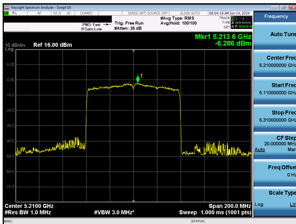
Plot 7-130. Power Spectral Density Plot MIMO ANT2 (80MHz BW 802.11ax – 996 Tones (UNII Band 1) – Ch. 42)
