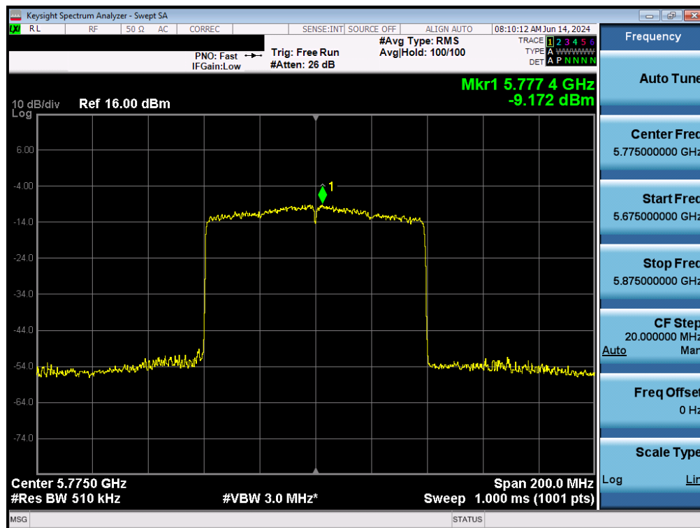
Plot 7-141. Power Spectral Density Plot MIMO ANT2 (80MHz BW 802.11ax – 996 Tones (UNII Band 3) – Ch. 155)
