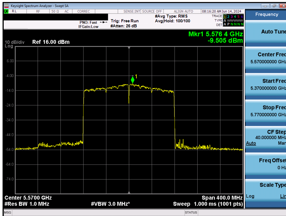
Plot 7-138. Power Spectral Density Plot MIMO ANT2 (160MHz BW 802.11ax – 2x996 Tones (UNII Band 2C) – Ch. 114)
