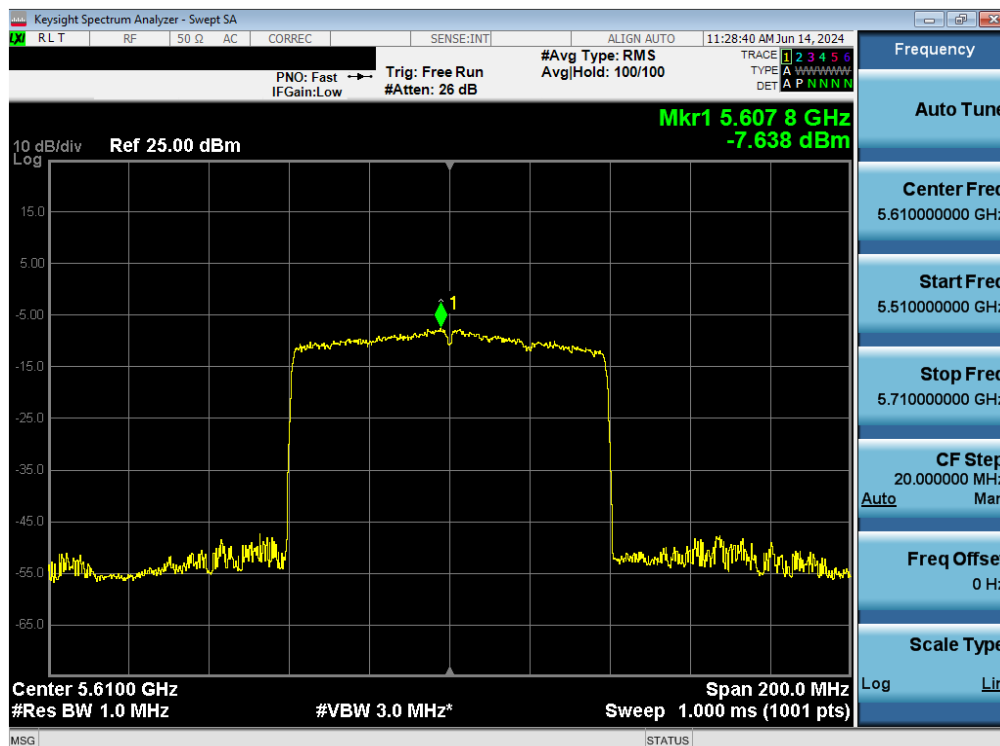
Plot 7-101. Power Spectral Density Plot MIMO ANT1 (80MHz BW 802.11ax – 996 Tones (UNII Band 2C) – Ch. 122)
