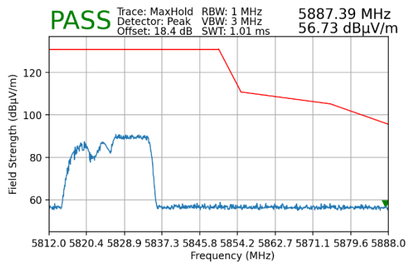
Plot 7-166. Radiated Upper Band Edge Plot MIMO (Peak – UNII Band 3 – 106 Tones)
