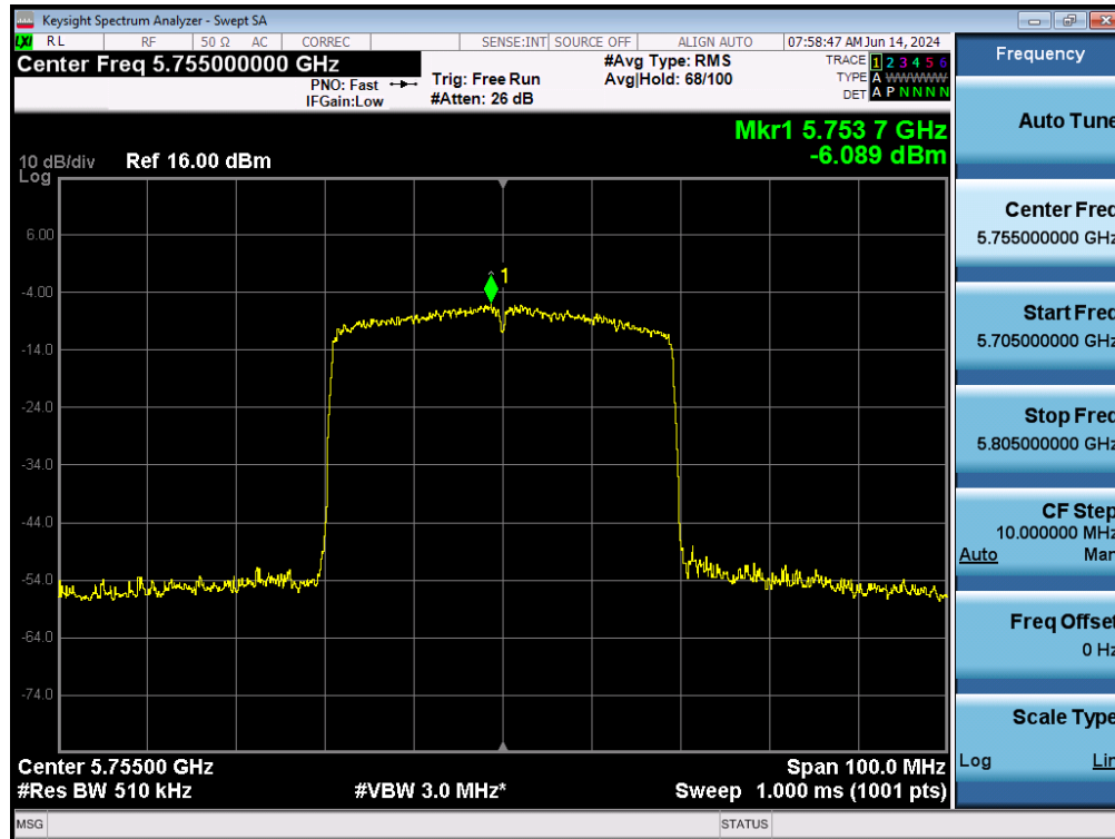
Plot 7-140. Power Spectral Density Plot MIMO ANT2 (40MHz BW 802.11ax – 484 Tones (UNII Band 3) – Ch. 151)
