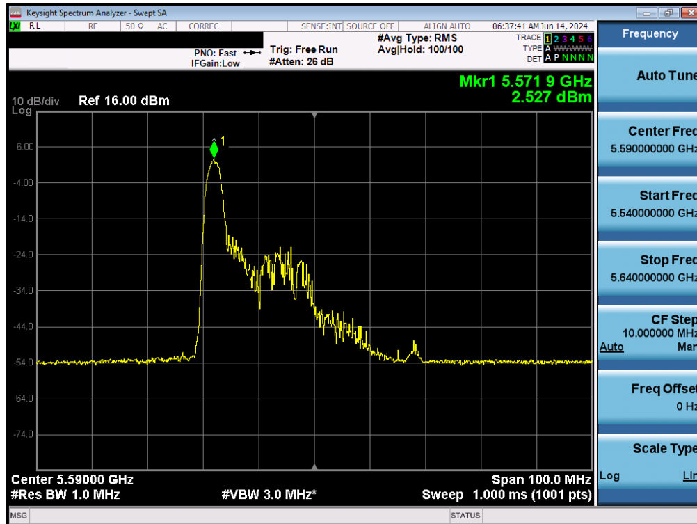
Plot 7-118. Power Spectral Density Plot MIMO ANT2 (40MHz BW 802.11ax – 26 Tones (UNII Band 2C) – Ch. 118)
