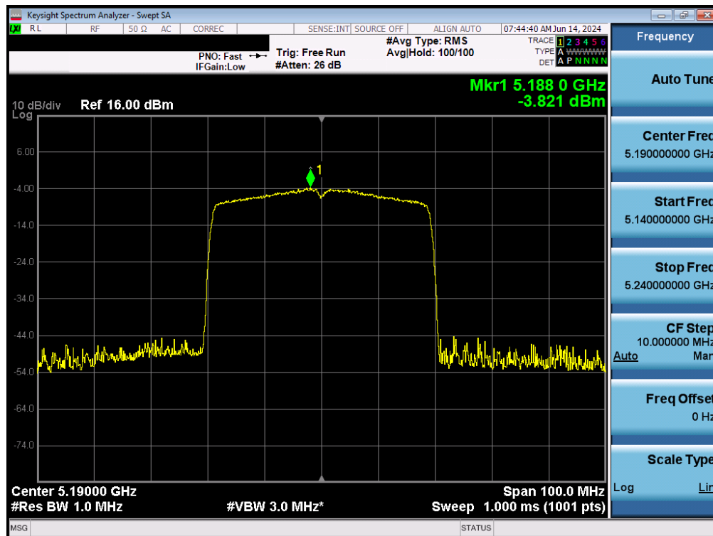
Plot 7-129. Power Spectral Density Plot MIMO ANT2 (40MHz BW 802.11ax – 484 Tones (UNII Band 1) – Ch. 38)
