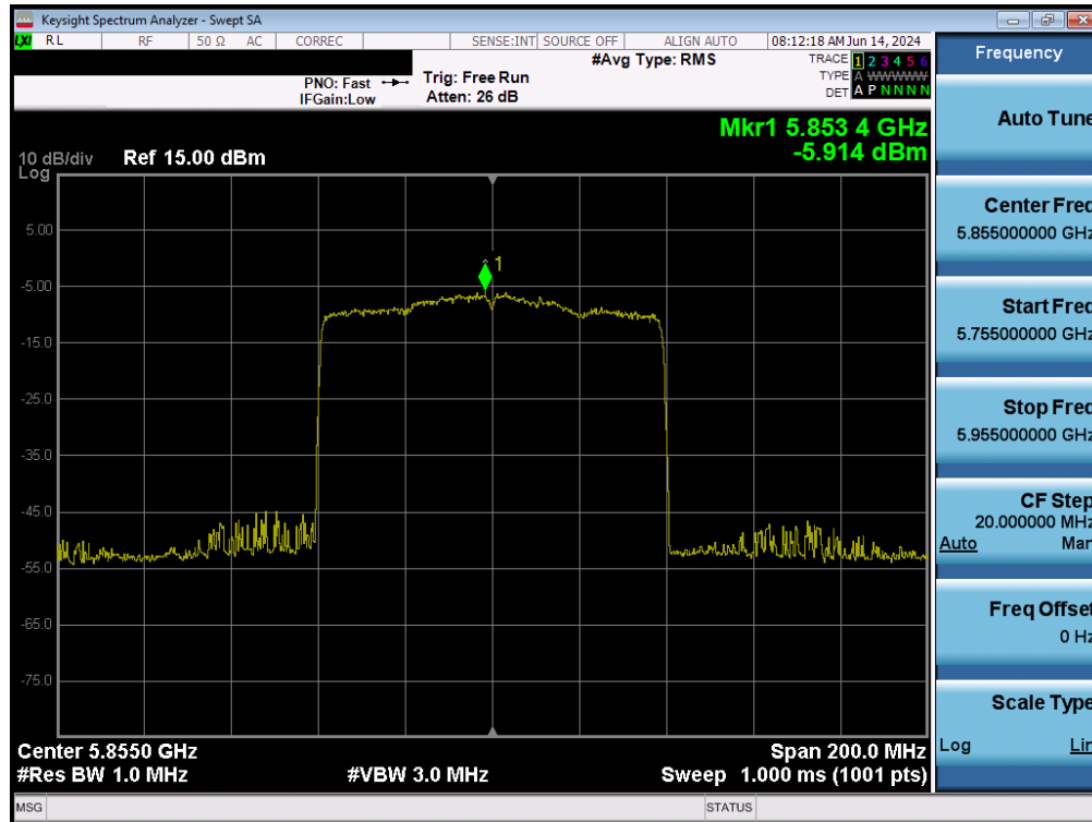
Plot 7-144. Power Spectral Density Plot MIMO ANT2 (80MHz BW 802.11ax – 996 Tones (UNII Band 3/4) – Ch. 171)
