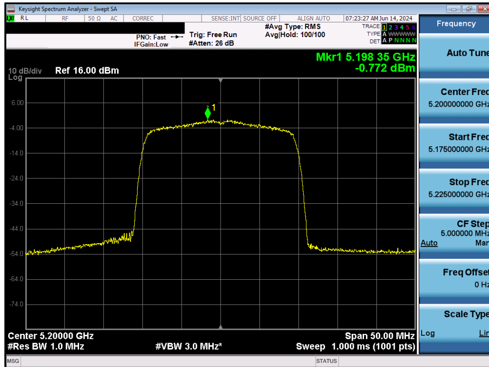
Plot 7-128. Power Spectral Density Plot MIMO ANT2 (20MHz BW 802.11ax – 242 Tones (UNII Band 1) – Ch. 40)
