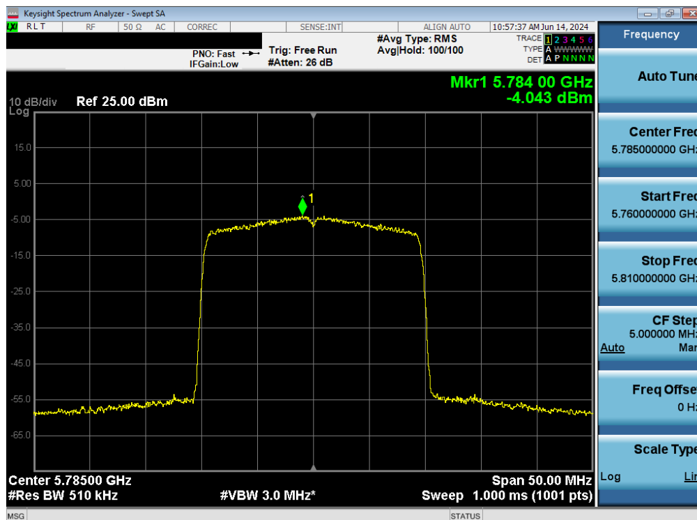
Plot 7-103. Power Spectral Density Plot MIMO ANT1 (20MHz BW 802.11ax – 242 Tones (UNII Band 3) – Ch. 157)
