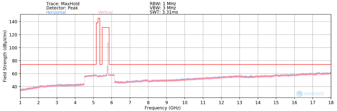
Plot 7-156. Radiated Spurious Plot above 1GHz MIMO (802.11ax – UNII 3 Ch. 157)
