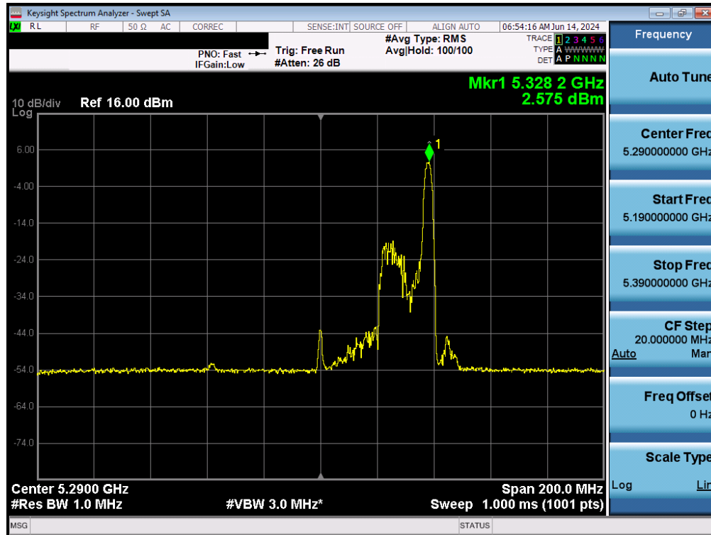
Plot 7-116. Power Spectral Density Plot MIMO ANT2 (80MHz BW 802.11ax – 26 Tones (UNII Band 2A) – Ch. 58)
