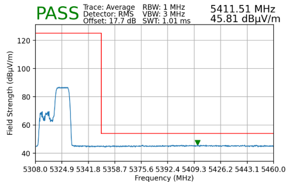
Plot 7-162. Radiated Upper Band Edge Plot MIMO (Average – UNII Band 2A – 106 Tones)
