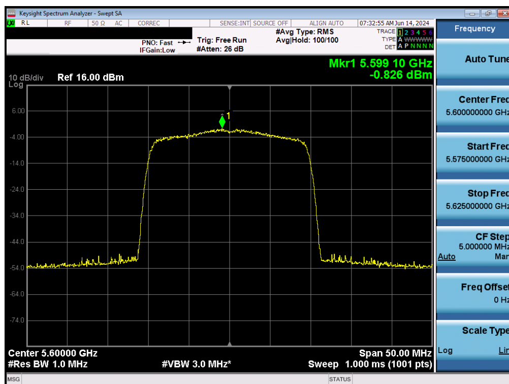
Plot 7-135. Power Spectral Density Plot MIMO ANT2 (20MHz BW 802.11ax – 242 Tones (UNII Band 2C) – Ch. 120)
