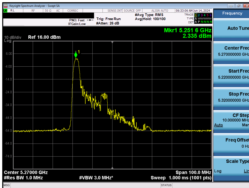
Plot 7-115. Power Spectral Density Plot MIMO ANT2 (40MHz BW 802.11ax – 26 Tones (UNII Band 2A) – Ch. 54)
