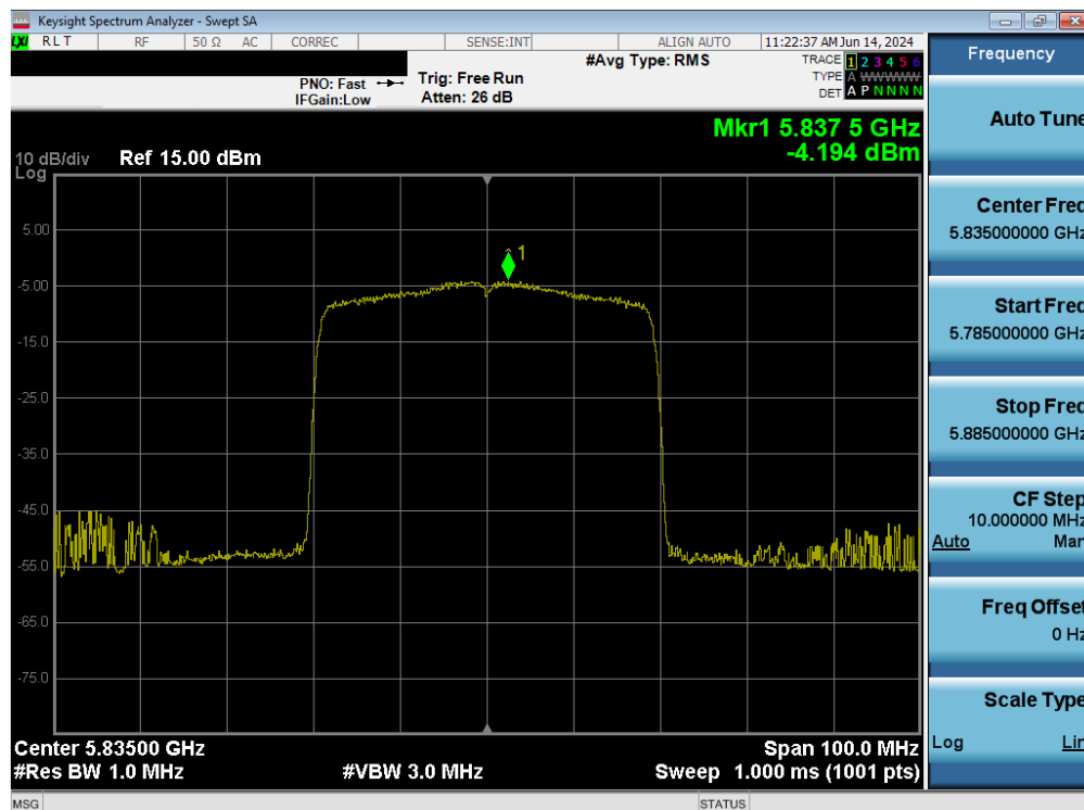
Plot 7-107. Power Spectral Density Plot MIMO ANT1 (40MHz BW 802.11ax – 484 Tones (UNII Band 3/4) – Ch. 167)
