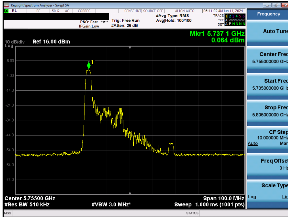
Plot 7-122. Power Spectral Density Plot MIMO ANT2 (40MHz BW 802.11ax – 26 Tones (UNII Band 3) – Ch. 151)
