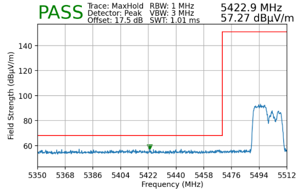
Plot 7-165. Radiated Lower Band Edge Plot MIMO (Peak – UNII Band 2C – 106 Tones)
