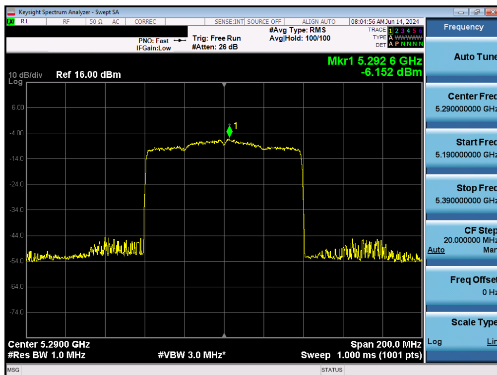
Plot 7-134. Power Spectral Density Plot MIMO ANT2 (80MHz BW 802.11ax – 996 Tones (UNII Band 2A) – Ch. 58)
