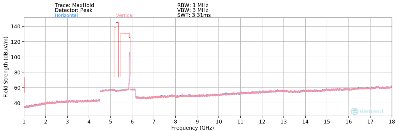
Plot 7-157. Radiated Spurious Plot above 1GHz MIMO (802.11ax – UNII 4 Ch. 173)
