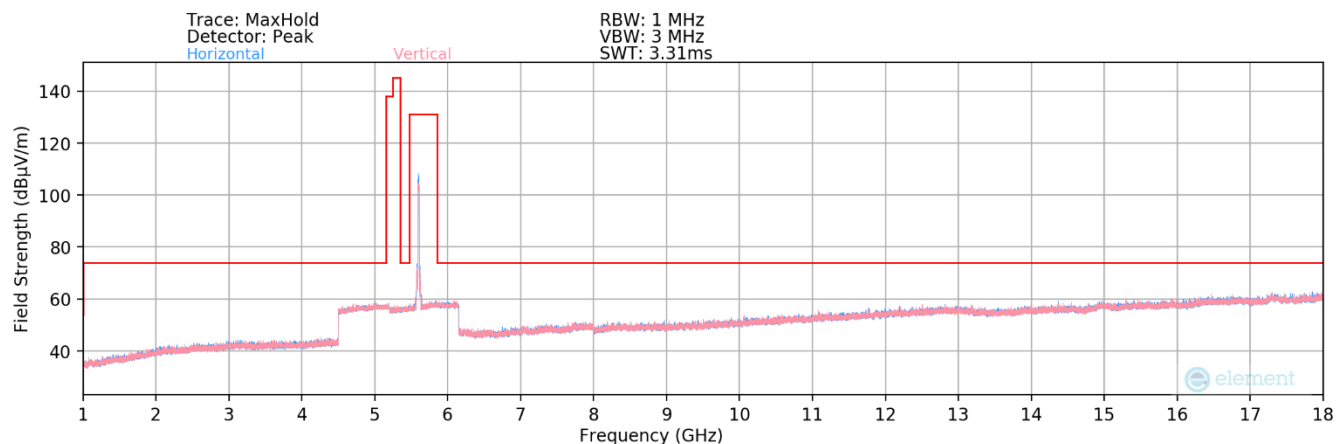
Plot 7-155. Radiated Spurious Plot above 1GHz MIMO (802.11ax – UNII 2C Ch. 120)
