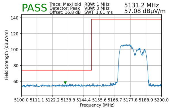
Plot 7-161. Radiated Lower Band Edge Plot MIMO (Peak – UNII Band 1 – 106 Tones)
