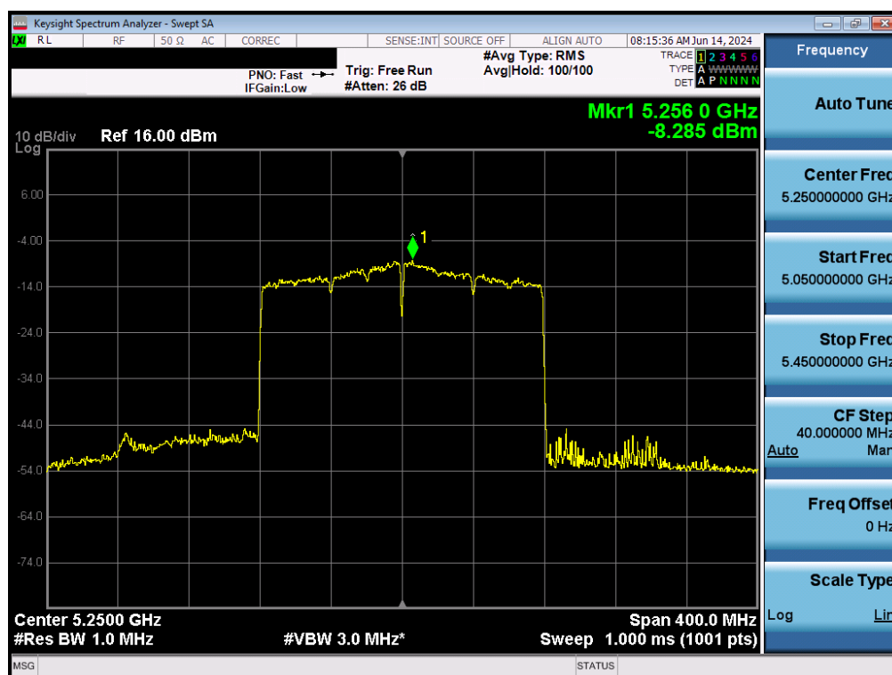
Plot 7-131. Power Spectral Density Plot MIMO ANT2 (160MHz BW 802.11ax – 2x996 Tones (UNII Band 1/2A) – Ch. 50)
