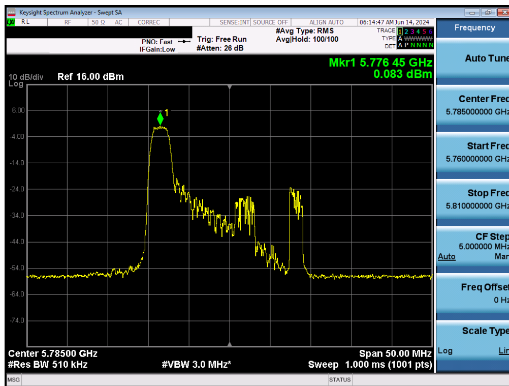
Plot 7-121. Power Spectral Density Plot MIMO ANT2 (20MHz BW 802.11ax – 26 Tones (UNII Band 3) – Ch. 157)
