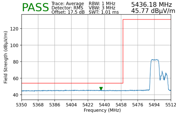
Plot 7-164. Radiated Lower Band Edge Plot MIMO (Average – UNII Band 2C – 106 Tones)
