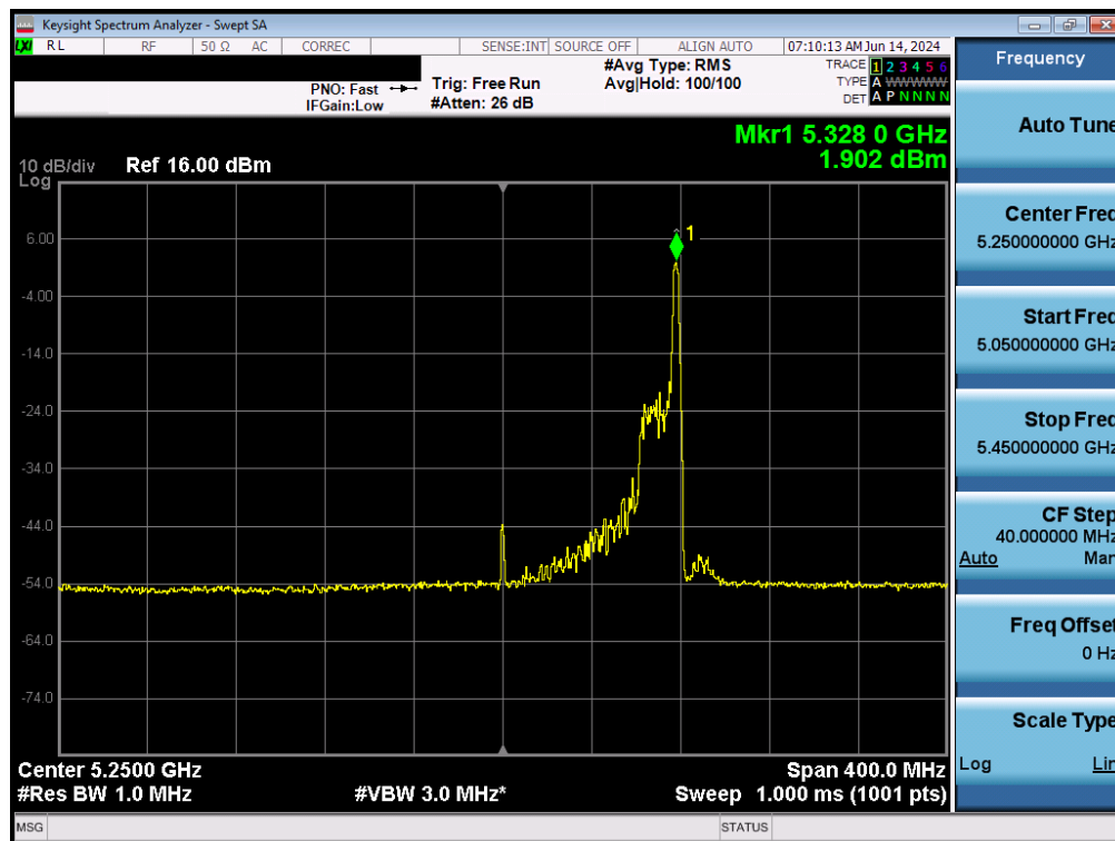
Plot 7-113. Power Spectral Density Plot MIMO ANT2 (160MHz BW 802.11ax – 26 Tones (UNII Band 1/2A) – Ch. 50)
