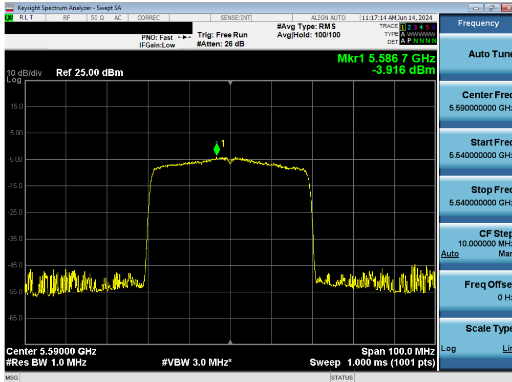
Plot 7-100. Power Spectral Density Plot MIMO ANT1 (40MHz BW 802.11ax – 484 Tones (UNII Band 2C) – Ch. 118)
