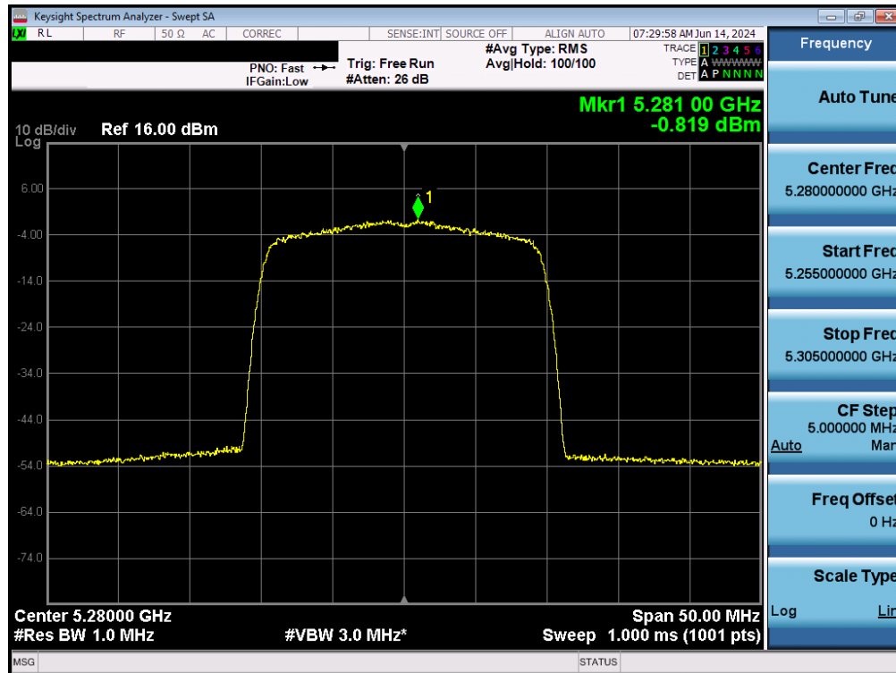
Plot 7-132. Power Spectral Density Plot MIMO ANT2 (20MHz BW 802.11ax – 242 Tones (UNII Band 2A) – Ch. 56)
