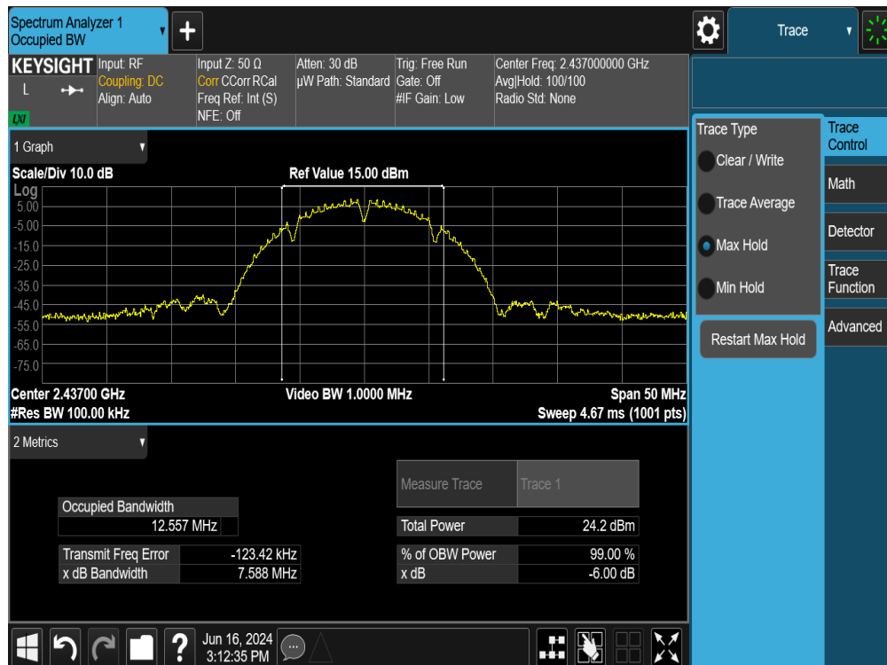
Plot 7-39. 6dB Bandwidth Plot MIMO ANT2 (802.11b – Ch. 6)
