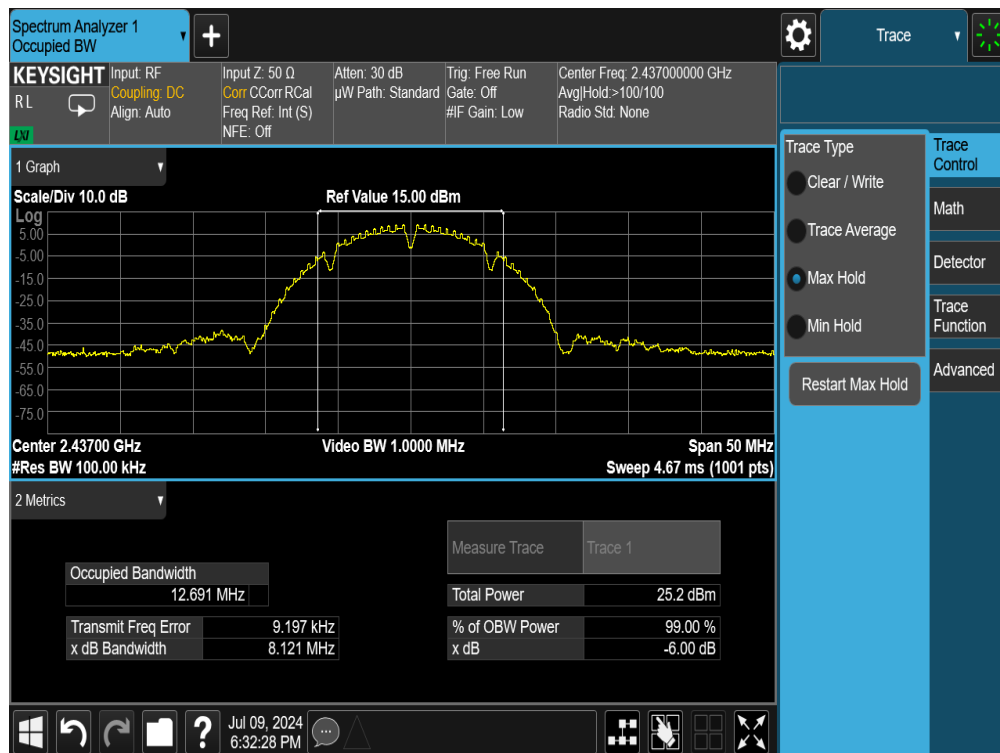
Plot 7-3. 6dB Bandwidth Plot SISO ANT1 (802.11b – Ch. 6)
