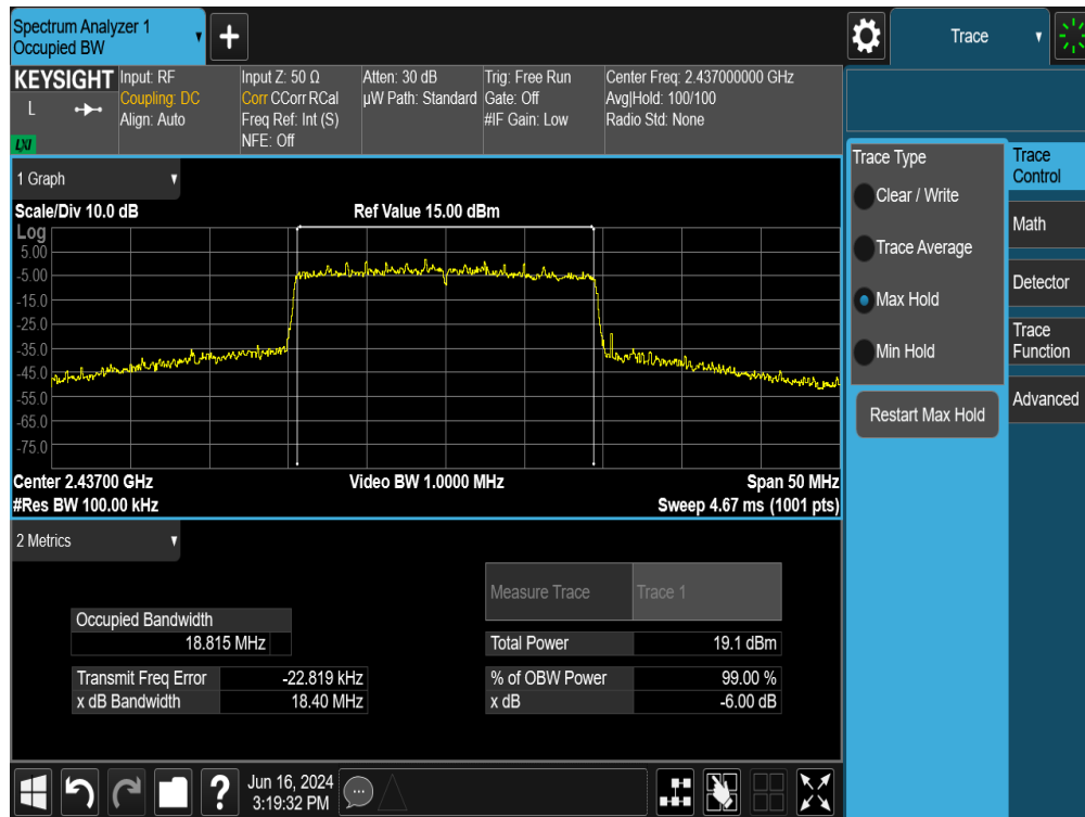
Plot 7-36. 6dB Bandwidth Plot MIMO ANT1 (802.11ax (2.4GHz) – Ch. 6)
