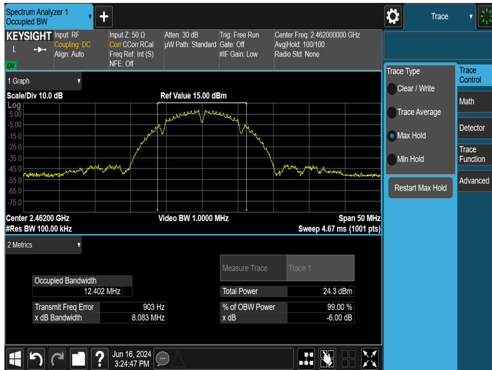
Plot 7-28. 6dB Bandwidth Plot MIMO ANT1 (802.11b – Ch. 11)
