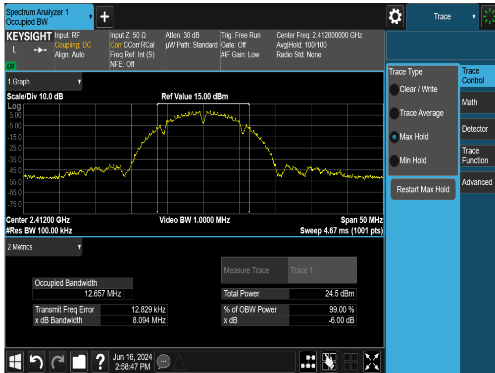
Plot 7-38. 6dB Bandwidth Plot MIMO ANT2 (802.11b – Ch. 1)
