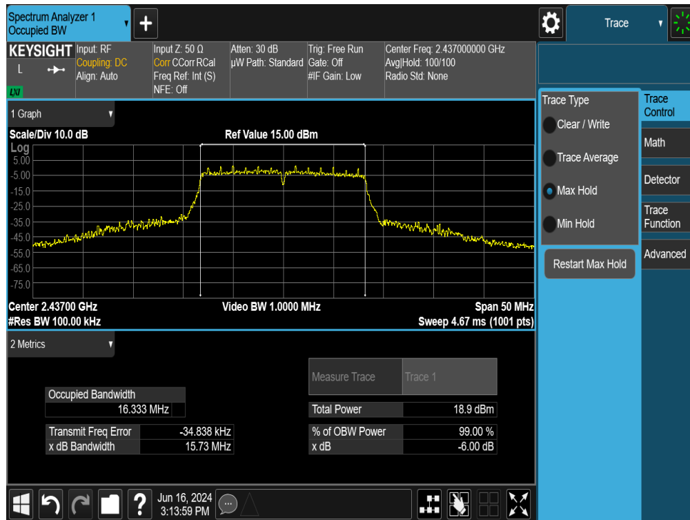
Plot 7-30. 6dB Bandwidth Plot MIMO ANT1 (802.11g - Ch. 6)
