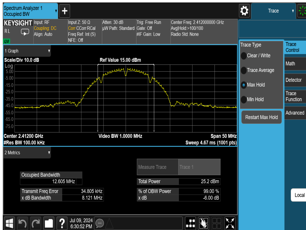
Plot 7-2. 6dB Bandwidth Plot SISO ANT1 (802.11b – Ch. 1)
