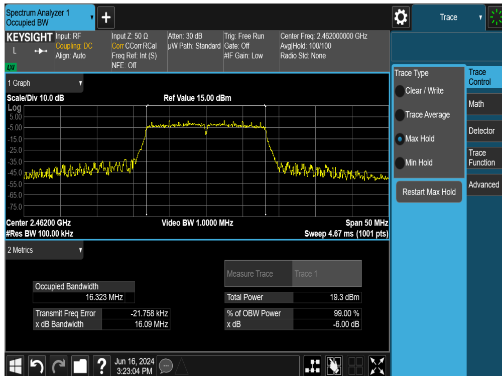
Plot 7-31. 6dB Bandwidth Plot MIMO ANT1 (802.11g - Ch. 11)
