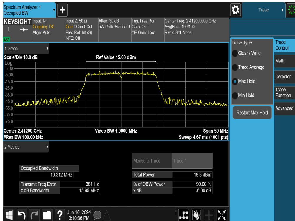
Plot 7-29. 6dB Bandwidth Plot MIMO ANT1 (802.11g – Ch. 1)
