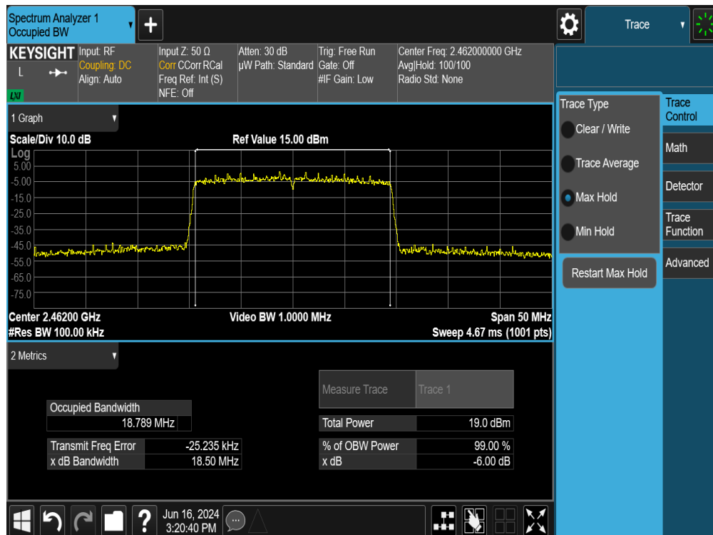
Plot 7-37. 6dB Bandwidth Plot MIMO ANT1 (802.11ax (2.4GHz) – Ch. 11)
