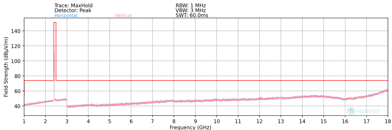
Plot 7-197. Radiated Spurious Plot above 1GHz MIMO (802.11b – Ch. 1)
