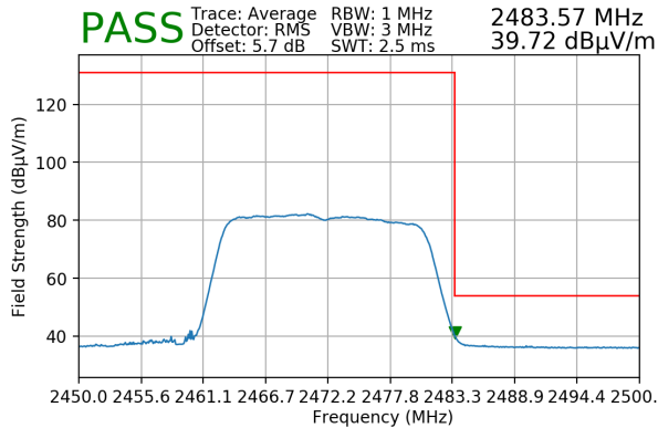
Plot 7-223. Radiated Restricted Upper Band Edge Measurement SISO ANT2 (Average)
