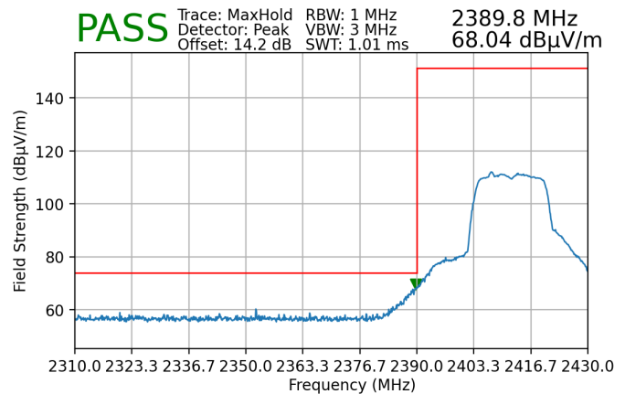
Plot 7-202. Radiated Restricted Lower Band Edge Measurement SISO ANT1 (Peak)
