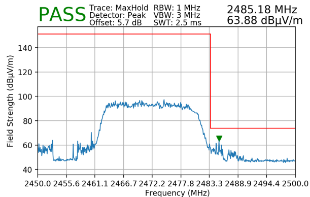
Plot 7-212. Radiated Restricted Upper Band Edge Measurement SISO ANT1 (Peak)
