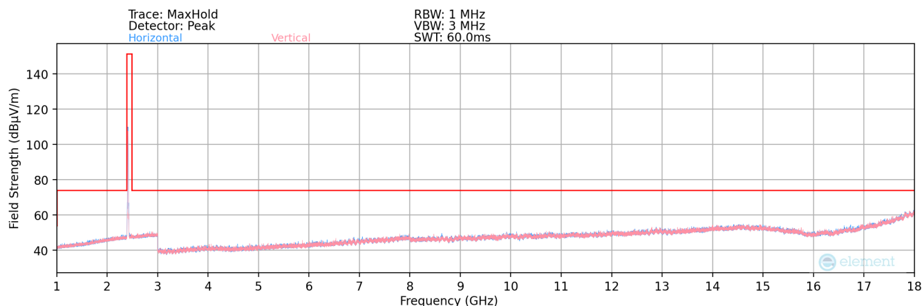
Plot 7-193. Radiated Spurious Plot above 1GHz SISO ANT2 (802.11b – Ch. 6)
