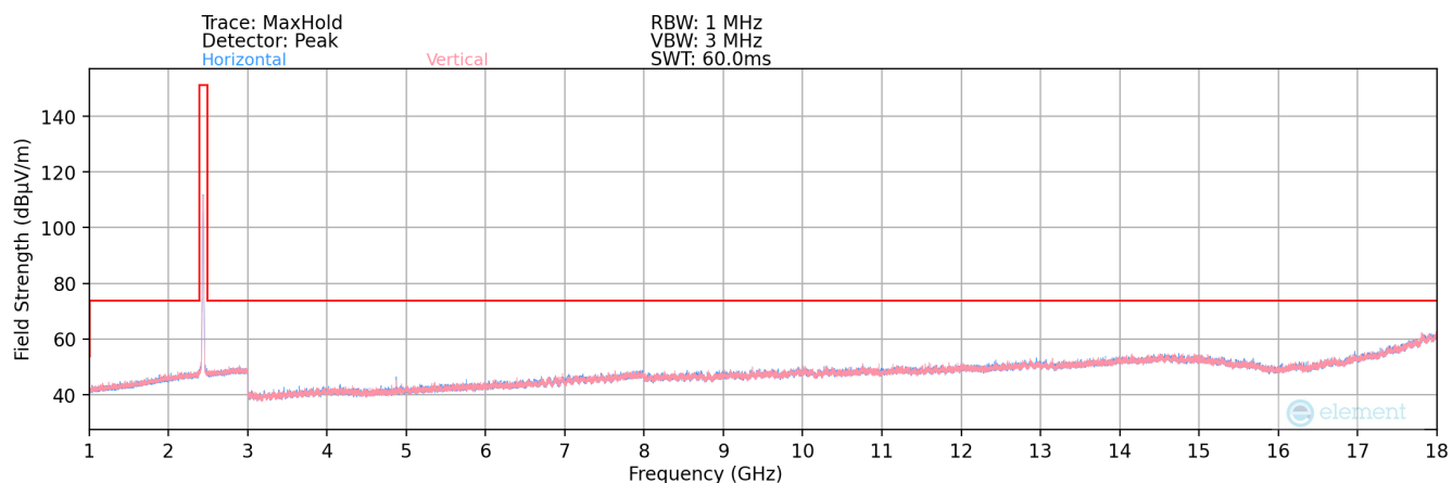
Plot 7-198. Radiated Spurious Plot above 1GHz MIMO (802.11b – Ch. 6)
