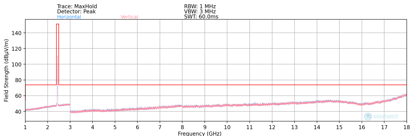
Plot 7-192. Radiated Spurious Plot above 1GHz SISO ANT2 (802.11b – Ch. 1)
