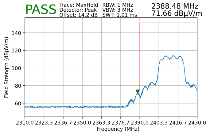
Plot 7-226. Radiated Restricted Lower Band Edge Measurement MIMO (Peak)
