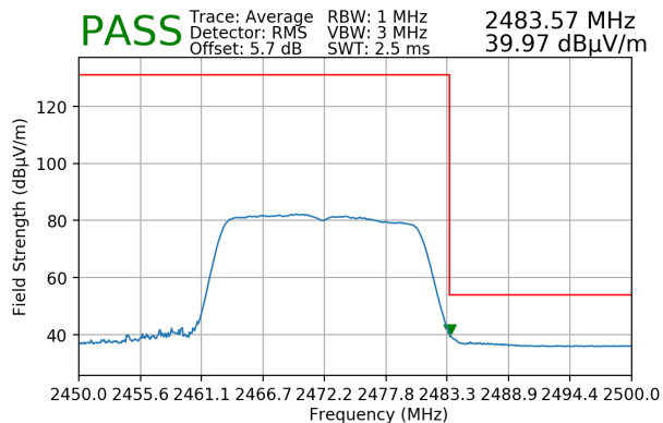
Plot 7-211. Radiated Restricted Upper Band Edge Measurement SISO ANT1 (Average)
