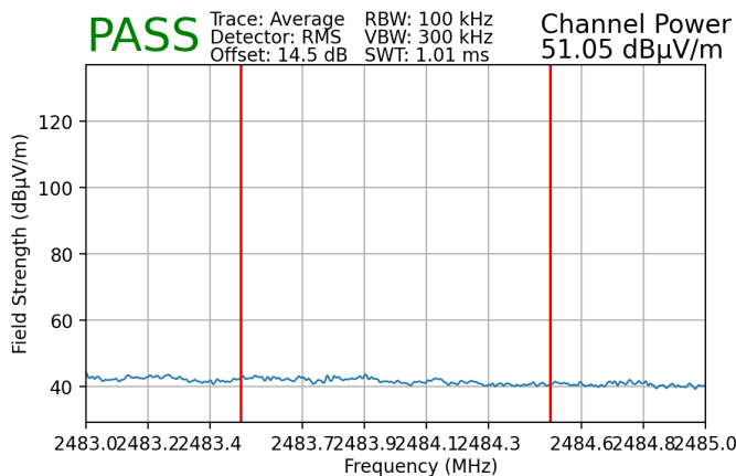
Plot 7-219. Radiated Restricted Upper Band Edge Measurement SISO ANT2 (Average)
