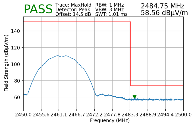
Plot 7-208. Radiated Restricted Upper Band Edge Measurement SISO ANT1 (Peak)
