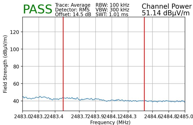
Plot 7-231. Radiated Restricted Upper Band Edge Measurement MIMO (Average)
