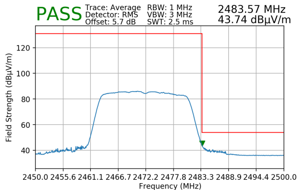
Plot 7-235. Radiated Restricted Upper Band Edge Measurement MIMO (Average)
