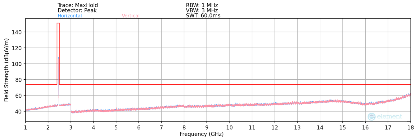
Plot 7-194. Radiated Spurious Plot above 1GHz SISO ANT2 (802.11b – Ch. 11)
