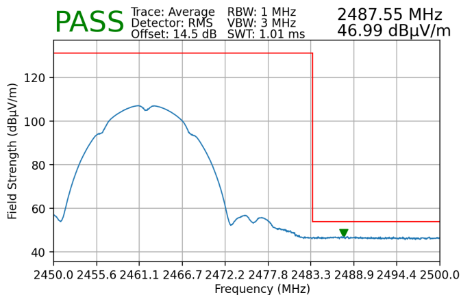
Plot 7-207. Radiated Restricted Upper Band Edge Measurement SISO ANT1 (Average)
