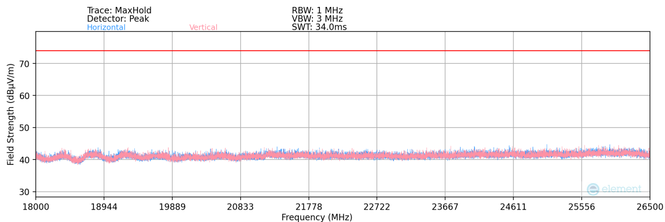
Plot 7-200. Radiated Spurious Plot above 18GHz MIMO
