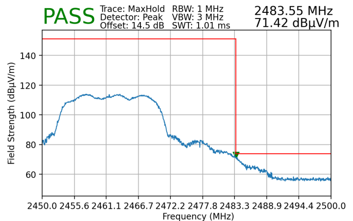
Plot 7-232. Radiated Restricted Upper Band Edge Measurement MIMO (Peak)
