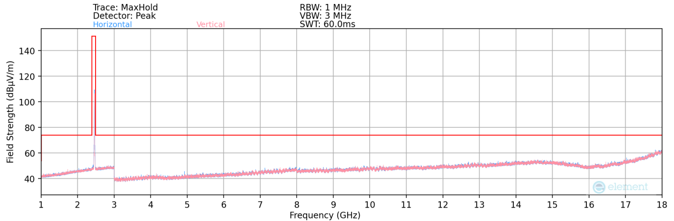
Plot 7-189. Radiated Spurious Plot above 1GHz SISO ANT1 (802.11b – Ch. 11)
