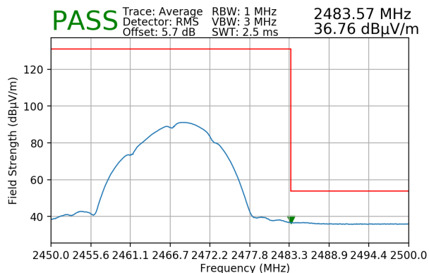
Plot 7-209. Radiated Restricted Upper Band Edge Measurement SISO ANT1 (Average)
