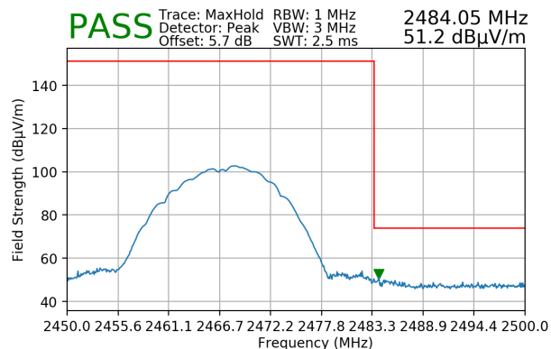
Plot 7-210. Radiated Restricted Upper Band Edge Measurement SISO ANT1 (Peak)
