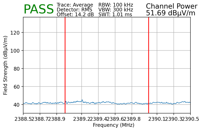
Plot 7-225. Radiated Restricted Lower Band Edge Measurement MIMO (Average)
