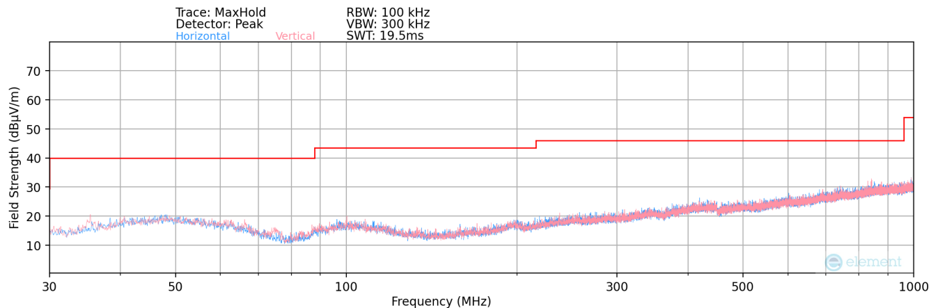
Plot 7-196. Radiated Spurious Plot below 1GHz MIMO
