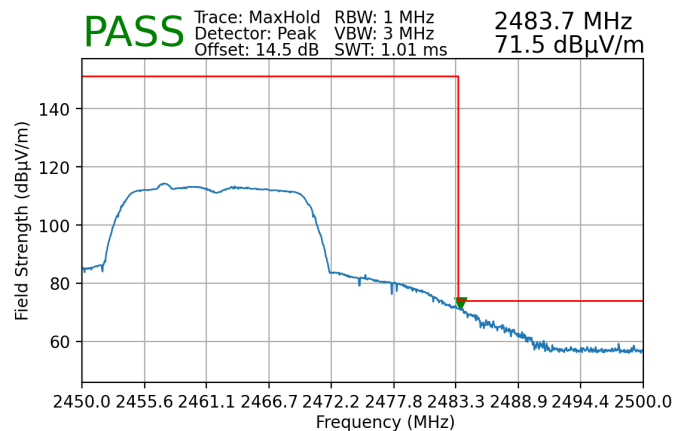
Plot 7-220. Radiated Restricted Upper Band Edge Measurement SISO ANT2 (Peak)
