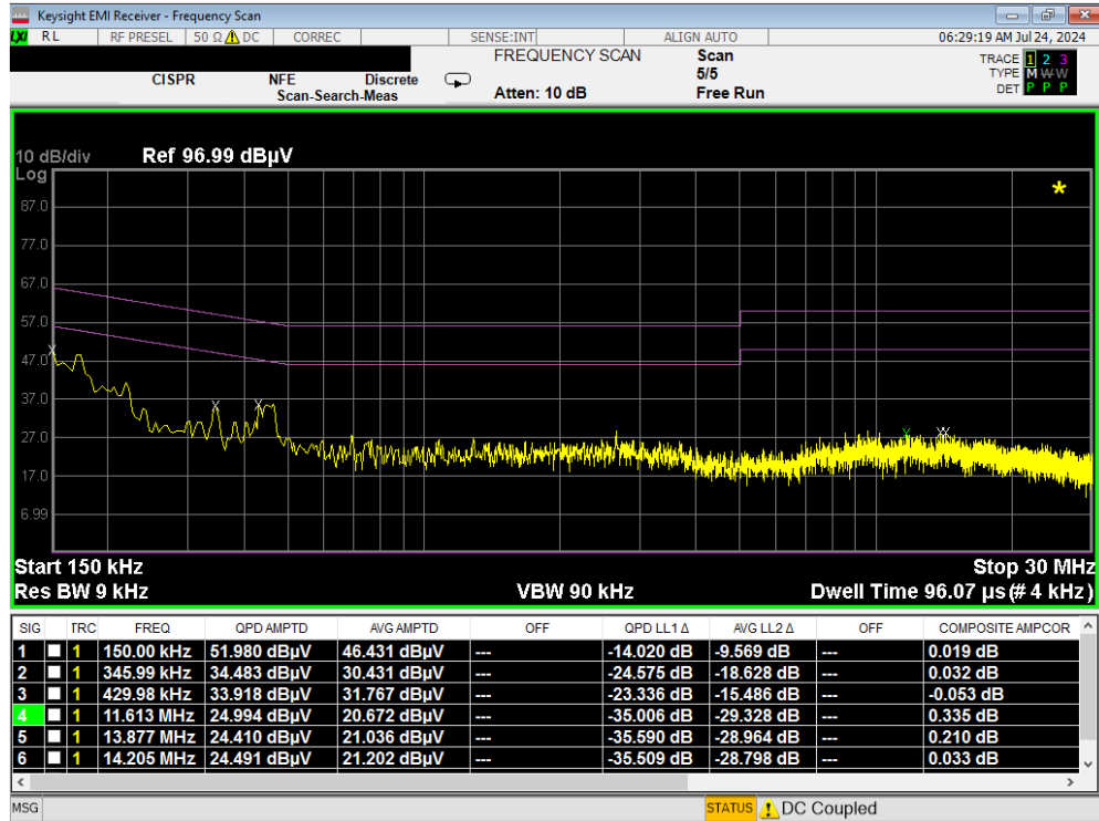
Plot 7-237. Line Conducted Plot with 802.11b (L1)
