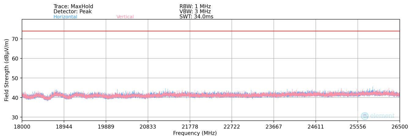
Plot 7-195. Radiated Spurious Plot above 18GHz SISO ANT2
