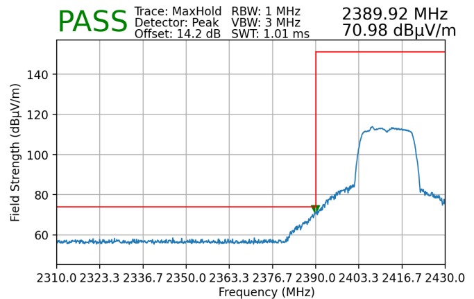
Plot 7-214. Radiated Restricted Lower Band Edge Measurement SISO ANT2 (Peak)
