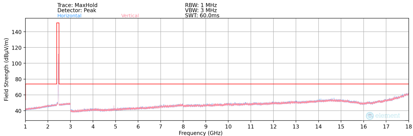
Plot 7-199. Radiated Spurious Plot above 1GHz MIMO (802.11b – Ch. 11)
