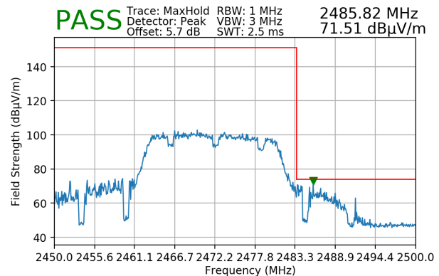
Plot 7-236. Radiated Restricted Upper Band Edge Measurement MIMO (Peak)
