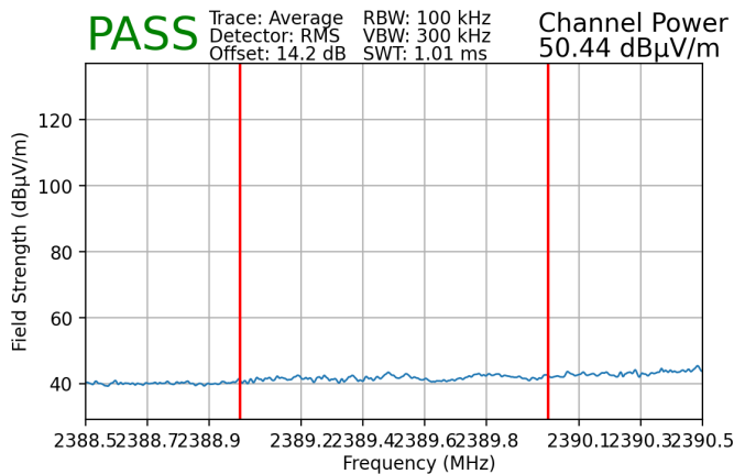
Plot 7-213. Radiated Restricted Lower Band Edge Measurement SISO ANT2 (Average)
