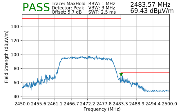
Plot 7-224. Radiated Restricted Upper Band Edge Measurement SISO ANT2 (Peak)
