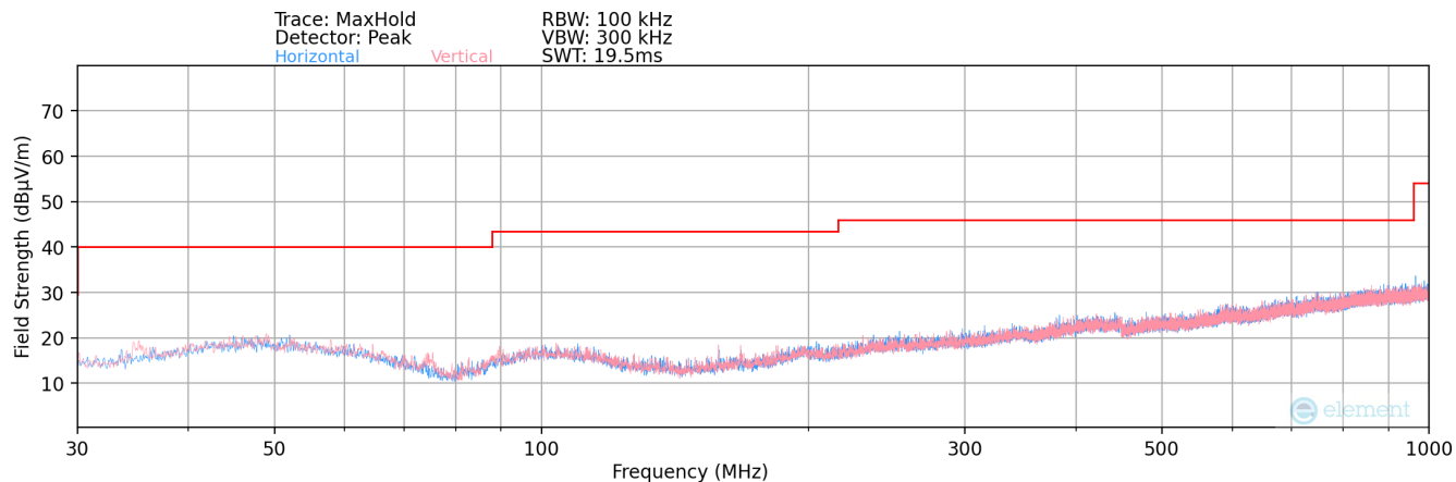
Plot 7-191. Radiated Spurious Plot below 1GHz SISO ANT2
