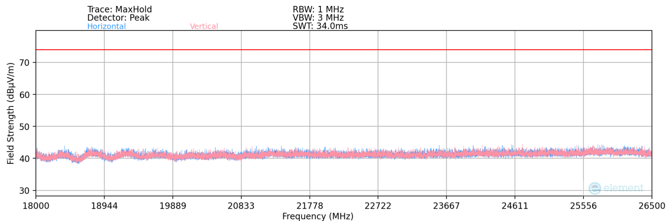
Plot 7-190. Radiated Spurious Plot above 18GHz SISO ANT1
