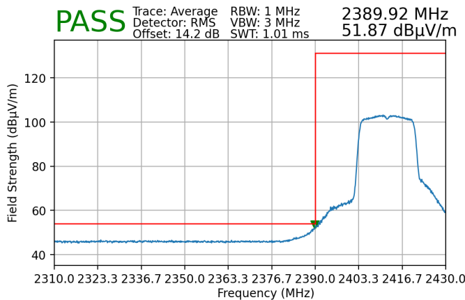
Plot 7-201. Radiated Restricted Lower Band Edge Measurement SISO ANT1 (Average)
