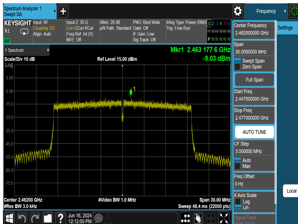
Plot 7-37. Power Spectral Density Plot SISO ANT2 (802.11ax OFDMA – 242 Tones – Ch. 11)
