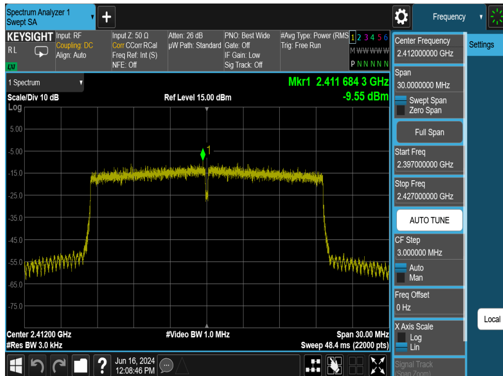
Plot 7-35. Power Spectral Density Plot SISO ANT2 (802.11ax OFDMA – 242 Tones – Ch. 1)
