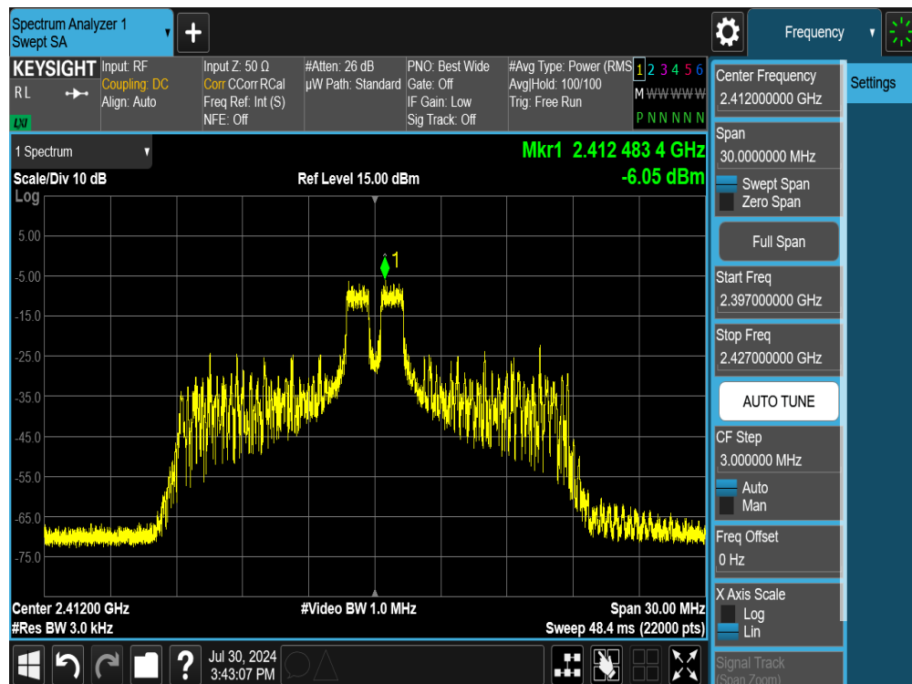
Plot 7-26. Power Spectral Density Plot SISO ANT1 (802.11ax OFDMA – 26 Tones – Ch. 1)
