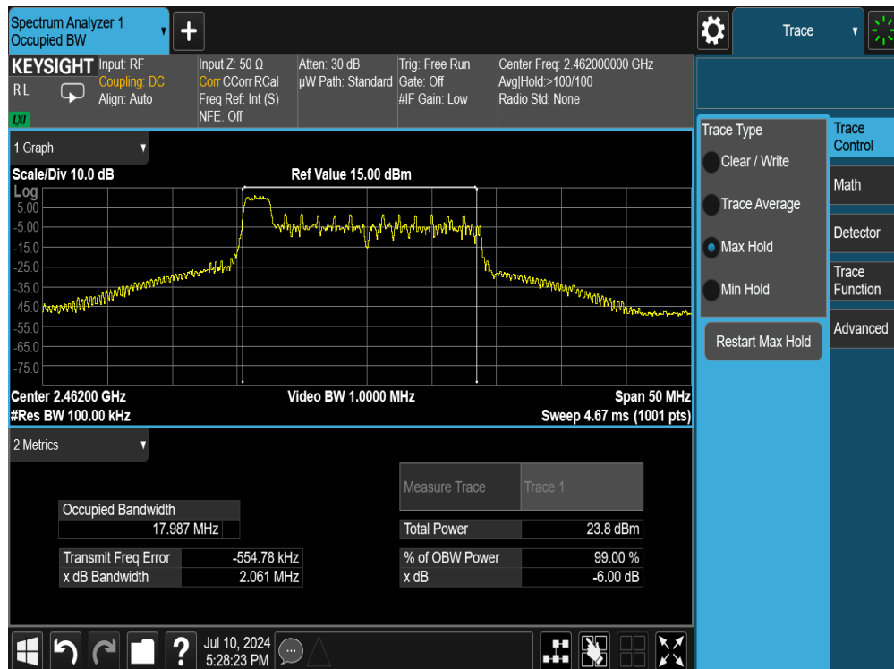
Plot 7-4. 6dB Bandwidth Plot SISO ANT1 (802.11ax OFDMA – 26 Tones – Ch. 11)
