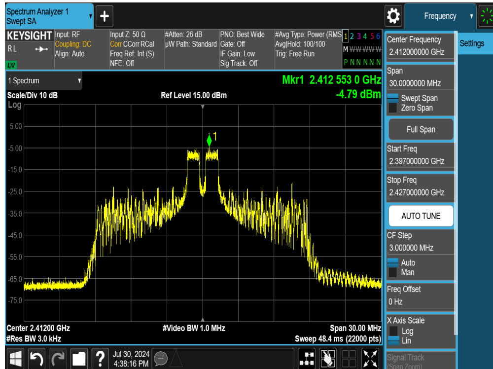
Plot 7-32. Power Spectral Density Plot SISO ANT2 (802.11ax OFDMA – 26 Tones – Ch. 1)
