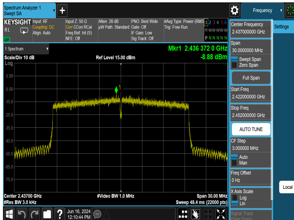
Plot 7-36. Power Spectral Density Plot SISO ANT2 (802.11ax OFDMA – 242 Tones – Ch. 6)
