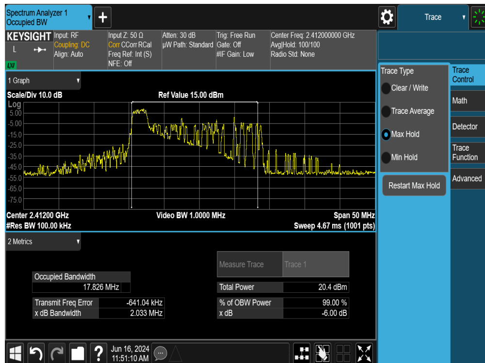
Plot 7-14. 6dB Bandwidth Plot MIMO ANT1 (802.11ax OFDMA – 26Tones – Ch. 1)
