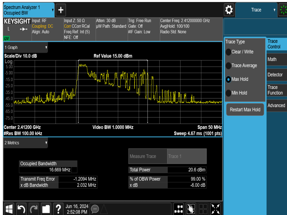
Plot 7-8. 6dB Bandwidth Plot SISO ANT2 (802.11ax OFDMA – 26 Tones – Ch. 1)
