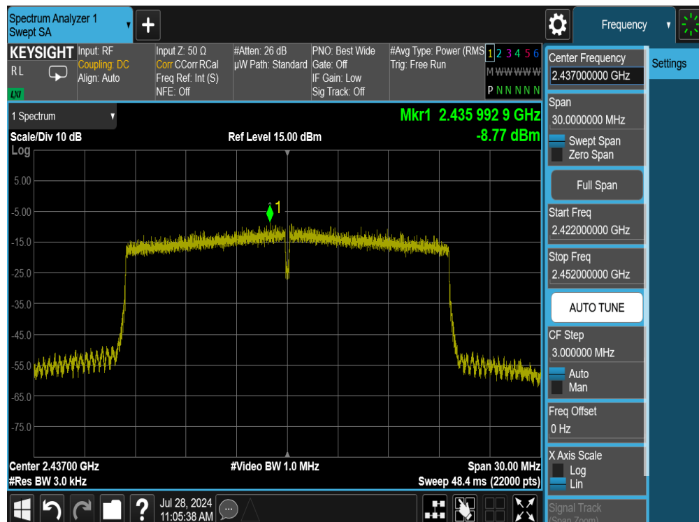
Plot 7-30. Power Spectral Density Plot SISO ANT1 (802.11ax OFDMA – 242 Tones – Ch. 6)
