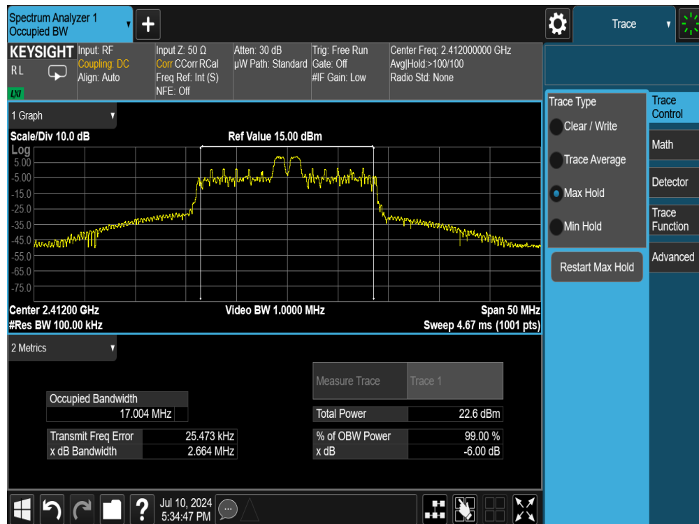
Plot 7-2. 6dB Bandwidth Plot SISO ANT1 (802.11ax OFDMA – 26 Tones – Ch. 1)
