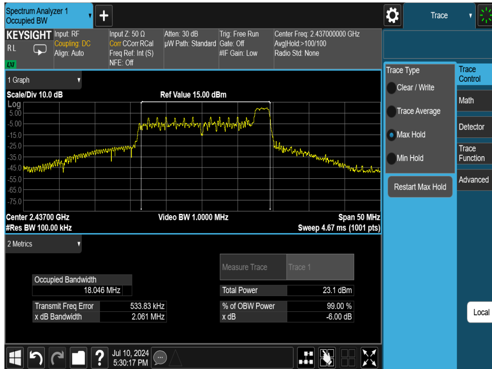
Plot 7-3. 6dB Bandwidth Plot SISO ANT1 (802.11ax OFDMA – 26 Tones – Ch. 6)
