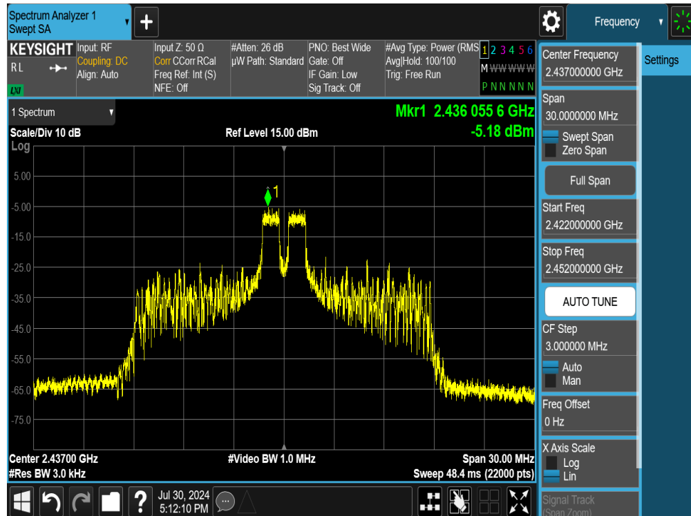
Plot 7-39. Power Spectral Density Plot MIMO ANT2 (802.11ax OFDMA – 26 Tones – Ch. 6)
