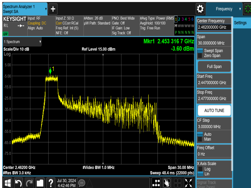
Plot 7-34. Power Spectral Density Plot SISO ANT2 (802.11ax OFDMA – 26 Tones – Ch. 11)
