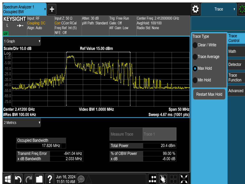
Plot 7-20. 6dB Bandwidth Plot MIMO ANT2 (802.11ax OFDMA – 26Tones – Ch. 1)
