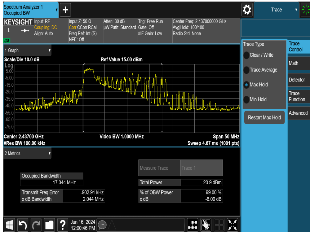
Plot 7-21. 6dB Bandwidth Plot MIMO ANT2 (802.11ax OFDMA – 26Tones – Ch. 6)
