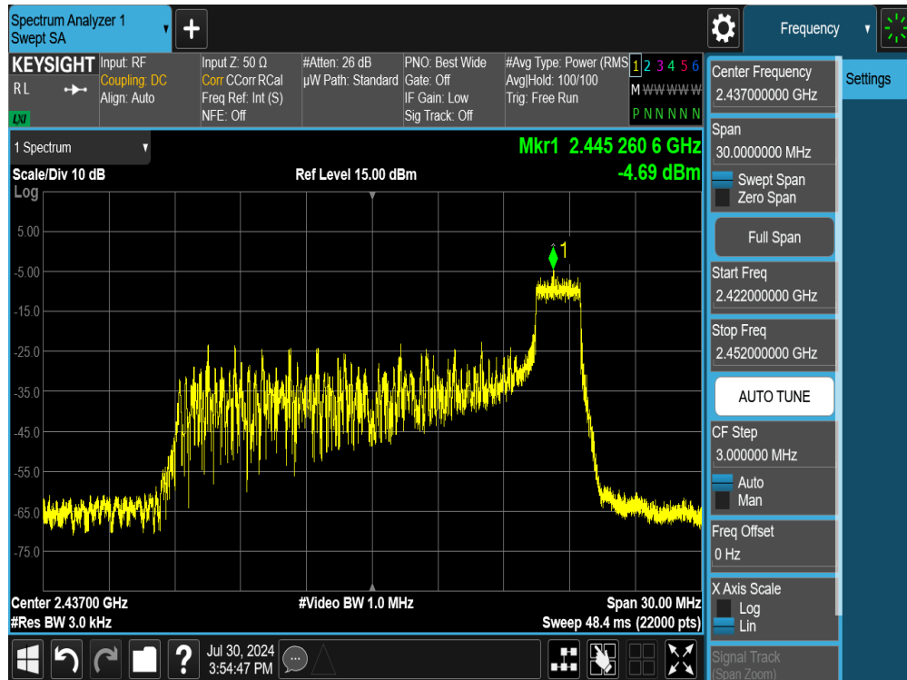
Plot 7-27. Power Spectral Density Plot SISO ANT1 (802.11ax OFDMA – 26 Tones – Ch. 6)
