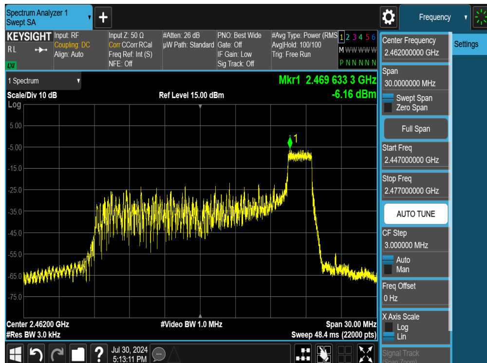
Plot 7-40. Power Spectral Density Plot MIMO ANT1 (802.11ax OFDMA – 26 Tones – Ch. 11)
