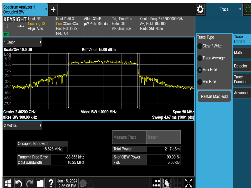
Plot 7-13. 6dB Bandwidth Plot SISO ANT2 (802.11ax OFDMA – 242 Tones – Ch. 11)
