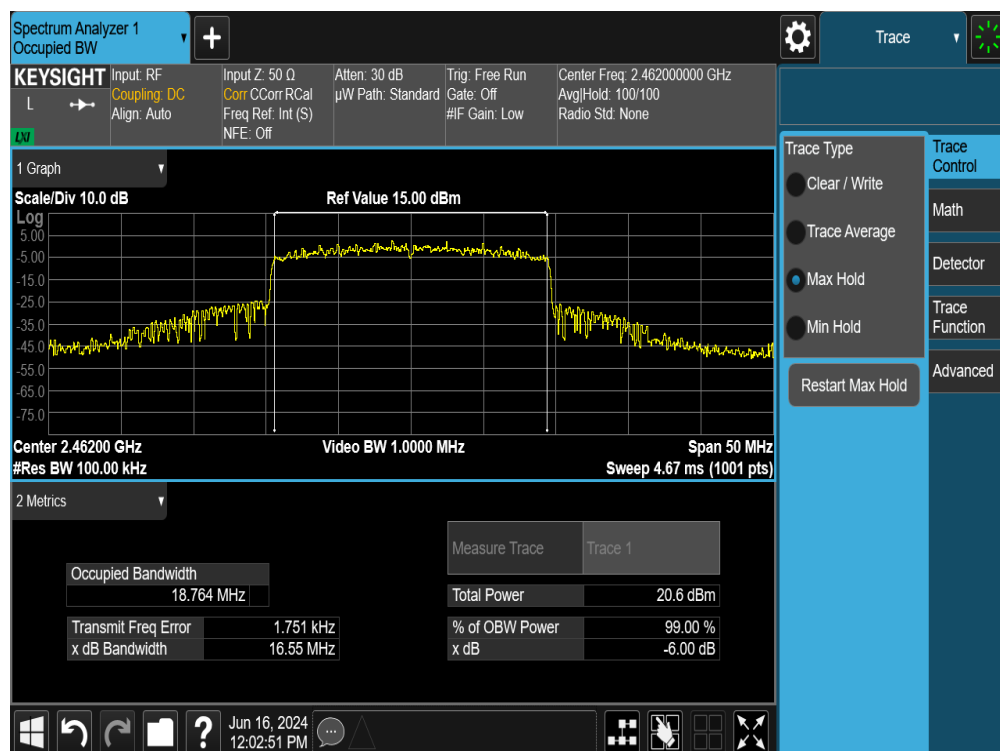
Plot 7-19. 6dB Bandwidth Plot MIMO ANT1 (802.11ax OFDMA – 242Tones – Ch. 11)
