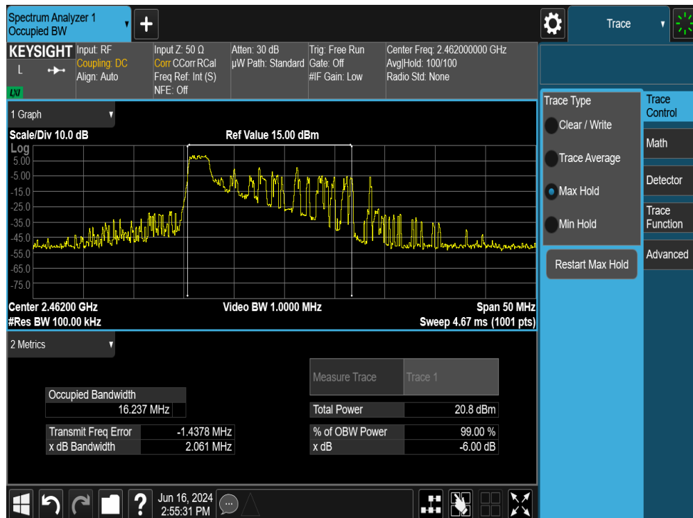
Plot 7-10. 6dB Bandwidth Plot SISO ANT2 (802.11ax OFDMA – 26 Tones – Ch. 11)
