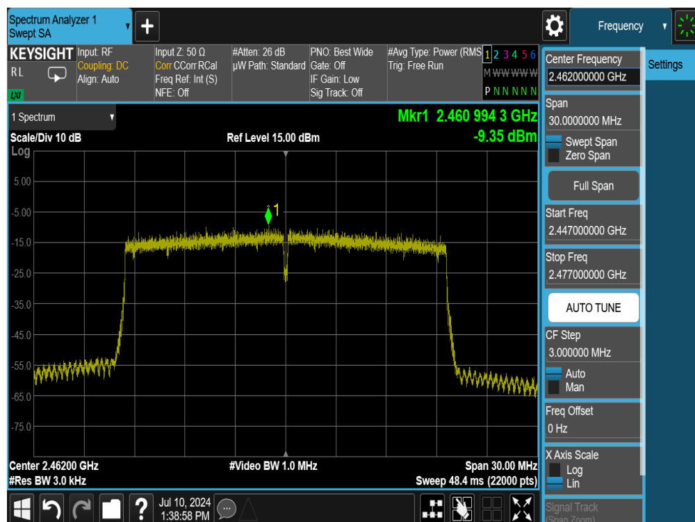
Plot 7-31. Power Spectral Density Plot SISO ANT1 (802.11ax OFDMA – 242 Tones – Ch. 11)
