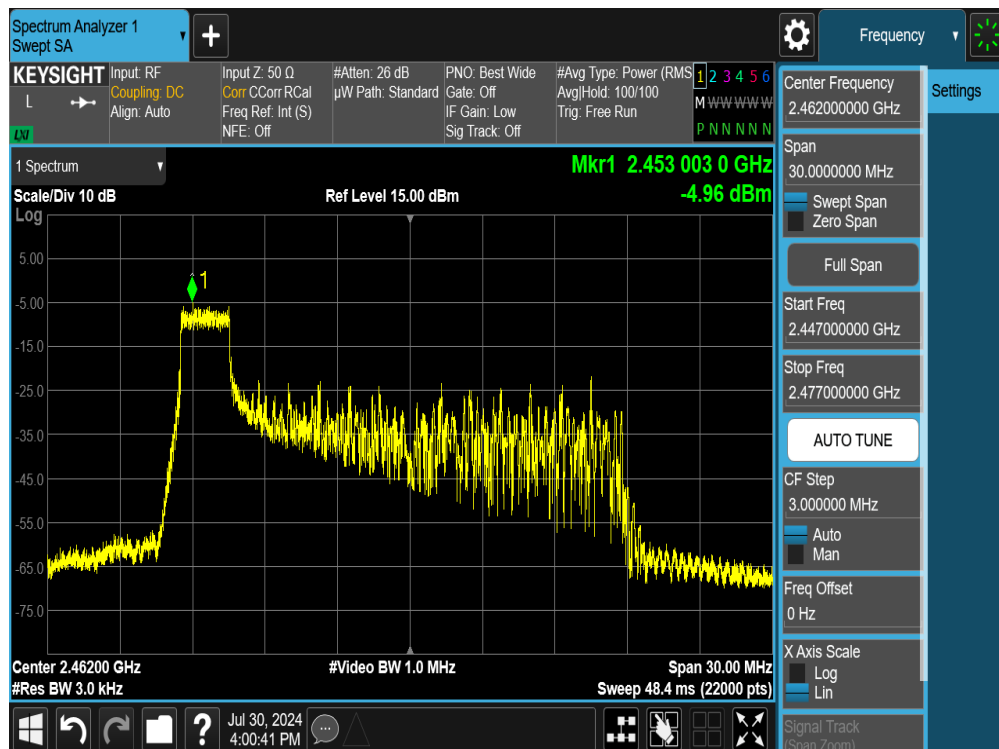
Plot 7-28. Power Spectral Density Plot SISO ANT1 (802.11ax OFDMA – 26 Tones – Ch. 11)
