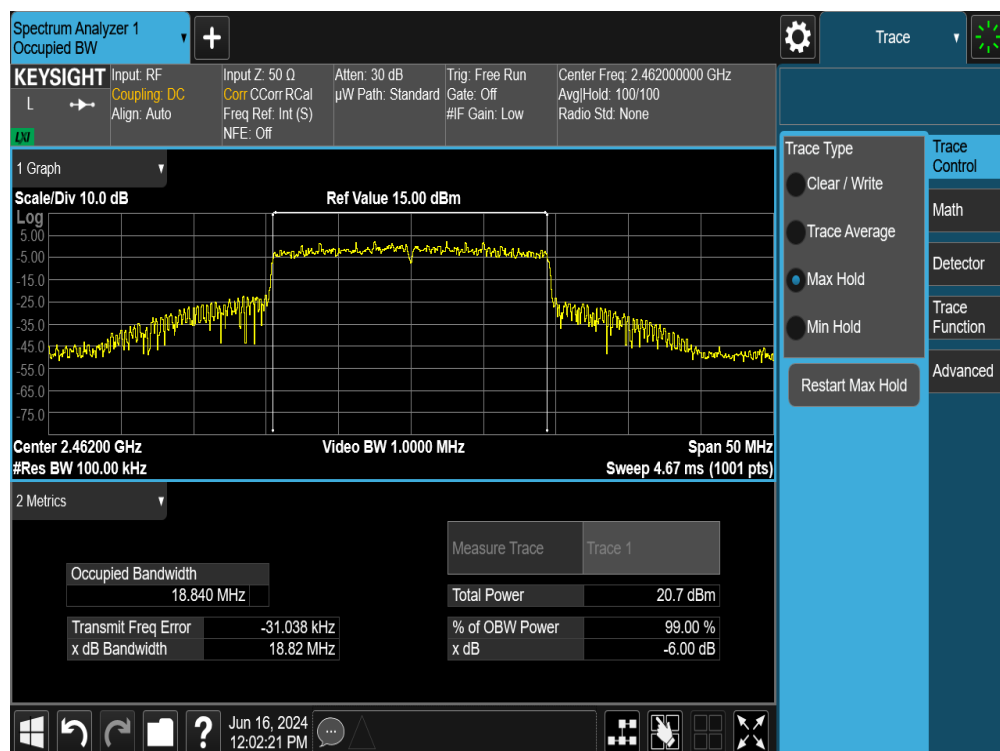
Plot 7-25. 6dB Bandwidth Plot MIMO ANT2 (802.11ax OFDMA – 242Tones – Ch. 11)
