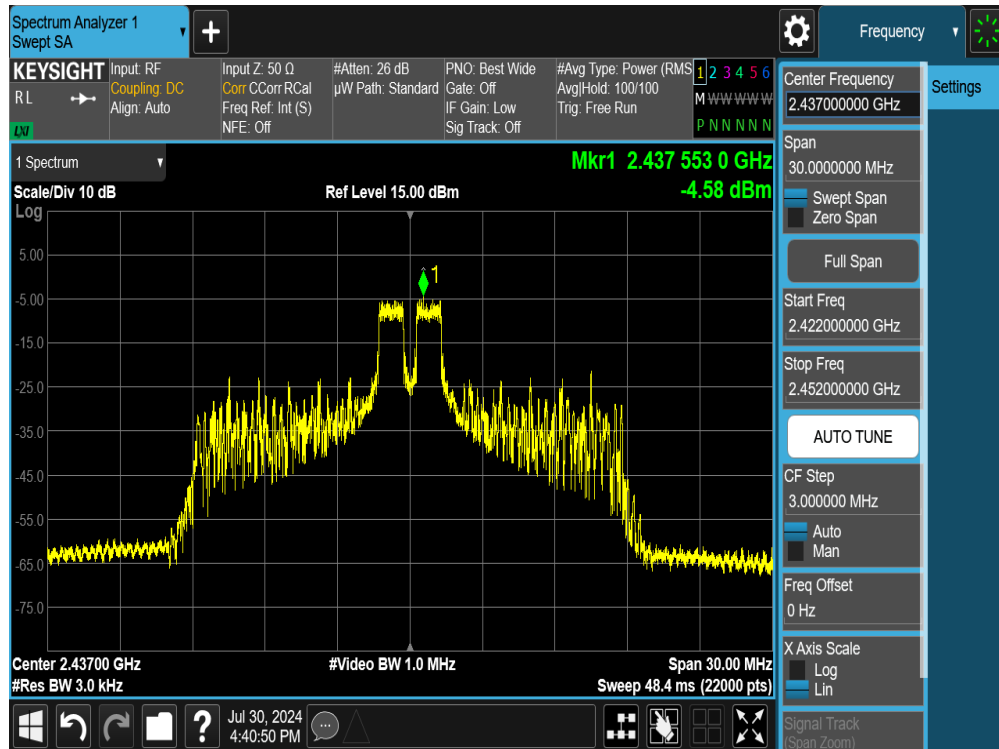
Plot 7-33. Power Spectral Density Plot SISO ANT2 (802.11ax OFDMA – 26 Tones – Ch. 6)
