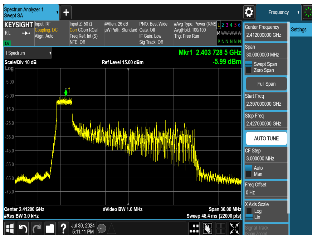
Plot 7-38. Power Spectral Density Plot MIMO ANT1 (802.11ax OFDMA – 26 Tones – Ch. 1)
