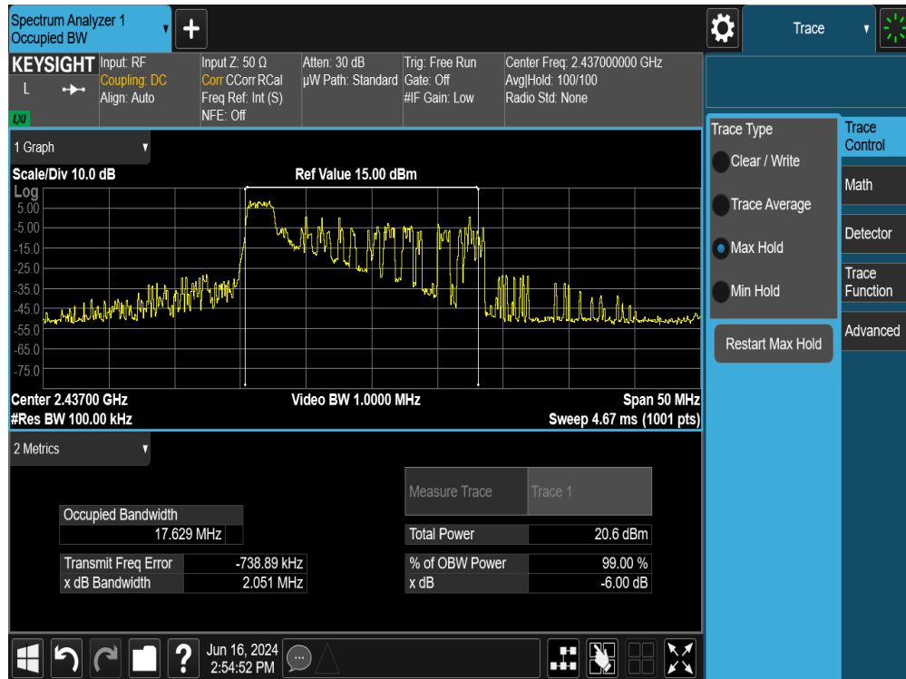
Plot 7-9. 6dB Bandwidth Plot SISO ANT2 (802.11ax OFDMA – 26 Tones – Ch. 6)
