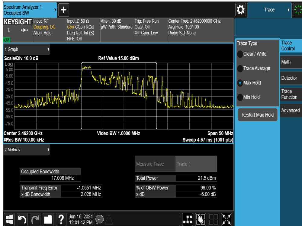
Plot 7-22. 6dB Bandwidth Plot MIMO ANT2 (802.11ax OFDMA – 26Tones – Ch. 11)
