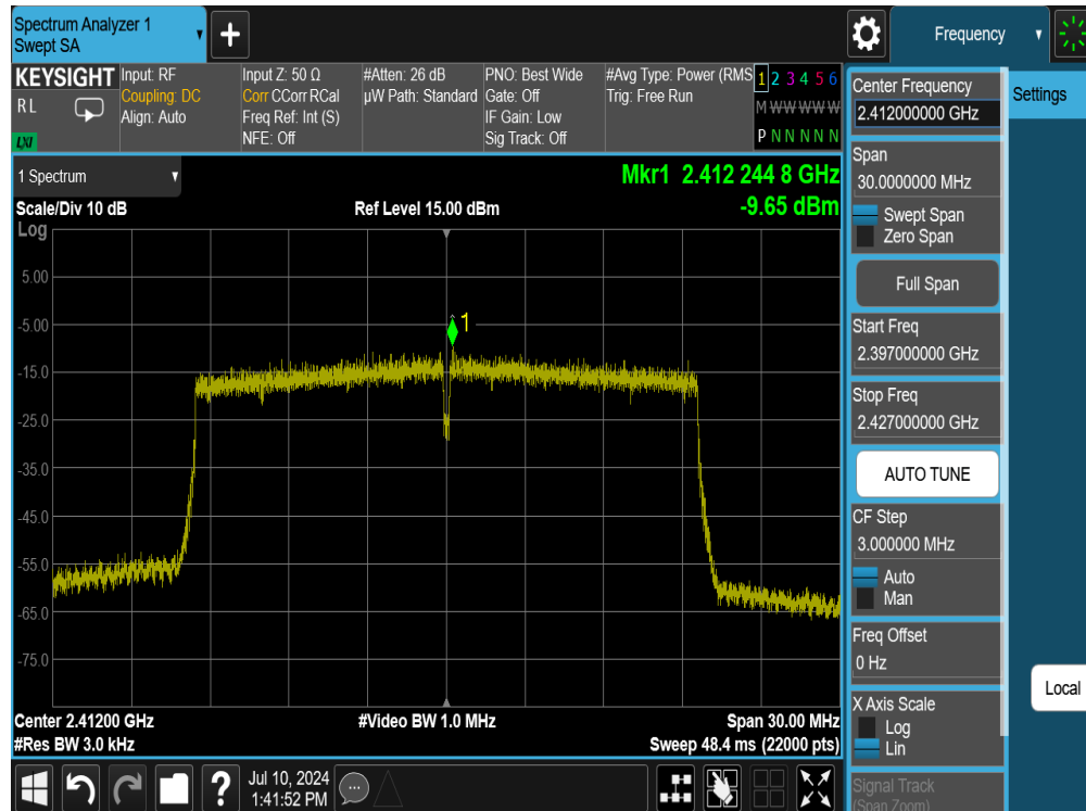
Plot 7-29. Power Spectral Density Plot SISO ANT1 (802.11ax OFDMA – 242 Tones – Ch. 1)
