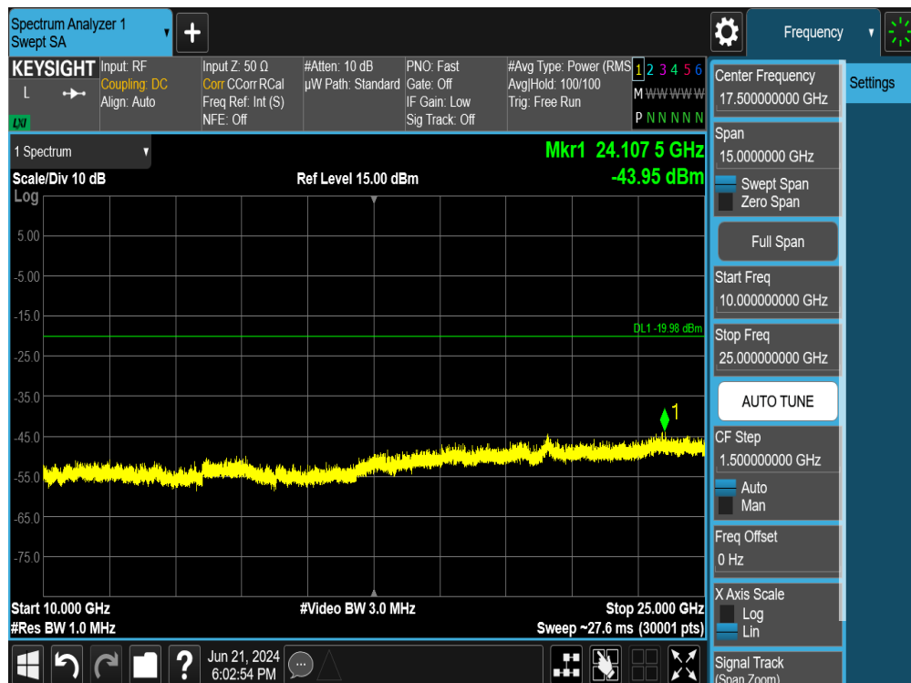
Plot 7-123. Conducted Spurious Plot MIMO ANT2 (802.11ax OFDMA – 26 Tones – Ch. 11)
