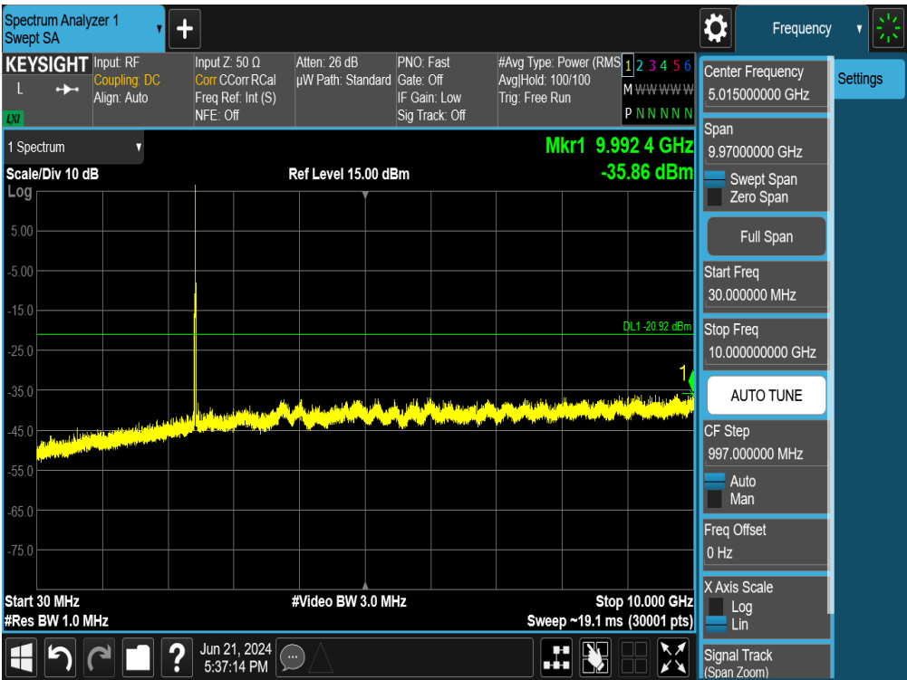
Plot 7-120. Conducted Spurious Plot MIMO ANT2 (802.11ax OFDMA – 26 Tones – Ch. 6)
