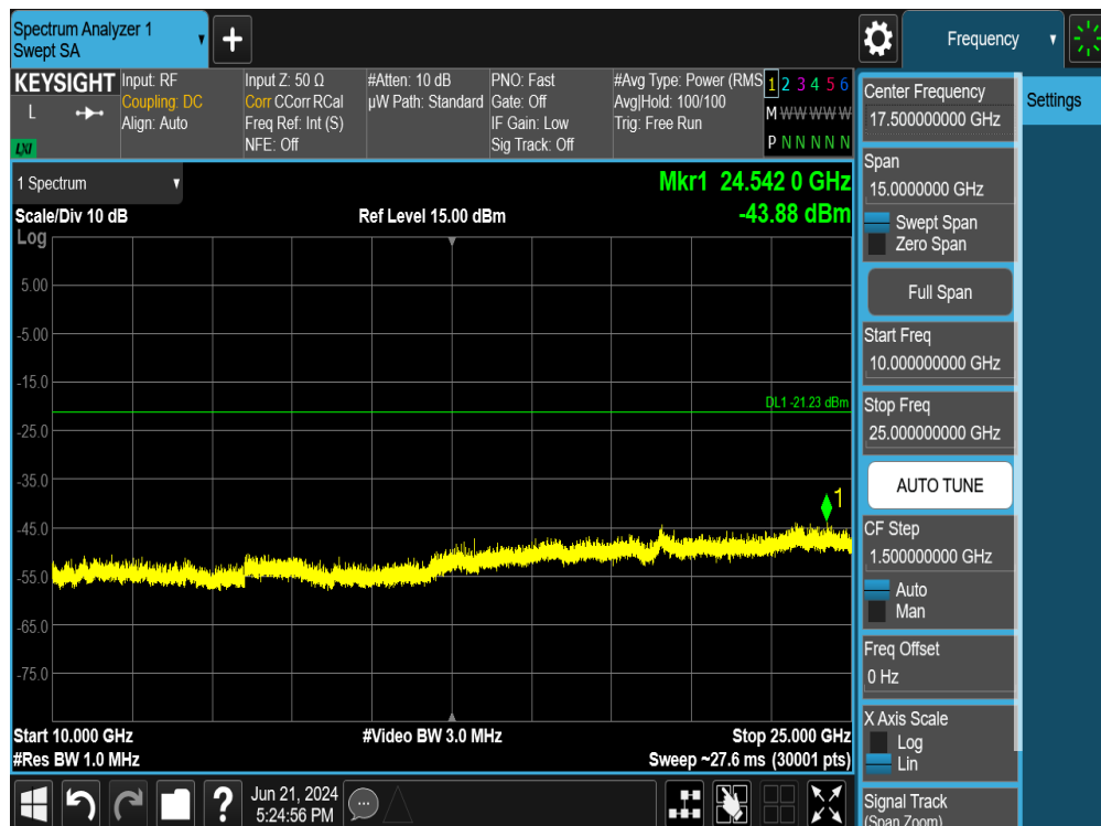
Plot 7-99. Conducted Spurious Plot SISO ANT2 (802.11ax OFDMA – 26 Tones – Ch. 11)
