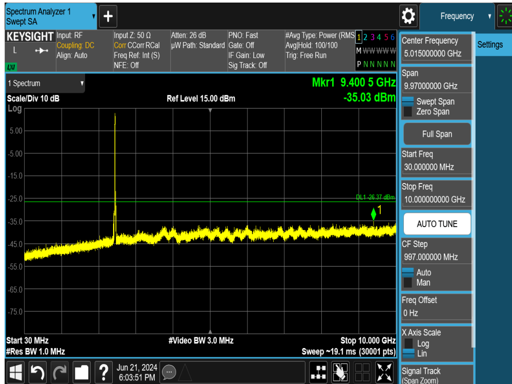
Plot 7-128. Conducted Spurious Plot MIMO ANT2 (802.11ax OFDMA – 242 Tones – Ch. 11)
