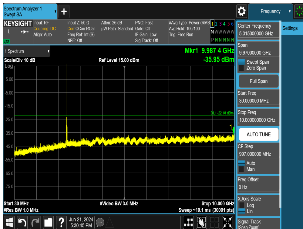
Plot 7-106. Conducted Spurious Plot MIMO ANT1 (802.11ax OFDMA – 26 Tones – Ch. 1)
