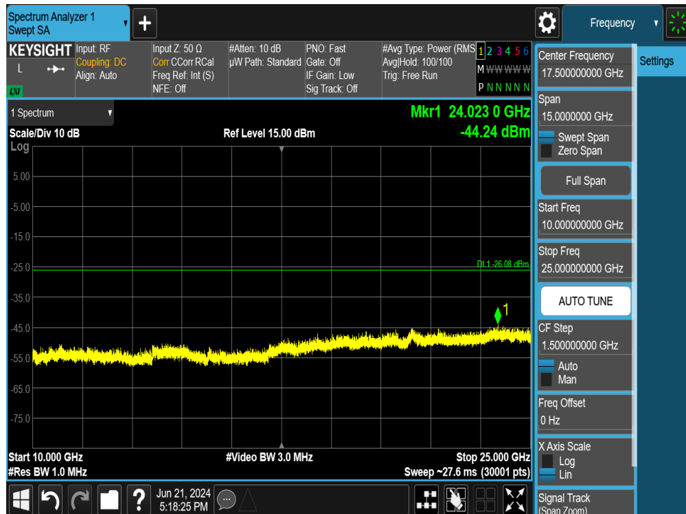
Plot 7-101. Conducted Spurious Plot SISO ANT2 (802.11ax OFDMA – 242 Tones – Ch. 1)
