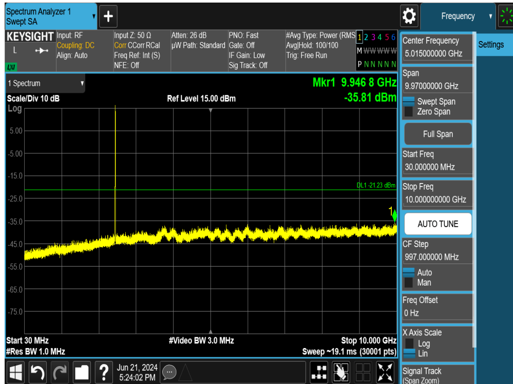
Plot 7-98. Conducted Spurious Plot SISO ANT2 (802.11ax OFDMA – 26 Tones – Ch. 11)
