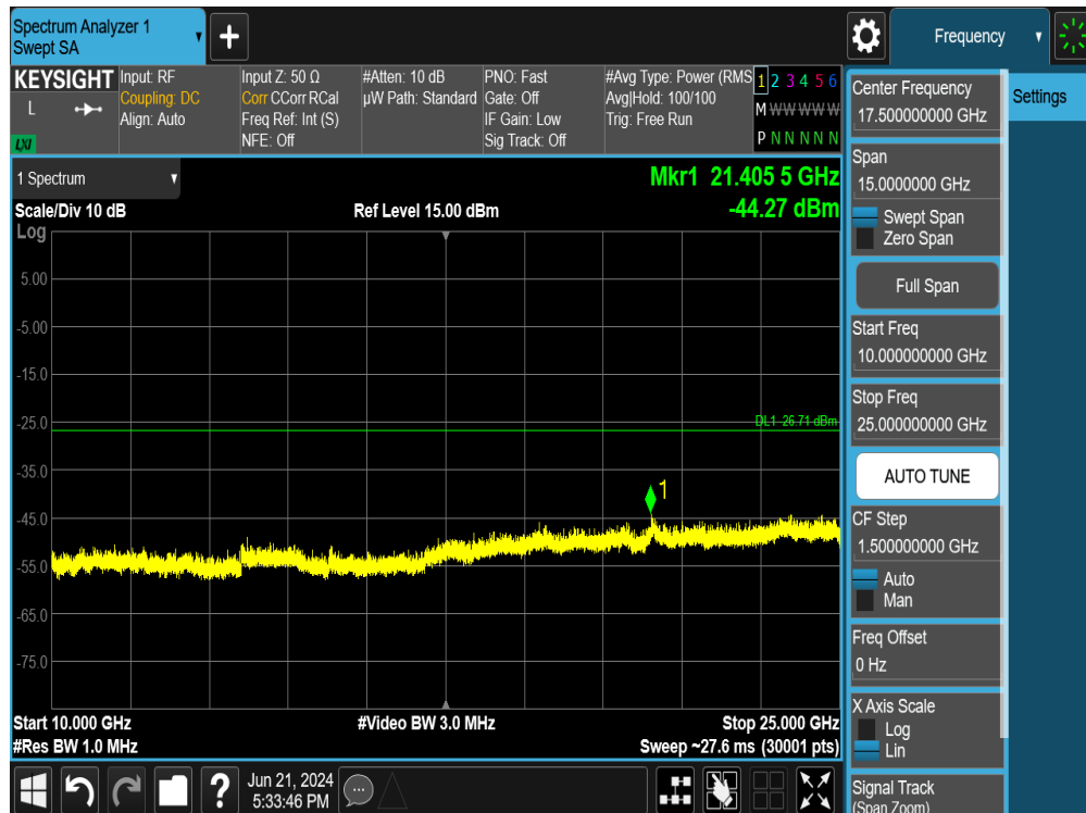
Plot 7-113. Conducted Spurious Plot MIMO ANT1 (802.11ax OFDMA – 242 Tones – Ch. 1)
