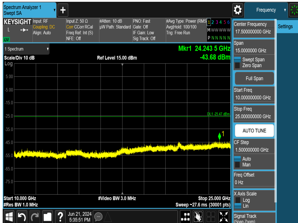
Plot 7-125. Conducted Spurious Plot MIMO ANT2 (802.11ax OFDMA – 242 Tones – Ch. 1)
