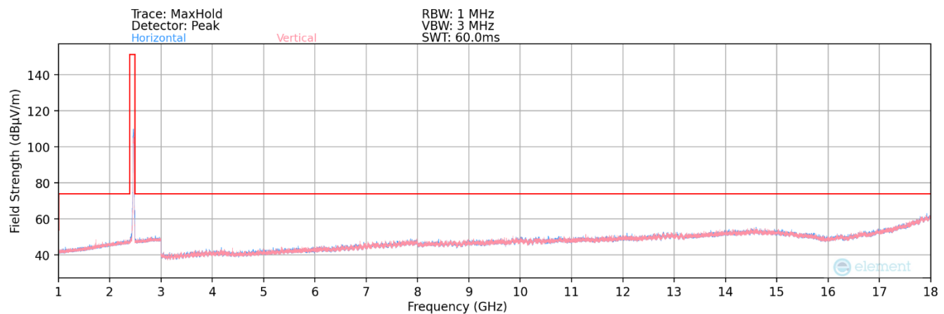
Plot 7-135. Radiated Spurious Plot above 1GHz – SISO ANT1 (802.11ax OFDMA – 242 Tones – Ch. 11)
