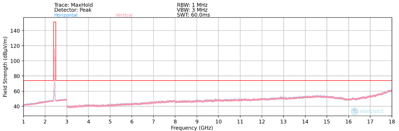
Plot 7-137. Radiated Spurious Plot above 1GHz – SISO ANT2 (802.11ax OFDMA – 26 Tones – Ch. 6)
