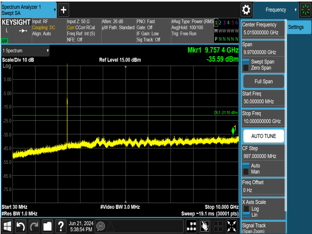
Plot 7-108. Conducted Spurious Plot MIMO ANT1 (802.11ax OFDMA – 26 Tones – Ch. 6)
