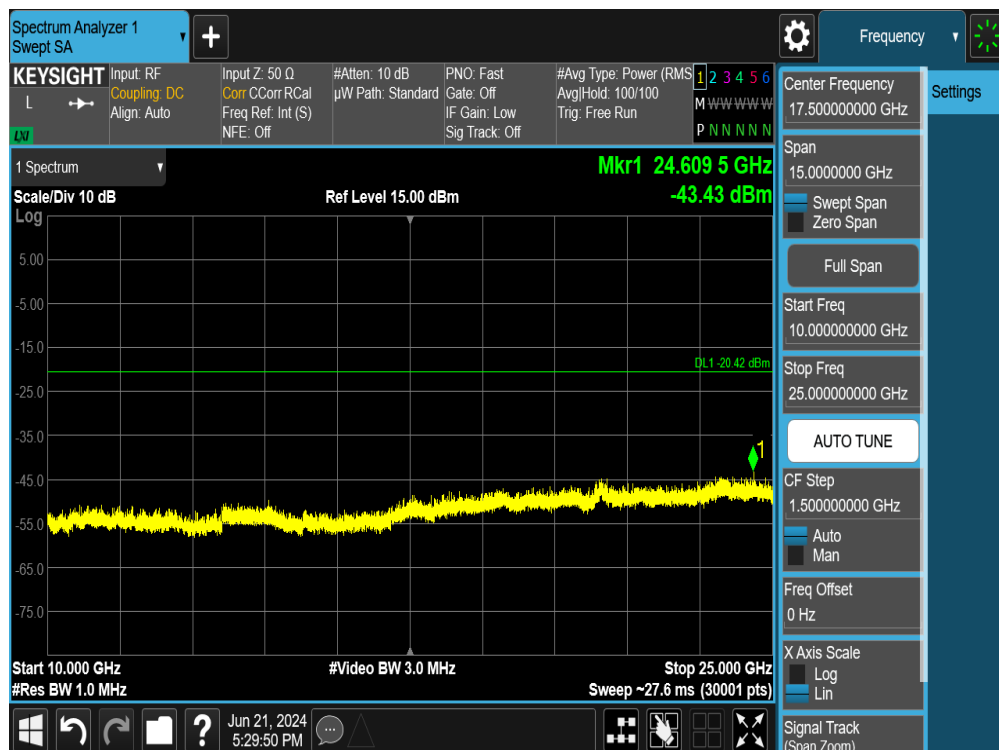
Plot 7-119. Conducted Spurious Plot MIMO ANT2 (802.11ax OFDMA – 26 Tones – Ch. 1)
