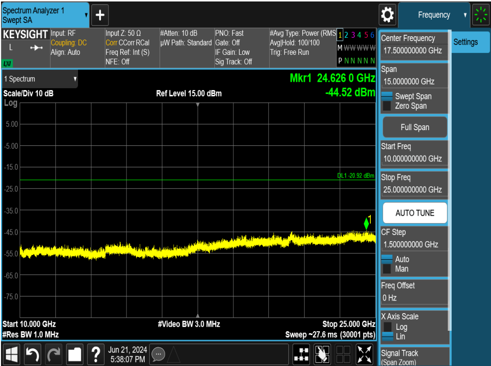
Plot 7-121. Conducted Spurious Plot MIMO ANT2 (802.11ax OFDMA – 26 Tones – Ch. 6)
