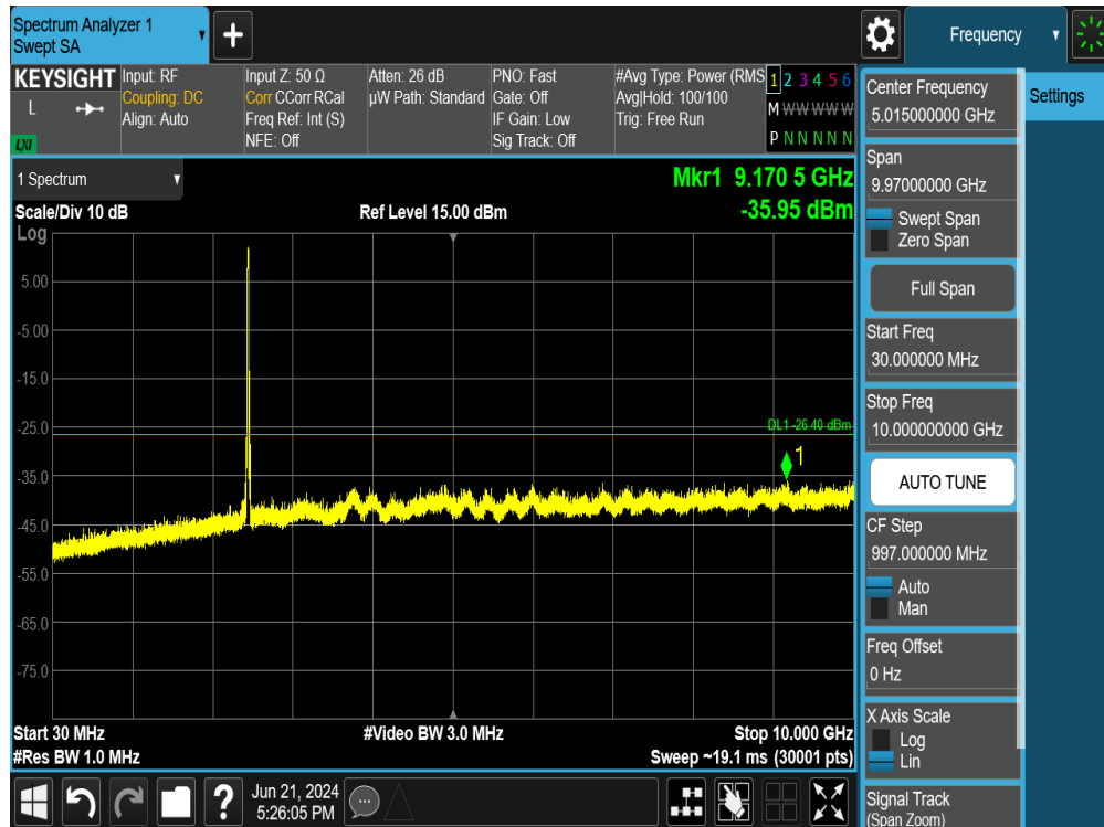
Plot 7-104. Conducted Spurious Plot SISO ANT2 (802.11ax OFDMA – 242 Tones – Ch. 11)
