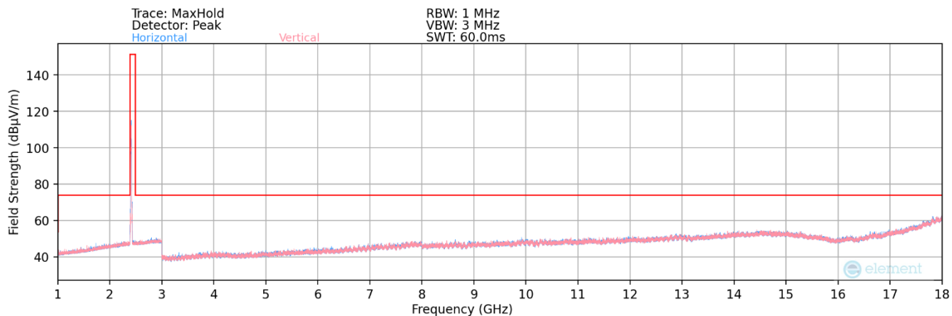
Plot 7-130. Radiated Spurious Plot above 1GHz – SISO ANT1 (802.11ax OFDMA – 26 Tones – Ch. 1)
