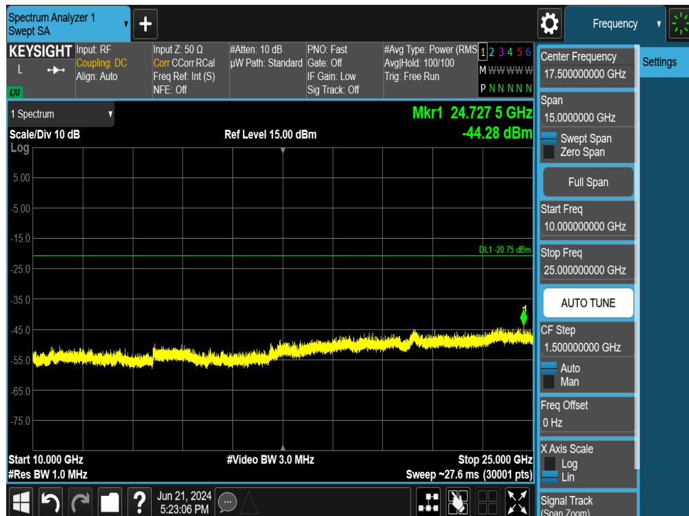
Plot 7-97. Conducted Spurious Plot SISO ANT2 (802.11ax OFDMA – 26 Tones – Ch. 6)
