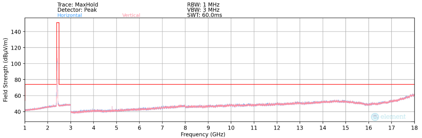
Plot 7-136. Radiated Spurious Plot above 1GHz – SISO ANT2 (802.11ax OFDMA – 26 Tones – Ch. 1)
