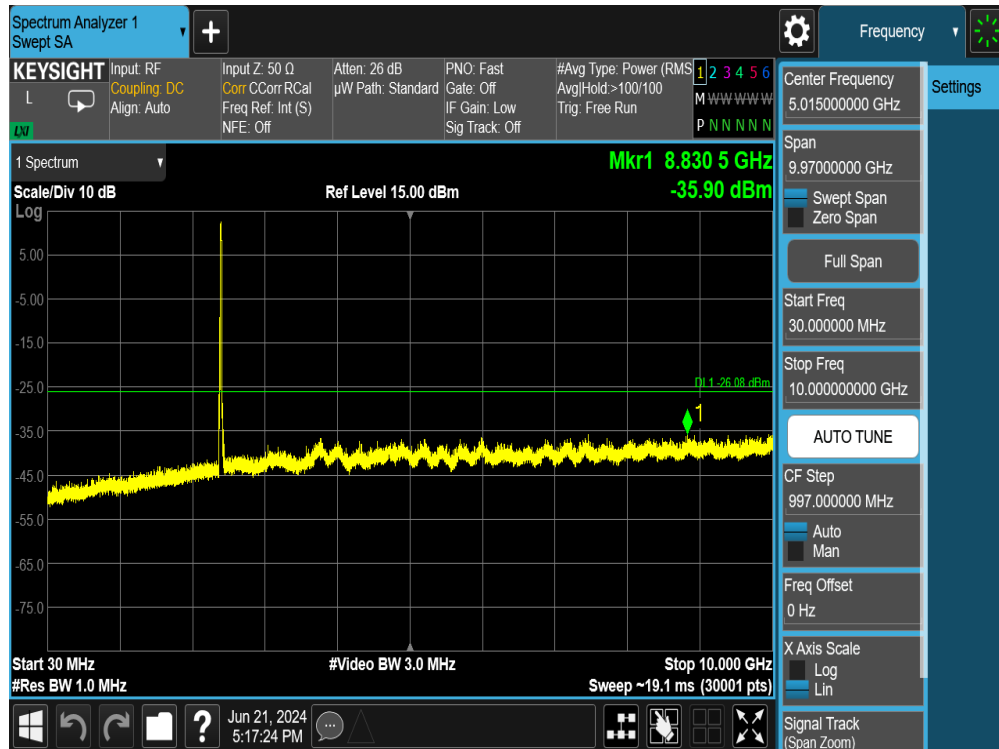
Plot 7-100. Conducted Spurious Plot SISO ANT2 (802.11ax OFDMA – 242 Tones – Ch. 1)
