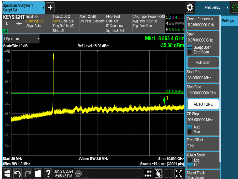
Plot 7-116. Conducted Spurious Plot MIMO ANT1 (802.11ax OFDMA – 242 Tones – Ch. 11)
