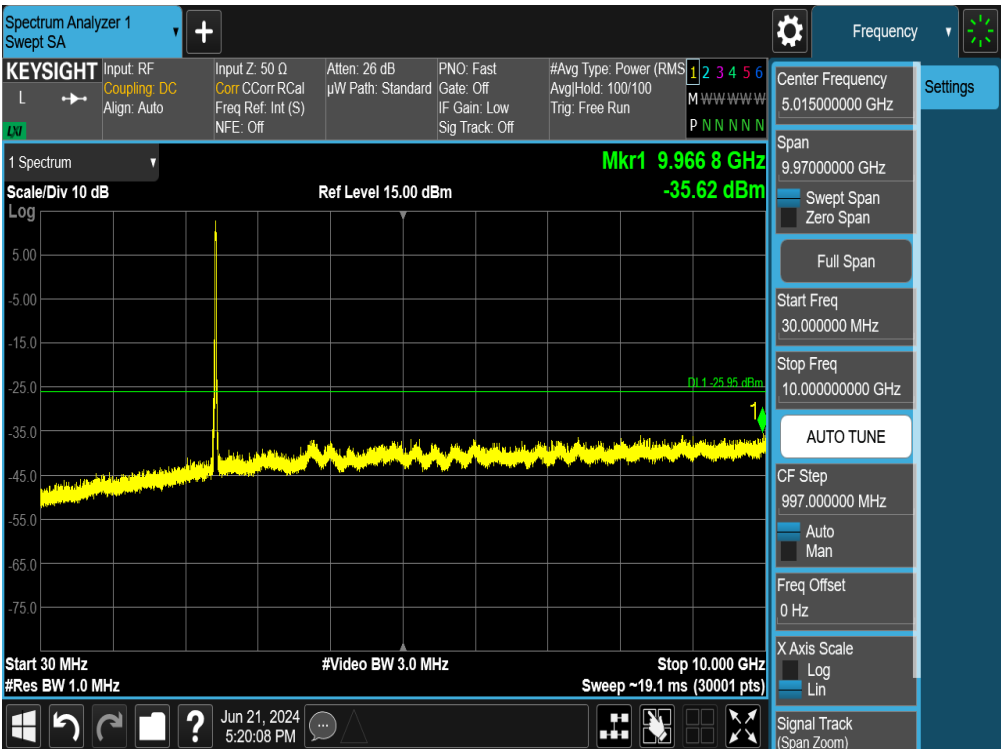
Plot 7-102. Conducted Spurious Plot SISO ANT2 (802.11ax OFDMA – 242 Tones – Ch. 6)
