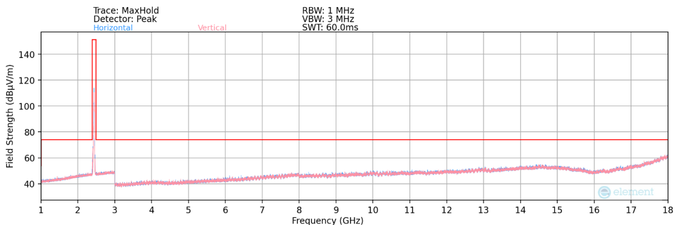
Plot 7-131. Radiated Spurious Plot above 1GHz – SISO ANT1 (802.11ax OFDMA – 26 Tones – Ch. 6)
