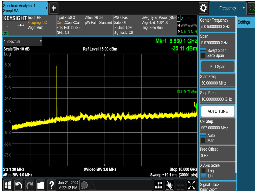
Plot 7-96. Conducted Spurious Plot SISO ANT2 (802.11ax OFDMA – 26 Tones – Ch. 6)
