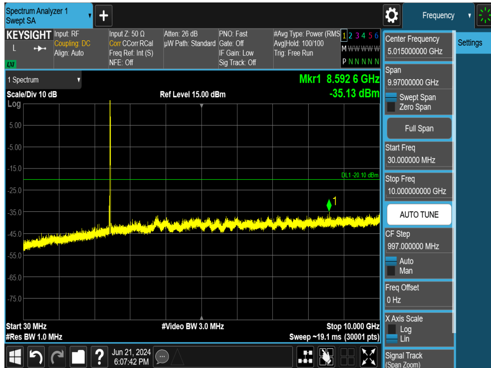
Plot 7-110. Conducted Spurious Plot MIMO ANT1 (802.11ax OFDMA – 26 Tones – Ch. 11)
