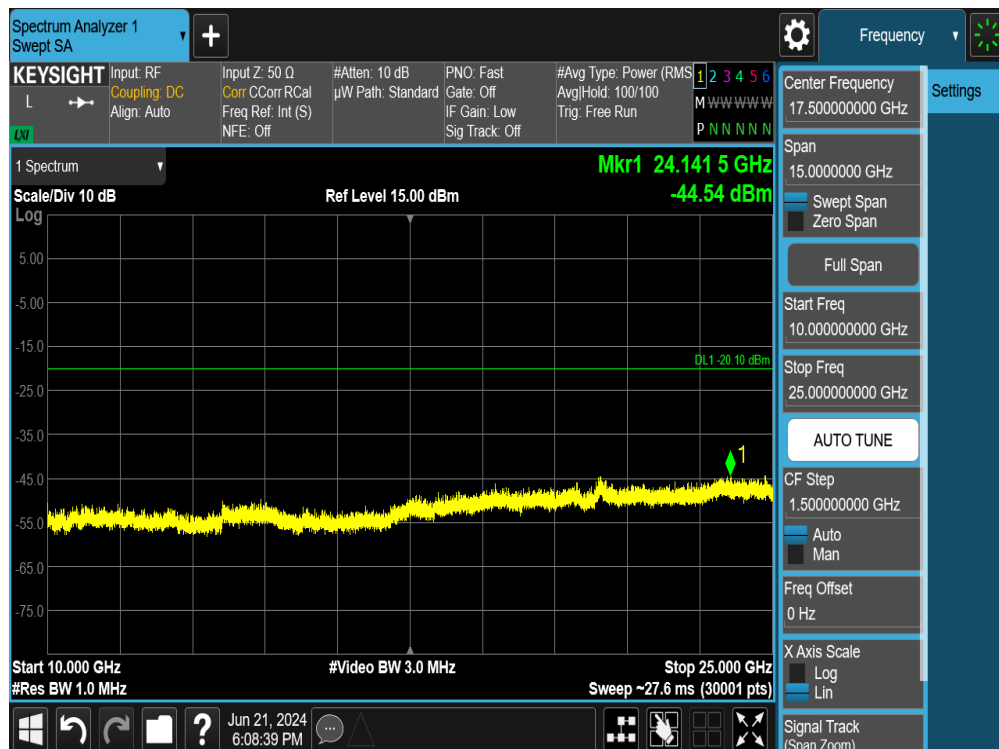
Plot 7-111. Conducted Spurious Plot MIMO ANT1 (802.11ax OFDMA – 26 Tones – Ch. 11)
