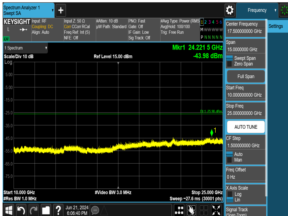
Plot 7-117. Conducted Spurious Plot MIMO ANT1 (802.11ax OFDMA – 242 Tones – Ch. 11)
