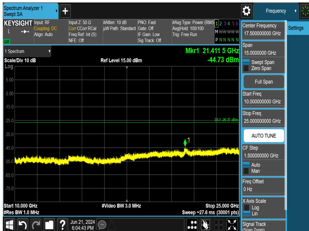
Plot 7-129. Conducted Spurious Plot MIMO ANT2 (802.11ax OFDMA – 242 Tones – Ch. 11)
