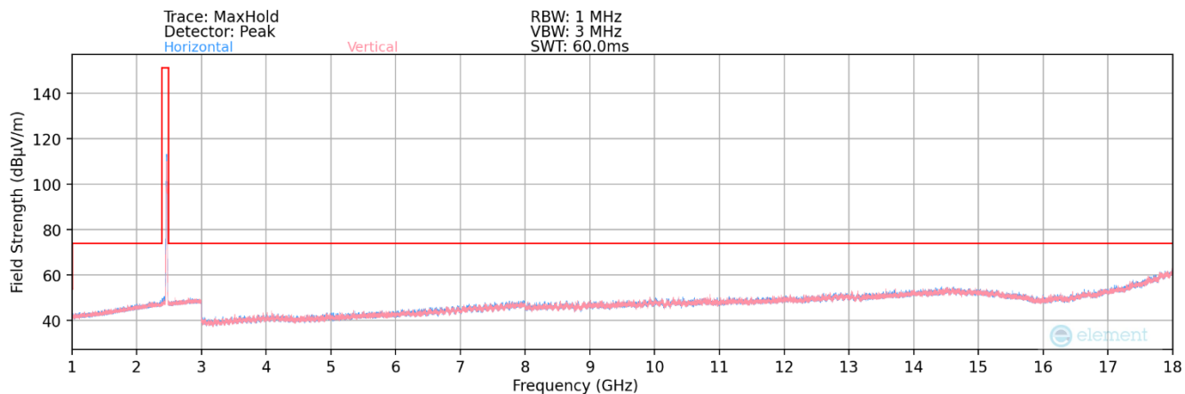
Plot 7-132. Radiated Spurious Plot above 1GHz– SISO ANT1 (802.11ax OFDMA – 26 Tones – Ch. 11)
