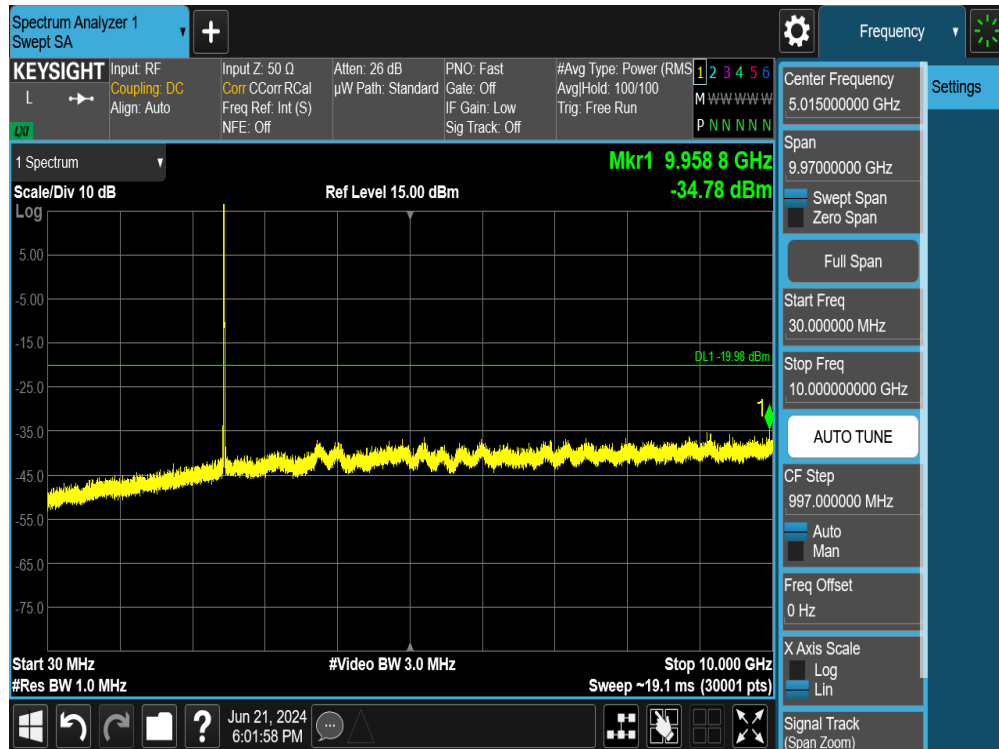
Plot 7-122. Conducted Spurious Plot MIMO ANT2 (802.11ax OFDMA – 26 Tones – Ch. 11)
