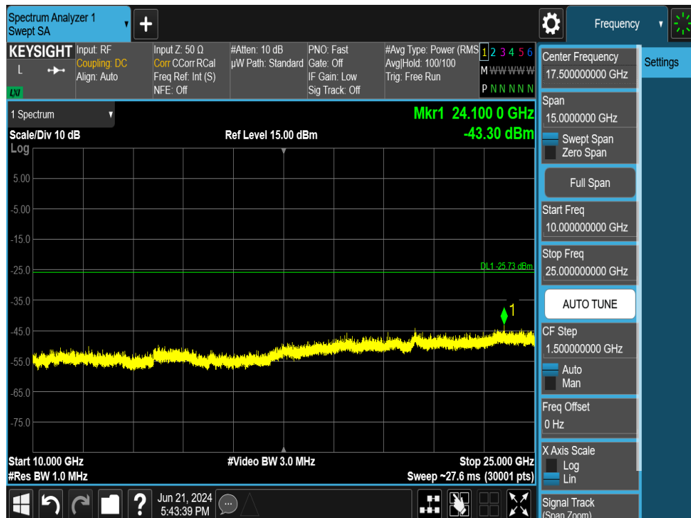
Plot 7-127. Conducted Spurious Plot MIMO ANT2 (802.11ax OFDMA – 242 Tones – Ch. 6)
