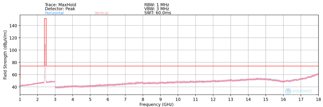
Plot 7-134. Radiated Spurious Plot above 1GHz – SISO ANT1 (802.11ax OFDMA – 242 Tones – Ch. 6)
