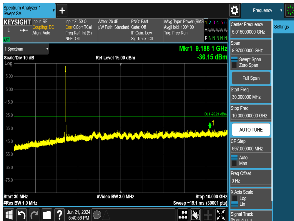
Plot 7-114. Conducted Spurious Plot MIMO ANT1 (802.11ax OFDMA – 242 Tones – Ch. 6)
