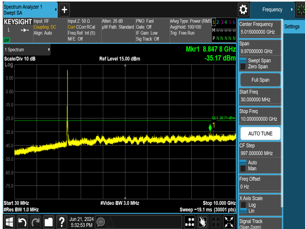
Plot 7-112. Conducted Spurious Plot MIMO ANT1 (802.11ax OFDMA – 242 Tones – Ch. 1)
