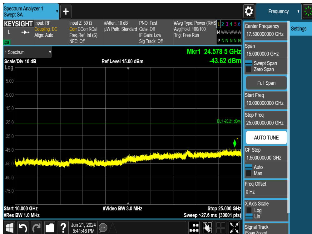
Plot 7-115. Conducted Spurious Plot MIMO ANT1 (802.11ax OFDMA – 242 Tones – Ch. 6)
