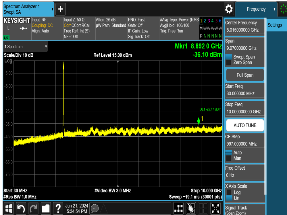
Plot 7-124. Conducted Spurious Plot MIMO ANT2 (802.11ax OFDMA – 242 Tones – Ch. 1)
