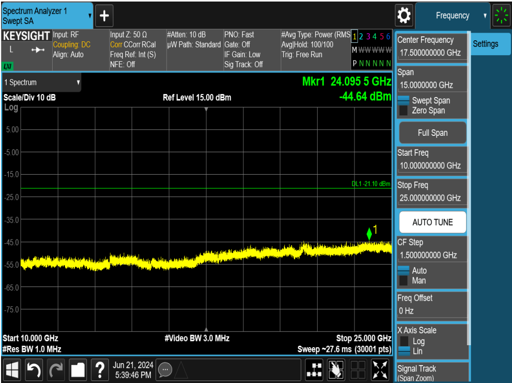
Plot 7-109. Conducted Spurious Plot MIMO ANT1 (802.11ax OFDMA – 26 Tones – Ch. 6)
