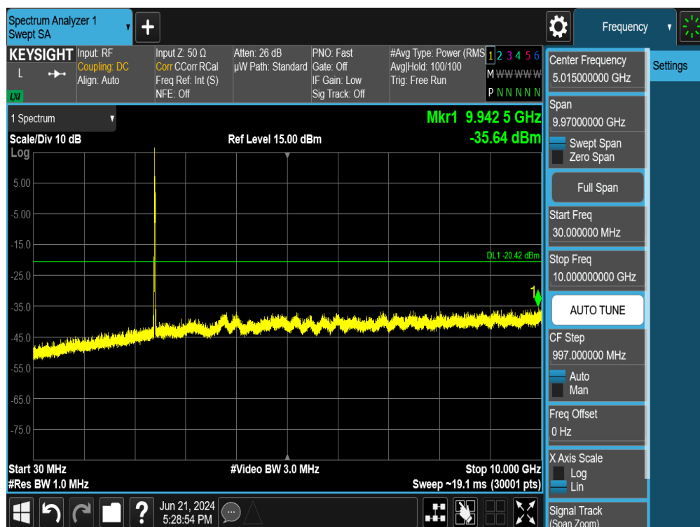
Plot 7-118. Conducted Spurious Plot MIMO ANT2 (802.11ax OFDMA – 26 Tones – Ch. 1)
