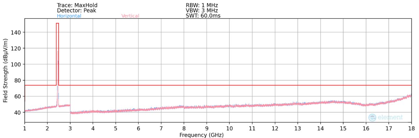
Plot 7-138. Radiated Spurious Plot above 1GHz– SISO ANT2 (802.11ax OFDMA – 26 Tones – Ch. 11)
