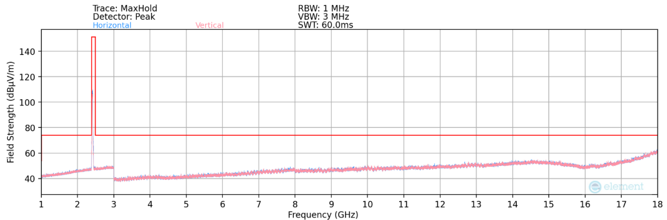
Plot 7-133. Radiated Spurious Plot above 1GHz – SISO ANT1 (802.11ax OFDMA – 242 Tones – Ch. 1)
