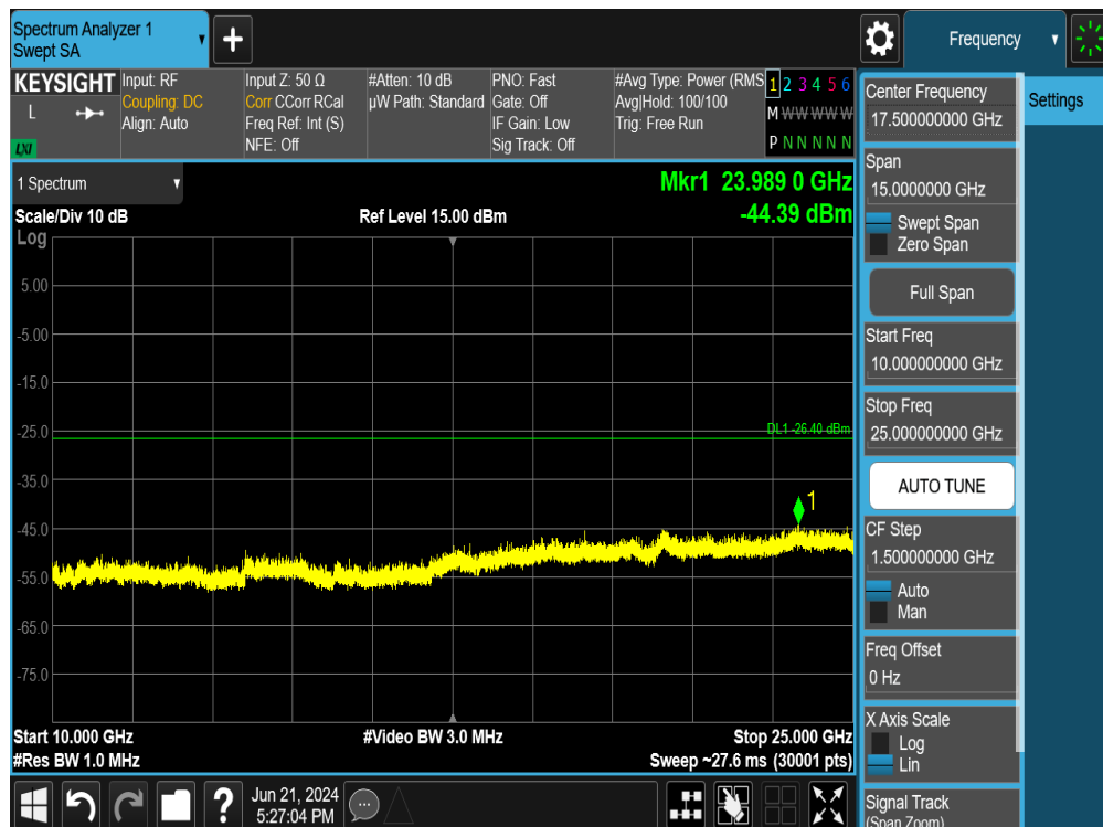
Plot 7-105. Conducted Spurious Plot SISO ANT2 (802.11ax OFDMA – 242 Tones – Ch. 11)
