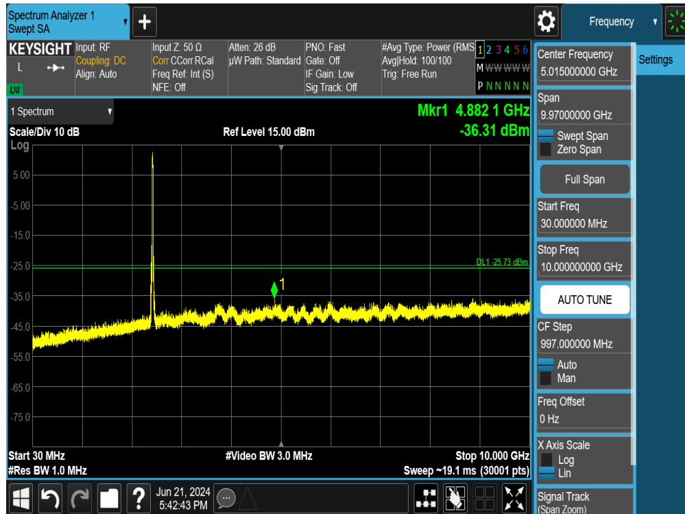
Plot 7-126. Conducted Spurious Plot MIMO ANT2 (802.11ax OFDMA – 242 Tones – Ch. 6)
