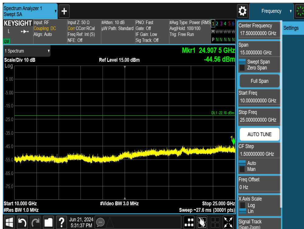
Plot 7-107. Conducted Spurious Plot MIMO ANT1 (802.11ax OFDMA – 26 Tones – Ch. 1)
