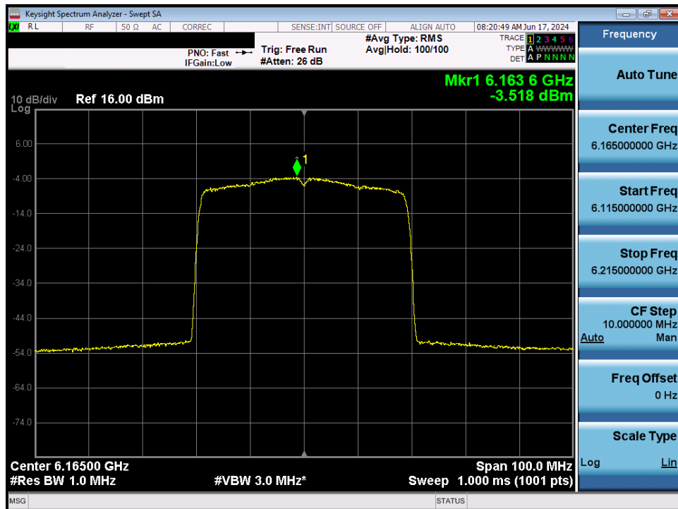
Plot 7-70. Power Spectral Density MIMO ANT2 (40MHz 802.11ax (UNII Band 5) – Ch. 43) - LPI/SP
