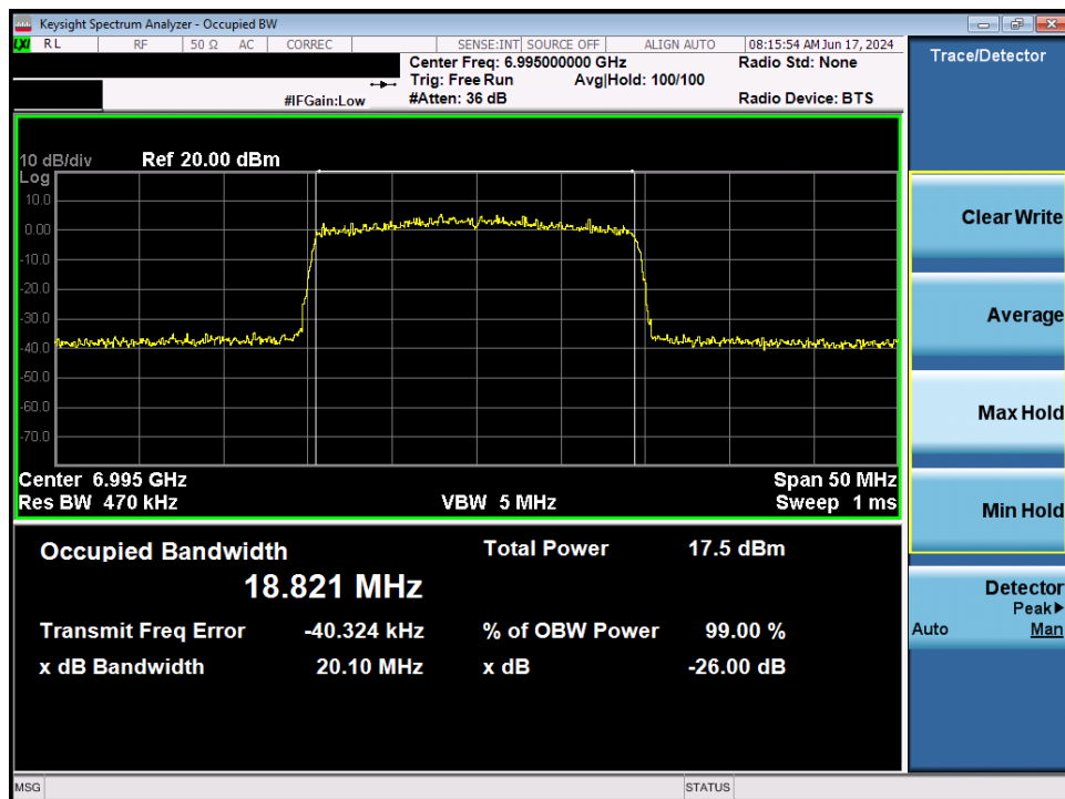
Plot 7-44. 26dB Bandwidth Plot MIMO ANT2 (20MHz 802.11ax (UNII Band 8) – Ch. 209)
