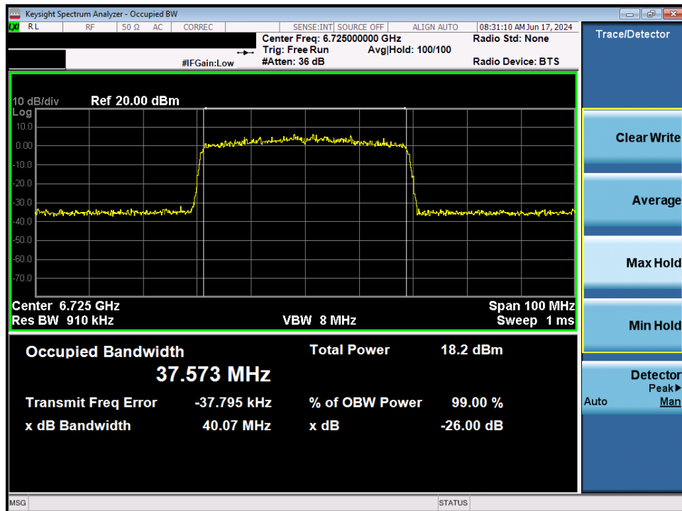
Plot 7-40. 26dB Bandwidth Plot MIMO ANT2 (40MHz 802.11ax (UNII Band 7) – Ch. 155)
