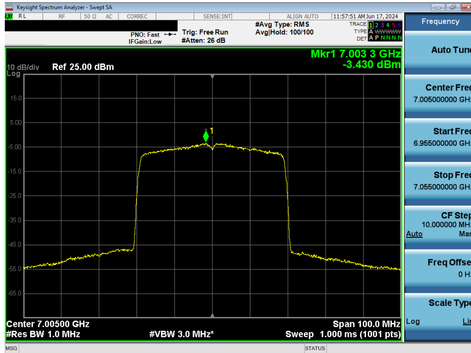
Plot 7-65. Power Spectral Density MIMO ANT1 (40MHz 802.11ax (UNII Band 8) – Ch. 211) - LPI
