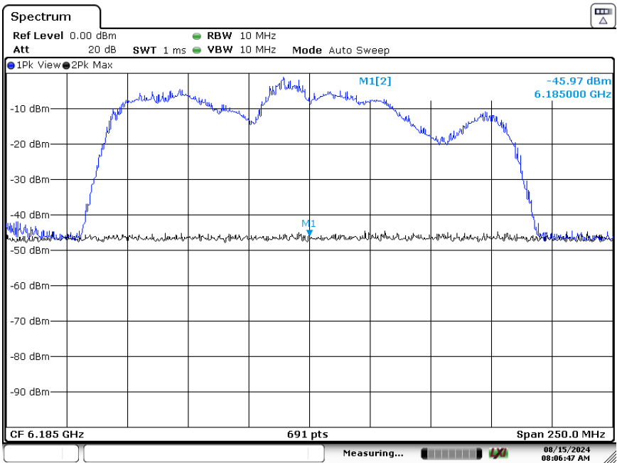
Plot 7-5. CBP 160MHz Channel - Injection Center – [6185 MHz]
