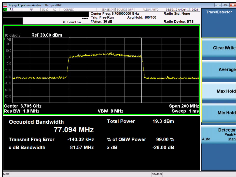
Plot 7-41. 26dB Bandwidth Plot MIMO ANT2 (80MHz 802.11ax (UNII Band 7) – Ch. 151)
