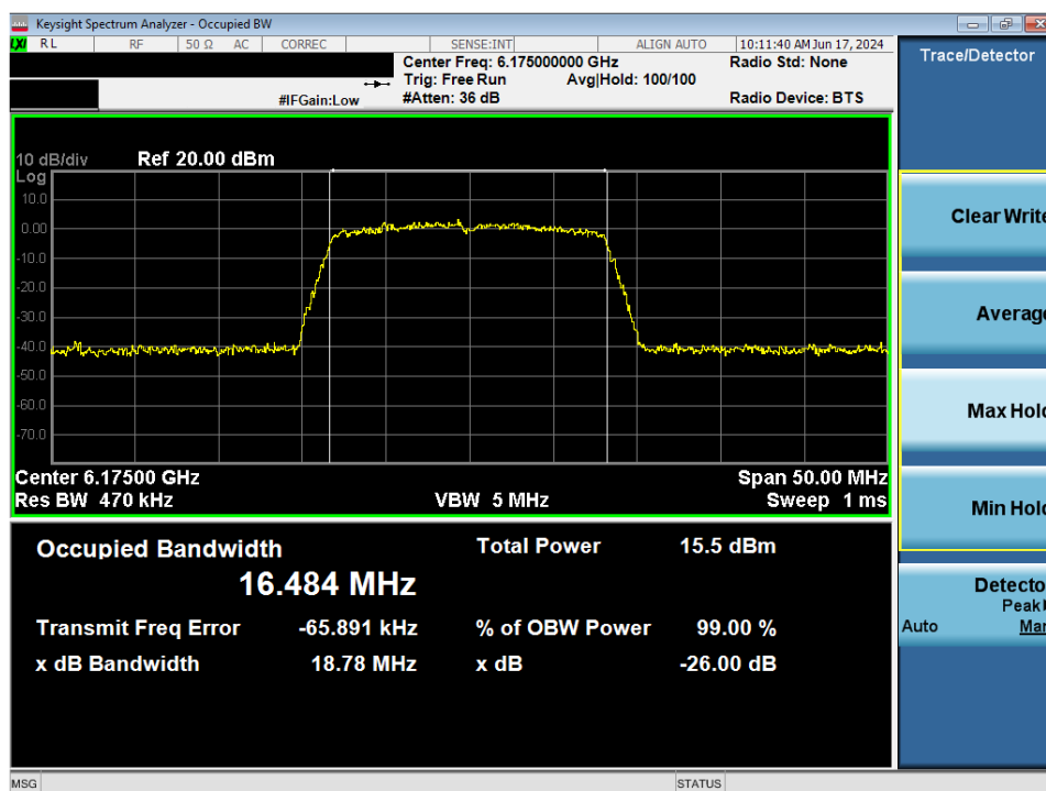
Plot 7-8. 26dB Bandwidth Plot MIMO ANT1 (20MHz 802.11a (UNII Band 5) – Ch. 45)
