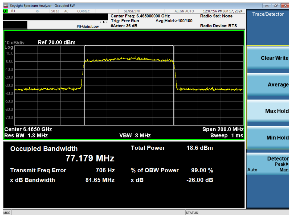
Plot 7-16. 26dB Bandwidth Plot MIMO ANT1 (80MHz 802.11ax (UNII Band 6) – Ch. 103)
