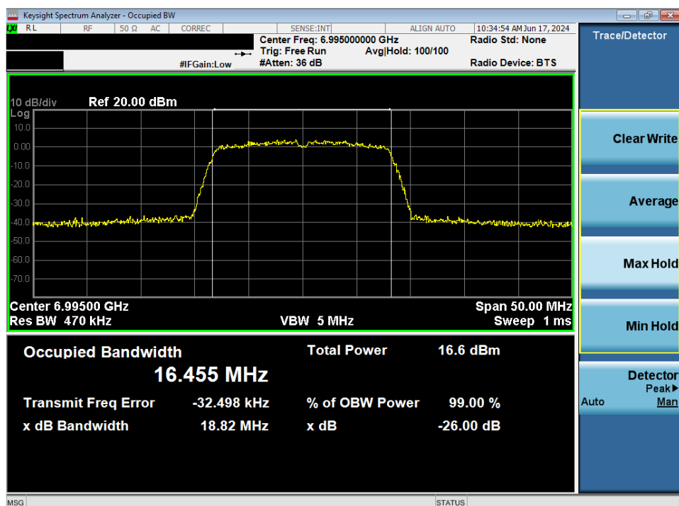
Plot 7-23. 26dB Bandwidth Plot MIMO ANT1 (20MHz 802.11a (UNII Band 8) – Ch. 209)
