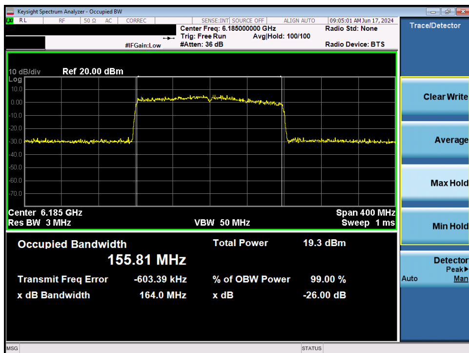
Plot 7-32. 26dB Bandwidth Plot MIMO ANT2 (160MHz 802.11ax (UNII Band 5) – Ch. 47)
