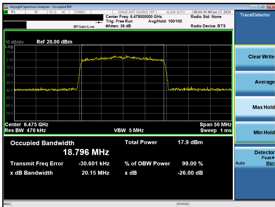
Plot 7-34. 26dB Bandwidth Plot MIMO ANT2 (20MHz 802.11ax (UNII Band 6) – Ch. 105)
