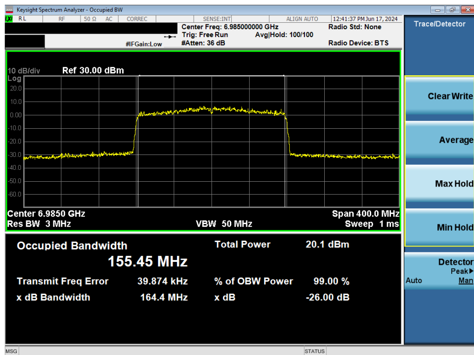
Plot 7-27. 26dB Bandwidth Plot MIMO ANT1 (160MHz 802.11ax (UNII Band 8) – Ch. 207)
