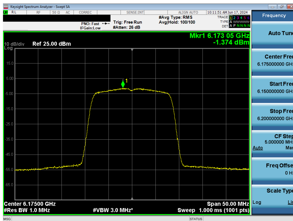
Plot 7-48. Power Spectral Density MIMO ANT1 (20MHz 802.11a (UNII Band 5) – Ch. 45) - LPI/SP
