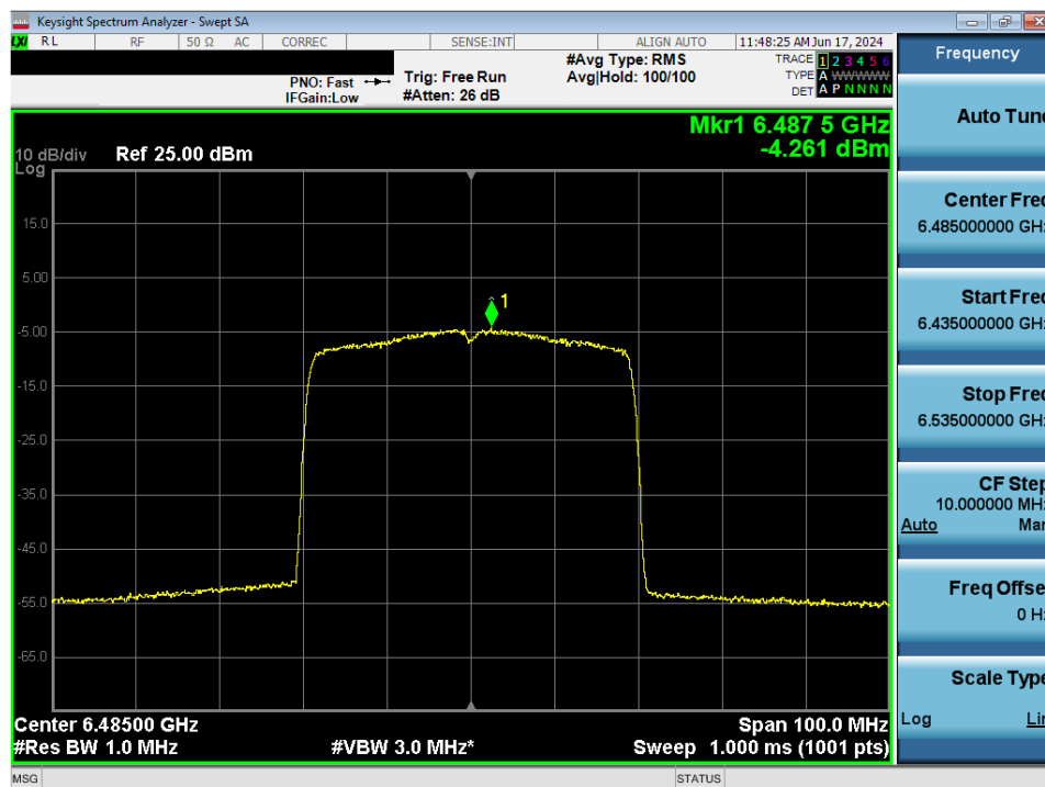
Plot 7-55. Power Spectral Density MIMO ANT1 (40MHz 802.11ax (UNII Band 6) – Ch. 107) - LPI
