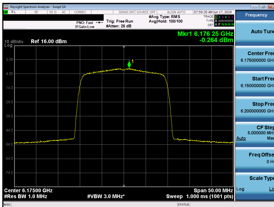
Plot 7-69. Power Spectral Density MIMO ANT2 (20MHz 802.11ax (UNII Band 5) – Ch. 45) - LPI/SP
