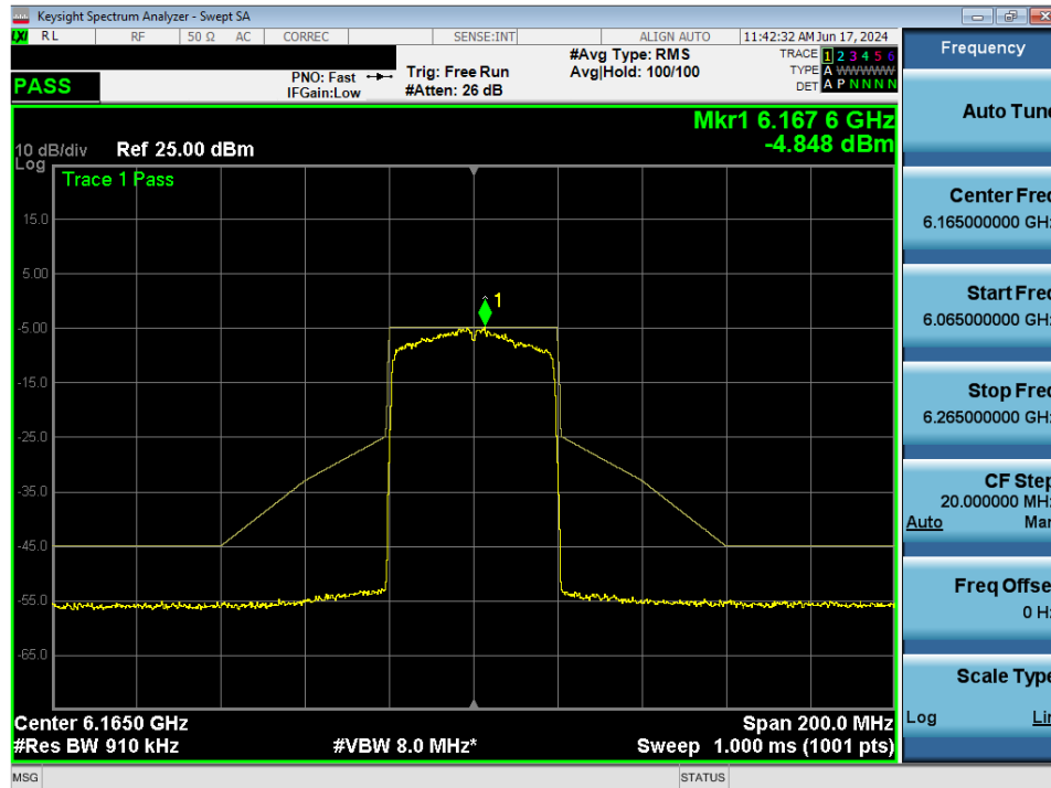
Plot 7-90. In-Band Emission MIMO ANT1 (40MHz 802.11ax (UNII Band 5) – Ch. 43)
