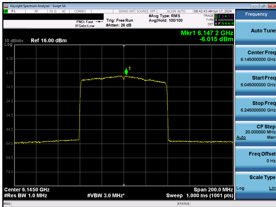
Plot 7-71. Power Spectral Density MIMO ANT2 (80MHz 802.11ax (UNII Band 5) – Ch. 39) - LPI/SP
