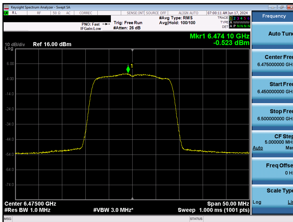
Plot 7-73. Power Spectral Density MIMO ANT2 (20MHz 802.11a (UNII Band 6) – Ch. 105) - LPI
