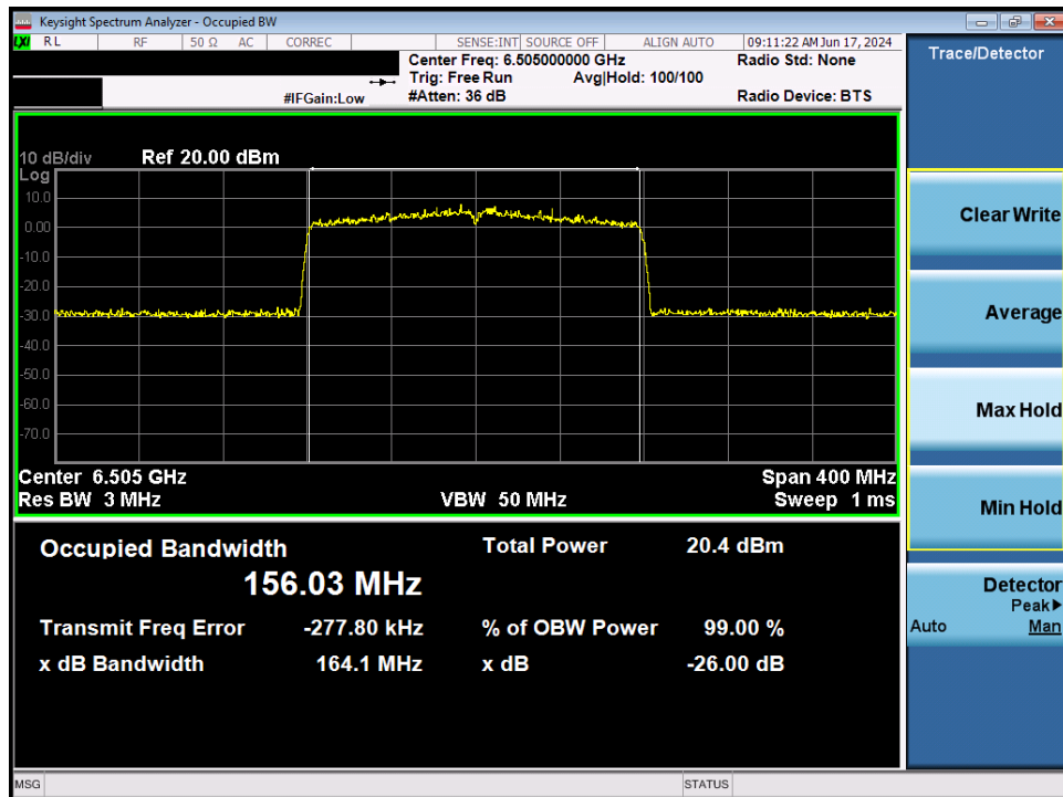
Plot 7-37. 26dB Bandwidth Plot MIMO ANT2 (160MHz 802.11ax (UNII Band 6) – Ch. 111)
