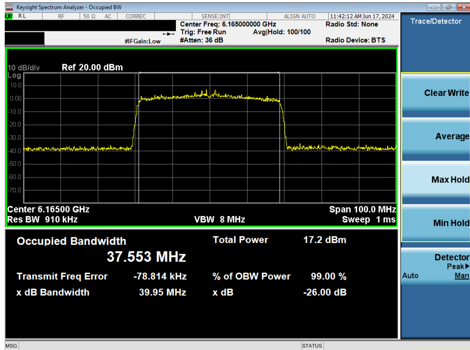
Plot 7-10. 26dB Bandwidth Plot MIMO ANT1 (40MHz 802.11ax (UNII Band 5) – Ch. 43)
