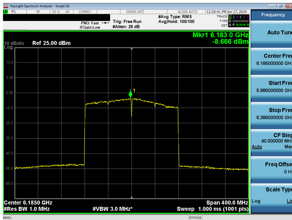
Plot 7-52. Power Spectral Density MIMO ANT1 (160MHz 802.11ax (UNII Band 5) – Ch. 47) - LPI/SP
