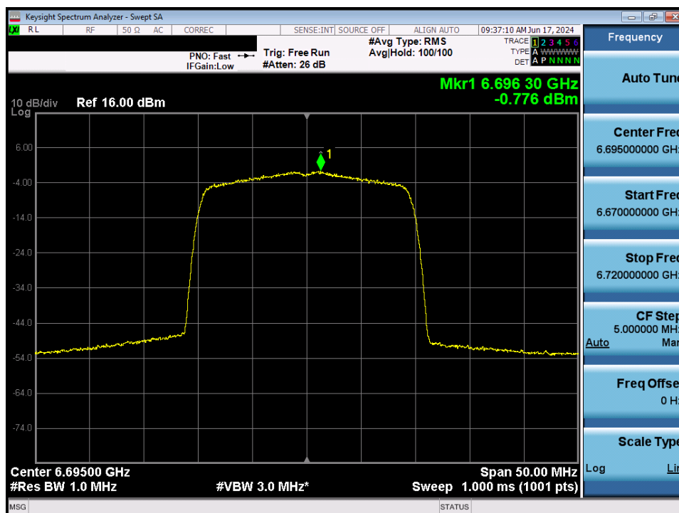
Plot 7-79. Power Spectral Density MIMO ANT2 (20MHz 802.11ax (UNII Band 7) – Ch. 149) - LPI/SP
