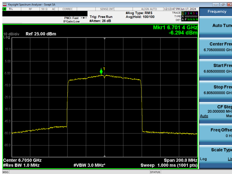
Plot 7-61. Power Spectral Density MIMO ANT1 (80MHz 802.11ax (UNII Band 7) – Ch. 151) - LPI/SP
