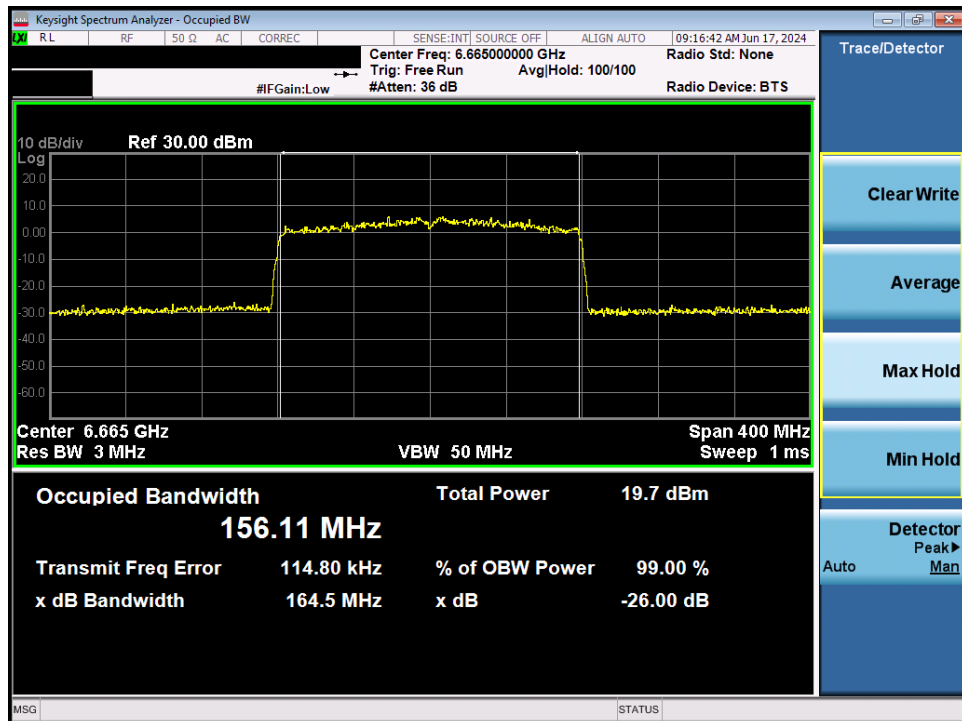
Plot 7-42. 26dB Bandwidth Plot MIMO ANT2 (160MHz 802.11ax (UNII Band 7) – Ch. 143)
