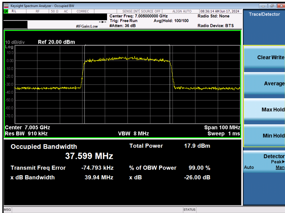
Plot 7-45. 26dB Bandwidth Plot MIMO ANT2 (40MHz 802.11ax (UNII Band 8) – Ch. 211)
