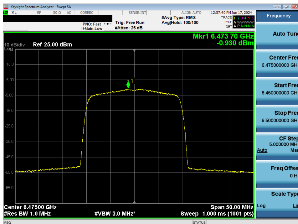
Plot 7-54. Power Spectral Density MIMO ANT1 (20MHz 802.11ax (UNII Band 6) – Ch. 105) - LPI
