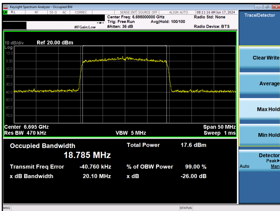
Plot 7-39. 26dB Bandwidth Plot MIMO ANT2 (20MHz 802.11ax (UNII Band 7) – Ch. 149)
