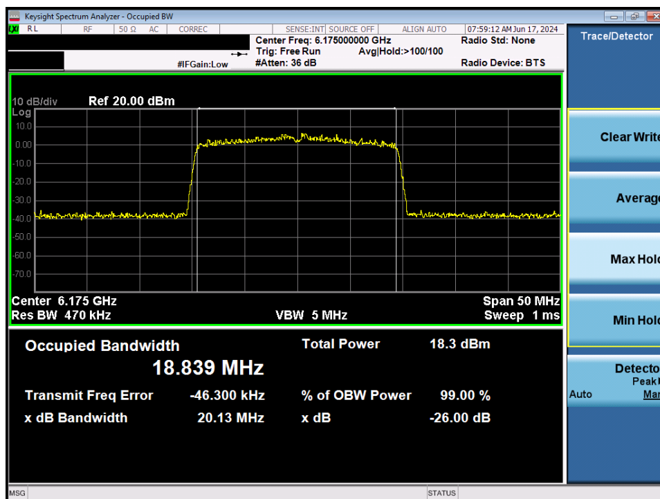
Plot 7-29. 26dB Bandwidth Plot MIMO ANT2 (20MHz 802.11ax (UNII Band 5) – Ch. 45)
