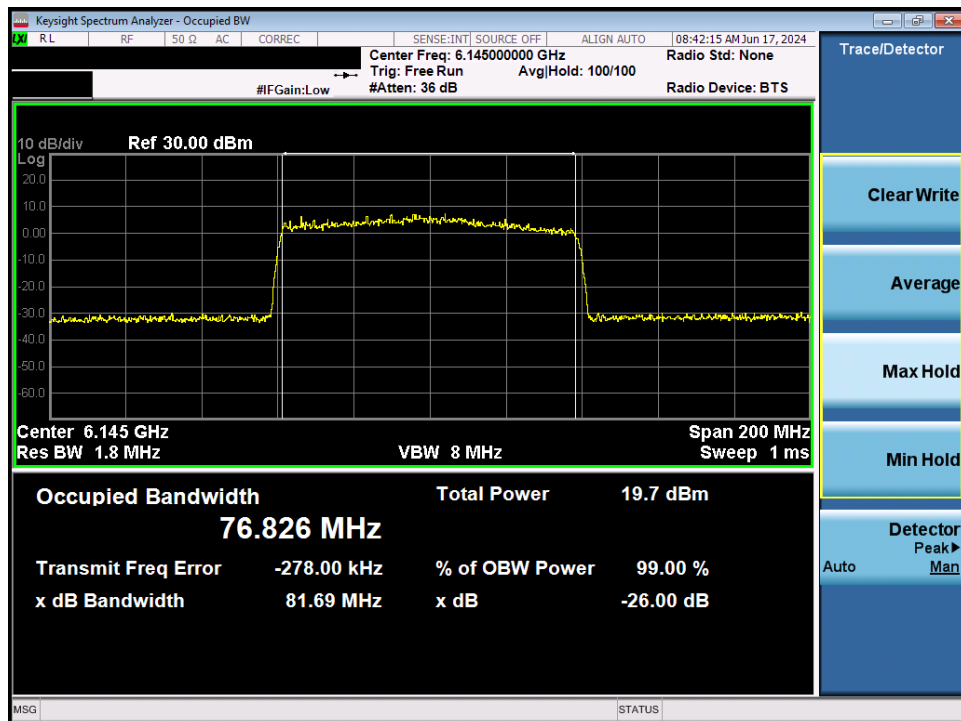
Plot 7-31. 26dB Bandwidth Plot MIMO ANT2 (80MHz 802.11ax (UNII Band 5) – Ch. 39)
