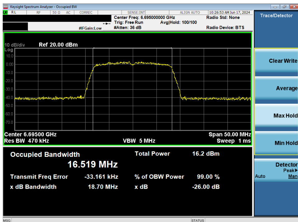
Plot 7-18. 26dB Bandwidth Plot MIMO ANT1 (20MHz 802.11a (UNII Band 7) – Ch. 149)
