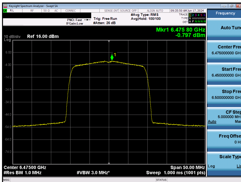
Plot 7-74. Power Spectral Density MIMO ANT2 (20MHz 802.11ax (UNII Band 6) – Ch. 105) - LPI
