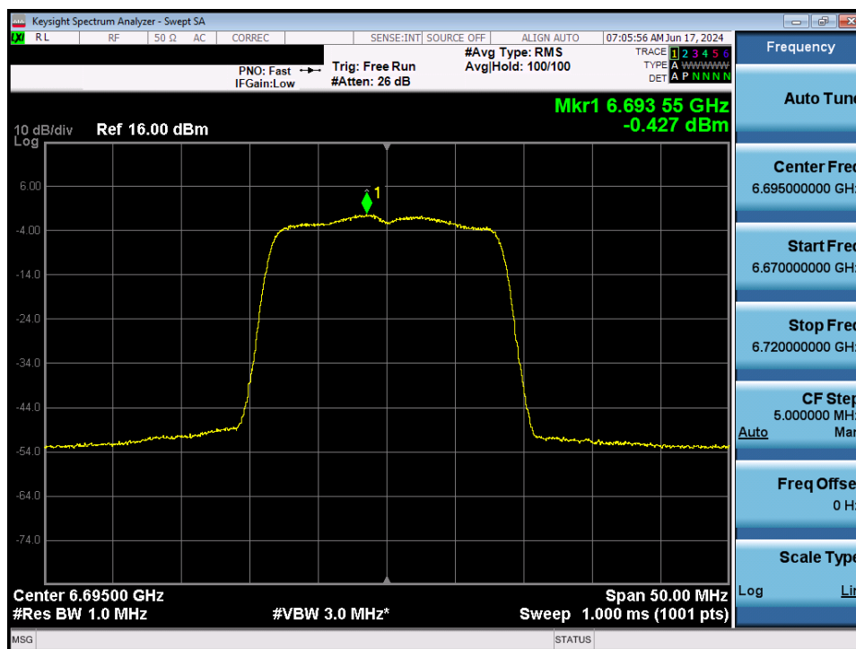
Plot 7-78. Power Spectral Density MIMO ANT2 (20MHz 802.11a (UNII Band 7) – Ch. 149) - LPI/SP
