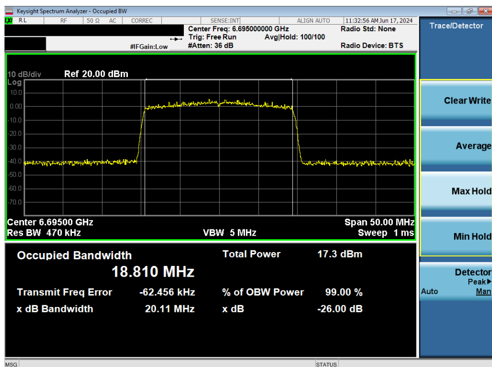
Plot 7-19. 26dB Bandwidth Plot MIMO ANT1 (20MHz 802.11ax (UNII Band 7) – Ch. 149)
