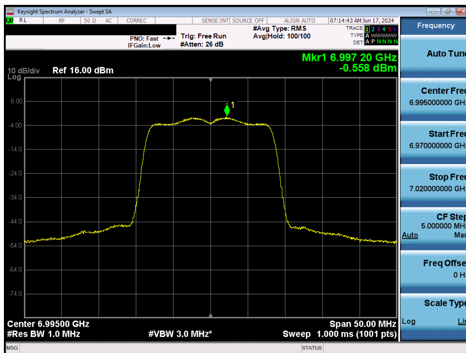
Plot 7-83. Power Spectral Density MIMO ANT2 (20MHz 802.11a (UNII Band 8) – Ch. 209) - LPI
