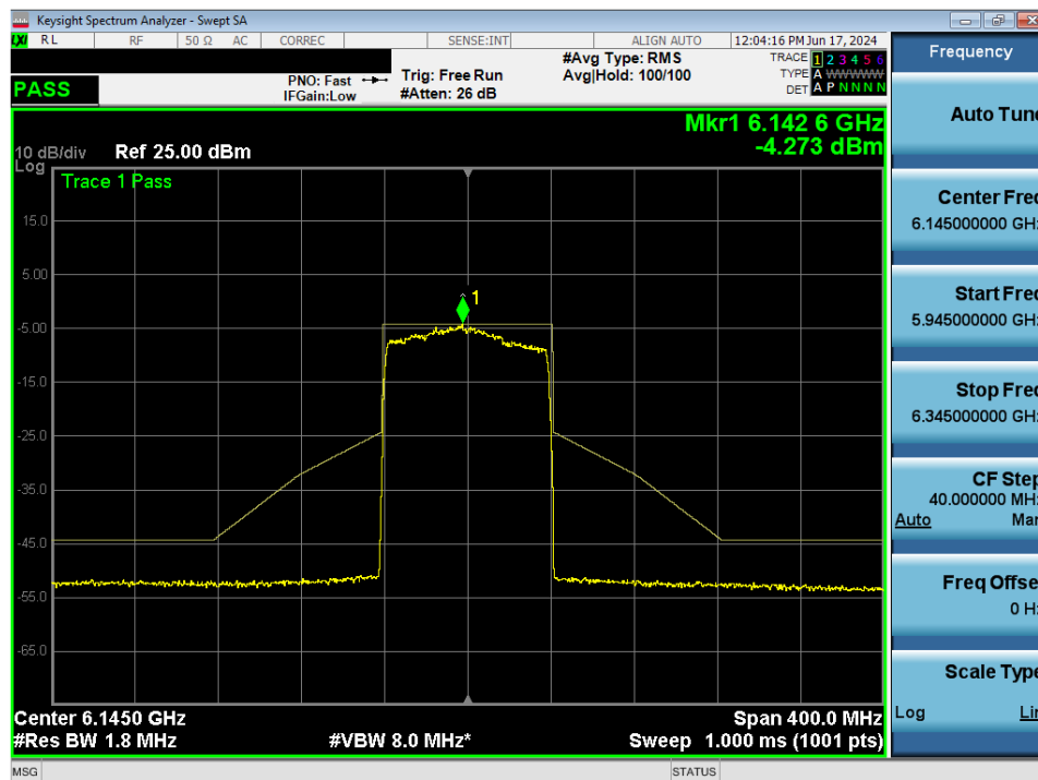
Plot 7-91. In-Band Emission MIMO ANT1 (80MHz 802.11ax (UNII Band 5) – Ch. 39)
