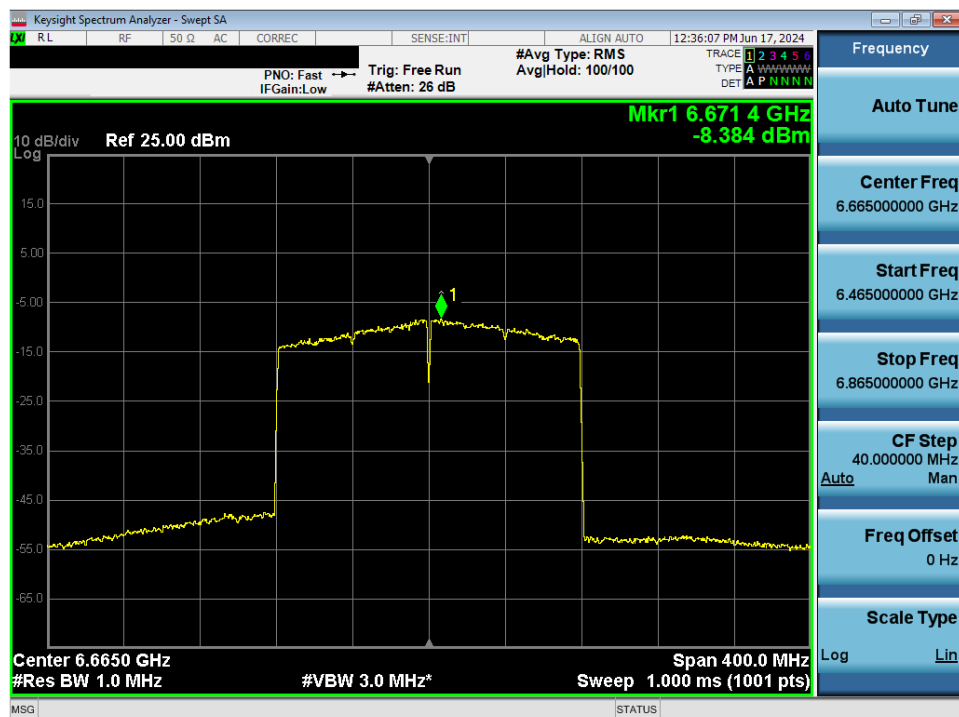
Plot 7-62. Power Spectral Density MIMO ANT1 (160MHz 802.11ax (UNII Band 7) – Ch. 143) - LPI/SP
