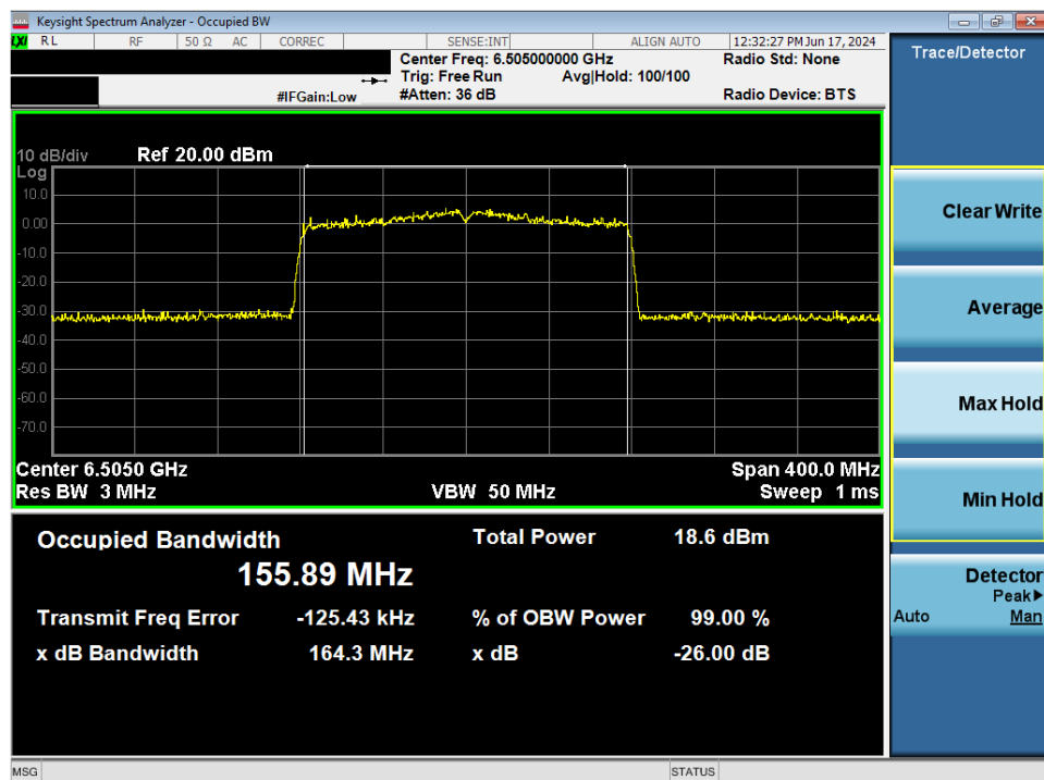
Plot 7-17. 26dB Bandwidth Plot MIMO ANT1 (160MHz 802.11ax (UNII Band 6) – Ch. 111)
