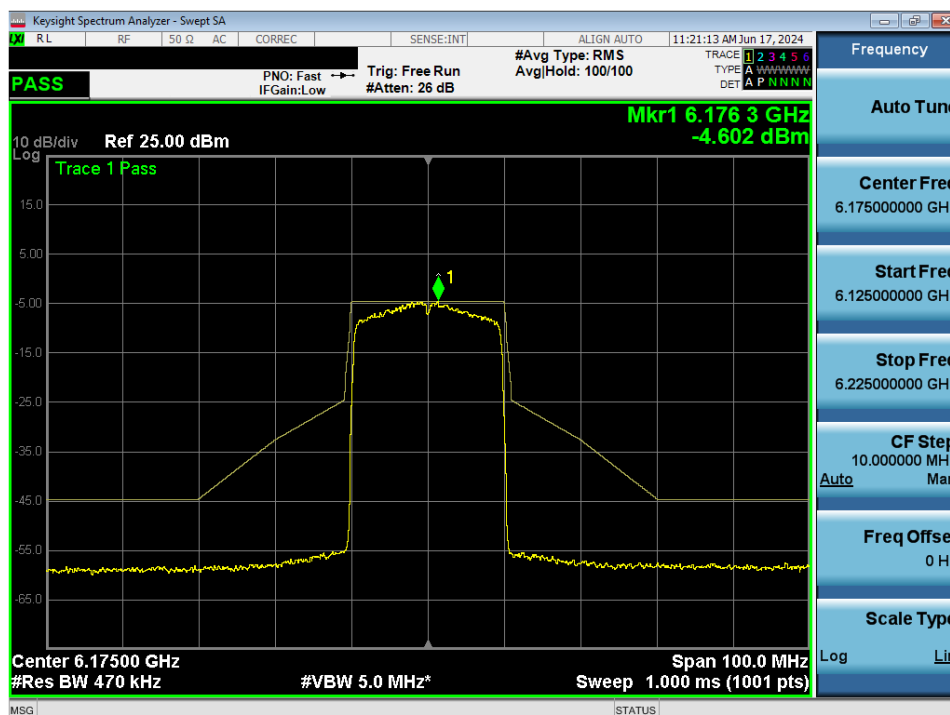
Plot 7-89. In-Band Emission MIMO ANT1 (20MHz 802.11ax (UNII Band 5) – Ch. 45)
