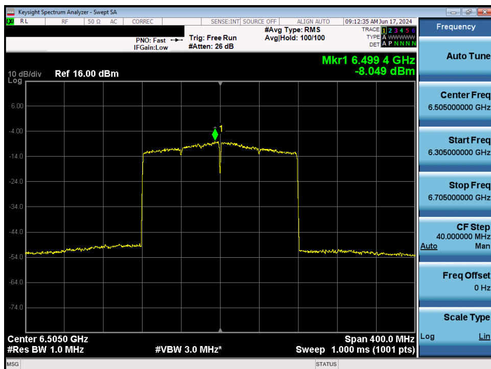
Plot 7-77. Power Spectral Density MIMO ANT2 (160MHz 802.11ax (UNII Band 6) – Ch. 111) - LPI
