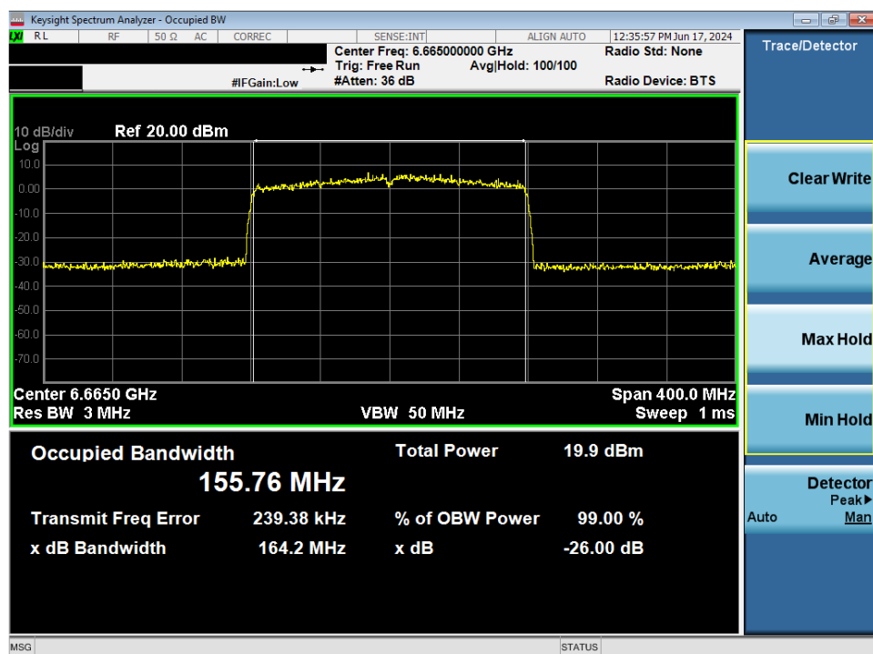
Plot 7-22. 26dB Bandwidth Plot MIMO ANT1 (160MHz 802.11ax (UNII Band 7) – Ch. 143)
