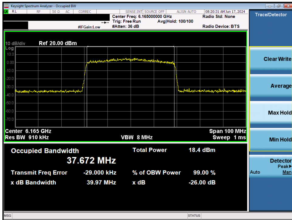
Plot 7-30. 26dB Bandwidth Plot MIMO ANT2 (40MHz 802.11ax (UNII Band 5) – Ch. 43)
