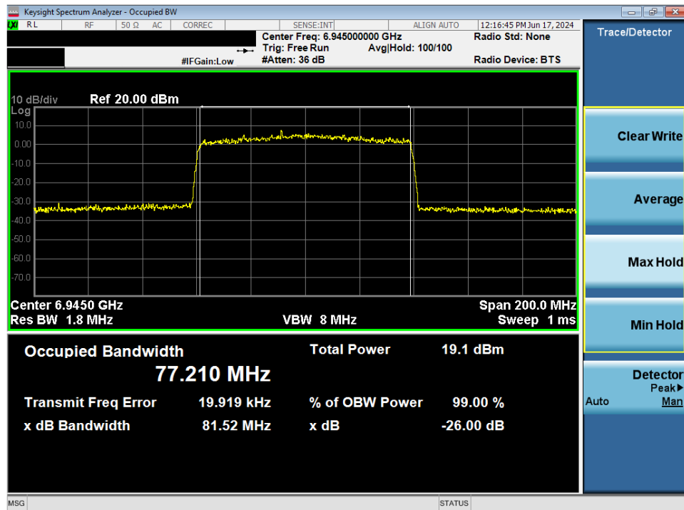
Plot 7-26. 26dB Bandwidth Plot MIMO ANT1 (80MHz 802.11ax (UNII Band 8) – Ch. 199)
