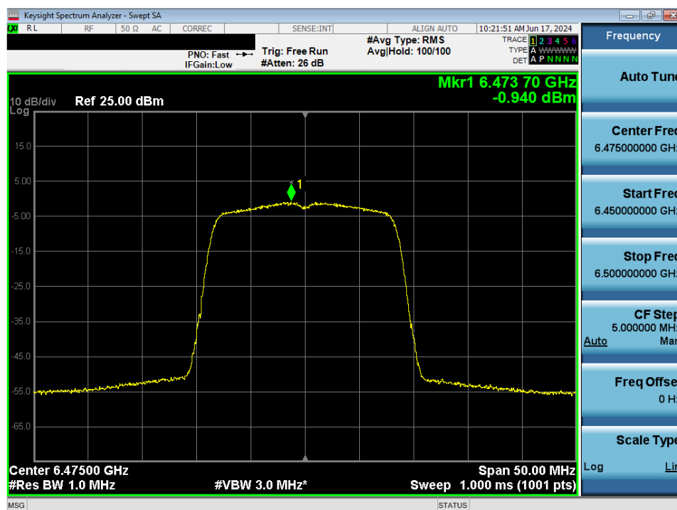
Plot 7-53. Power Spectral Density MIMO ANT1 (20MHz 802.11a (UNII Band 6) – Ch. 105) - LPI
