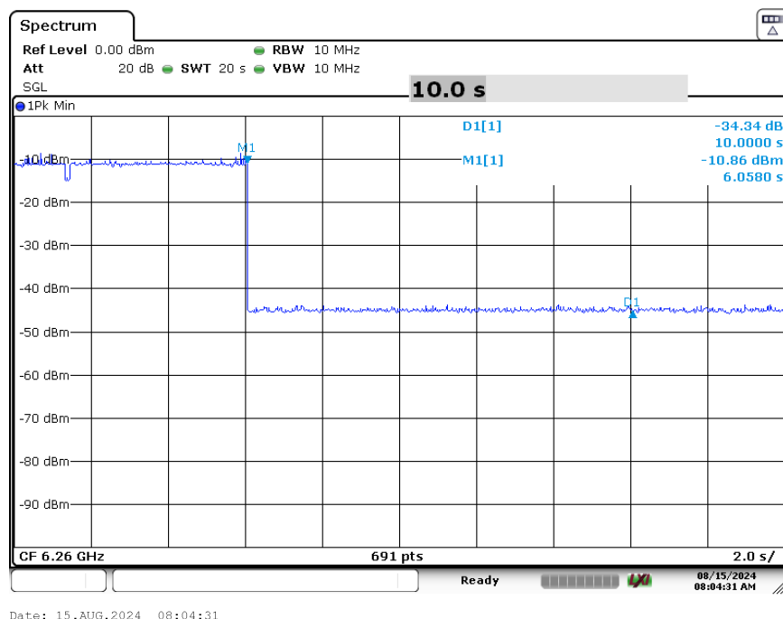
Plot 7-3. Contention Based Protocol Timing Plot (160MHz (UNII Band 5) – Ch. 47 High)
