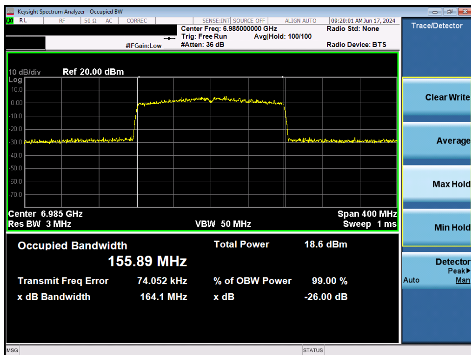
Plot 7-47. 26dB Bandwidth Plot MIMO ANT2 (160MHz 802.11ax (UNII Band 8) – Ch. 207)
