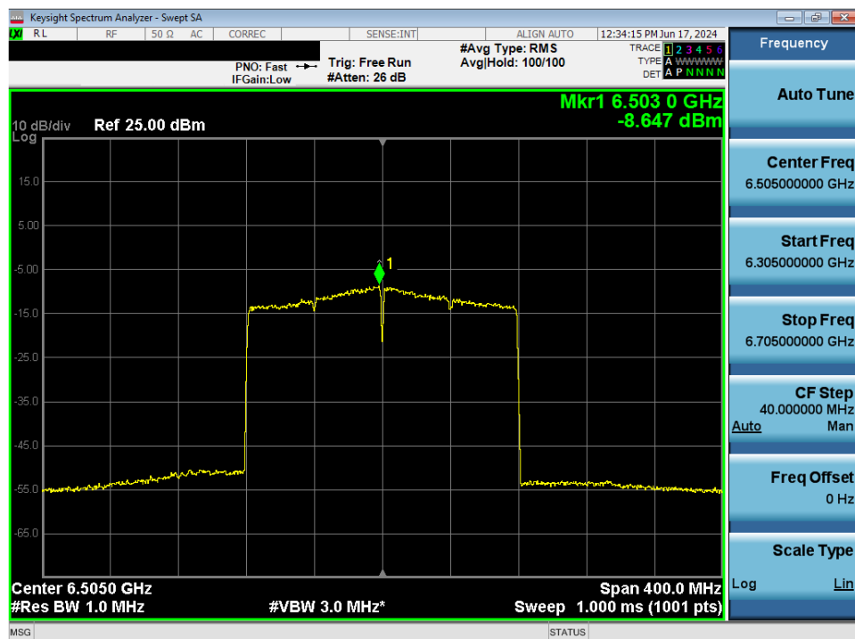
Plot 7-57. Power Spectral Density MIMO ANT1 (160MHz 802.11ax (UNII Band 6) – Ch. 111) - LPI
