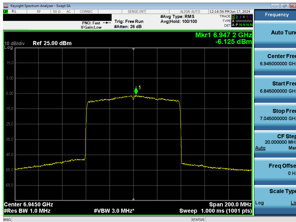
Plot 7-66. Power Spectral Density MIMO ANT1 (80MHz 802.11ax (UNII Band 8) – Ch. 199) - LPI
