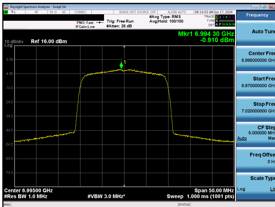
Plot 7-84. Power Spectral Density MIMO ANT2 (20MHz 802.11ax (UNII Band 8) – Ch. 209) - LPI
