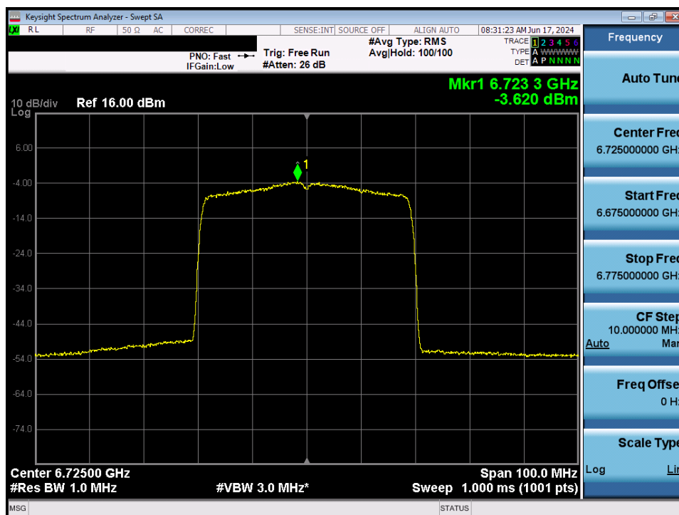
Plot 7-80. Power Spectral Density MIMO ANT2 (40MHz 802.11ax (UNII Band 7) – Ch. 155) - LPI/SP
