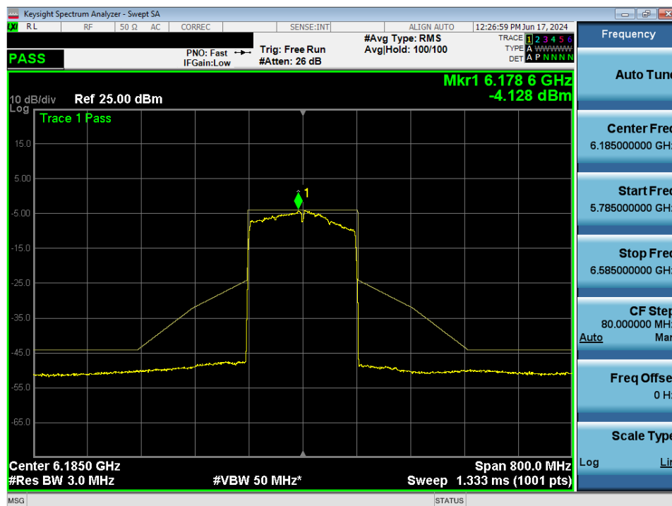
Plot 7-92. In-Band Emission MIMO ANT1 (160MHz 802.11ax (UNII Band 5) – Ch. 47)
