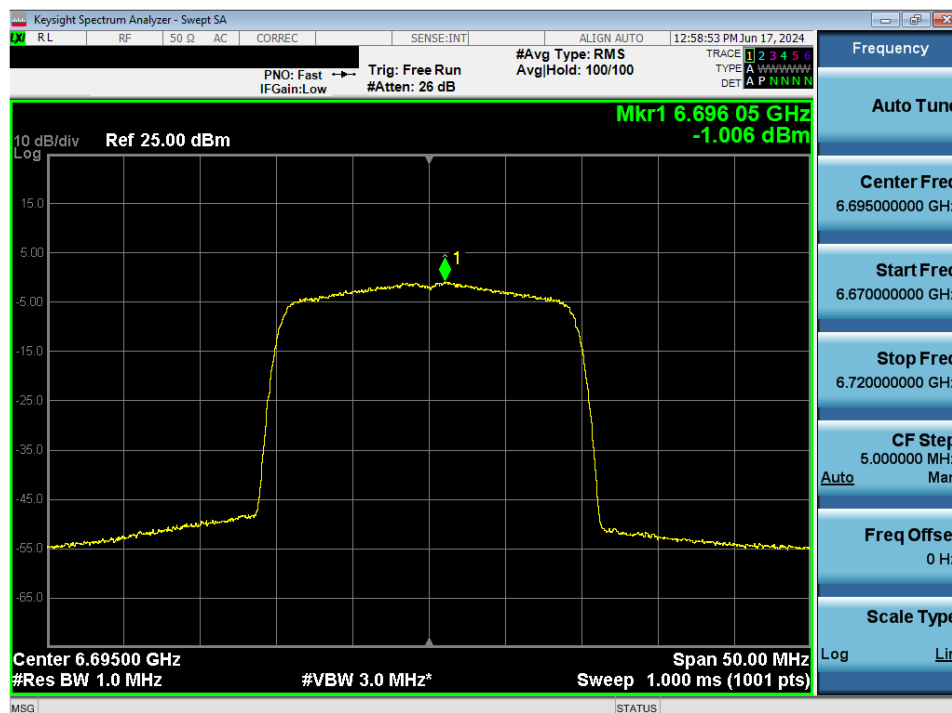
Plot 7-59. Power Spectral Density MIMO ANT1 (20MHz 802.11ax (UNII Band 7) – Ch. 149) - LPI/SP
