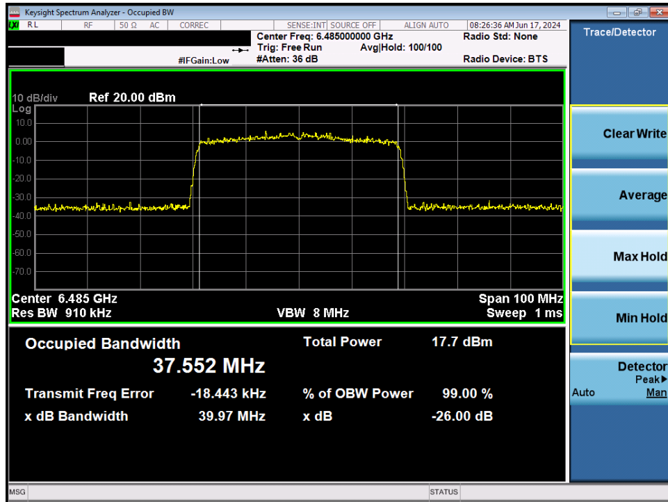
Plot 7-35. 26dB Bandwidth Plot MIMO ANT2 (40MHz 802.11ax (UNII Band 6) – Ch. 107)
