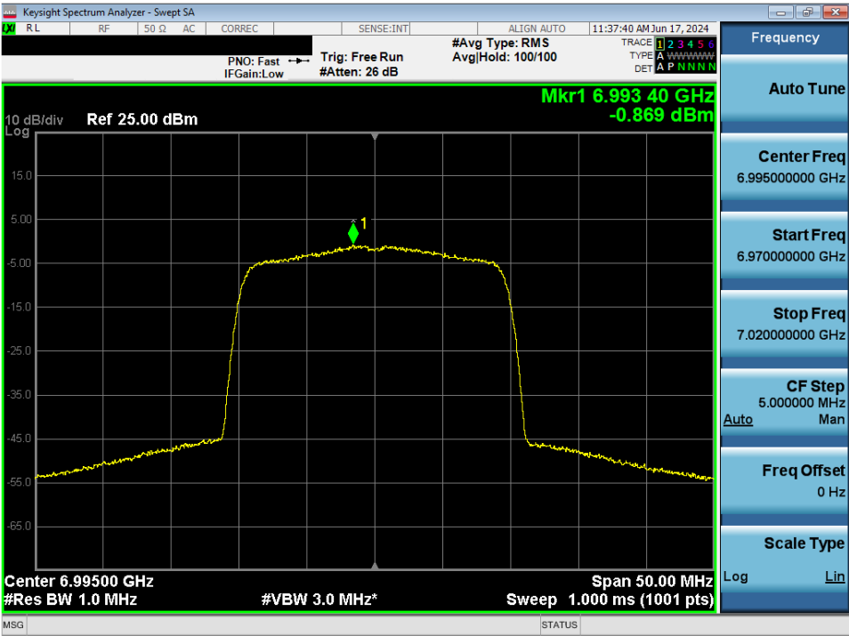
Plot 7-64. Power Spectral Density MIMO ANT1 (20MHz 802.11ax (UNII Band 8) – Ch. 209) - LPI
