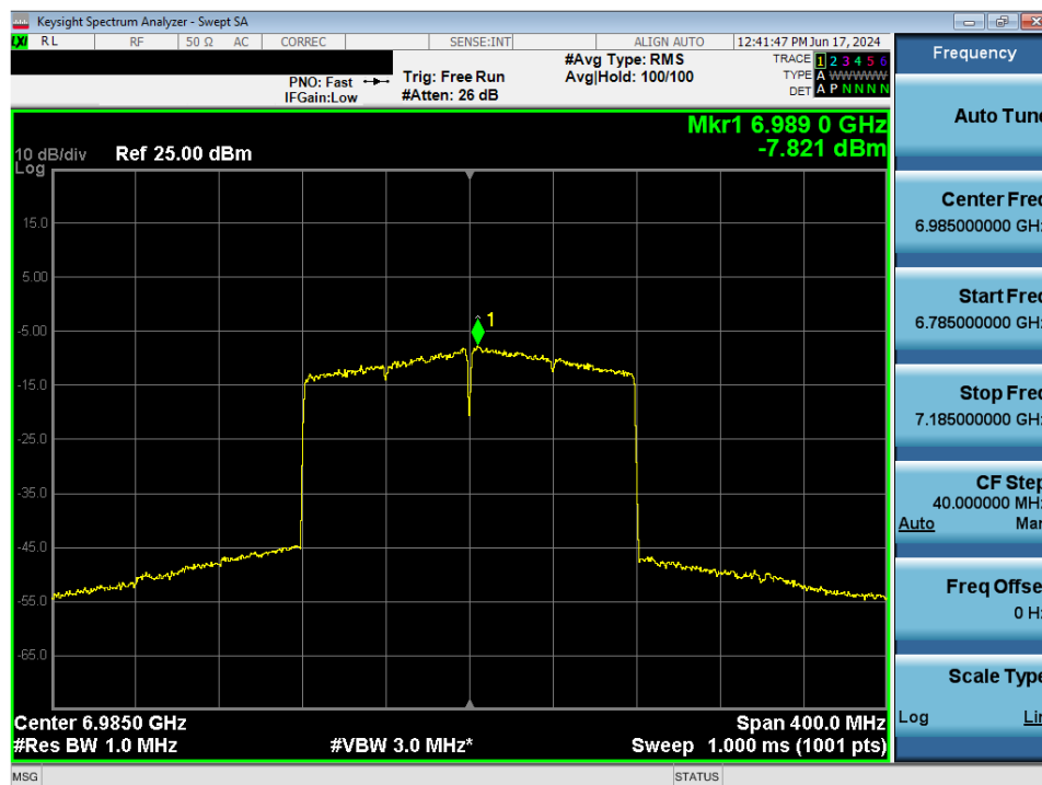
Plot 7-67. Power Spectral Density MIMO ANT1 (160MHz 802.11ax (UNII Band 8) – Ch. 207) - LPI
