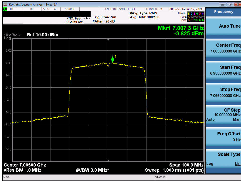
Plot 7-85. Power Spectral Density MIMO ANT2 (40MHz 802.11ax (UNII Band 8) – Ch. 211) - LPI
