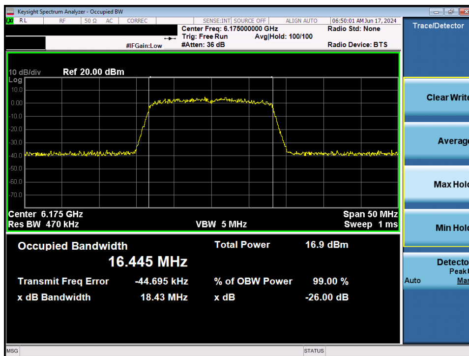
Plot 7-28. 26dB Bandwidth Plot MIMO ANT2 (20MHz 802.11a (UNII Band 5) – Ch. 45)
