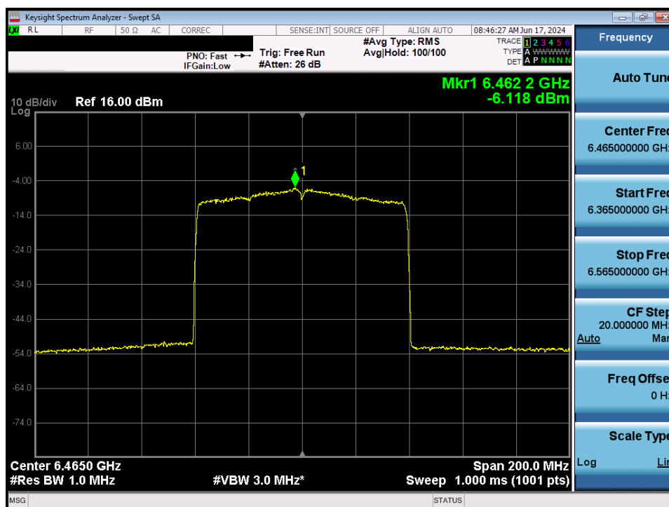
Plot 7-76. Power Spectral Density MIMO ANT2 (80MHz 802.11ax (UNII Band 6) – Ch. 103) - LPI
