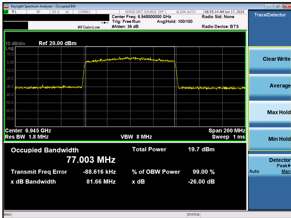
Plot 7-46. 26dB Bandwidth Plot MIMO ANT2 (80MHz 802.11ax (UNII Band 8) – Ch. 199)
