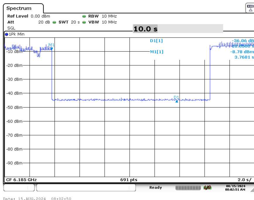
Plot 7-2. Contention Based Protocol Timing Plot (160MHz (UNII Band 5) – Ch. 47 Mid)
