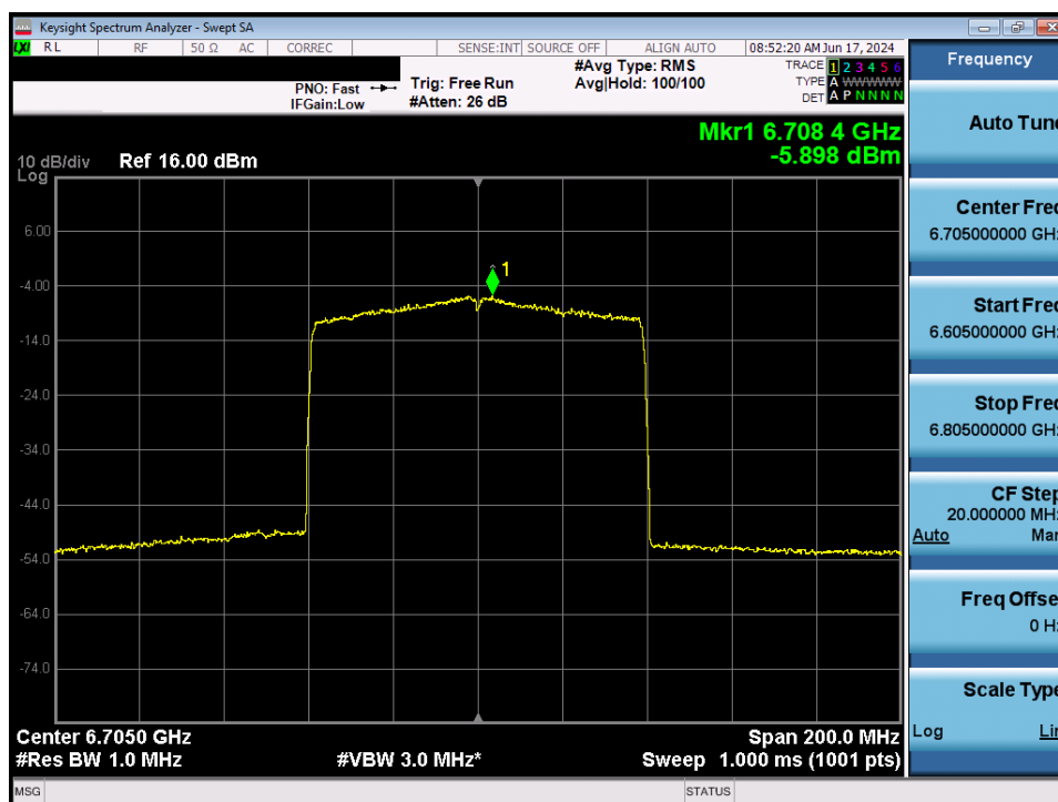
Plot 7-81. Power Spectral Density MIMO ANT2 (80MHz 802.11ax (UNII Band 7) – Ch. 151) - LPI/SP
