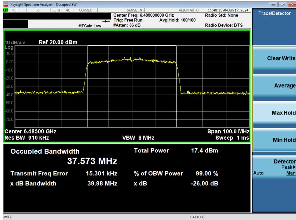
Plot 7-15. 26dB Bandwidth Plot MIMO ANT1 (40MHz 802.11ax (UNII Band 6) – Ch. 107)
