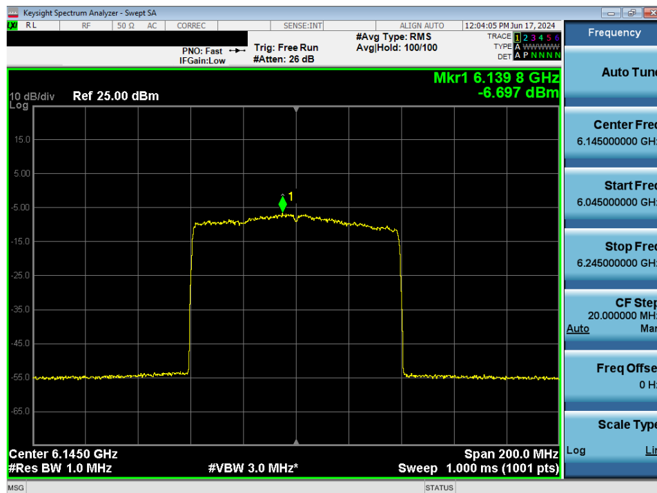
Plot 7-51. Power Spectral Density MIMO ANT1 (80MHz 802.11ax (UNII Band 5) – Ch. 39) - LPI/SP
