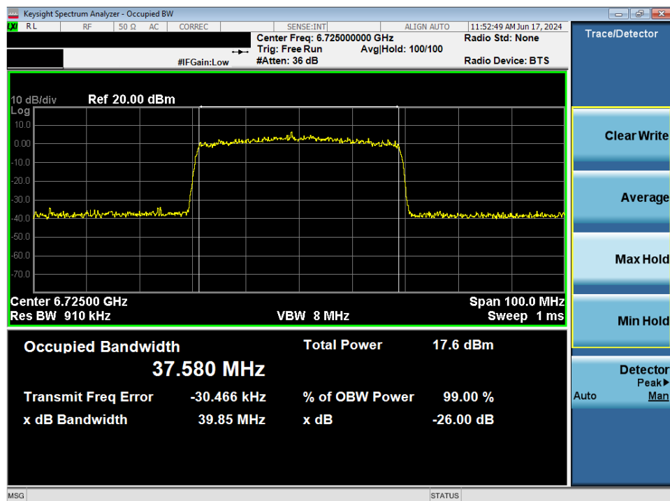
Plot 7-20. 26dB Bandwidth Plot MIMO ANT1 (40MHz 802.11ax (UNII Band 7) – Ch. 155)
