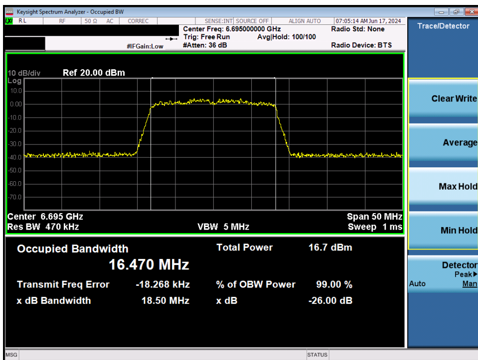
Plot 7-38. 26dB Bandwidth Plot MIMO ANT2 (20MHz 802.11a (UNII Band 7) – Ch. 149)
