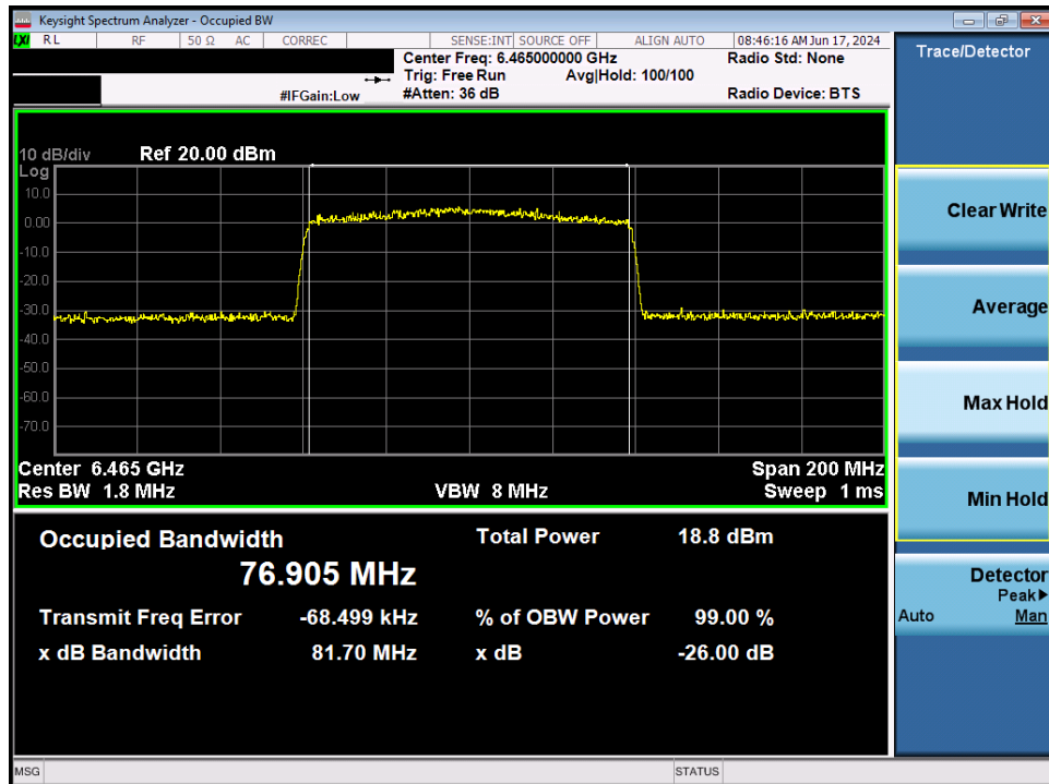
Plot 7-36. 26dB Bandwidth Plot MIMO ANT2 (80MHz 802.11ax (UNII Band 6) – Ch. 103)
