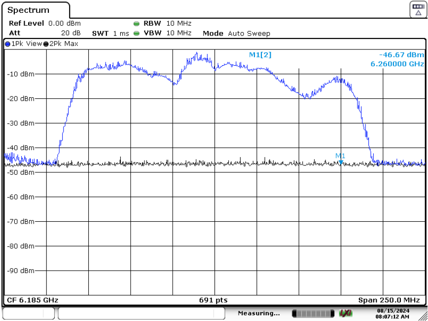
Plot 7-6. CBP 160MHz Channel - Injection Upper Edge – [6260 MHz]
