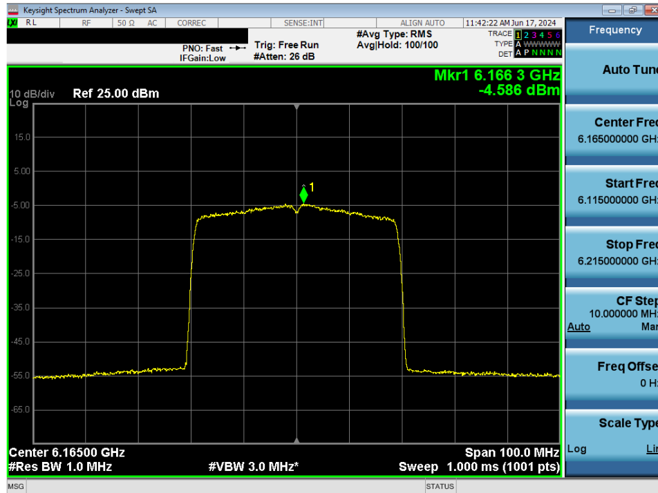
Plot 7-50. Power Spectral Density MIMO ANT1 (40MHz 802.11ax (UNII Band 5) – Ch. 43) - LPI/SP
