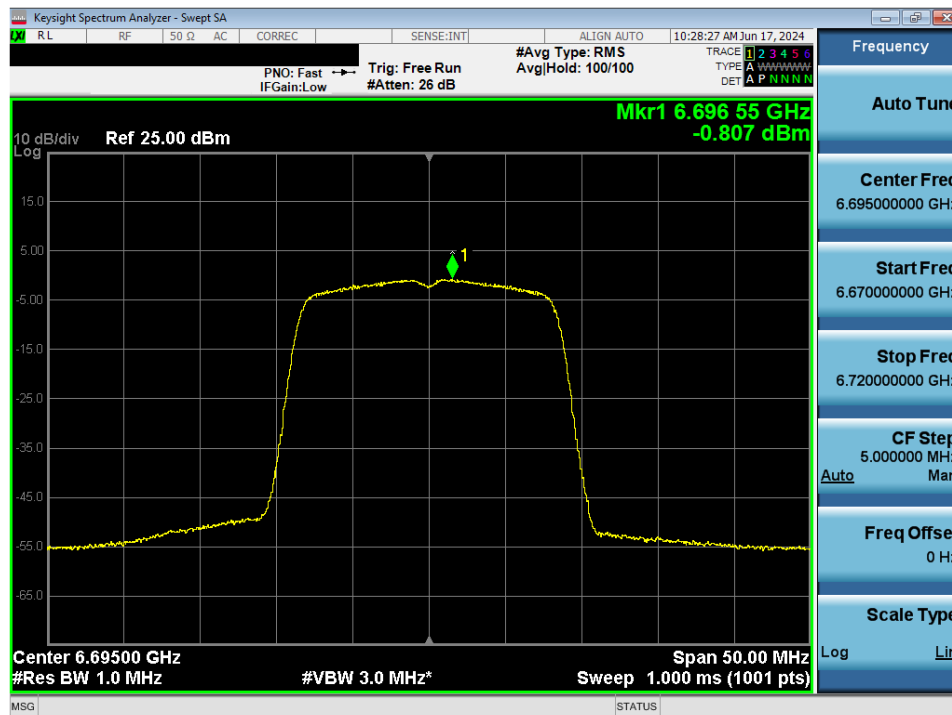
Plot 7-58. Power Spectral Density MIMO ANT1 (20MHz 802.11a (UNII Band 7) – Ch. 149) - LPI/SP
