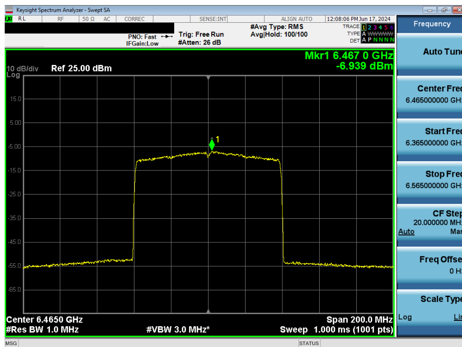
Plot 7-56. Power Spectral Density MIMO ANT1 (80MHz 802.11ax (UNII Band 6) – Ch. 103) - LPI
