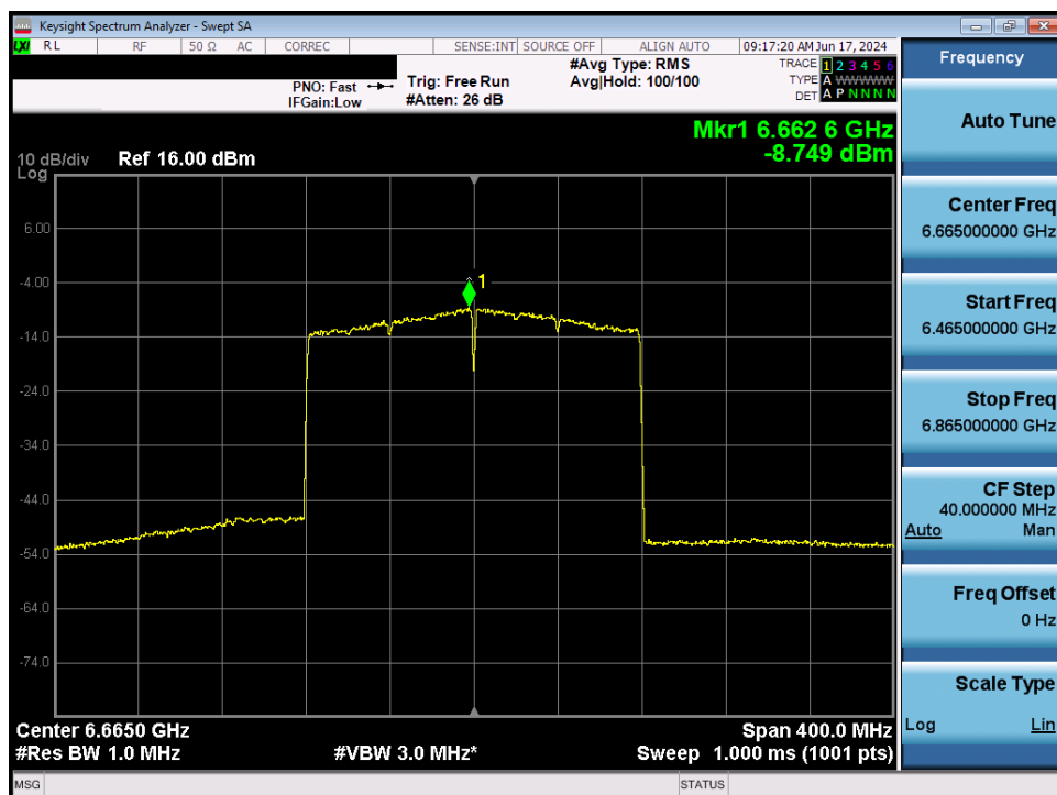
Plot 7-82. Power Spectral Density MIMO ANT2 (160MHz 802.11ax (UNII Band 7) – Ch. 143) - LPI/SP
