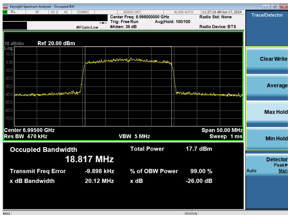
Plot 7-24. 26dB Bandwidth Plot MIMO ANT1 (20MHz 802.11ax (UNII Band 8) – Ch. 209)
