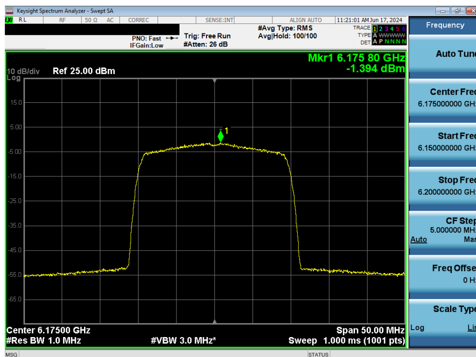
Plot 7-49. Power Spectral Density MIMO ANT1 (20MHz 802.11ax (UNII Band 5) – Ch. 45) - LPI/SP
