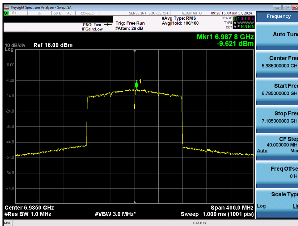
Plot 7-87. Power Spectral Density MIMO ANT2 (160MHz 802.11ax (UNII Band 8) – Ch. 207) - LPI
