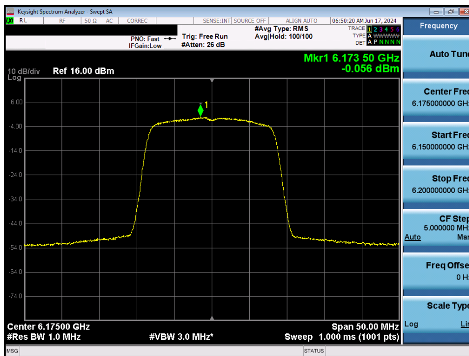
Plot 7-68. Power Spectral Density MIMO ANT2 (20MHz 802.11a (UNII Band 5) – Ch. 45) - LPI/SP
