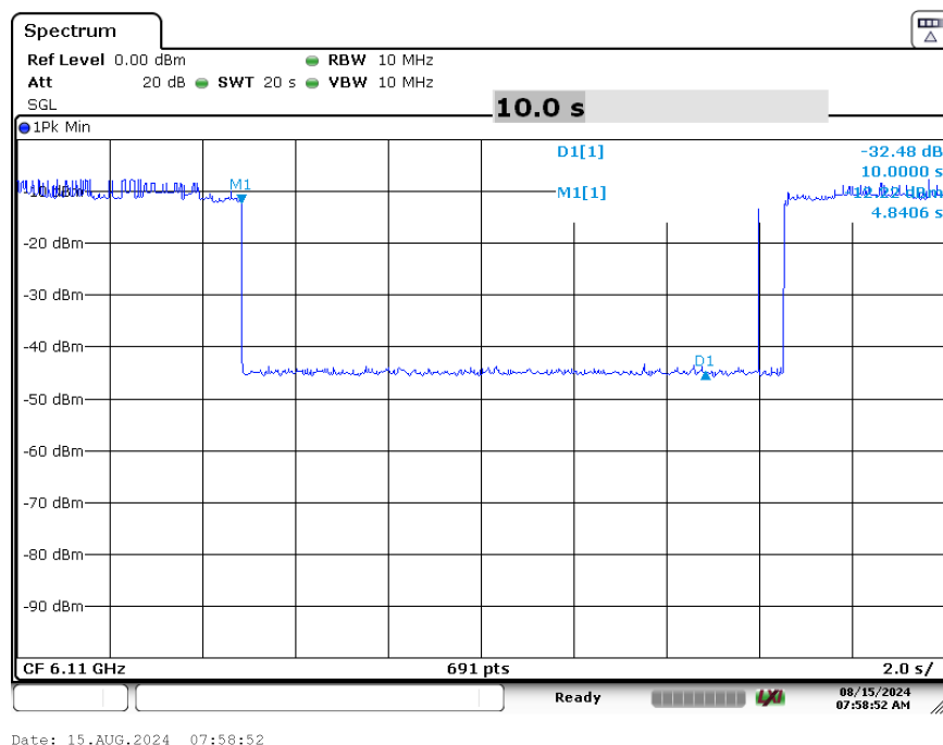
Plot 7-1. Contention Based Protocol Timing Plot (160MHz (UNII Band 5) – Ch. 47 Low)
