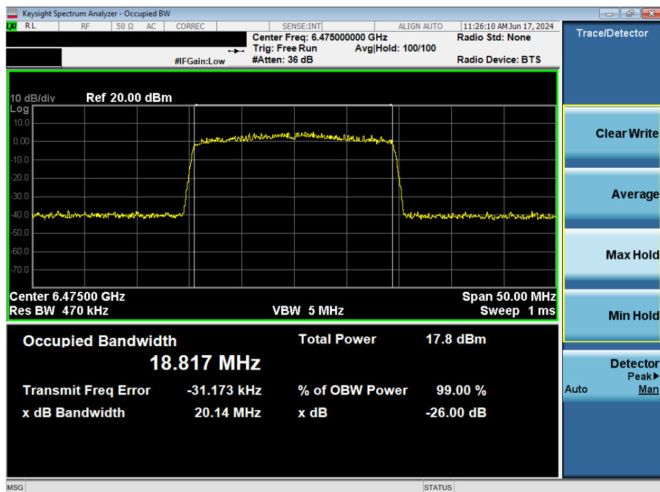
Plot 7-14. 26dB Bandwidth Plot MIMO ANT1 (20MHz 802.11ax (UNII Band 6) – Ch. 105)
