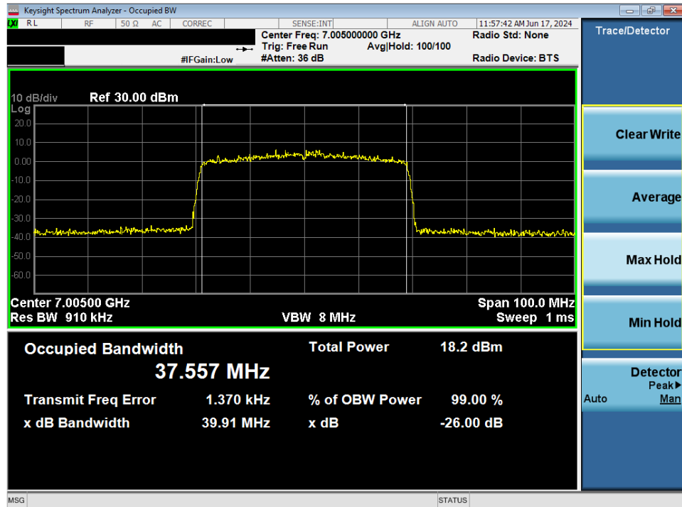
Plot 7-25. 26dB Bandwidth Plot MIMO ANT1 (40MHz 802.11ax (UNII Band 8) – Ch. 211)
