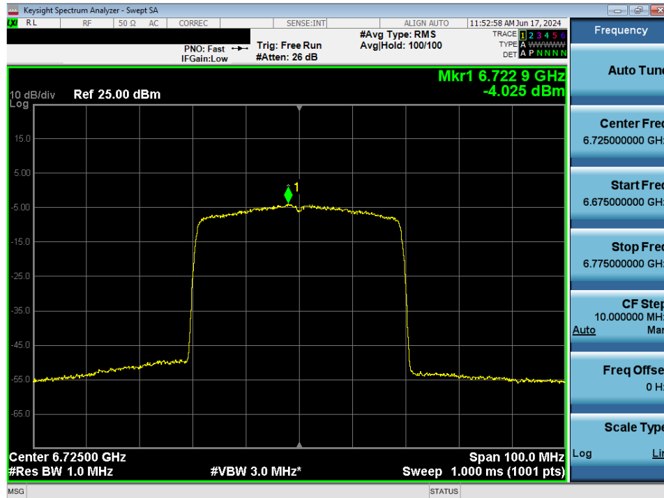
Plot 7-60. Power Spectral Density MIMO ANT1 (40MHz 802.11ax (UNII Band 7) – Ch. 155) - LPI/SP
