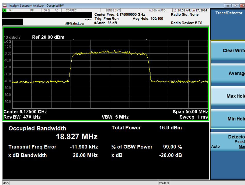
Plot 7-9. 26dB Bandwidth Plot MIMO ANT1 (20MHz 802.11ax (UNII Band 5) – Ch. 45)
