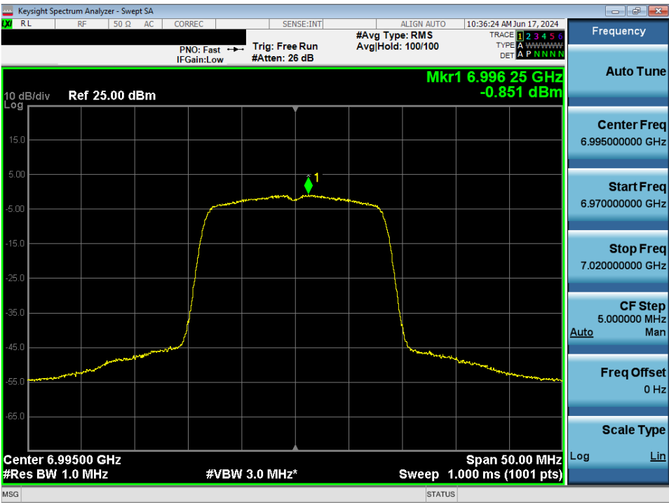
Plot 7-63. Power Spectral Density MIMO ANT1 (20MHz 802.11a (UNII Band 8) – Ch. 209) - LPI
