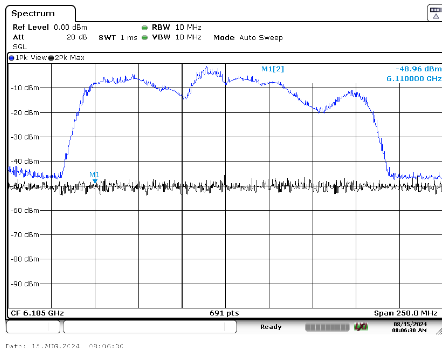
Plot 7-4. CBP 160MHz Channel - Injection Lower Edge – [6110 MHz]
