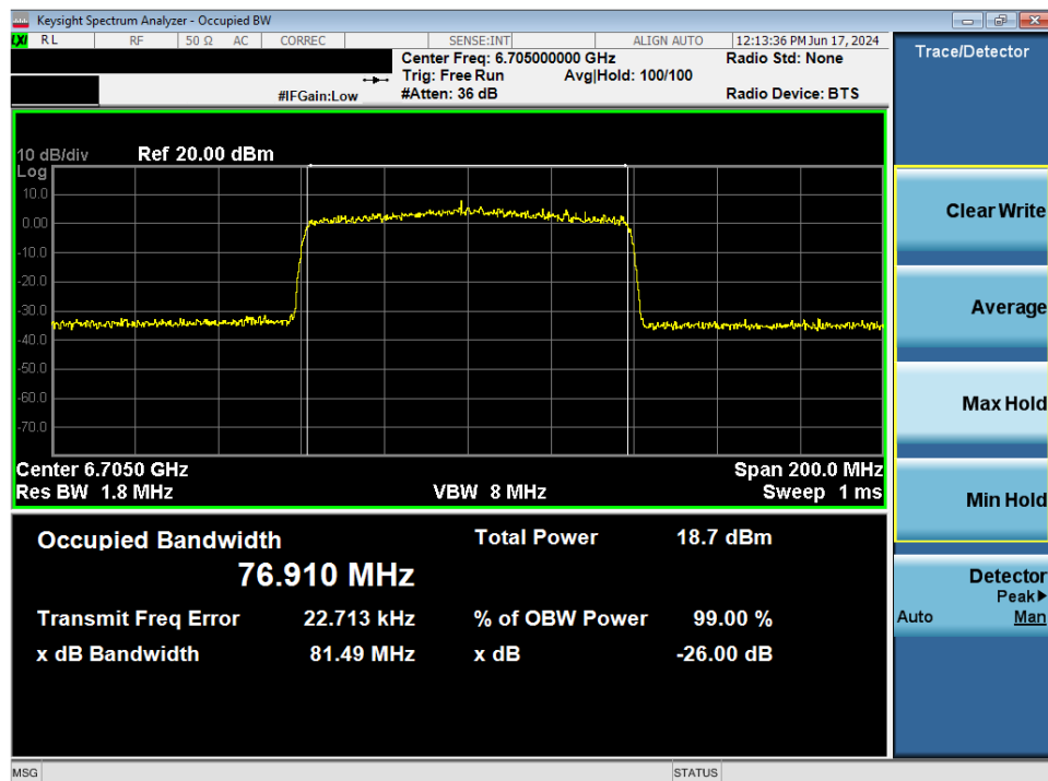
Plot 7-21. 26dB Bandwidth Plot MIMO ANT1 (80MHz 802.11ax (UNII Band 7) – Ch. 151)
