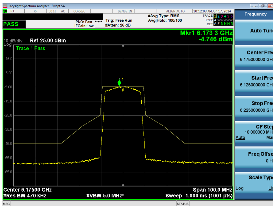
Plot 7-88. In-Band Emission MIMO ANT1 (20MHz 802.11a (UNII Band 5) – Ch. 45)
