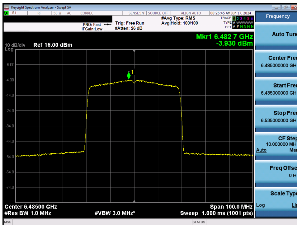
Plot 7-75. Power Spectral Density MIMO ANT2 (40MHz 802.11ax (UNII Band 6) – Ch. 107) - LPI
