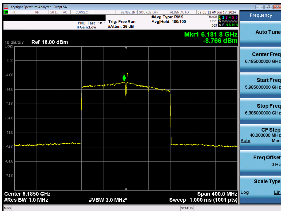
Plot 7-72. Power Spectral Density MIMO ANT2 (160MHz 802.11ax (UNII Band 5) – Ch. 47) - LPI/SP
