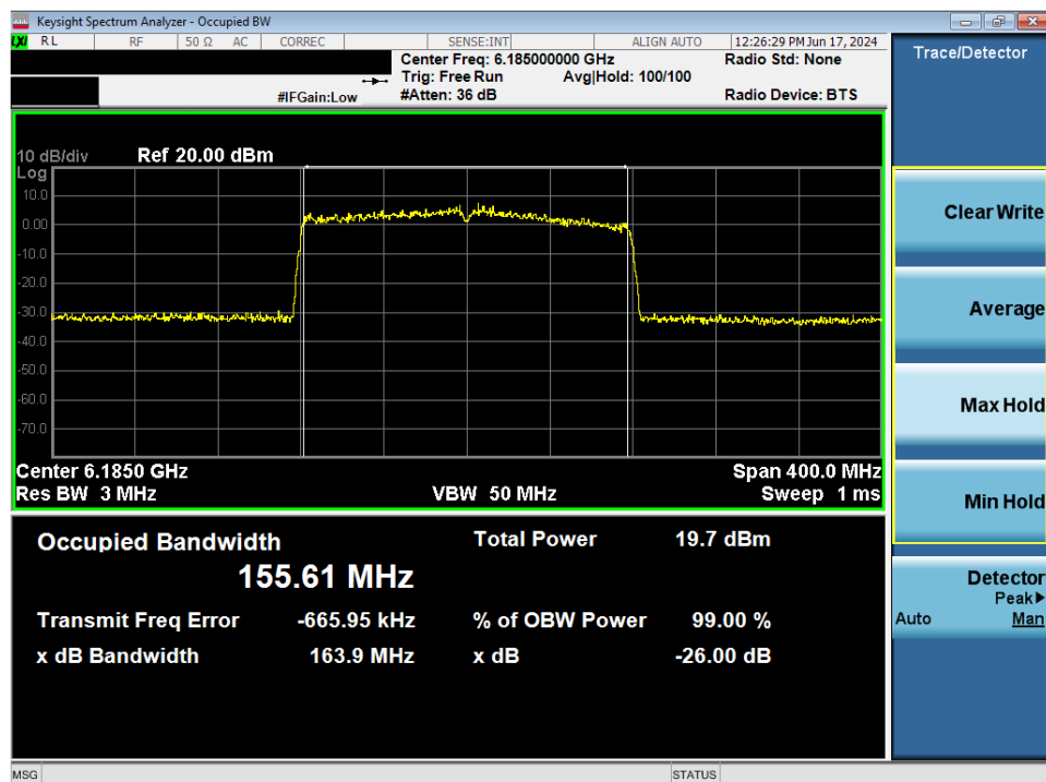
Plot 7-12. 26dB Bandwidth Plot MIMO ANT1 (160MHz 802.11ax (UNII Band 5) – Ch. 47)
